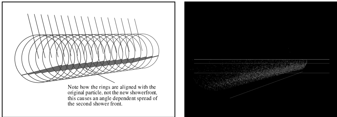
FIGURE 5. a) Depicts a toy model EAS incident on the pond at an angle. Note again the double front, with the second front showing angle dependent smearing. b) A still from a full Monte Carlo animation of the toy model EAS. The angled line shows where the particles of the EAS would be if they had not encountered the pond. Close examination of this image shows the refraction, bifurcation, and angle dependent smearing predicted by the bowl-ring model of Cherenkov light emission. The full animation can be seen in Web Figure 3.
