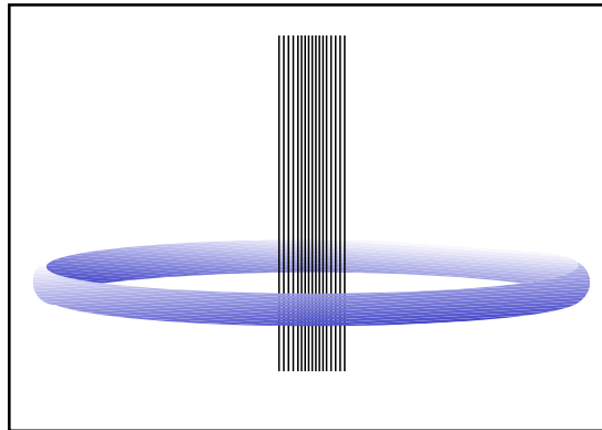
FIGURE 2. The particles of the EAS core are travelling colinearly as they enter the pond. The Cherenkov rings from each particle add to form one bright Cherenkov ring.
