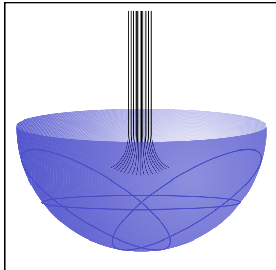
FIGURE 3. As the particles in the EAS core penetrate into the pond they suffer multiple scattering. This scatters the orientation of the individual Cherenkov rings. The individual rings no longer add to form one ring, but instead form the surface of a bowl. Combining the ring from when the particles first enter the pond and the bowl formed due to multiple scattering gives the bowl and ring structure observed in the computer animations.
