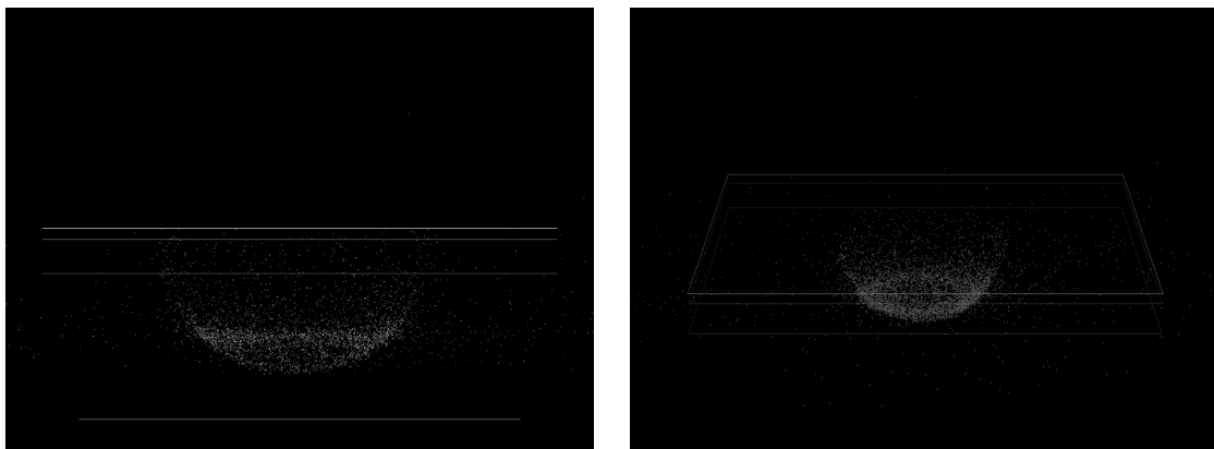
FIGURE 1. These stills show an EAS from a 2 TeV gamma primary as it interacts with the Milagro pond. a) The pond viewed from the side with the top horizontal line representing the surface of the pond, and the next two lines representing the layers of photo detectors. Almost all of the particles seen in this image are Cherenkov photons. Notice the bowl structure of Cherenkov light. b) The same shower from a slightly elevated perspective to clearly show the three dimensional structure of the Cherenkov light emission. Note the distinctive bowl and ring shape, not just the classic Cherenkov ring. The full color animation these stills are derived from can be seen in Web Figure 1 at http://scipp.ucsc.edu/milagro/Animations/Snowbird99.html .
