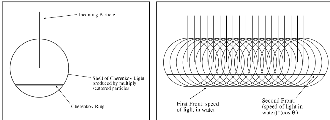
FIGURE 4. a) This diagram sketches the probability density of Cherenkov light emission from a single incoming particle. b) A plane particles from zenith with all emit photons in the same bowl-ring structure. The bowls add to form a leading photon front that travels at the speed of light in water. The rings add to form a secondary front that propagates more slowly. This diagram also shows that there is a lot of diffuse light that not associated with either front.
