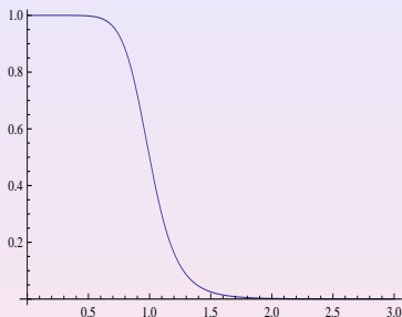
Figure: z-scaling distribution (297), \Psi(z, 9, 9, 1, 1)
