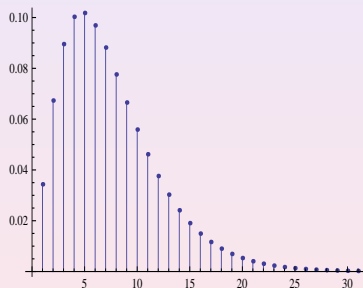
Figure: P(n) , (168), r = 2.8 , p = 0.3 , \langle n \rangle = 6
