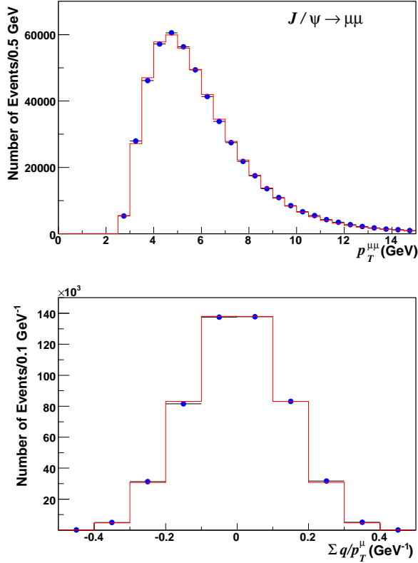
FIG. 21: The J/\psi \rightarrow \mu\mu data (points) and tuned simulation (histogram) distributions of p_T^{\mu\mu} (top) and \sum q/p_T^{\mu} (bottom). The \sum q/p_T^{\mu} is equal to the sum of the track curvatures of muons from a J/\psi decay, divided by 2.11593 \times 10^{-3} .
