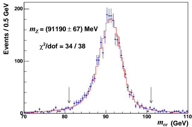
FIG. 31: The m_Z fit to data (points) in the 81 \text{ GeV} < m_{ee} < 101 \text{ GeV} region (denoted by arrows). The uncertainty is statistical only.
