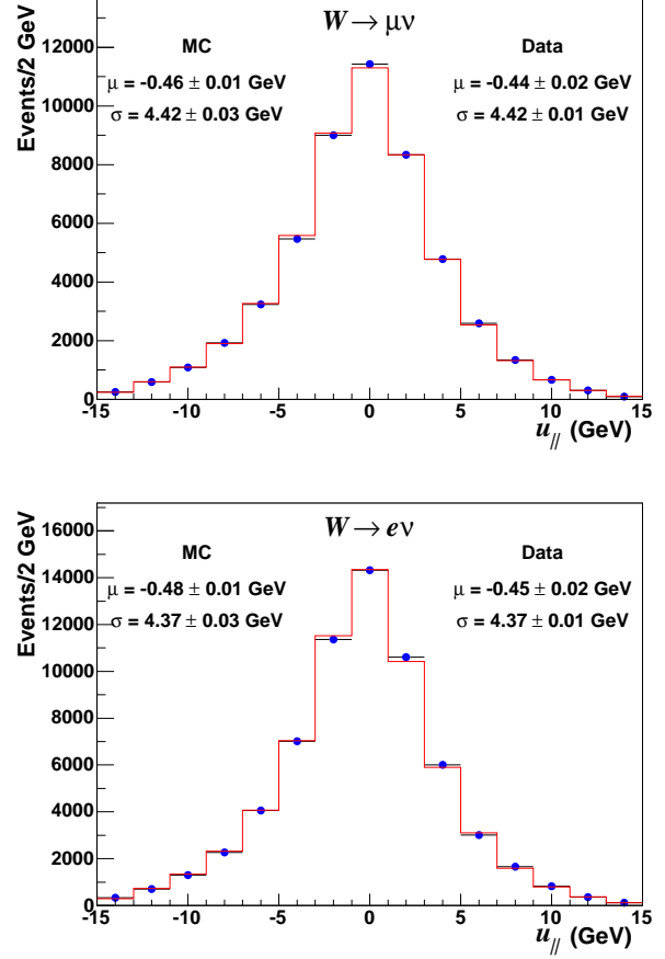
FIG. 42: The simulation (solid) and data (circles) u_{\parallel} distributions for W boson decays to \mu\nu (top) and e\nu (bottom). The simulation uses parameters fit from Z boson data, and the uncertainty on the simulation is due to the statistical uncertainty on these parameters. The data mean ( \mu ) and RMS ( \sigma ) are well-modeled by the simulation.
