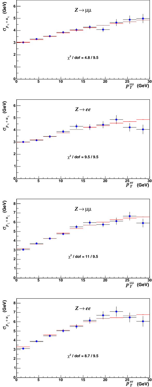
FIG. 41: The simulation (solid) and data (circles) p_{\eta}^{\parallel} + u_{\eta} (top) and p_{\xi}^{\parallel} + u_{\xi} (bottom) resolutions for Z boson decays to muons and electrons. The sum of the four \chi^2 values is minimized in the fit for the recoil resolution parameters N_{W,Z} and s_{hard} . Since there are four distributions and two fit parameters, each distribution contributes half a degree of freedom to the fit.
