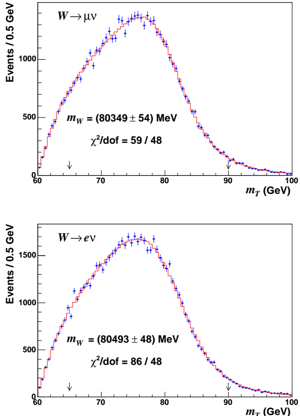
FIG. 51: The simulation (solid) and data (points) m_T distributions for W boson decays to \mu\nu (top) and e\nu (bottom). The simulation corresponds to the best-fit m_W , determined using events between the two arrows. The uncertainty is statistical only. The large \chi^2 for the electron fit is due to individual bin fluctuations (Fig. 55) and does not bias the fit result, as evidenced by the small change in the fit m_W when the fit window is varied (Fig. 58).
