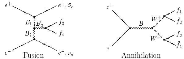
Fig. 1. Four-fermion production classes of diagrams in e^+e^- annihilation following the convention of [1]: B = Z, \gamma and B_1, B_2, B_3 = Z, \gamma, W^\pm . Diagrams involving Higgs boson exchange are not shown
