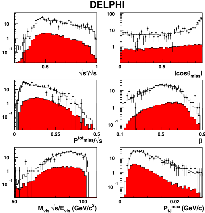
Fig. 2. ev_e W channel ( W \rightarrow q\bar{q}' ) at \sqrt{s} = 200 GeV. Distribution of some Neural Network input variables, as defined in the text, in the real data (points with error bars) and in the simulation of the Standard Model predictions (histograms) after the preselection stage (see text). The distributions of these variables for the ev_e W signal are shown as well (filled histograms). The |\cos\theta_{\text{miss}}| distribution (top-right) stops at 0.98, as explained in the text
