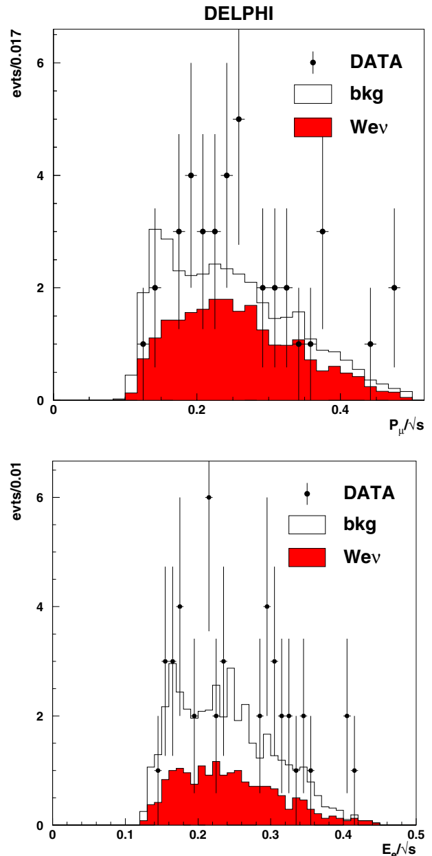
Fig. 4. e\nu_e W channel ( W \rightarrow l^+ \nu_l ) summed over all centre-of-mass energies: momentum distribution of the muon (top) and energy distribution of the electron (bottom) in the real data (points with error bars) and in the simulation of the Standard Model predictions (histograms) for the events selected at the end of the analysis. The filled histograms represent the single- W signal, the open area is the background expectation
