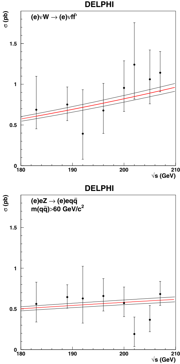
Fig. 8. Cross-sections as a function of \sqrt{s} for the \nu_e W channel (top) and the Zee channel Zee \rightarrow e^+e^-q\bar{q} (bottom). The solid curves are the Standard Model predictions, with a 5% uncertainty band, computed with WPHACT [12]
