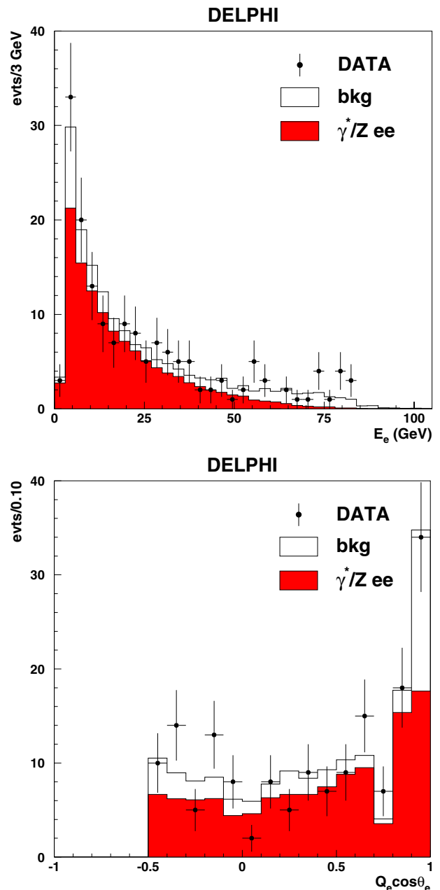
Fig. 7. \gamma^*/Zee channel summed over all centre-of-mass energies: energy spectrum (top) and signed angle Q_e \cos \theta_e , (bottom) of the tag electron for hadronic and \mu^+\mu^- final states with m_{f\bar{f}} > 60 GeV/ c^2 , in the selected signal sample. The points with error bars represent real data, the histograms the simulation
