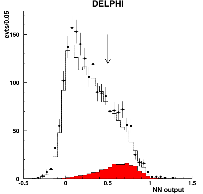
Fig. 3. ev_e W channel ( W \rightarrow q\bar{q}' ) summed over all centre-of-mass energies: distribution of the Neural Network output variable in the real data (points with error bars) and in the simulation of the Standard Model predictions (histograms). The filled histogram represents the single- W signal, the open area is the background expectation. The arrow indicates the cut applied on this variable for the final event selection
