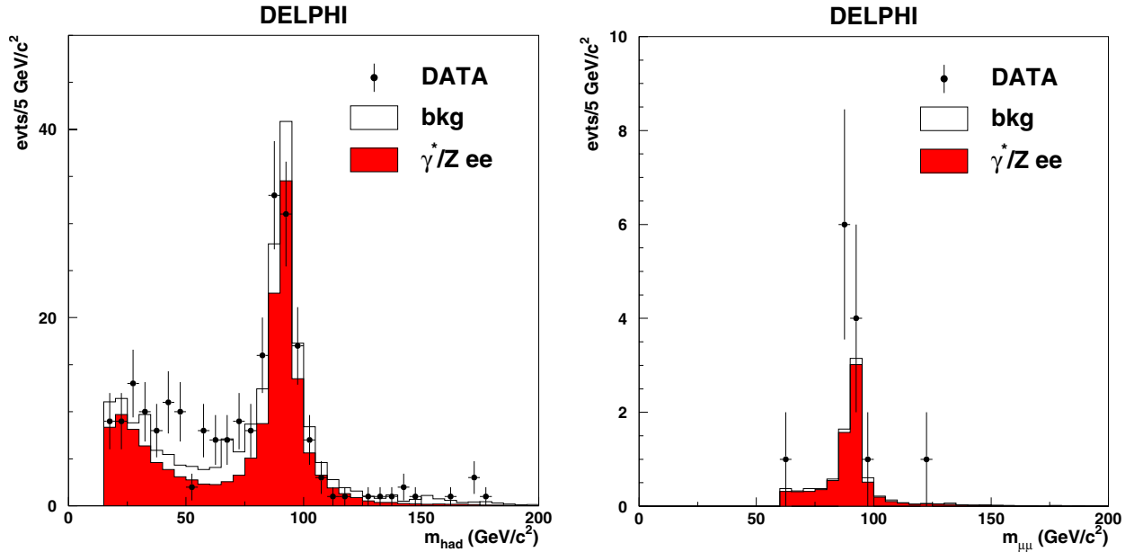
Fig. 6. \gamma^*/Zee channel summed over all centre-of-mass energies: invariant mass distribution of the \gamma^*/Z system in the real data (points with error bars) and in the simulation of the Standard Model predictions (histograms) for hadronic (left) and \mu^+\mu^- (right) final states, in the selected signal sample
