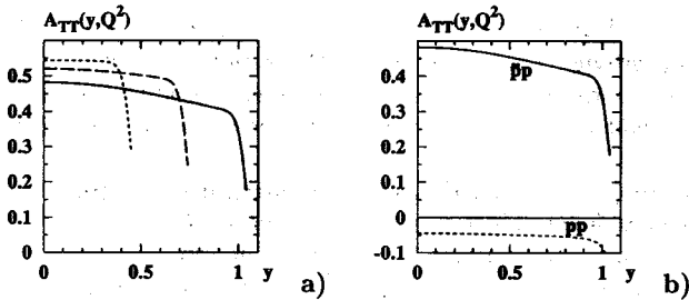
Figure 1: a) The asymmetry A_{TT}(y, M^2) at PAX as a function of the rapidity y for Q^2 = 5 \text{ GeV}^2 (solid) and 9 \text{ GeV}^2 (dashed) and 16 \text{ GeV}^2 (dotted line) for s = 45 \text{ GeV}^2 . b) Comparison of A_{TT}(y, M^2) from proton-antiproton (solid) and proton-proton (dotted line) collisions for Q^2 = 5 \text{ GeV}^2 .
