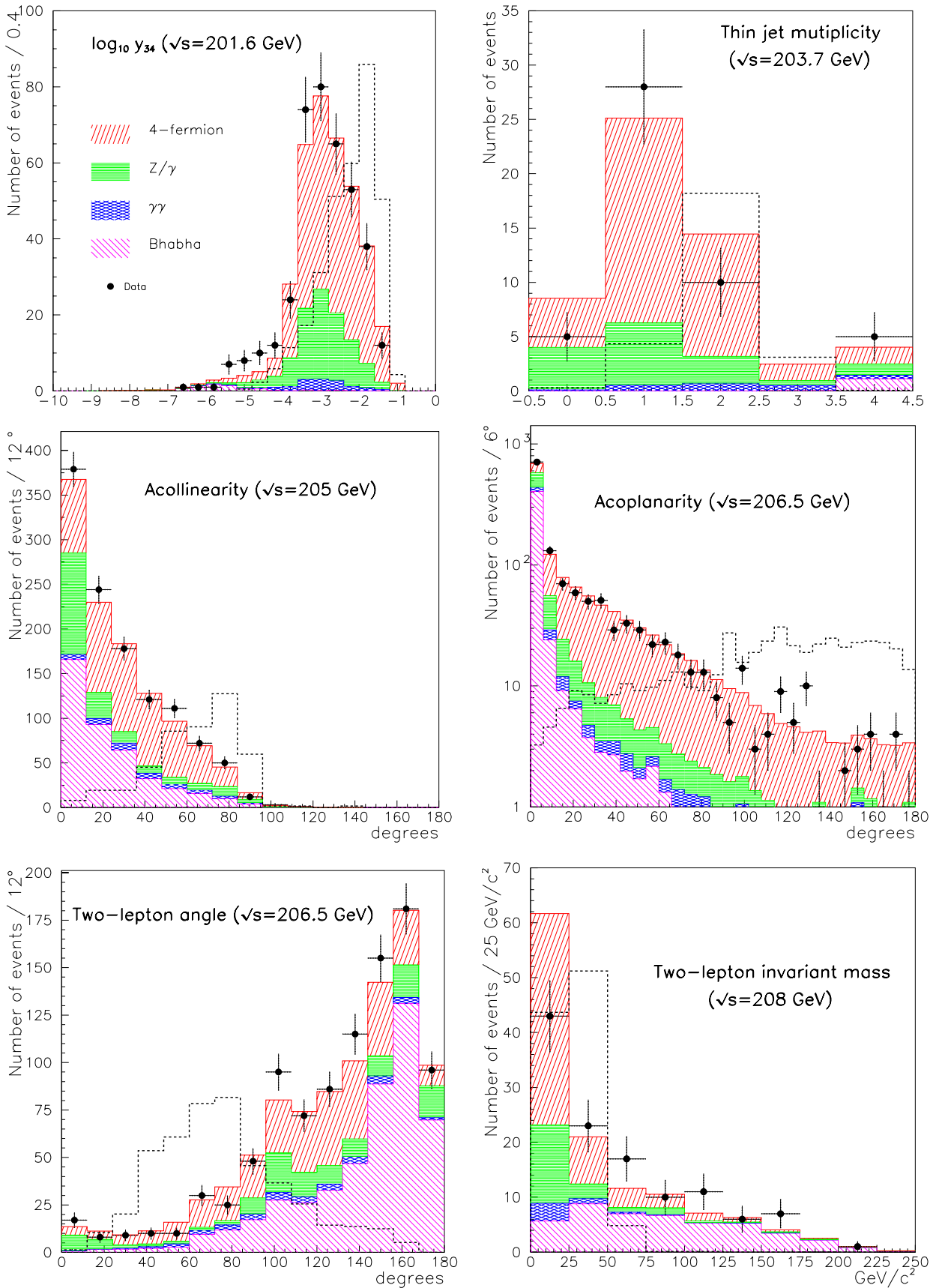
Fig. 3. Additional examples of data-simulation comparison at preselection level (the \log_{10} y_{34} and jet multiplicity distributions are given for events with at least four charged particles). The dashed lines are examples of signal distributions (see text)
