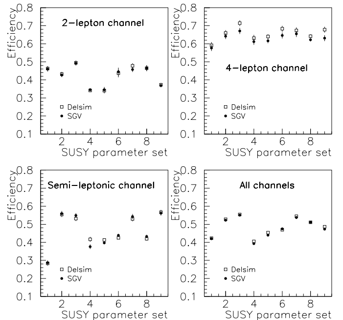
Fig. 4. SGV-DELSIM comparison for nine SUSY parameter sets with different sneutrino masses and total widths (see Table 2) in the case of a \lambda_{121} coupling and for \tan\beta = 1.5 , \sqrt{s} = 206.5 GeV. For this comparison, the same number of events was simulated with SGV and DELSIM
