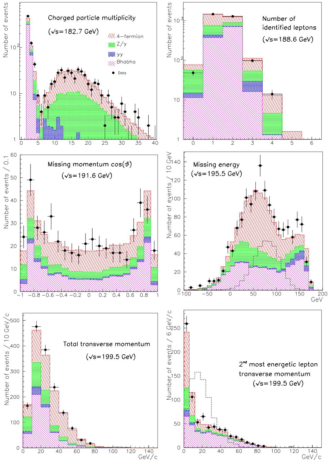
Fig. 2. Examples of data-simulation comparison at preselection level. The dashed lines are examples of signal distributions (see text)
