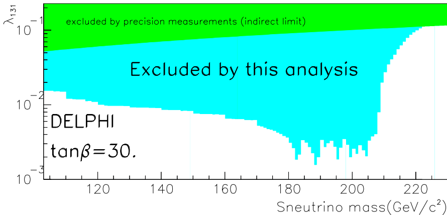
Fig. 8. For \tan\beta = 30 , upper limit on \lambda_{131} as a function of M_{\tilde{\nu}} and \Gamma_{\tilde{\nu}} ( top ) and as a function of M_{\tilde{\nu}} assuming \Gamma_{\tilde{\nu}} > 150 \text{ MeV}/c^2 ( bottom ). The white zone in the top plot corresponds to non existing sneutrino widths given the \mu parameter range. The area entitled ‘no limit on \lambda' ’ corresponds to upper limits larger than 0.1. The indirect limit coming from precision measurements is drawn in the bottom plot assuming M_{\tilde{e}_R} = M_{\tilde{\nu}}
