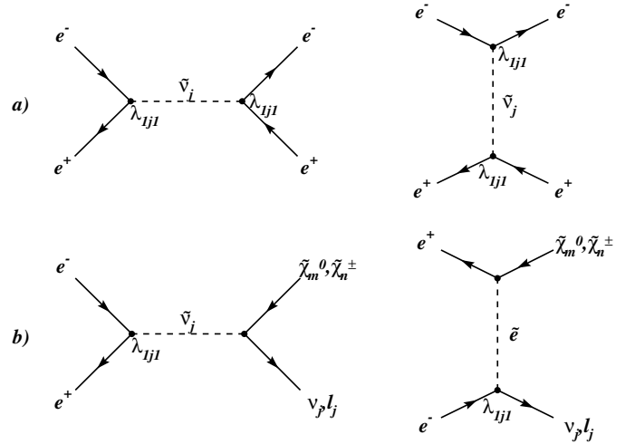
Fig. 1a,b. Lowest order Feynman diagrams for single sneutrino production and decay: a direct decay, b indirect decay ( \nu_j = \nu_\mu, \nu_\tau ; l_j = \mu, \tau ; m = 1, 4 ; n = 1, 2 )
