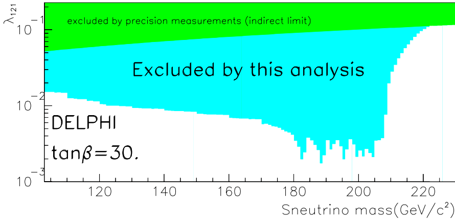
Fig. 6. For \tan\beta = 30 , upper limit on \lambda_{121} as a function of M_{\tilde{\nu}} and \Gamma_{\tilde{\nu}} ( top ) and as a function of M_{\tilde{\nu}} assuming \Gamma_{\tilde{\nu}} > 150 \text{ MeV}/c^2 ( bottom ). The white zone in the top plot corresponds to non existing sneutrino widths given the \mu parameter range. The area entitled ‘no limit on \lambda' ’ corresponds to upper limits larger than 0.1. The indirect limit coming from precision measurements is drawn in the bottom plot assuming M_{\tilde{e}_R} = M_{\tilde{\nu}}
