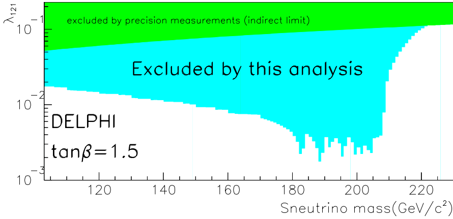
Fig. 5. For \tan\beta = 1.5 , upper limit on \lambda_{121} as a function of M_{\tilde{\nu}} and \Gamma_{\tilde{\nu}} ( top ) and as a function of M_{\tilde{\nu}} assuming \Gamma_{\tilde{\nu}} > 150 \text{ MeV}/c^2 ( bottom ). The white zone in the top plot corresponds to non existing sneutrino widths given the \mu parameter range. The area entitled ‘no limit on \lambda' ’ corresponds to upper limits larger than 0.1. The indirect limit coming from precision measurements is drawn in the bottom plot assuming M_{\tilde{e}_R} = M_{\tilde{\nu}}
