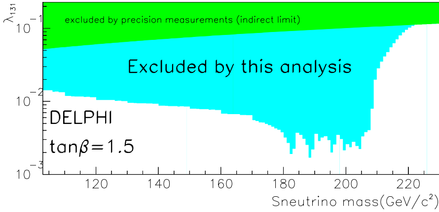
Fig. 7. For \tan\beta = 1.5 , upper limit on \lambda_{131} as a function of M_{\tilde{\nu}} and \Gamma_{\tilde{\nu}} ( top ) and as a function of M_{\tilde{\nu}} assuming \Gamma_{\tilde{\nu}} > 150 \text{ MeV}/c^2 ( bottom ). The white zone in the top plot corresponds to non existing sneutrino widths given the \mu parameter range. The area entitled ‘no limit on \lambda' ’ corresponds to upper limits larger than 0.1. The indirect limit coming from precision measurements is drawn in the bottom plot assuming M_{\tilde{e}_R} = M_{\tilde{\nu}}
