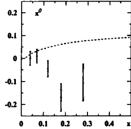
A_{UT}^{\text{sin}(\phi^{++})}(x) vs. HERMES preliminary
