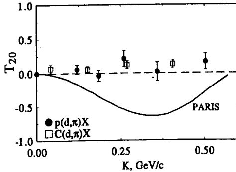
Fig. 3: SPHERE Collaboration. Measurement of the tensor analyzing power T_{20} in inclusive polarized deuteron fragmentation into pion at zero angle.
