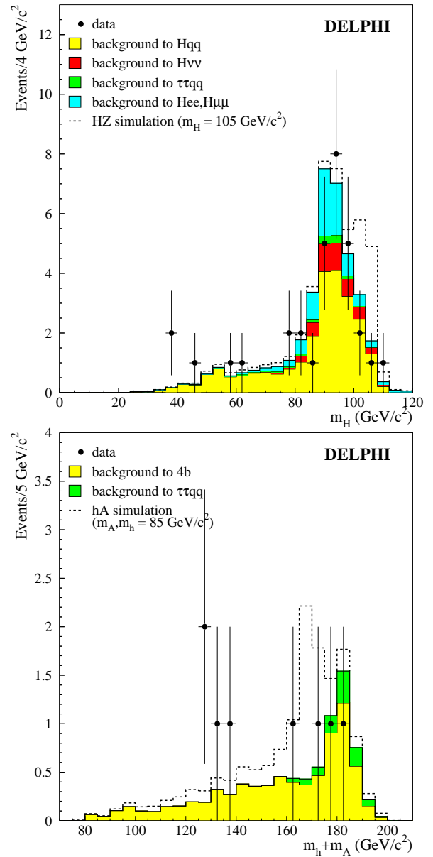
Fig. 11. Distribution of the reconstructed Higgs boson mass(es) when combining all HZ or hA analyses at 191.6-201.7 GeV. Data (dots) are compared with SM background expectations (full histograms) and with the normalised signal spectrum added to the background contributions (dashed histogram). Mass hypotheses for the simulated signal spectra are m_H = 105 GeV/c 2 in the HZ channel and m_A = 85 GeV/c 2 , \tan\beta = 20 in the hA channel
