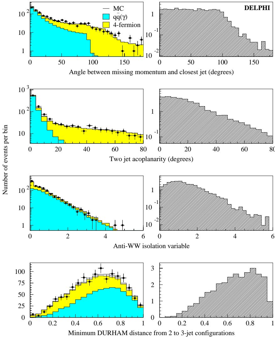
Fig. 5. H\nu\bar{\nu} channel: distributions of four analysis variables, as described in the text, at preselection level. Data at \sqrt{s} = 191.6 – 201.7 GeV (dots) are compared with SM background expectations (left-hand side histograms) and with the expected distribution for a 105 \text{ GeV}/c^2 signal (right-hand side histogram, normalised to 10 times the expected rate)
