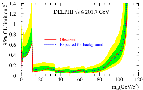
Fig. 14. 95% CL upper bound on \xi^2 , where \xi is the HVV ( V=W^\pm or Z ) coupling normalised to that in the SM, assuming SM branching fractions for the Higgs boson. The limit observed in data (solid line) is shown together with the expected median limit in background-only experiments (dashed line). The bands correspond to the 68.3% and 95.0% confidence intervals from background-only experiments. Most of the jumps below 40 GeV/ c^2 correspond to the different analyses applied to different subsets of LEP1 data to cover the various topologies expected from a Higgs boson. The jumps at 12, 50 and 65 GeV/ c^2 indicate where the LEP2 results at 191.6-201.7, 182.7 and 188.7 GeV/ c^2 respectively start to contribute
