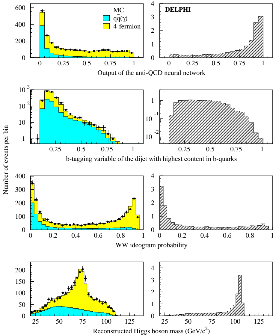
Fig. 7. Hq\bar{q} channel: distributions of four analysis variables, as described in the text, at preselection level. Data at \sqrt{s} = 191.6 -201.7 GeV (dots) are compared with SM background expectations (left-hand side histograms) and with the expected distribution for a 105 \text{ GeV}/c^2 signal (right-hand side histogram, normalised to the expected rate)
