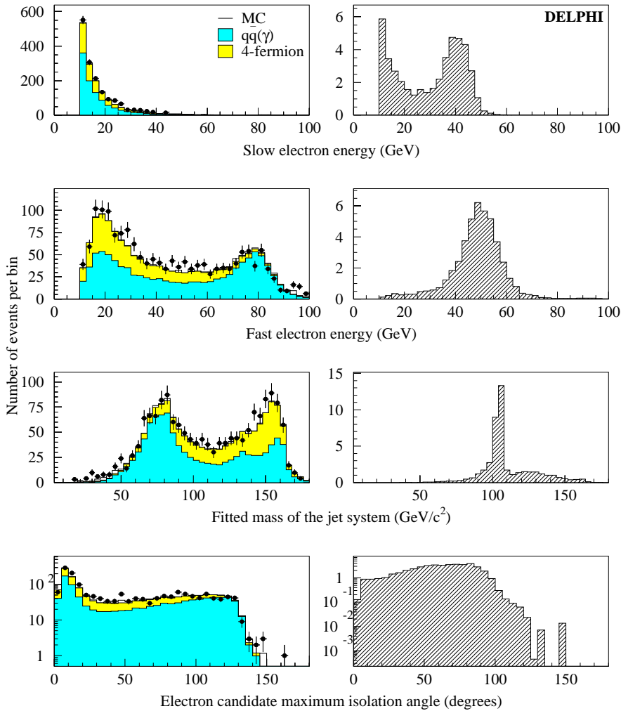
Fig. 2. He^+e^- channel: distributions of four analysis variables, as described in the text, at preselection level. Data at \sqrt{s} = 191.6 -201.7 GeV (dots) are compared with SM background expectations (left-hand side histograms) and with the expected distribution for a 105 \text{ GeV}/c^2 signal (right-hand side histogram, normalised to 50 times the expected rate)
