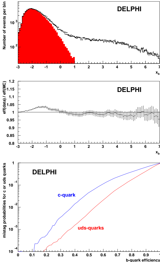
Fig. 1. b-tagging: Top: distributions of the combined b-tagging variable x_b , in 1999 Z data (dots) and simulation (histogram). The contribution of udsc -quarks is shown as the dark histogram. Middle: ratio of integrated tagging rates in Z data and simulation as a function of the cut in x_b . Bottom: mistag probabilities for c or uds-quarks as a function of the efficiency for b-quarks, estimated from simulated Z data
