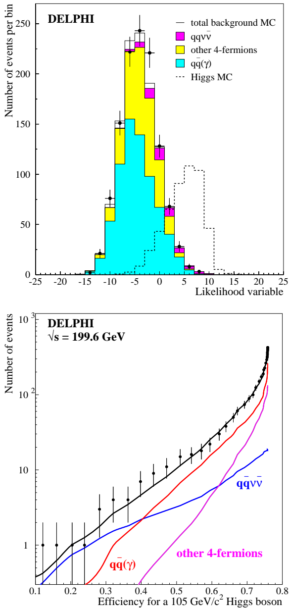
Fig. 6. H\nu\bar{\nu} channel: Top: distributions of the likelihood variable for the expected SM backgrounds (full histograms), 191.6–201.7 GeV data (dots) and the expected Higgs signal at 105 \text{GeV}/c^2 (dashed histogram, normalised to 100 times the expected rate). Bottom: curve of the expected SM background rate at \sqrt{s} = 199.6 GeV as a function of the efficiency for a 105 \text{GeV}/c^2 Higgs signal when varying the cut on the likelihood variable. The different background contributions are shown separately. The dots represent the data
