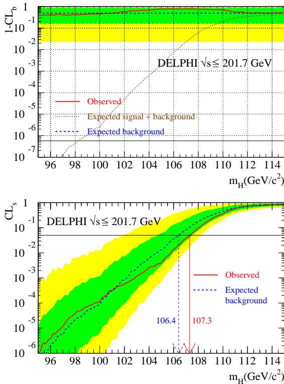
Fig. 12. SM Higgs boson: confidence levels as a function of m_H . Curves are the observed (solid) and expected median (dashed) confidences from background-only experiments while the bands correspond to the 68.3% and 95.0% confidence intervals from background-only experiments. Top: 1 - CL_b for the background hypothesis. Also shown here is the curve of the median confidence as expected for a signal of mass given in the abscissa (dotted line). The sensitivity for a 5\sigma discovery, defined by the horizontal line at 5.7 \cdot 10^{-7} , is for Higgs masses up to 98.2 \text{ GeV}/c^2 . Bottom: CL_s , the pseudo-confidence level for the signal hypothesis. The intersections of the curves with the horizontal line at 5% define the expected and observed 95% CL lower limits on m_H
