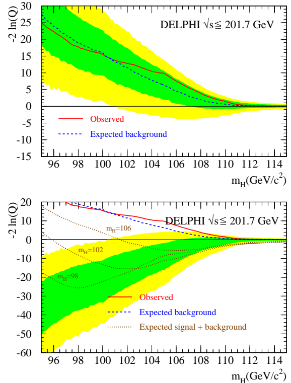
Fig. 13. SM Higgs boson: test-statistic Q for each m_H hypothesis in data (solid) and its expected median value in background-only experiments (dashed). Top: the bands correspond to the 68.3% and 95.0% confidence intervals from background-only experiments. Bottom: the bands represent the confidence intervals around the minima of the -2\ln Q curves expected for a signal of mass given in the abscissa while the dotted lines show the median curves expected for three mass hypotheses
