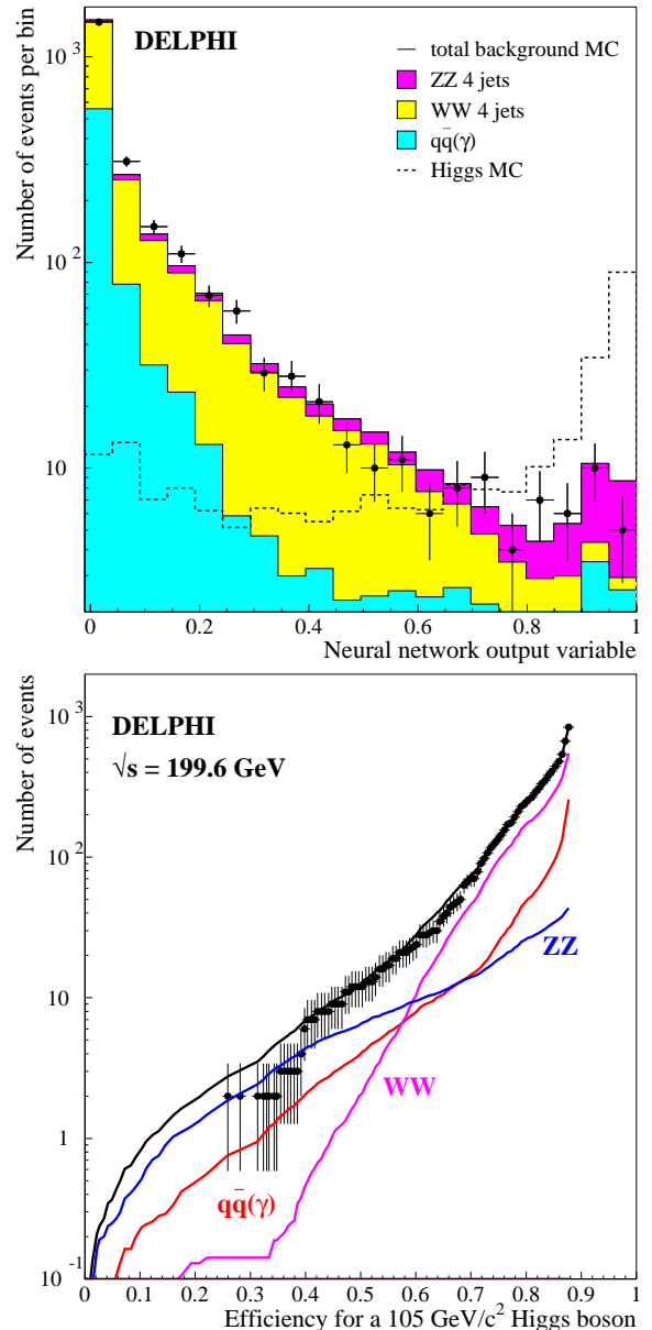
Fig. 8. H q\bar{q} channel: Top: distributions of the neural network variable for the expected SM backgrounds (full histograms), 191.6-201.7 GeV data (dots) and the expected Higgs signal at 105 GeV/ c^2 (dashed histogram, normalised to 20 times the expected rate). Bottom: curve of the expected SM background rate at \sqrt{s} = 199.6 GeV as a function of the efficiency for a 105 GeV/ c^2 Higgs signal when varying the cut on the neural network variable. The different background contributions are shown separately. The dots represent the data
