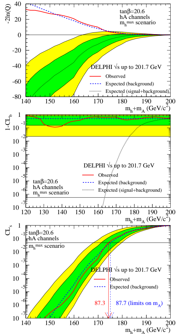
Fig. 15. hA analyses: test-statistic (top) and confidence levels in background hypothesis (middle) and in signal hypothesis (bottom) as functions of m_h+m_A . Curves are the observed (solid) and median expected (dashed) confidences from background-only experiments while the bands correspond to the 68.3% and 95.0% confidence intervals from background+signal experiments for a signal of mass given in the abscissa (top) and from background-only experiments (middle and bottom)
