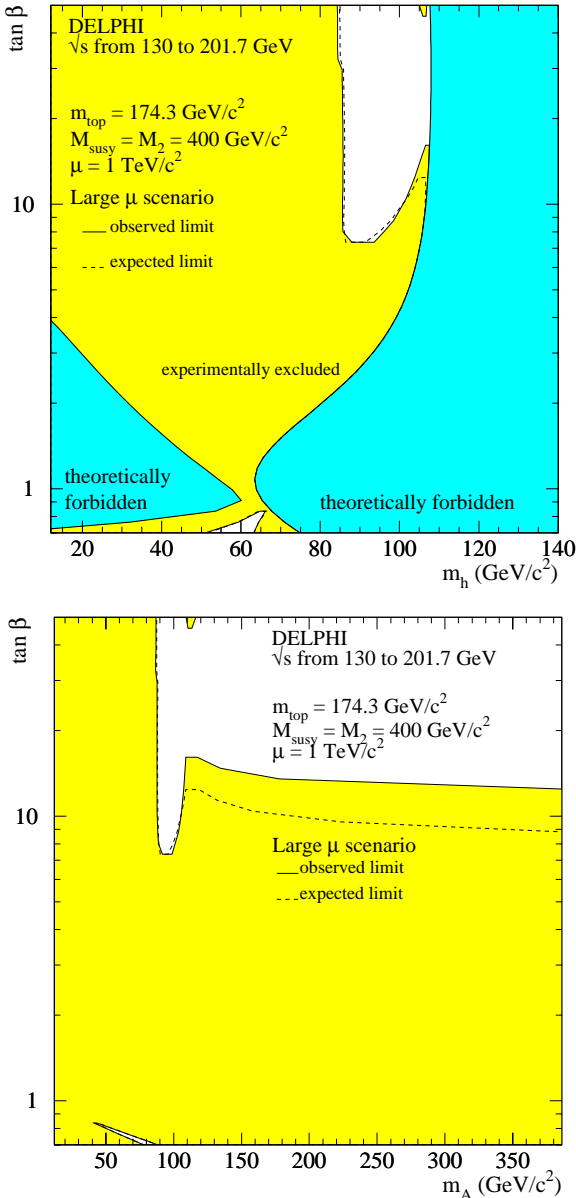
Fig. 18. MSSM Higgs bosons: regions excluded at 95% CL, by the searches in the hZ and hA channels up to \sqrt{s} = 201.7 GeV, in the large \mu scenario. The dark shaded areas are the regions not allowed by the MSSM model in this scenario. The dashed lines show the median expected limits
