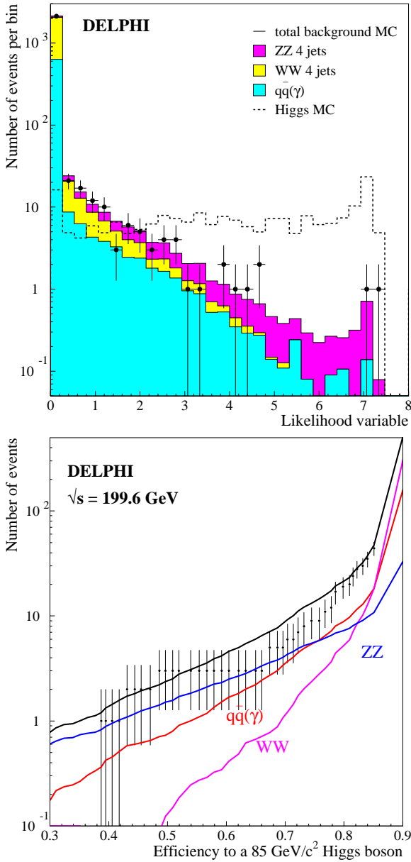
Fig. 10. hA hadronic channel: Top: distributions of the likelihood variable for the expected SM backgrounds (full histograms), 191.6-201.7 GeV data (dots) and the expected 85 GeV/c 2 Higgs signal at \tan\beta = 20 (dashed histogram, normalised to 20 times the expected rate). Bottom: curve of the expected SM background rate at \sqrt{s} = 199.6 GeV as a function of the efficiency for a 85 GeV/c 2 Higgs signal at \tan\beta = 20 when varying the cut on the likelihood variable. The different background contributions are shown separately. The dots show the data
