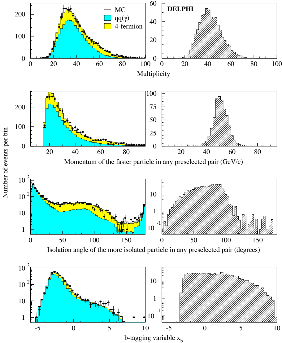
Fig. 3. H\mu^+\mu^- channel: distributions of four analysis variables, as described in the text, at preselection level. Data at \sqrt{s} = 191.6 - 201.7 GeV (dots) are compared with SM background expectations (left-hand side histograms) and with the expected distribution for a 105 \text{ GeV}/c^2 signal (right-hand side histogram, normalised to one thousand times the expected rate)
