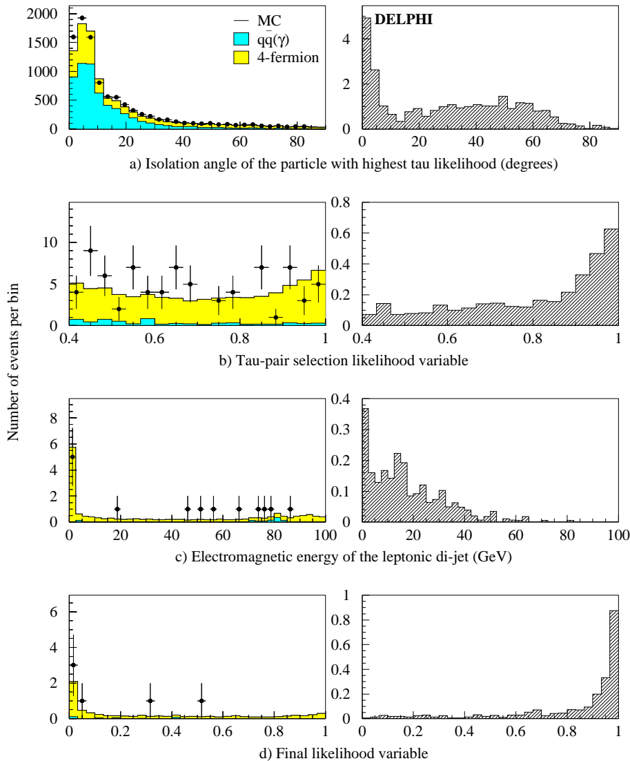
Fig. 4a–d. \tau^+\tau^-q\bar{q} channel: distributions of four analysis variables at different levels of the selection, as described in the text. Data at \sqrt{s} = 191.6 – 201.7 GeV (dots) are compared with SM background expectations (left-hand side histograms) and with the expected distribution for a 105 \text{ GeV}/c^2 signal in the (h \rightarrow \tau^+\tau^-)(Z \rightarrow q\bar{q}) (right-hand side histogram, normalised to one hundred times the expected rate)
