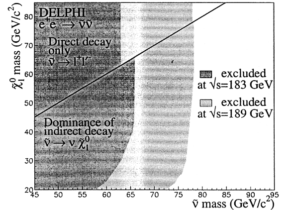
Fig. 5. Excluded region at 95% C.L. in m_{\tilde{\chi}_1^0}, m_{\tilde{\nu}} parameter space by \tilde{\nu} pair production for direct and indirect decays. The dark grey area shows the part excluded by the searches at 183 GeV, the light grey area the one excluded by the present analysis.
