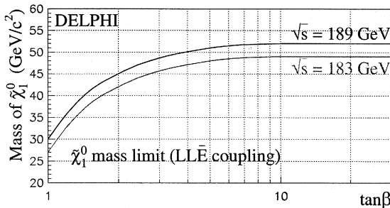
Fig. 3. The excluded lightest neutralino mass as a function of \tan\beta at 95% confidence level. This limit is valid for all generation indices i, j, k of the \lambda_{ijk} coupling and all values of m_0 .
