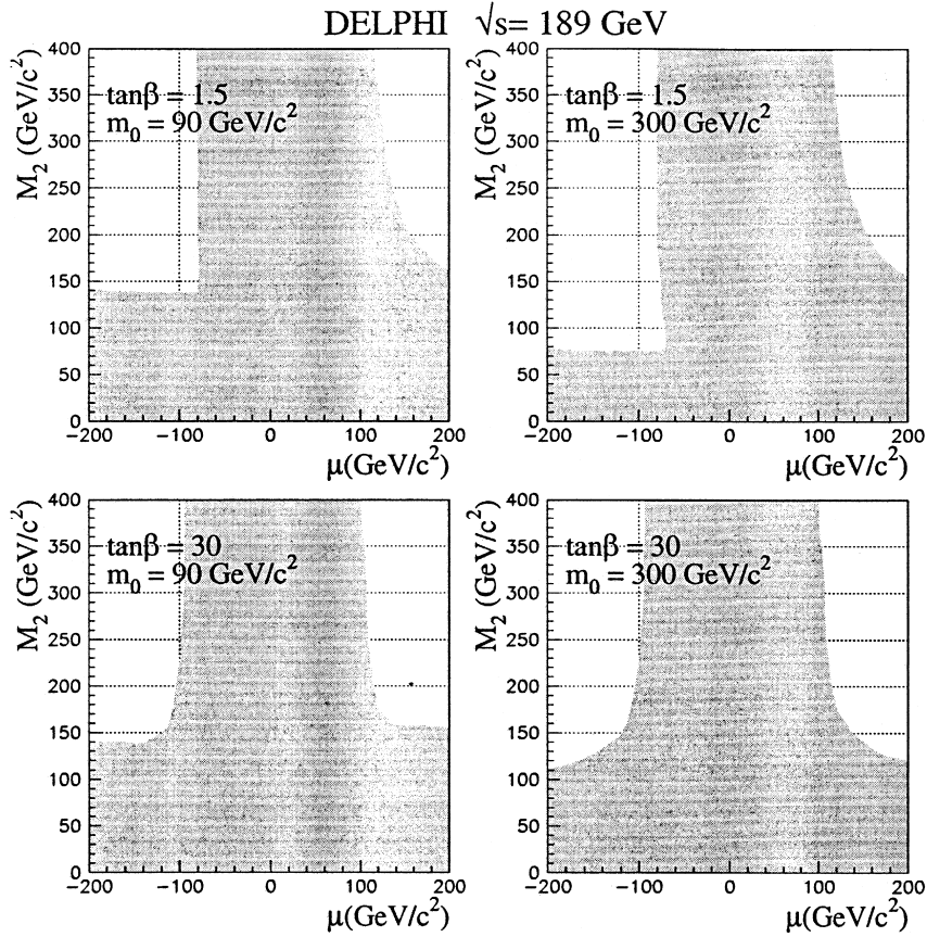
Fig. 2. Decays through the \lambda R -parity violating operator: excluded regions at 95% C.L. in the \mu, M_2 parameter space by the neutralino and chargino searches in DELPHI at 189 GeV for two values of \tan\beta and two values of m_0 .
