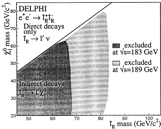
Fig. 6. Charged slepton indirect decay: excluded region at 95% C.L. in m_{\tilde{\chi}_1^0} , m_{\tilde{\tau}_R} parameter space by \tilde{\ell}_R pair production. The dark grey area shows the part excluded by the searches at 183 GeV, the light grey area the one excluded by the present searches at 189 GeV.
