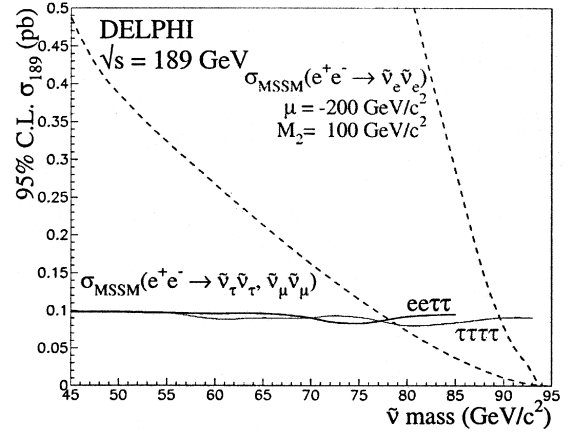
Fig. 4. Sneutrino direct decay with \lambda_{133} coupling: limit on the \tilde{\nu}\tilde{\nu} production cross-section as a function of the mass for two different final states. The MSSM cross-sections are reported in order to derive a limit on the sneutrino mass in the case of direct \tilde{R}_p decay. The dashed lower curve corresponds to both \tilde{\nu}_\mu\tilde{\nu}_\mu and \tilde{\nu}_\tau\tilde{\nu}_\tau cross-sections which depend only on the \tilde{\nu} mass. The dashed upper curve is the \tilde{\nu}_e\tilde{\nu}_e cross-section obtained for \mu = -200 \text{ GeV}/c^2 and M_2 = 100 \text{ GeV}/c^2 , the corresponding chargino mass lies between 90 and 120 \text{ GeV}/c^2 .
