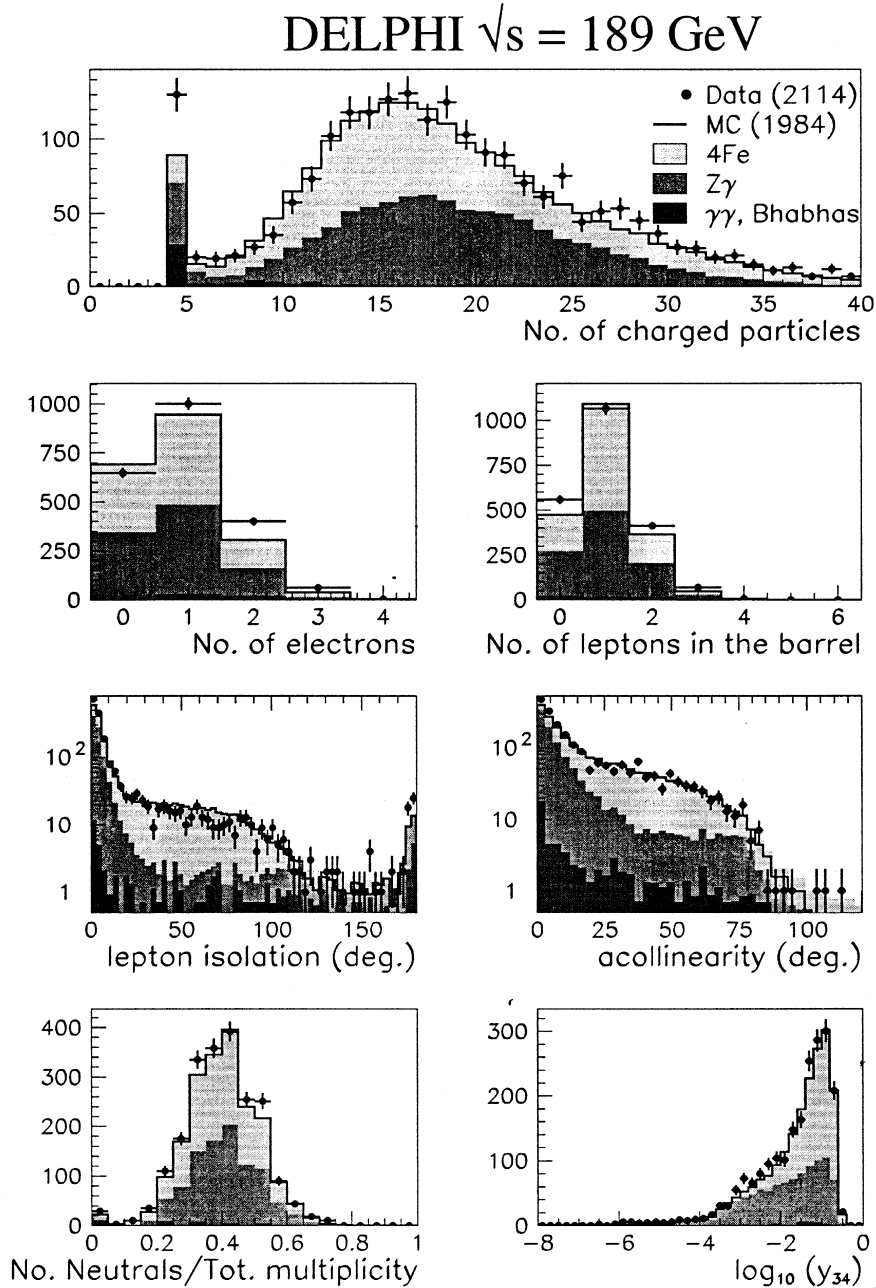
Fig. 1. Distributions, after the preselection applied for the \lambda_{133} analyses, of the number of charged particles, the number of well identified electrons in the event, the number of identified leptons with a polar angle between 40^\circ and 140^\circ , the lepton isolation angle, the acollinearity, the ratio of the number of neutral particles to the total event multiplicity, and the \log_{10}(y_{34}) . The black dots show the real data distributions, and the shaded histograms the expected background from Standard Model processes.
