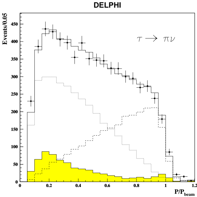
Fig. 8. The spectrum, for \tau \rightarrow \pi(K)\nu decays as a function of the \pi(K) momentum normalised to the beam momentum. The circles are data and the solid line is simulation for the fitted value of \langle \mathcal{P}_\tau \rangle . The hatched area is background and the dashed and dotted lines correspond to the positive and the negative polarisation contributions respectively
