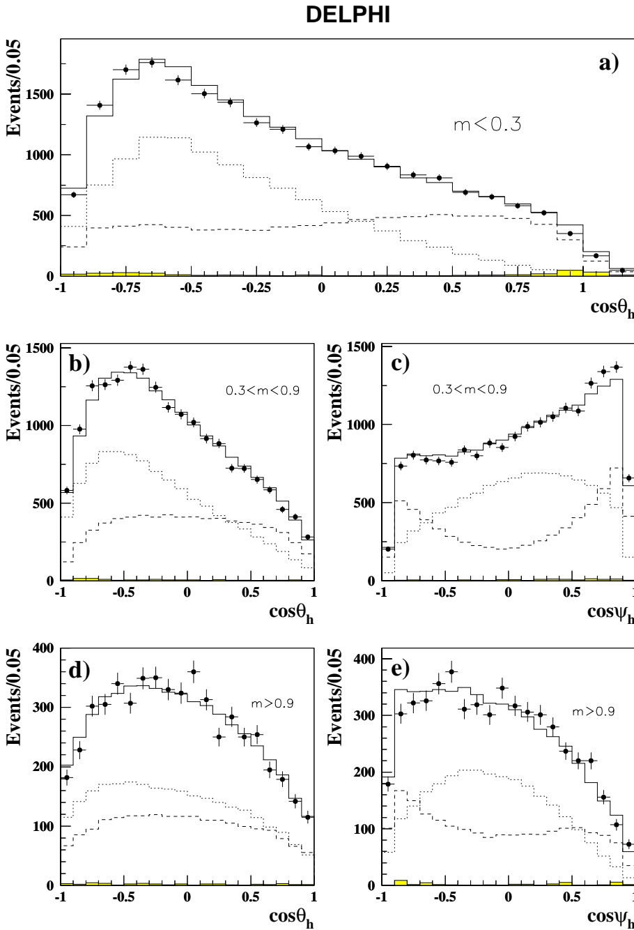
Fig. 14a–e. For the one-prong hadron inclusive analysis, the projections of the \cos\theta_h vs \cos\psi_h 2-dimensional distributions for the three invariant mass regions (only \cos\theta_h for the first mass range, where \cos\psi_h has no significance): a m_h < 0.3 \text{GeV}/c^2 ; b and c 0.3 \text{GeV}/c^2 < m_h < 0.9 \text{GeV}/c^2 ; d and e 0.9 \text{GeV}/c^2 < m_h < 1.8 \text{GeV}/c^2 ; The circles are data and the solid line is simulation for the fitted value of \langle \mathcal{P}_\tau \rangle . The hatched area is background and the dashed and dotted lines correspond to the positive and the negative polarisation contributions respectively
