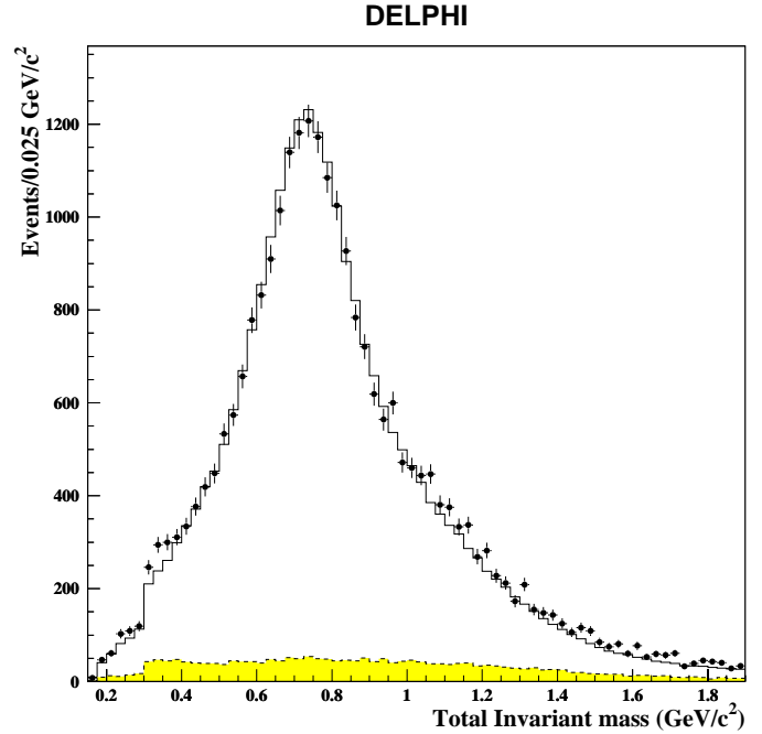
Fig. 13. The observed invariant mass distribution for candidate events in the barrel in the one-prong hadron inclusive analysis. The circles are data, the solid line is simulation, and the hatched area represents the external background and all \tau decays excepting the \tau \rightarrow \pi(K)\nu , \tau \rightarrow \rho\nu and \tau \rightarrow a_1\nu
