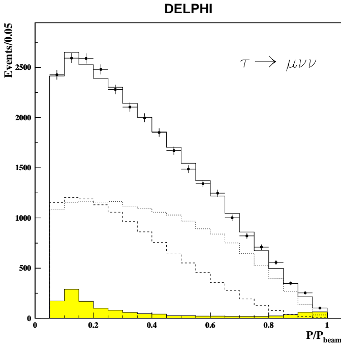
Fig. 7. P/p_{beam} spectrum for candidate \tau \rightarrow \mu\nu\bar{\nu} decays. The circles are data and the solid line is simulation for the fitted value of \langle \mathcal{P}_\tau \rangle . The hatched area is background and the dashed and dotted lines correspond to the positive and the negative polarisation contributions respectively
