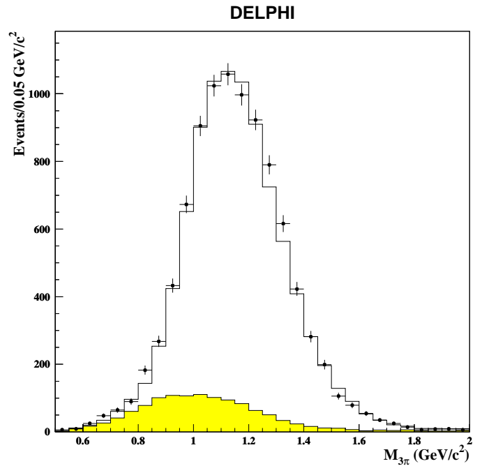
Fig. 11. The 3\pi invariant mass spectrum from \tau \rightarrow 3\pi^\pm\nu_\tau decays. The circles are data, the histogram corresponds to simulation and the hatched area is background
