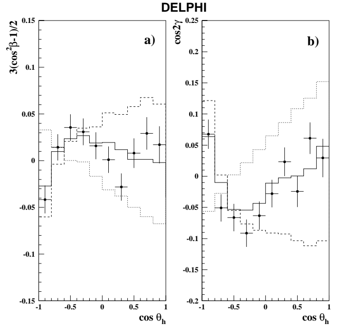
Fig. 12a,b. The two most sensitive moments in the polarisation fit of the \tau \rightarrow a_1\nu channel as a function of \cos\theta_h : a \langle (3\cos^2\beta - 1)/2 \rangle and b \langle \cos 2\gamma \rangle . The circles show the data and the solid line is simulation for the fitted value of \langle \mathcal{P}_\tau \rangle . The dashed and dotted lines correspond to the positive and the negative polarisation distributions respectively
