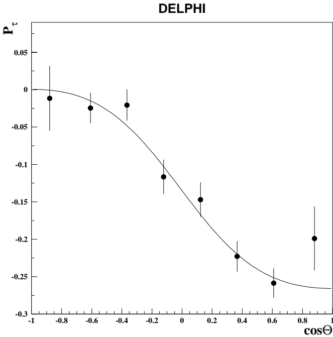
Fig. 15. Data points show measured \mathcal{P}_\tau as a function of \cos\Theta . The full curve represents theoretical expectation for the fit result
