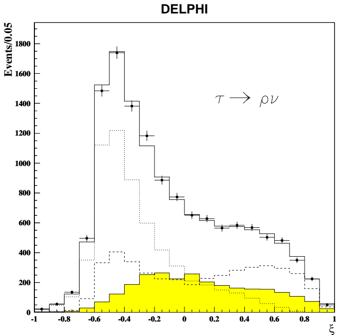
Fig. 10. The observed \xi spectrum of candidate \tau \rightarrow \rho\nu decays. The circles are data and the solid line is simulation for the fitted value of \langle P_\tau \rangle . The hatched area is background and the dashed and dotted lines correspond to the positive and the negative polarisation contributions respectively
