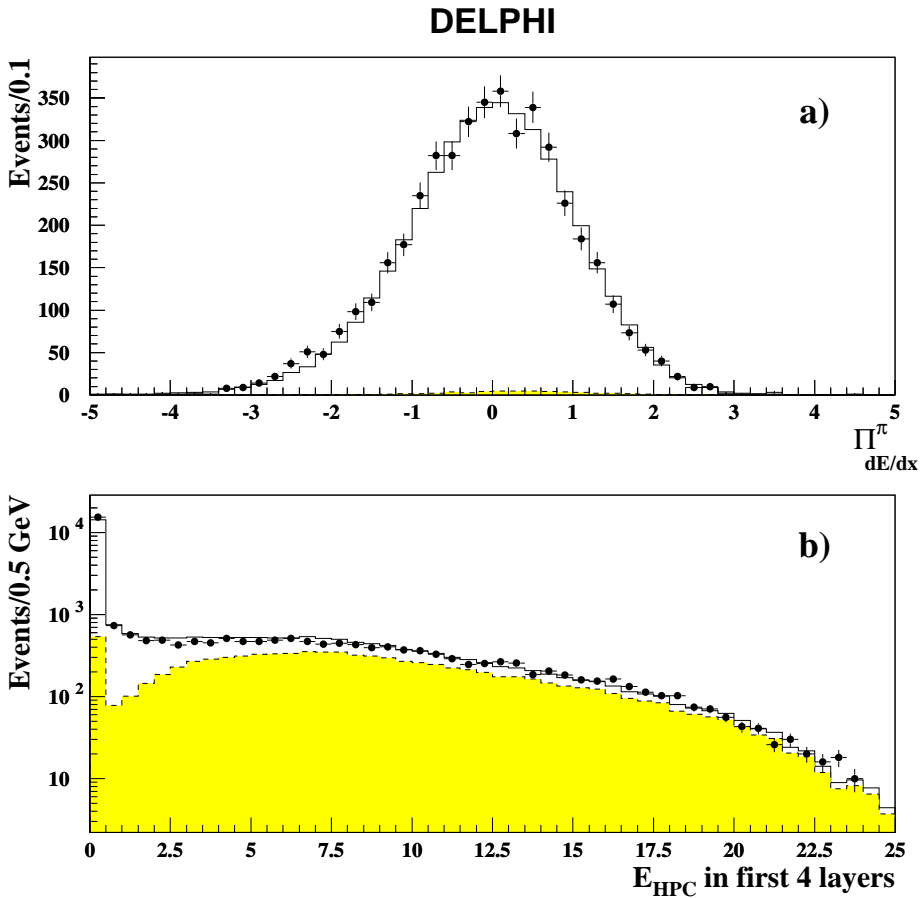
Fig. 2a,b. Distribution of hadron identification variables for charged hadrons from \tau decays: a pull dE/dx for \pi hypothesis and b energy deposited in the first four layers of the HPC. Circles are data, the solid line is simulation and the hatched area represents the background (anything except \tau decays to hadrons)
