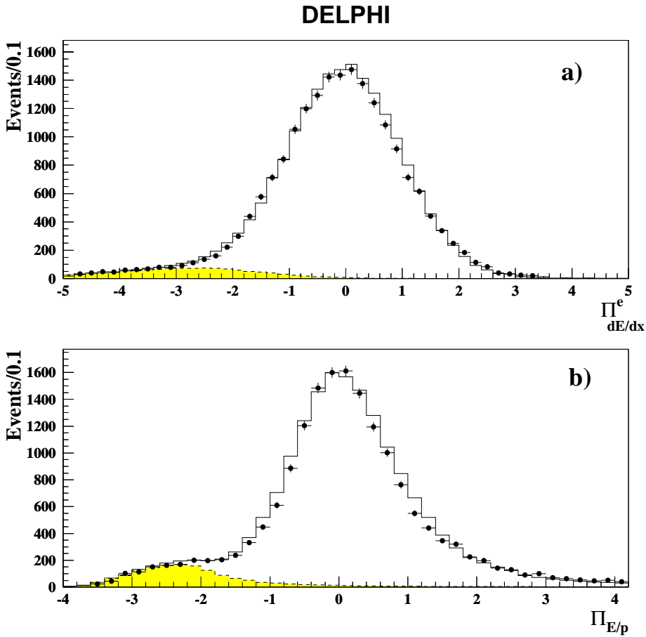
Fig. 1a,b Distribution of electron identification variables for electron test samples: a pull dE/dx and b pull E/p for electron hypothesis. The solid line is for all simulation, the hatched area represents the background (anything except \tau decays to electrons) and the circles are the data
