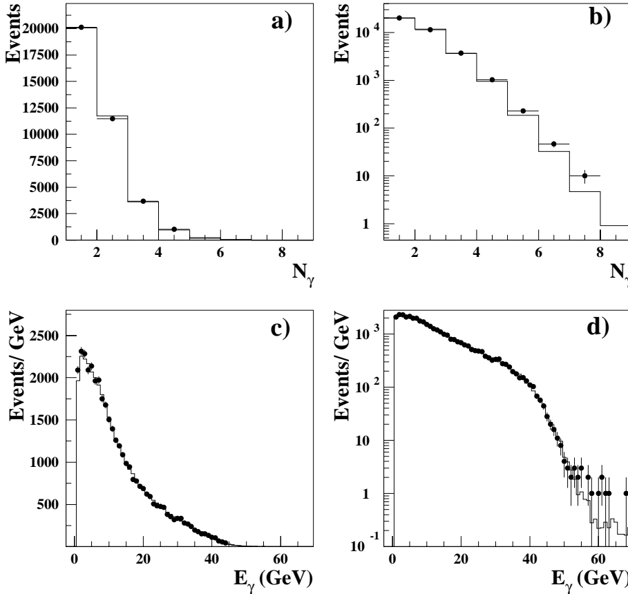
Fig. 3. a,b Neutral multiplicity and c,d energy spectra for all identified \gamma for an inclusive \tau sample. Left hand side plots are in linear scale and right hand side in logarithmic scale. Circles are data and the solid line is simulation
