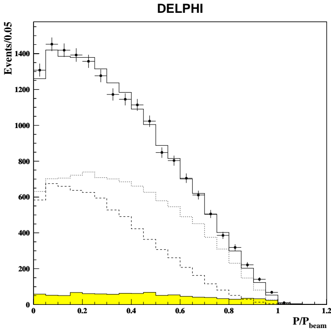
Fig. 6. p_{el}/p_{beam} spectrum for candidate \tau \rightarrow e\nu\bar{\nu} decays. The circles are data and the solid line is simulation for the fitted value of \langle \mathcal{P}_\tau \rangle . The hatched area is background and the dashed and dotted lines correspond to the positive and the negative polarisation contributions respectively
