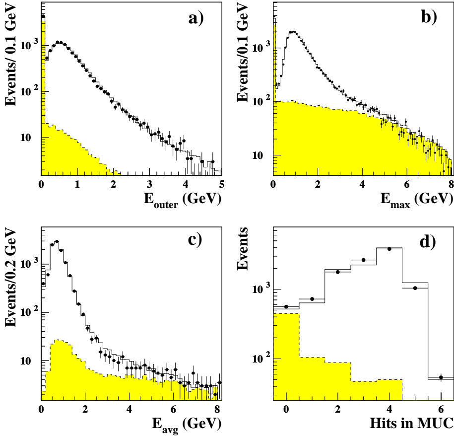
Fig. 5a–d. Distribution of muon identification variables for muon test samples. a Energy in the outermost HCAL layer, b largest HCAL energy deposition, c average HCAL energy and d muon chamber hits. Circles are data, the solid line is simulation and the hatched area represents the background (anything except \tau decays to muons)
