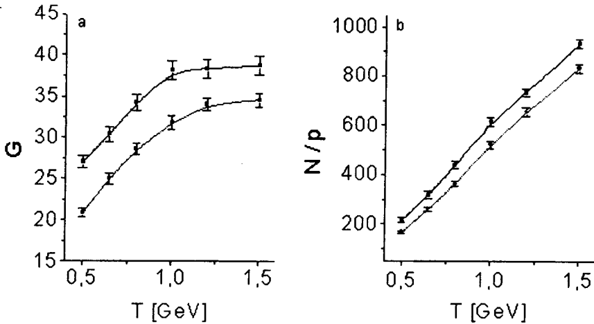
Fig.2. Energetic gain G and the number of neutrons per proton produced in the system N/p vs. incident proton energy T for k_{eff}=0.945 / 0.003/ (The upper curve-for the lead target, the lower- for tungsten one)
