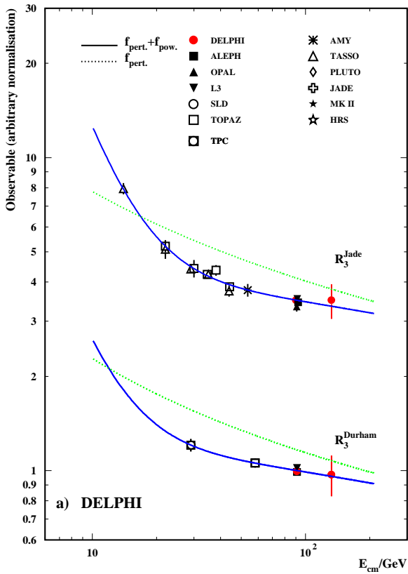
Fig. 8a–c. Energy dependence of event shape observables using the cuts defined in Table 2. The curves are results of the fits to equations (1–3). The corresponding parameters are given in Table 3. In b the fits with C_2 = 0 are displayed. The dotted lines correspond to the pure second order perturbative prediction, \langle f_{pert} \rangle , the full curves represent the sum of the perturbative and power terms, \langle f_{pert} \rangle + \langle f_{pow} \rangle
