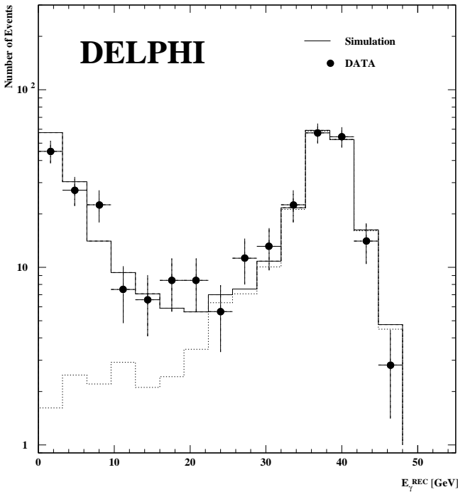
Fig. 1. Reconstructed energy spectrum of photons from initial state radiation (ISR). The peak at E_{\gamma}^{rec} near 40 GeV due to radiative return to the Z is clearly seen. Events with E_{\gamma}^{rec} above 20 GeV are rejected in this analysis. The dotted histogram shows the E_{\gamma}^{rec} distribution for fully simulated events generated with E_{\gamma} \geq 20 GeV
