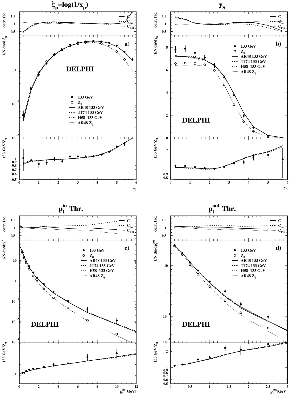
Fig. 2a–d. The four central plots show inclusive charged particle distributions at 133 GeV (full circles) and at the Z (open circles) as a function of (a) \xi_p , (b) y_S , (c) p_t^{in} , and (d) p_t^{out} . The curves show the predictions from ARIADNE 4.8 (full curve for 133 GeV, dotted for the Z ) and, for 133 GeV only, from JETSET 7.4 (dashed) and HERWIG 5.8 (dot-dashed). The upper insets display the correction factors explained in the text: the dashed line shows the detector correction, the dotted line the ISR correction, and the full line the total correction. The lower insets show the ratio of the 133 GeV data to the Z data and the corresponding model predictions
