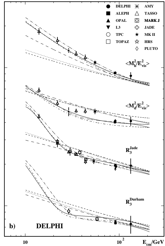
Fig. 6a,b. Energy dependence of event shape variables using the cuts (where relevant) defined in Table 2 compared with predictions of the ARIADNE, HERWIG, and JETSET fragmentation models. The curves correspond to the hadronic (full and dot-dashed curves close to data) and partonic (dashed curves showing weaker energy dependence) final states
