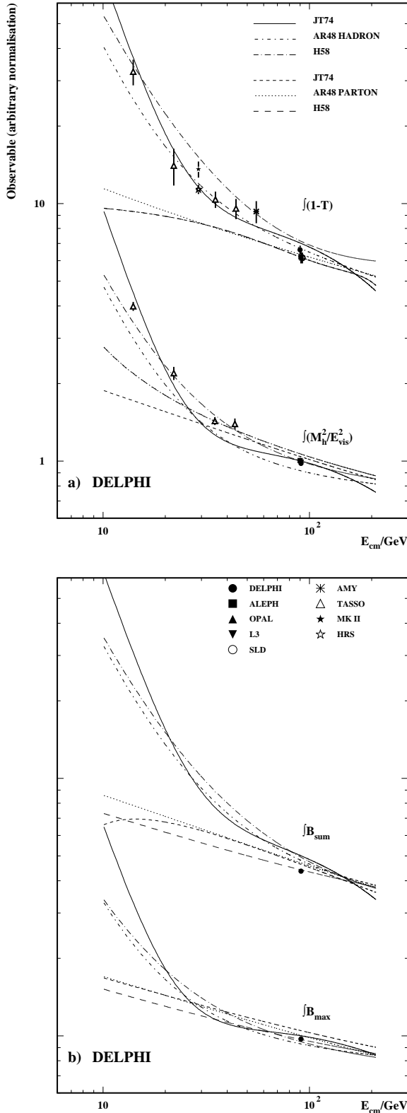
Fig. 7a,b. Energy dependence of event shape variables using the cuts (where relevant) defined in Table 2 compared with predictions of the ARIADNE, HERWIG, and JETSET fragmentation models. The curves correspond to the hadronic (full and dot-dashed curves close to data) and partonic (dashed curves showing weaker energy dependence) final states
