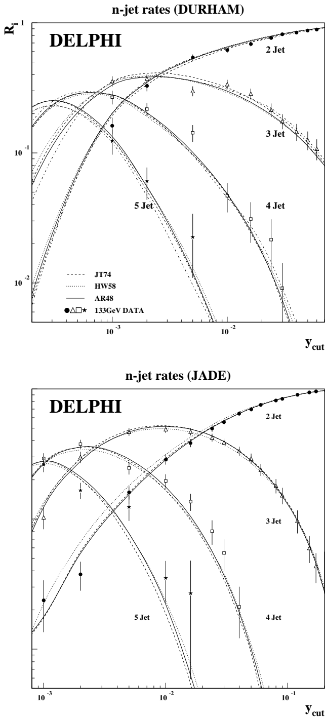
Fig. 5. Measured 2-jet, 3-jet, 4-jet and 5-jet rates at 133 GeV as a function of y_{cut} for the Durham and JADE jet algorithms compared with the predictions of ARIADNE 4.8 (full curve), JETSET 7.4 (dashed), and HERWIG 5.8 (dotted)
