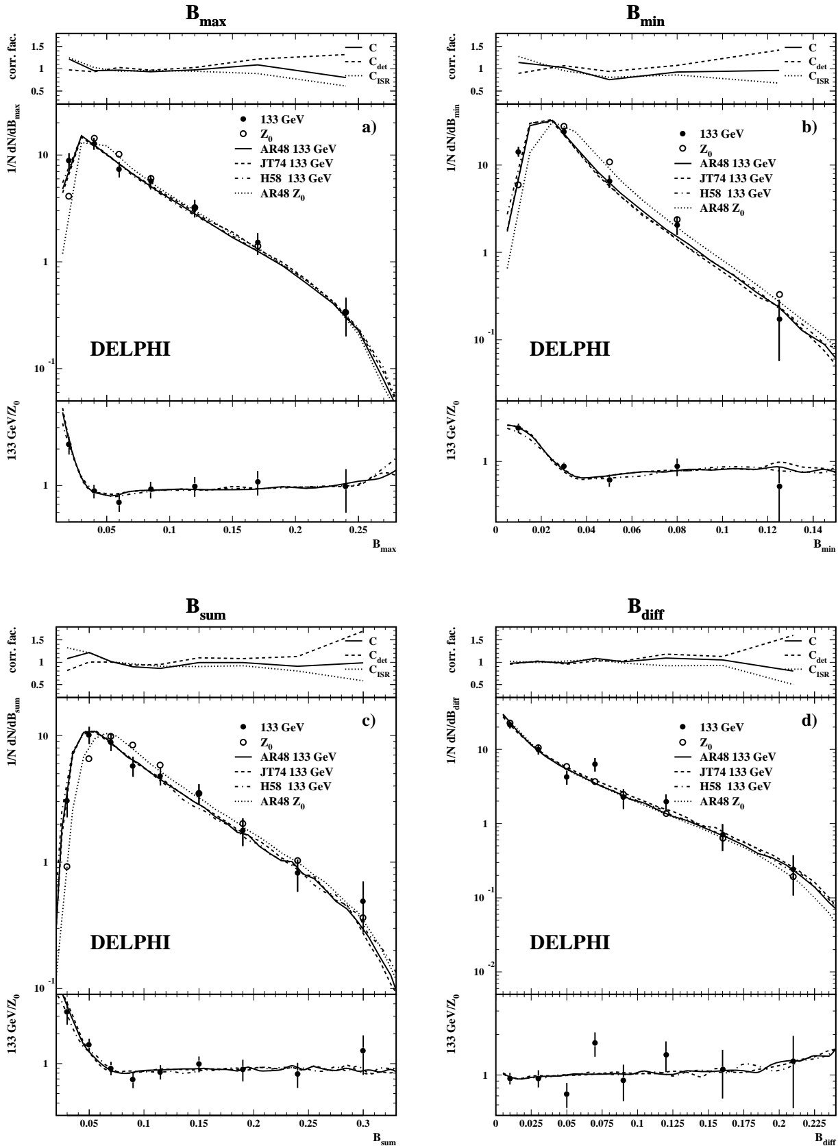
Fig. 4a–d. Distribution of a Wide Hemisphere Broadening, b Narrow Hemisphere Broadening, c Total Hemisphere Broadening and d Difference of the Hemisphere Broadenings. The insets, symbols and curves are as in Fig. 2
