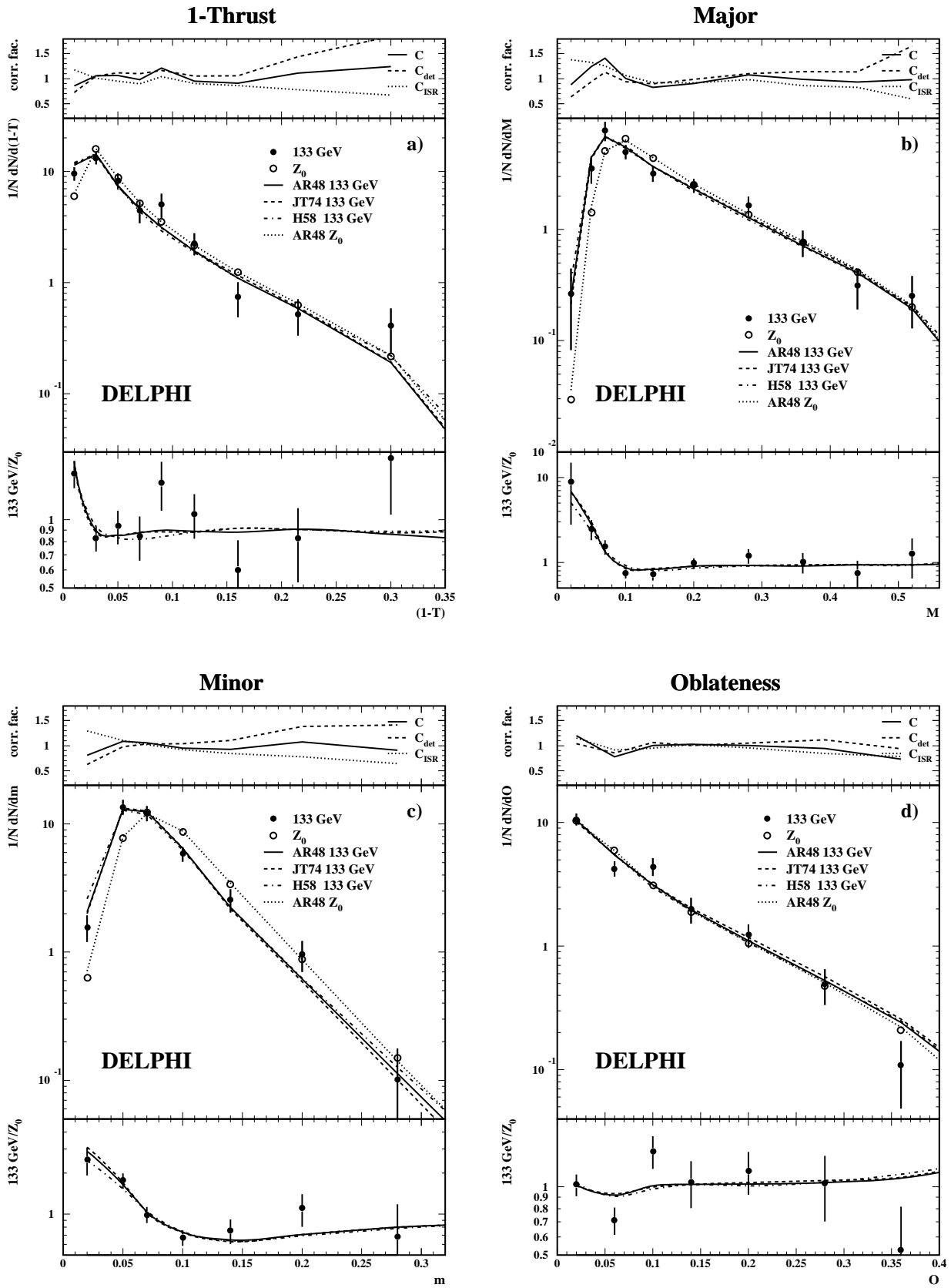
Fig. 3. a 1-Thrust, b Major, c Minor and d Oblateness distributions. The insets, symbols and curves are as in Fig. 2
