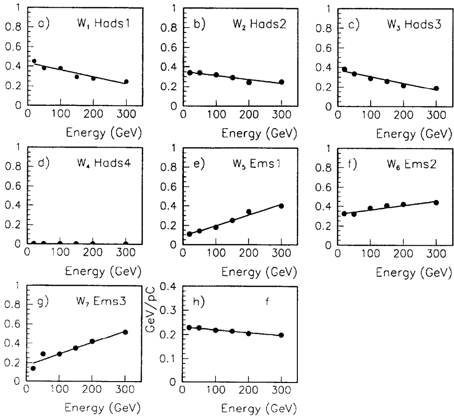
Fig. 7. Parametrization of the weight for each longitudinal sampling and of the intercalibration parameter as a function of the beam energy.
