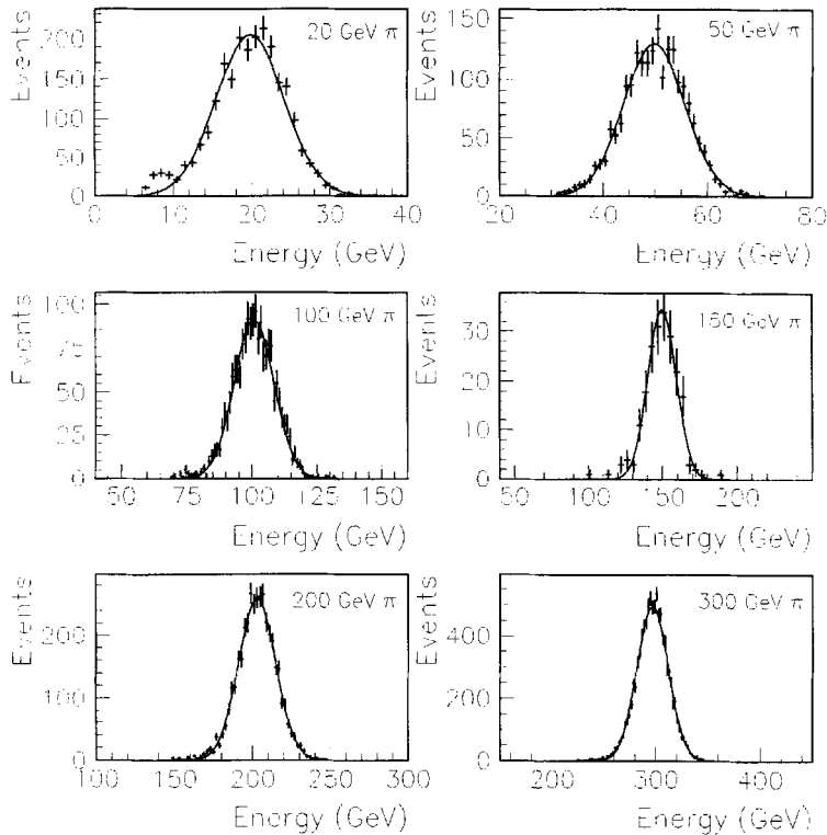
Fig. 4. Pion energy spectra at different incident energies, obtained with the benchmark algorithm. The mean and \sigma values are listed in Table 1.
