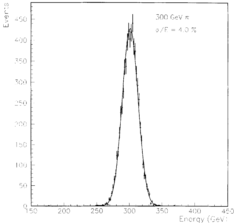
Fig. 8. Energy spectrum of 300 GeV pions, where the energy is reconstructed with the weighting method.
