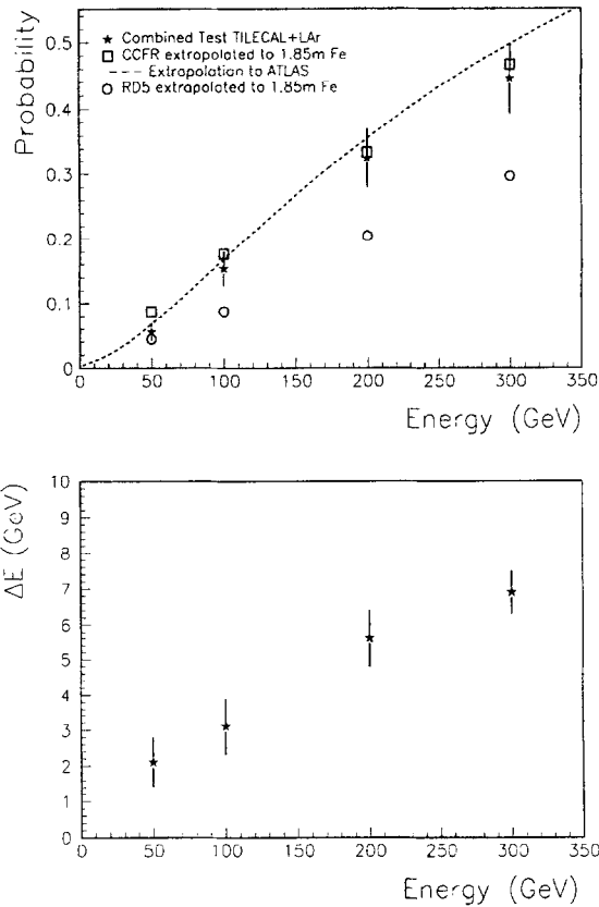
Fig. 14. (a) Punchthrough probability for pions. Results from the RD5 and CCFR Collaboration (recalculated for 1.85 m of iron) are also plotted. The dashed line shows the expectation for the ATLAS configuration. (b) Average energy loss vs. beam energy for events with longitudinal leakage.
