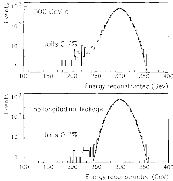
Fig. 5. Low energy tails in the 300 GeV pion spectrum before (upper plot) and after (lower plot) rejecting the events with a signal in the muon wall.
