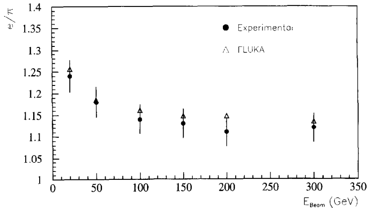
Fig. 6. Values of the e/\pi ratio vs. the beam energy. Standalone FLUKA results are also shown.
