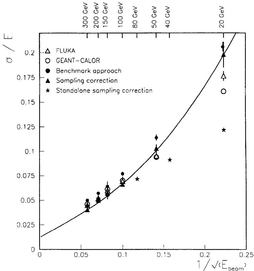
Fig. 9. Energy resolutions with the benchmark approach and with the weighting method (‘sampling corrections’). The data are compared with the combined Monte Carlo simulations and with the results from the stand-alone hadron calorimeter test beam (stars).
