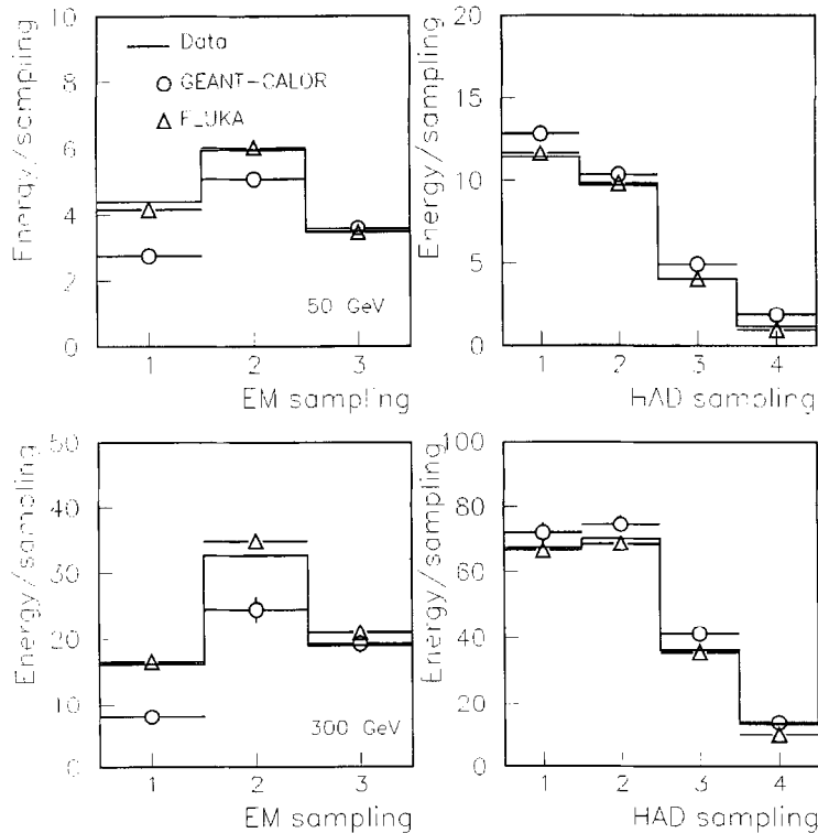
Fig. 11. Energy deposition in each sampling of the electromagnetic (on the left) and hadronic (on the right) calorimeters for pions of 50 (on top) and 300 GeV (on bottom). The data are compared with both Monte Carlo simulations.
