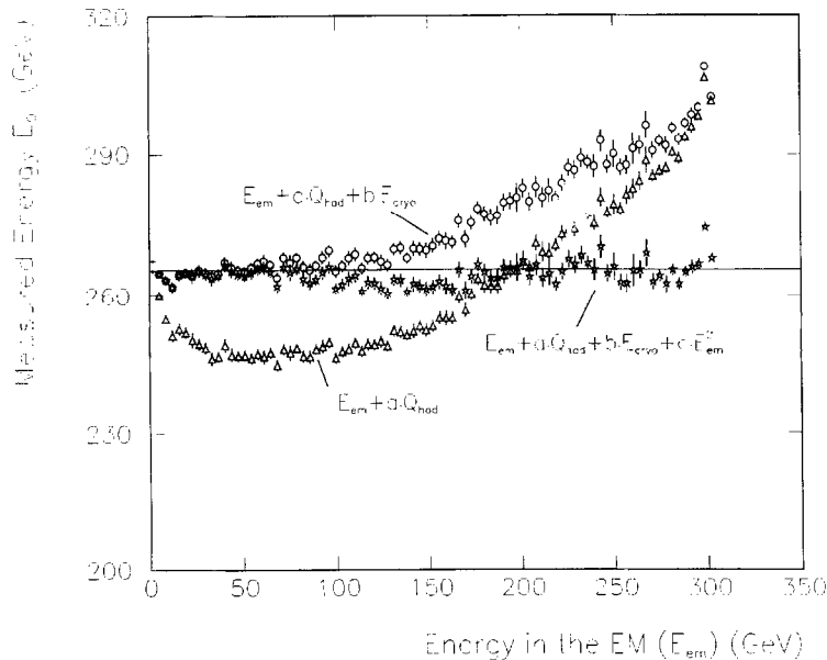
Fig. 2. Components of the first pass energy E_0 vs. energy in the EM calorimeter using the 'benchmark' energy reconstruction method for 300 GeV pions.
