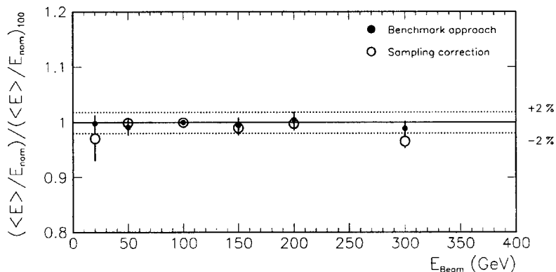
Fig. 10. Linearity of the pion response with the benchmark approach and with the weighting method (‘sampling corrections’). All the points are normalized to the point at 100 GeV.
