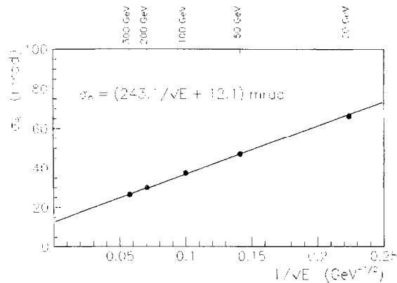
Fig. 13. Angular resolution for pions as a function of the beam energy.
