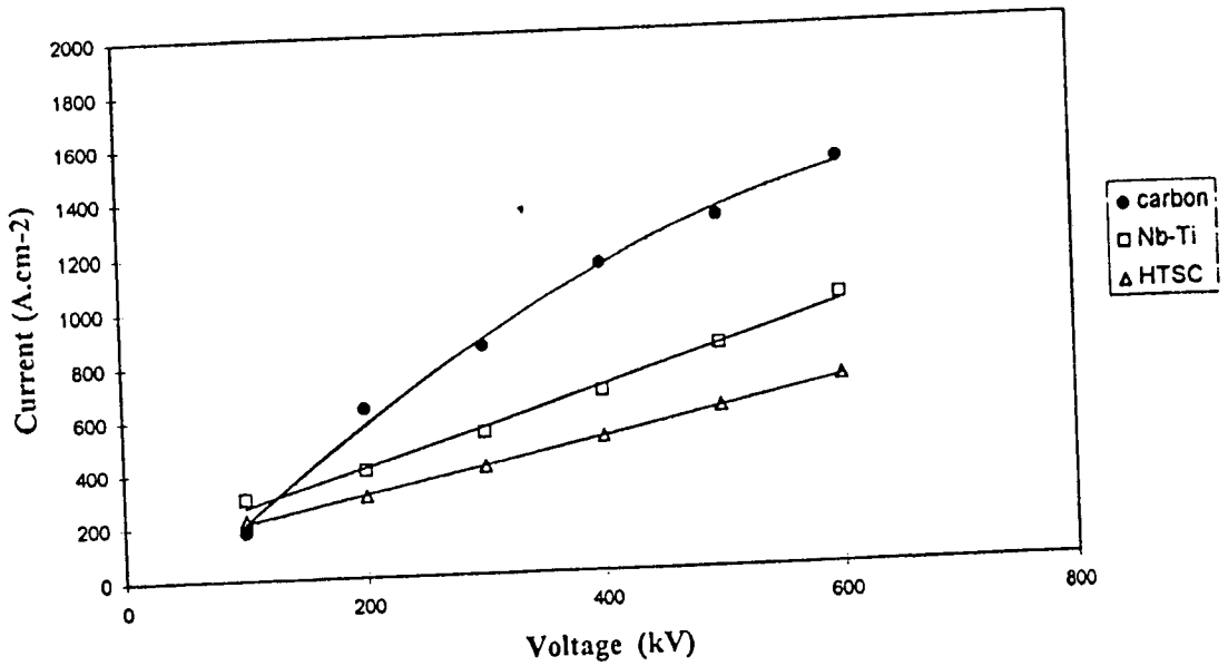
Fig.2. Emission characteristics of source in an electron regime.
