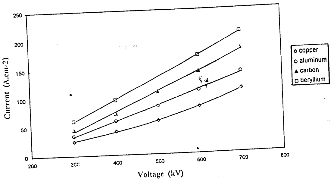
Fig.3. Emission characteristics of source in ion regime.
