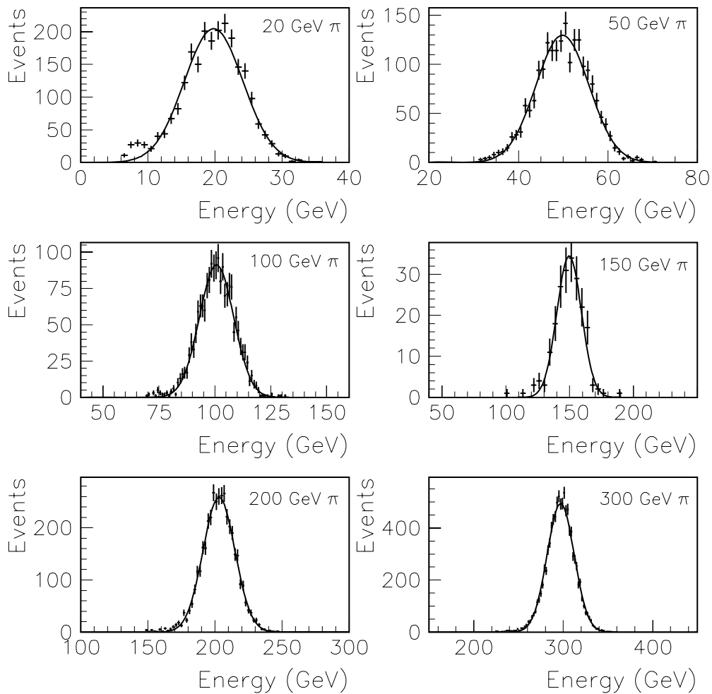
Figure 4: Pion energy spectra at different incident energies, obtained with the benchmark algorithm. The mean and \sigma values are listed in Table 1.
