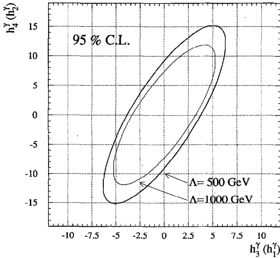
Fig. 3. Upper limits at the 95% C.L. on the Z\gamma\gamma coupling from the DELPHI single photon data for two different values of \Lambda .
