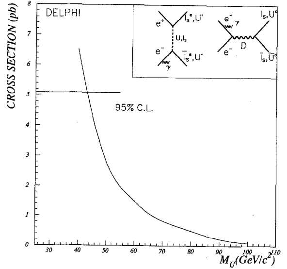
Fig. 4. Limit at 95% C.L. for the mass of the W-type U boson. The curve shows the predicted cross section as a function of M_U according to [10]. The insert shows two examples of the Feynman graphs contributing to the calculated cross-sections.
