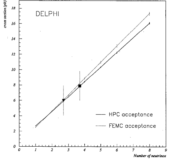
Fig. 2. Cross-sections for radiative neutrino production in the region of acceptance of the HPC (square for the data and solid line for theoretical prediction) and FEMC (triangle and dotted line respectively).
