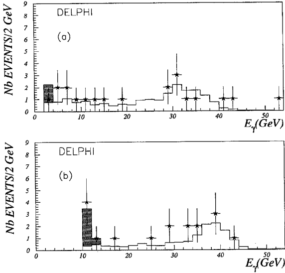
Fig. 1. Energy spectrum of selected single photons a) in the barrel region (HPC) and b) in the forward region (FEMC). The hatched histogram is the background from the QED process e^+e^- \rightarrow \gamma e^+e^- , and the unhatched histogram is the expected spectrum from e^+e^- \rightarrow \nu\bar{\nu}\gamma . The event in (a) with E_\gamma = 52 GeV is close to a crack of the detector and an \alpha is mixed in its deposited energy, which is therefore badly determined.
