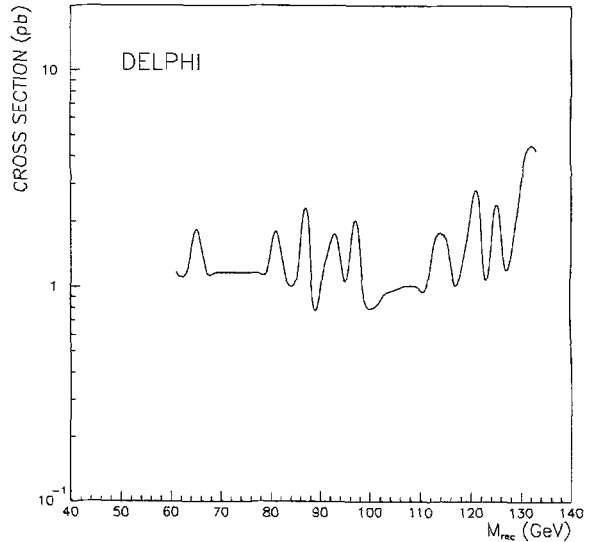
Fig. 5. Upper limit at 95% C.L. for the cross-section of \gamma X final state as a function of the mass of X.
