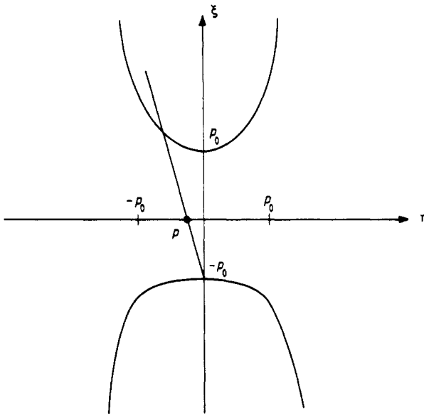
Figure 2. Mapping of the range of momentum p onto the upper branch of the hyperbola \xi - \eta^2 = p_0^2 .
