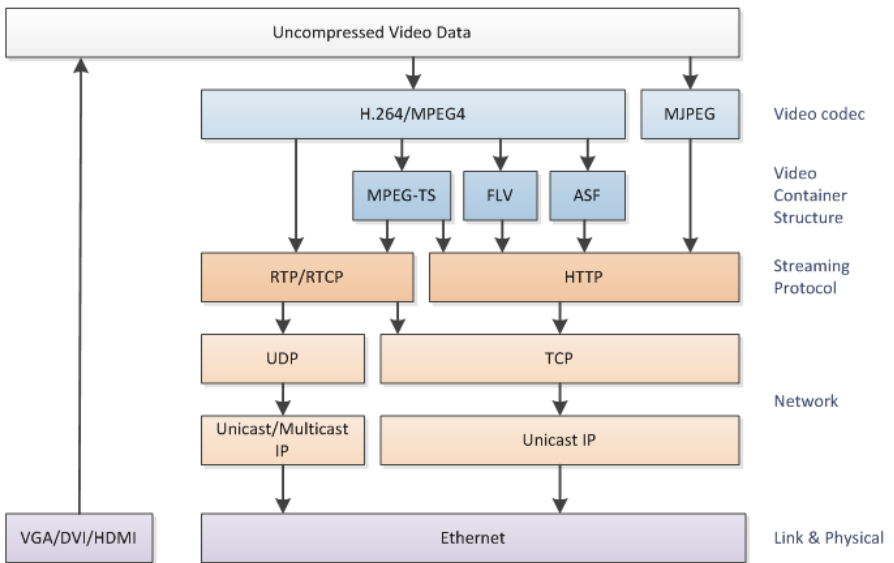
Figure 21 Protocol Stack Diagram
