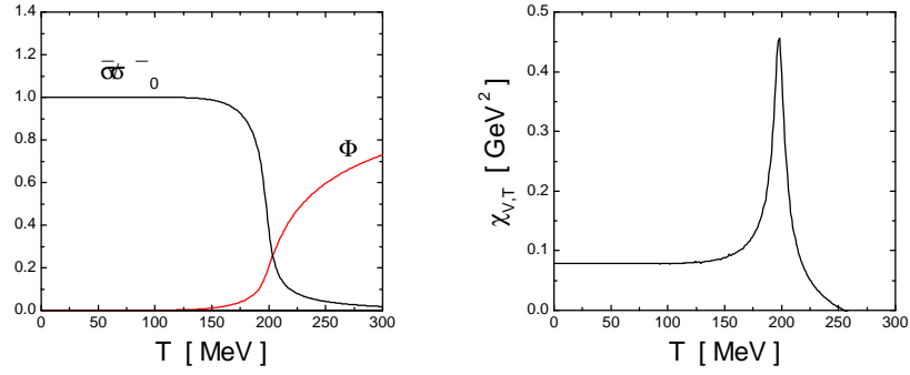
Figure 1. (a) normalized mean field value \bar{\sigma}_u / \bar{\sigma}_u(T=0) and Polyakov loop \Phi as functions of T . (b) chiral susceptibility \chi_{V,T} as function of T .
