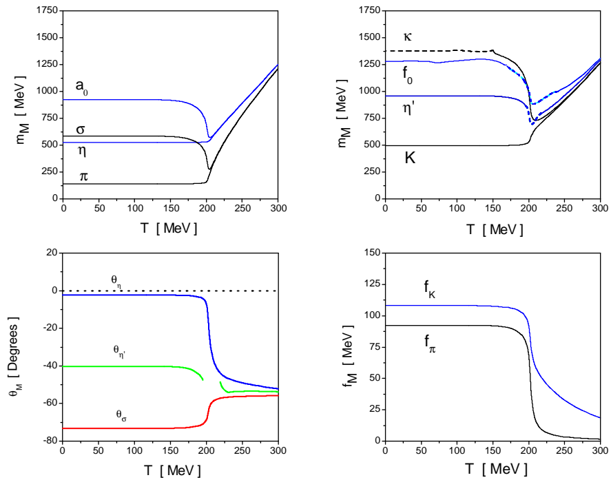
Figure 2. Meson properties as functions of the temperature. In upper panels we display the meson masses, while in the lower panels we quote the values of mixing angles (left) and decay constants (right).
