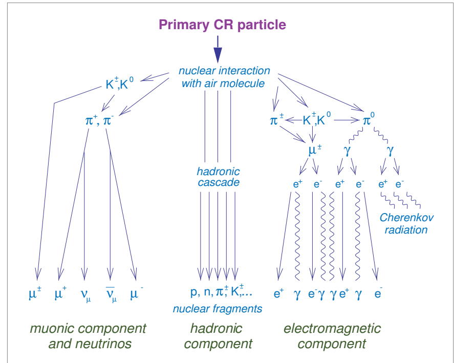
Figure 38: Schematic view of atmospheric cascade initiated by a primary CR particle.
