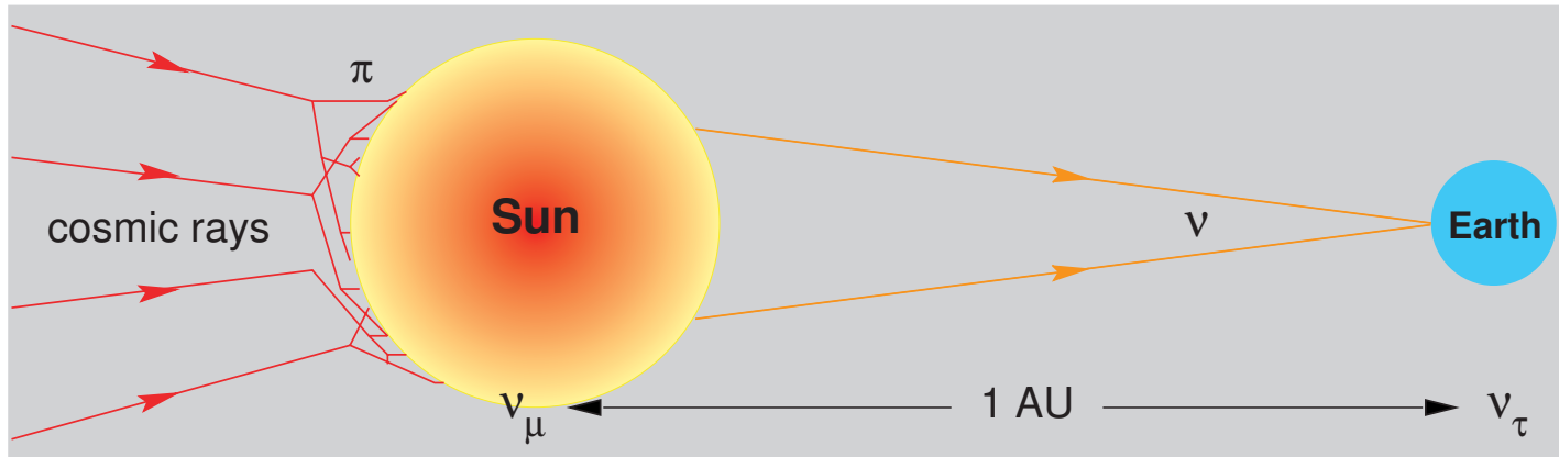
Figure 201: Cosmic rays hitting the Sun produce \nu_{\mu} 's which propagate further to Earth. At an energy of 10 TeV the length for \nu_{\mu} \leftrightarrow \nu_{\tau} oscillations is (according to the SK AN result) about 1 AU. [From J. G. Learned and K. Mannheim, Ann. Rev. Nucl. Part. Sci. 50 (2000) 679, Fig. 7.]
