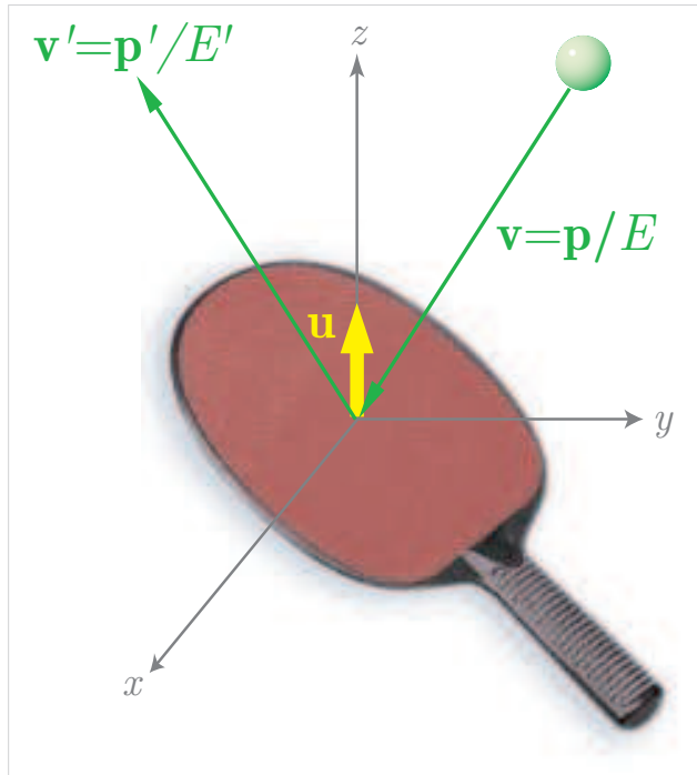
Figure 212: Relativistic pingpong.
