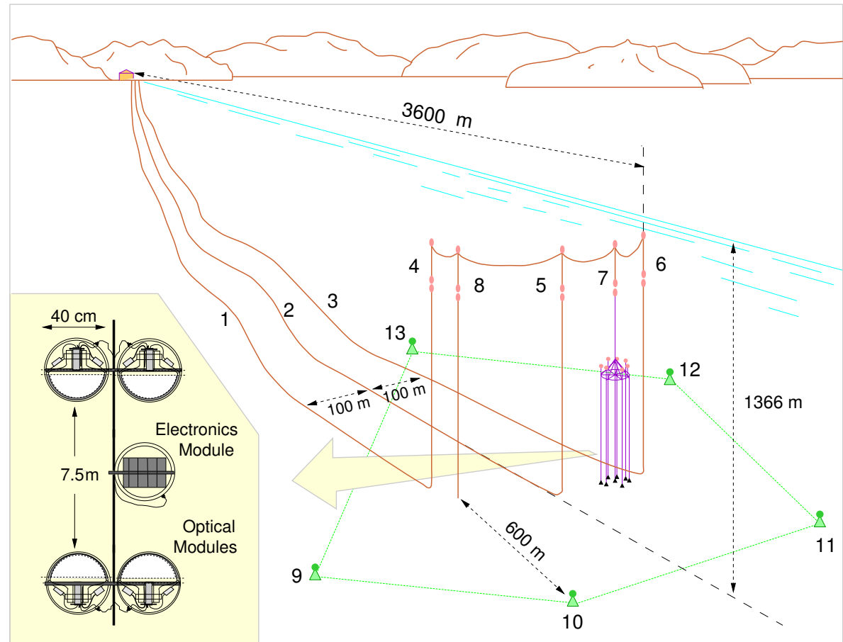
Figure 154: Overall view of the NT-200 complex in Lake Baikal. [From V. A. Balkanov et al., "In-situ measurements of optical parameters in Lake Baikal with the help of a neutrino telescope," Appl. Opt. 33 (1999) 6818–6825 (astro-ph/9903342).]
