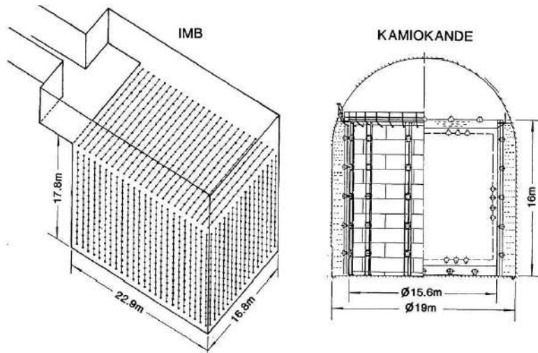
Figure 42: Water Cherenkov detectors.
