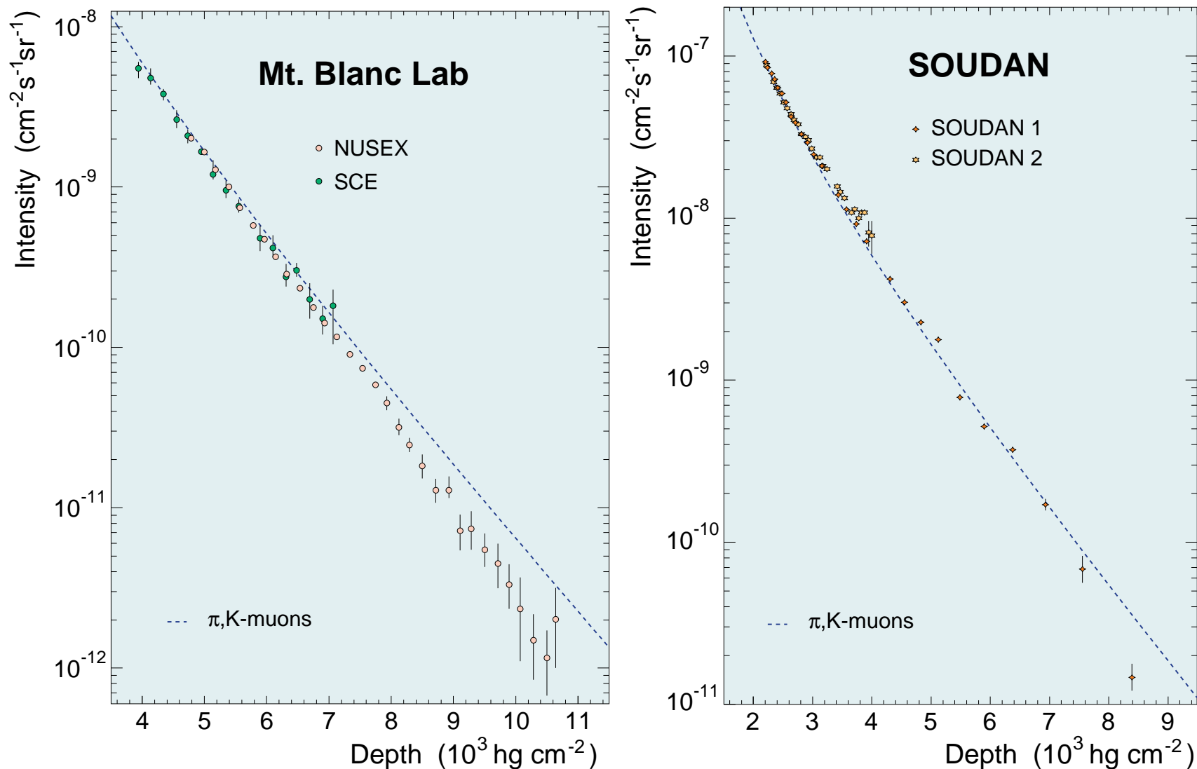
Figure 82: Muon DIR from the SCE, NUSEX, SOUDAN 1 and SOUDAN 2 experiments.
