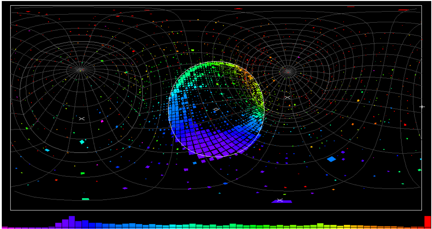
Figure 105: The same event as in the right panel of Fig. 104 but in cylindrical projection. This is a 4\pi view. Un-hit PMTs are hidden but detector grid is shown. The observer is positioned in the event vertex.
