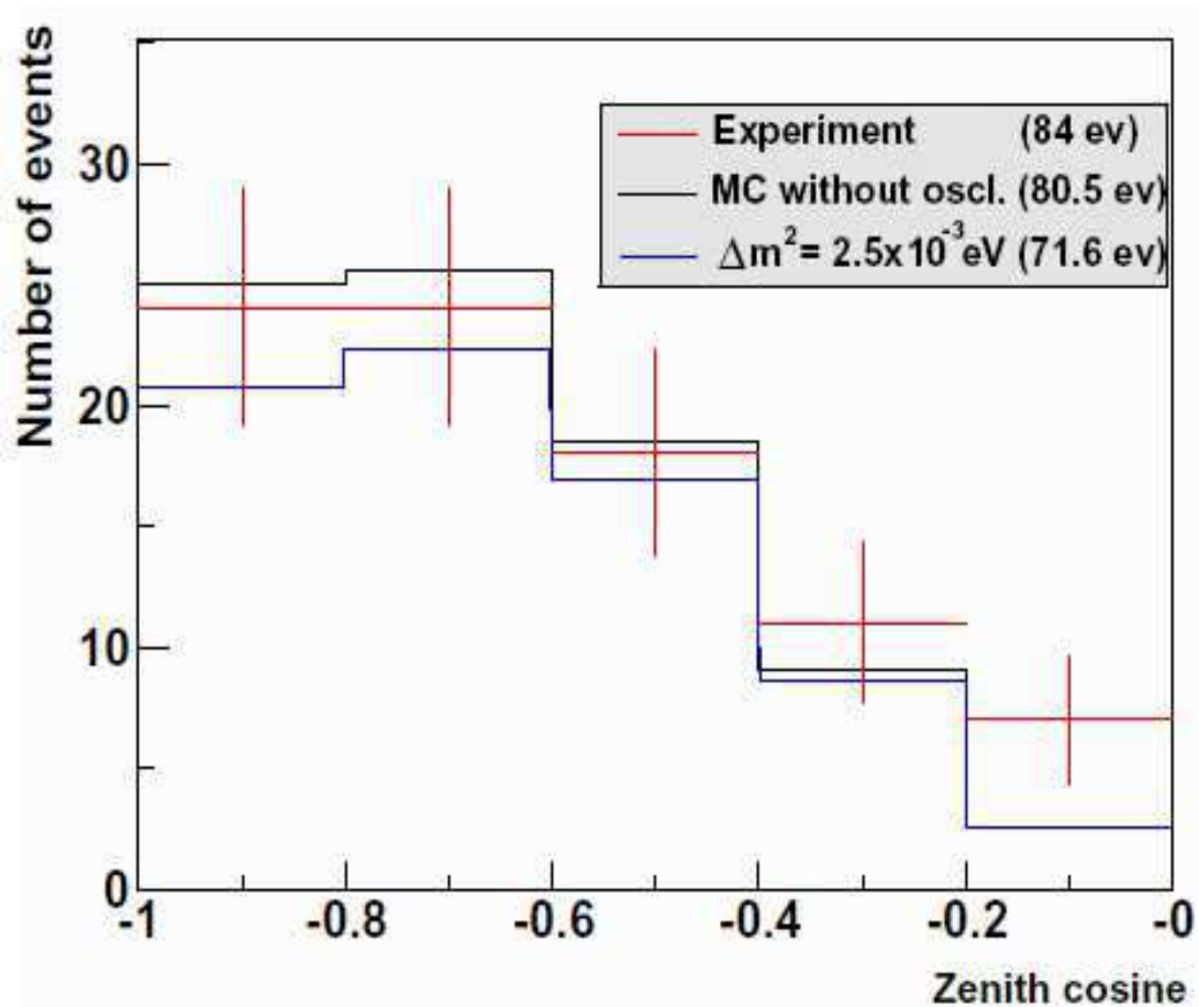
Figure 157: Zenith angle distribution of 84 upward-going reconstructed events in the Baikal NT-200 experiment and MC simulated distribution of upward muon tracks due to atmospheric neutrinos. E_{\text{th}} = 15 - 20 \text{ GeV} in this experiment. [From V. Aynutdinov et al. , “The BAIKAL neutrino project: Status, results and perspectives,” Nucl. Phys. B (Proc. Suppl.) 143 (2005) 335–342.]
