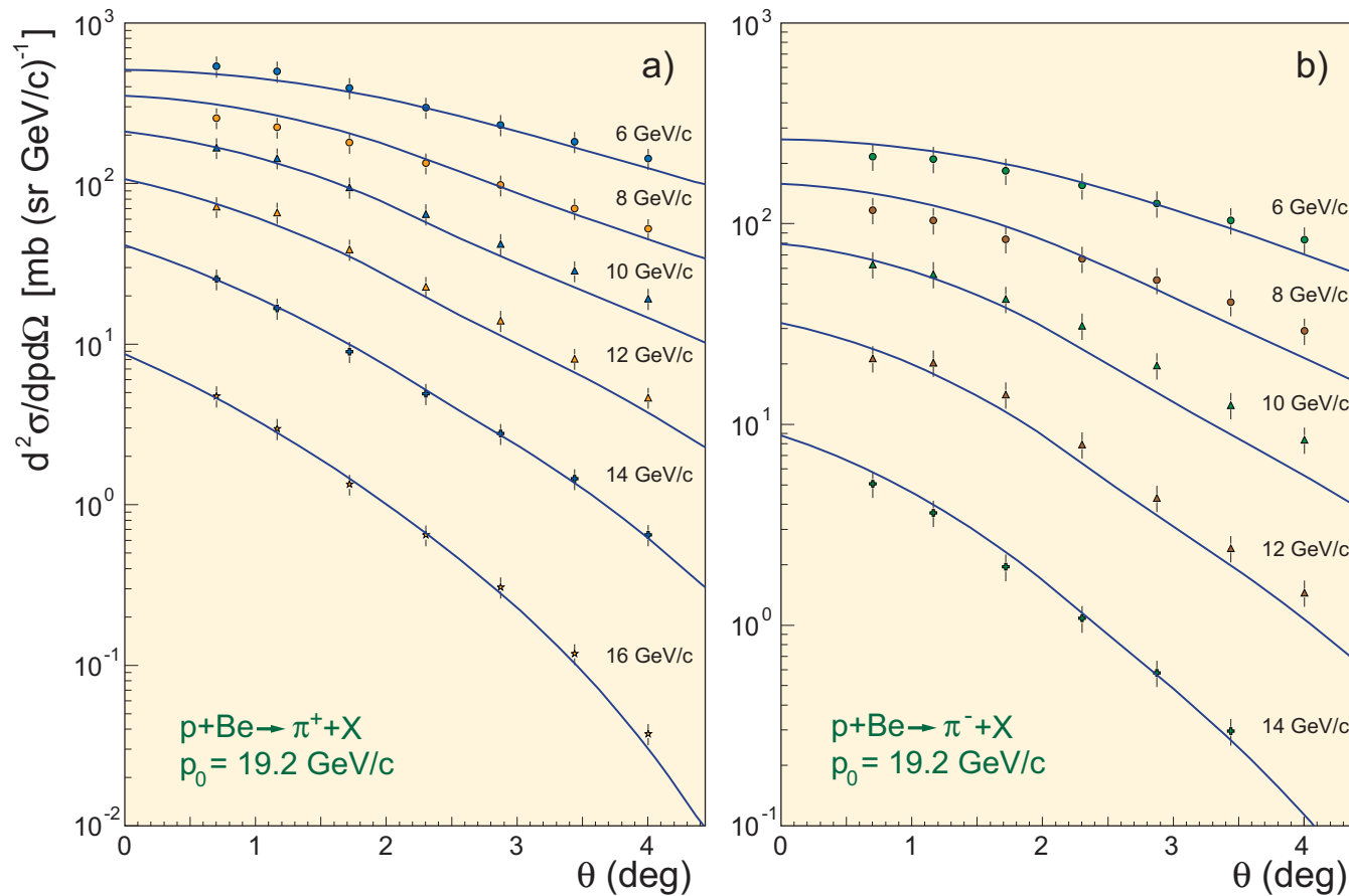
Figure 49: Differential cross sections of \pi^\pm production in interactions of 19.2 GeV/c momentum protons with Be target vs scattering angle. Curves are calculated in the KM model. Pion momenta are shown near the curves. Data points are from J. V. Allaby et al. , CERN Yellow Report 70–12, 1970 (unpublished).
