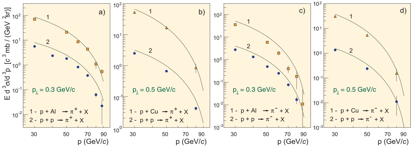
Figure 51: Invariant inclusive cross sections of \pi^\pm production in interactions of 100 GeV/c protons with p , Al an Cu targets vs pion momentum at two values of the pion transverse momentum. Curves are calculated in the KM model. Data points are from D. S. Barton et al. , Phys. Rev. D 27 (1983) 2580.
