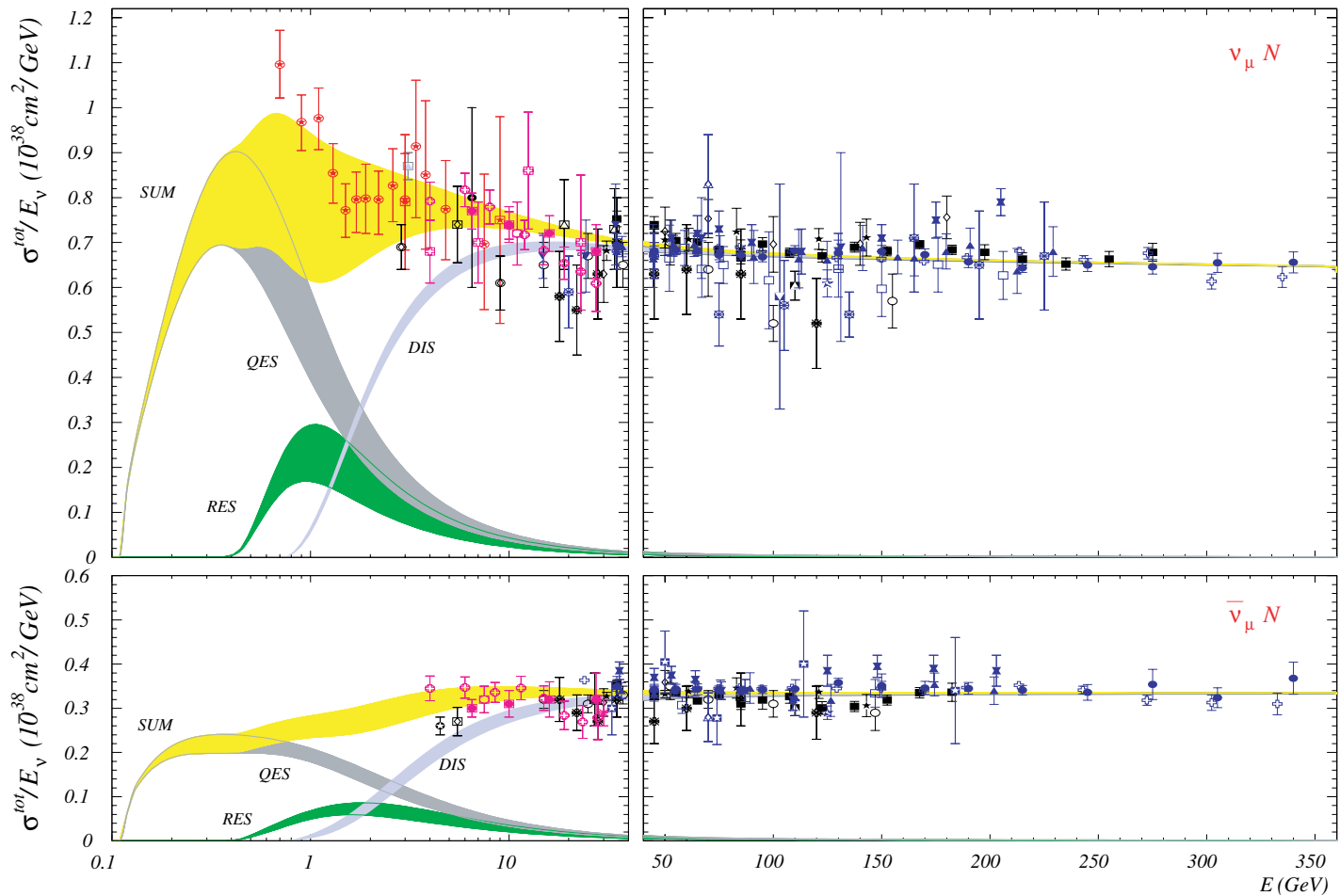
Figure 41: Comparison of theoretical estimation of the CC total cross sections for \nu_{\mu}N and \bar{\nu}_{\mu}N interactions with world survey experimental data. Uncertainties of the three main contributions and their sum are shown by the bands.
