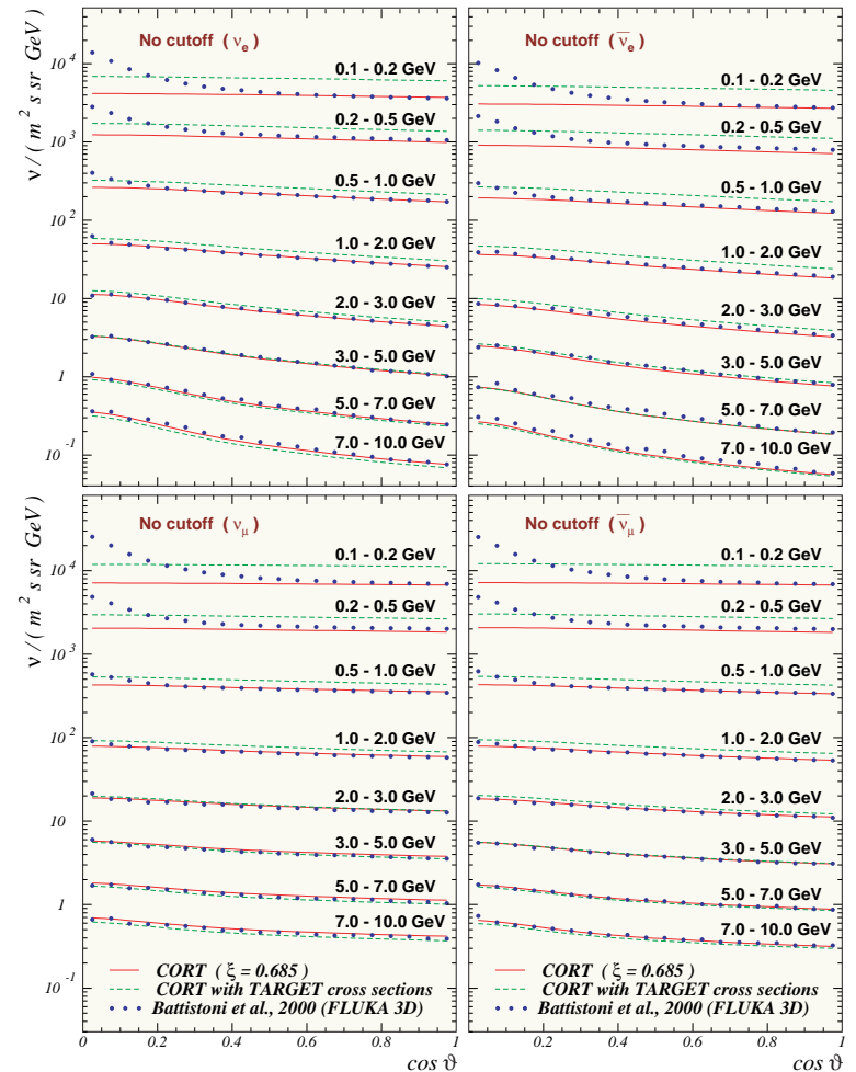
Figure 90: Zenithal distributions of down-going ANs on geomagnetic poles.
