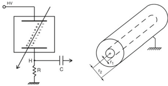
Fig. 4.15 Left Operational scheme of a ionization chamber. Right A chamber made in a “tube” shape, using coaxial cylindrical electrodes. From Braibant, Giacomelli and Spurio, “Particles and fundamental interactions,” Springer 2014
