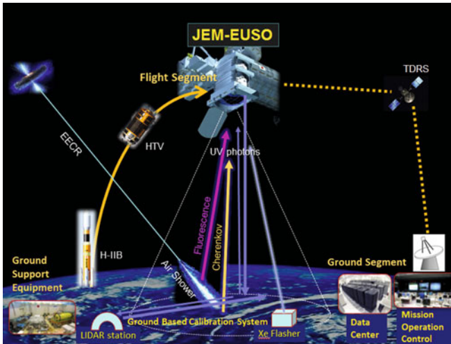
Fig. 4.46 JEM-EUSO observational principle. From http://jemeuso.riken.jp/en/
