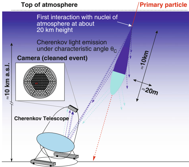
Fig. 4.51 The observational technique adopted by Cherenkov telescopes. Credit: R.M. Wagner, dissertation, MPI Munich 2007
