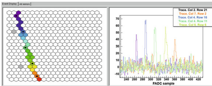
Fig. 4.40 Display of one shower in the focal plane of one of the Pierre Auger fluorescence telescopes. Left Pattern of the pixels with signal; right response (signal versus time, with a time bin of 100 ns) of the selected pixels (marked with a black dot in the left panel). The development of the shower in the atmosphere can be qualitatively pictured. From https://www.auger.org
