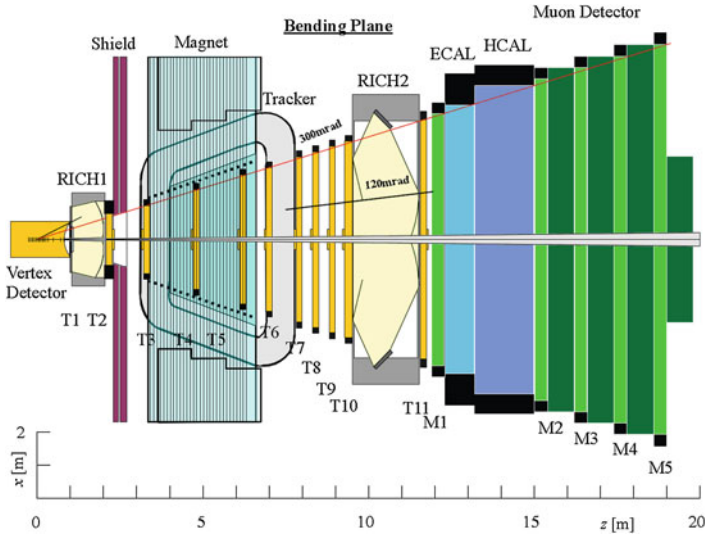
Fig. 4.27 Sketch of the LHCb detector. Credit: CERN
