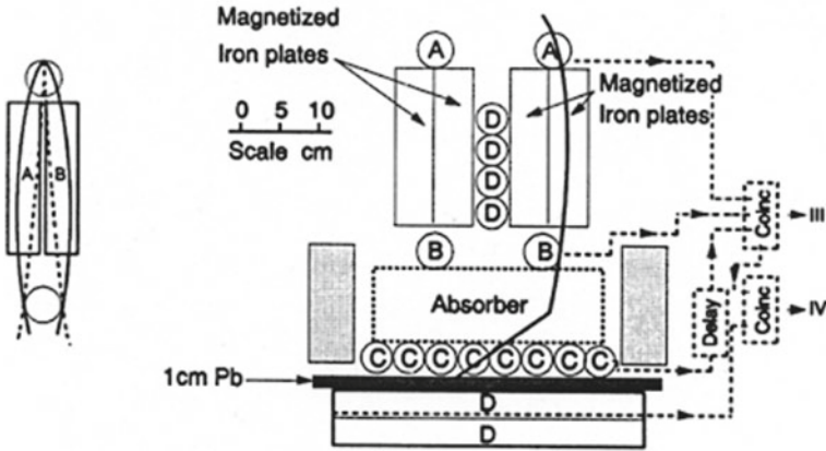
Fig. 3.10 Left a magnetic lens (invented by Rossi in 1930). Right setup of the Conversi, Pancini and Piccioni experiment. From M. Conversi, E. Pancini, O. Piccioni, “On the disintegration of negative mesons”, Physical Review 71 (1947) 209
