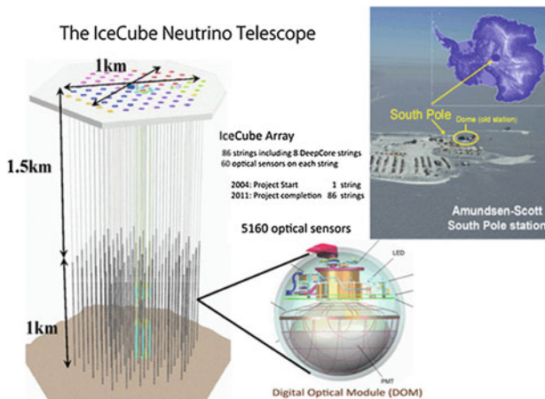
Fig. 4.59 The IceCube detector. Credit: http://www.icehap.chiba-u.jp/en/frontier/
