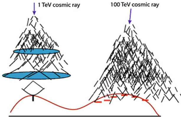
Fig. 4.49 Sketch of the operation of Cherenkov telescopes and of EAS detectors
