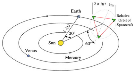
Fig. 4.62 The proposed LISA detector (the size is increased by a factor of 10). From M. Pitkin et al., “Gravitational Wave Detection by Interferometry (Ground and Space),” http://www.livingreviews.org/lrr-2011-5
