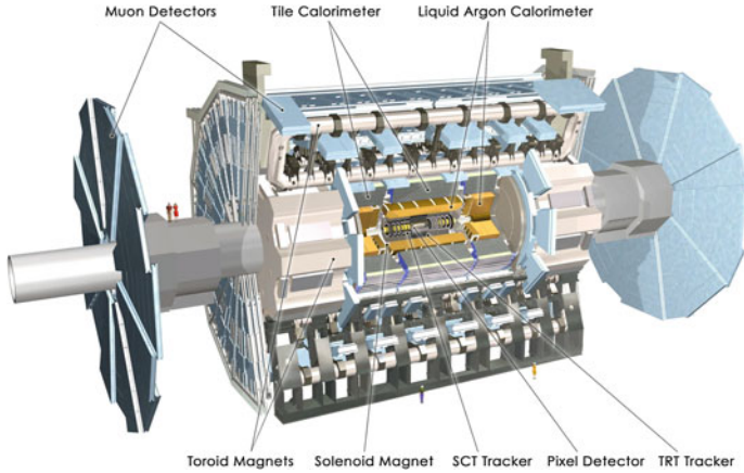
Fig. 4.33 Sketch of the ATLAS detector. Credit: CERN
