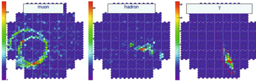
Fig. 4.53 Images from the focal camera of a Cherenkov telescope. The electromagnetic events differ from the hadronic events by several features: the envelope of the electromagnetic shower can be quite well described by an ellipse whereas the important fraction of large transverse momentum particles in hadronic showers will result in a more scattered reconstructed image. Muons are characterized by a conical section. From http://www.isdc.unige.ch/cta/images/outreach/
