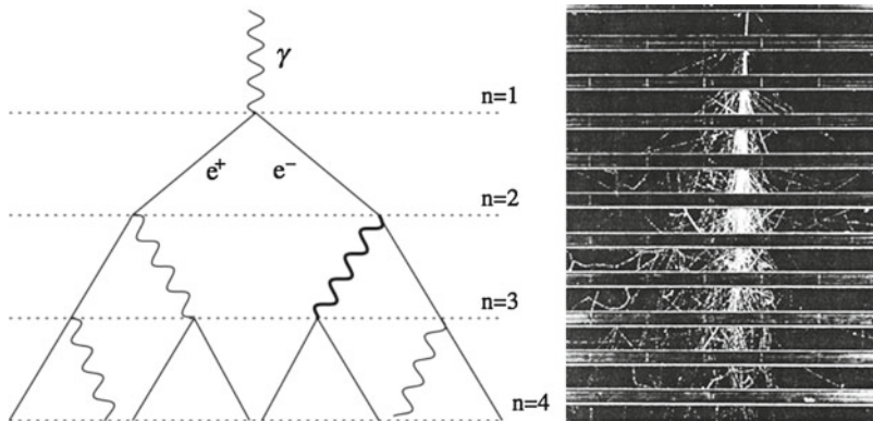
Fig. 4.10 Left Scheme of the Heitler approximation for the development of an electromagnetic shower. From J. Matthews, Astropart. Phys. 22 (2005) 387. Right Image of an electromagnetic shower developing through a number of brass plates 1.25 cm thick placed across a cloud chamber (from B. Rossi, “Cosmic rays”, McGraw-Hill 1964)
