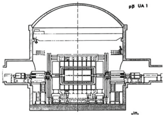
Fig. 6.32 Longitudinal cross section of the UA1 detector. From CERN http://cern-discoveries.web.cern.ch/cern-discoveries/courier/experiments/page-20.jpg
