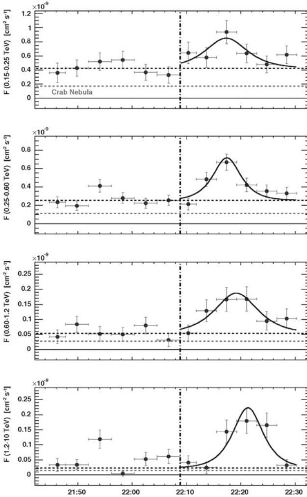
Fig. 10.59 Integral flux of Mkn 501 detected by MAGIC in four different energy ranges. From J. Albert et al., Phys. Lett. B668 (2008) 253
