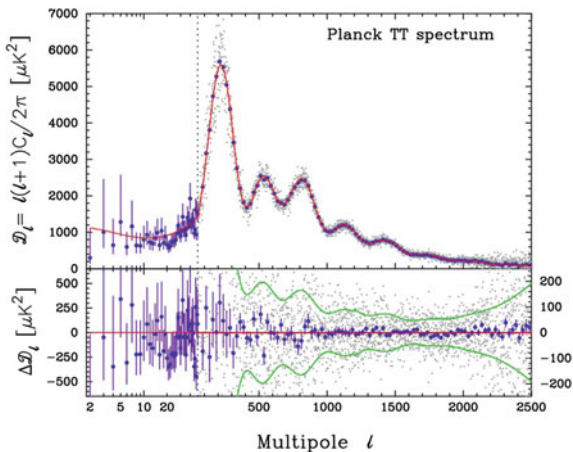
Fig. 8.10 Temperature power spectrum from the Planck experiment. In the lower panel the residuals with respect to the best \Lambda CDM fit (see later) are shown. Credits: Planck collaboration, P.A.R. Ade et al., Astr. Astrophys. 571 (2014) A16
