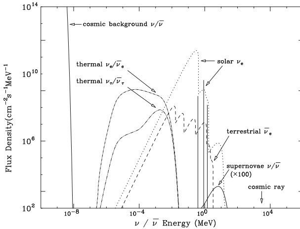
Fig. 10.41 Sources of neutrinos with energies below 1 TeV. From W.C. Haxton, arXiv:1209.3743 , to appear in Wiley’s Encyclopedia of Nuclear Physics
