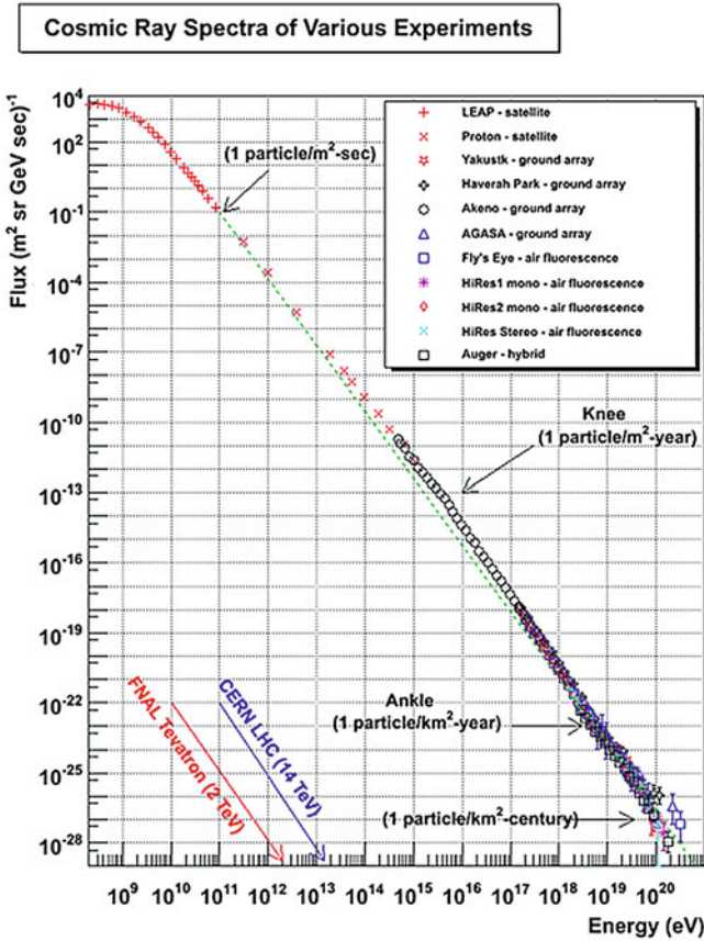
Fig. 10.1 Energy spectrum of charged cosmic rays. Credits: http://www.physics.utah.edu/~whanlon/spectrum.html
