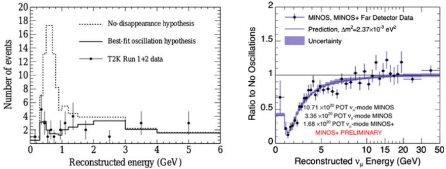
Fig. 9.13 Left The first T2K study on the disappearance of muon neutrinos: muon-antineutrino events with well-reconstructed energy recorded before 2011. The energy distribution is compared to the calculations with and without oscillations. From Phys. Rev. D 85, 031103 (2012). Right The ratio of the observed spectrum of muon neutrino interactions from MINOS to the predicted spectrum in the absence oscillations. The dark band represents the prediction assuming oscillations and its 1\sigma systematic uncertainty, using the best-fit oscillation parameters from MINOS. The observed data are well described by the oscillation model. From http://www-nuui.fnl.gov/PublicInfo/forscientists.html
