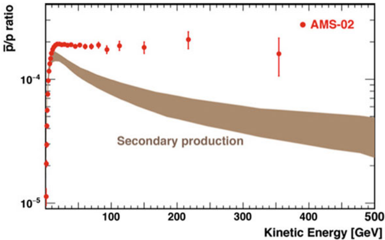
Fig. 10.11 Antiproton to proton ratio measured by AMS-02. Within the existing models of secondary production, the ratio lacks explanation
