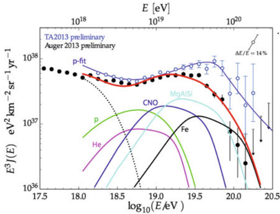
Fig. 10.54 Flux of UHE cosmic rays measured by the Telescope Array and by the Pierre Auger Observatory. Superposed are fits assuming pure proton ( light blue curve ) and mixed composition ( red curve ) scenarios. The curves below the result from the mixed mass composition fit. From K-H Kampert, P. Tinyakov, http://arxiv.org/abs/1405.0575 (Color in online)
