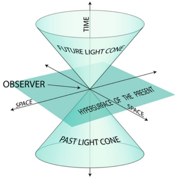
Fig. 2.15 Light cone. By Stib at en.wikipedia [GFDL http://www.gnu.org/copyleft/fdl.html ], via Wikimedia Commons
