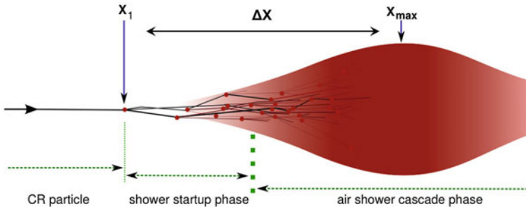
Fig. 10.3 Shower development scheme. Adapted from the Ph.D. thesis of R. Ulrich: “Measurement of the proton–air cross section using hybrid data of the Pierre Auger Observatory,” http://bibliothek.fzk.de/zb/berichte/FZKA7389.pdf
