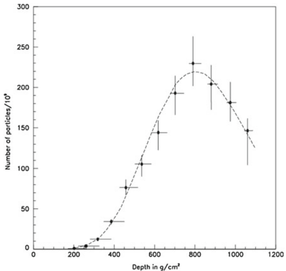
Fig. 4.42 Shower longitudinal profile of the most energetic event observed by the Fly's Eye experiment. From D.J. Bird et al., Astrophys. J. 441 (1995) 144
