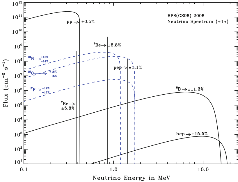
Fig. 9.3 The solar neutrino energy spectrum predicted by the SSM. For continuum sources, the fluxes are expressed in units of \text{cm}^{-2}\text{s}^{-1} \text{MeV}^{-1} at the Earth’s surface. For line sources, the units are number of neutrinos \text{cm}^{-2}\text{s}^{-1} . The total theoretical errors are quoted for each source. Source http://arxiv.org/abs/0811.2424
