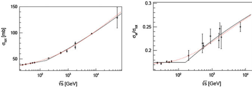
Fig. 6.70 The total cross section ( left ) and the ratio of the elastic and total cross sections in proton–proton interactions as a function of the center-of-mass energy. Points are experimental data and the lines are coming from a fit using one gray disk model. From R. Conceição et al., Nuclear Physics A 888 (2012) 58
