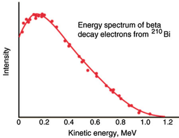
Fig. 2.3 Energy spectrum of electrons coming from the \beta decay of the ^{210}\text{Bi} (called historically “Radium E”) to ^{210}\text{Po} (called historically “Radium F”). From http://hyperphysics.phy-astr.gsu.edu/ ; the measurements are from G. J. Neary, Roy. Phys. Soc. (London) A175 (1940) 71
