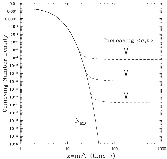
Fig. 8.26 The number density of a nonrelativistic massive particle as a function of time (expressed in terms of the ratio \frac{m_\chi c^2}{k_B T} ) for different values of \langle\sigma v\rangle (from D. Hooper, “TASI 2008 Lectures on Dark Matter”, arXiv:0901.4090 [hep-ph])
