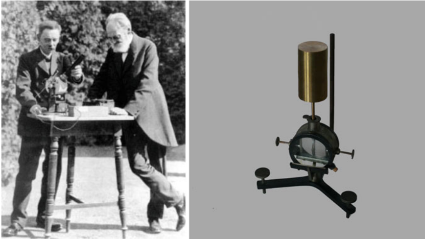
Fig. 3.2 Left The two friends Julius Elster and Hans Geitel, gymnasium teachers in Wolfenbittel, around 1900. Credit http://www.elster-geitel.de . Right an electroscopes developed by Elster and Geitel in the same period (private collection R. Fricke; photo by A. De Angelis)
