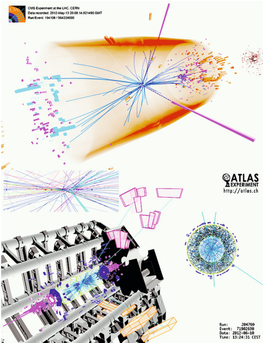
Fig. 7.23 Candidate Higgs boson events at the LHC. The upper is a Higgs decay into two photons ( dashed lines and towers ) recorded by CMS. The lower is a decay into four muons ( thick solid tracks ) recorded by ATLAS. Source CERN
