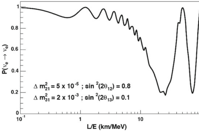
Fig. 9.10 The \nu_e survival probability as a function of L/E for fixed oscillation parameters as indicated in the figure. From http://www.hep.anl.gov/minos/reactor13/reactor13.pdf
