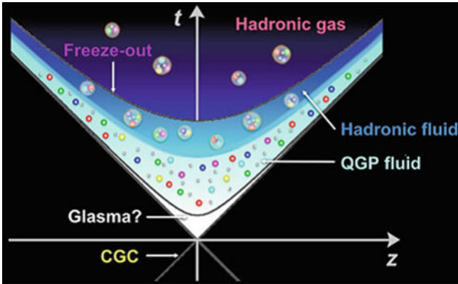
Fig. 6.78 An artistic representation of the time–space diagram of the evolution of the states created in Heavy Ion collisions. From “Relativistic Dissipative Hydrodynamic description of the Quark-Gluon Plasma” A. Monai 2014 ( http://www.springer.com/978-4-431-54797-6 )
