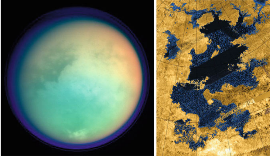
Fig. 11.8 Left Titan, a satellite of Saturn. Right Detail of Titan: note the presence of lakes on its surface. Credits: NASA (Cassini)
