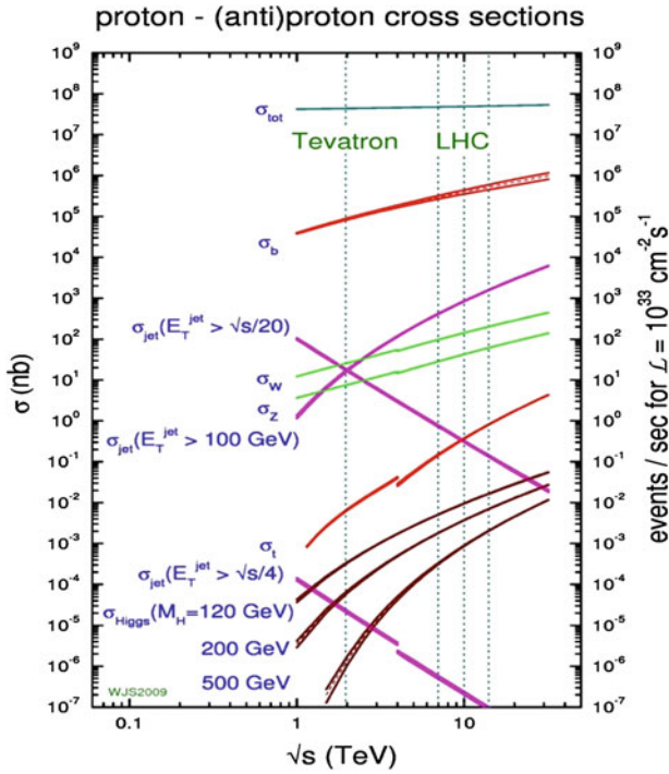
Fig. 6.63 Proton–(anti)proton cross sections at high energies. Cross section values for several important processes are given. The right vertical axis reports the number of events for a luminosity value L = 10^{33} \text{ cm}^{-2} \text{ s}^{-1} . From N. Cartiglia, arXiv:1305.6131 [hep-ex]
