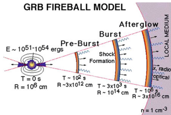
Fig. 10.38 The fireball model. Credits: http://www.swift.ac.uk/about/grb.php
