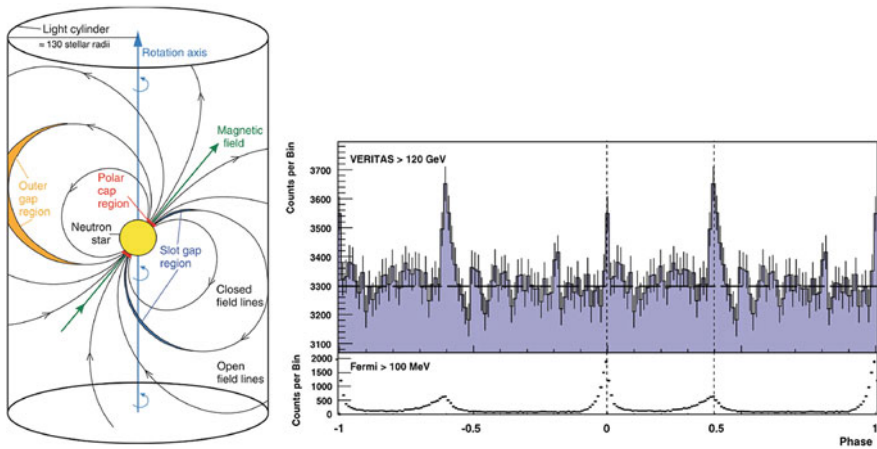
Fig. 10.33 Left Schematic of the Crab Pulsar. Electrons are trapped and accelerated along the magnetic field lines of the pulsar and can emit electromagnetic synchrotron radiation. Vacuum gaps or vacuum regions occur at the “polar cap” close to the neutron star surface and in the outer region; in these regions density varies and thus one can have acceleration. From MAGIC Collaboration, Science 322 (2008) 1221. Right Time-resolved emission from the Crab Pulsar at HE and VHE; the period is about 33 ms. From VERITAS Collaboration, Science 334 (2011) 69
