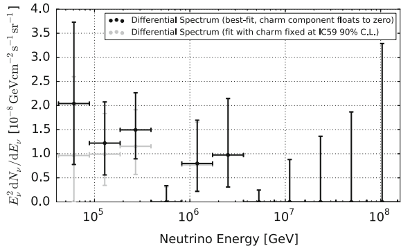
Fig. 10.24 Extraterrestrial neutrino flux ( \nu + \bar{\nu} ) as a function of energy, after subtraction of the background from atmospheric neutrinos ( gray lines indicate an extreme model of background). Credit: IceCube collaboration
