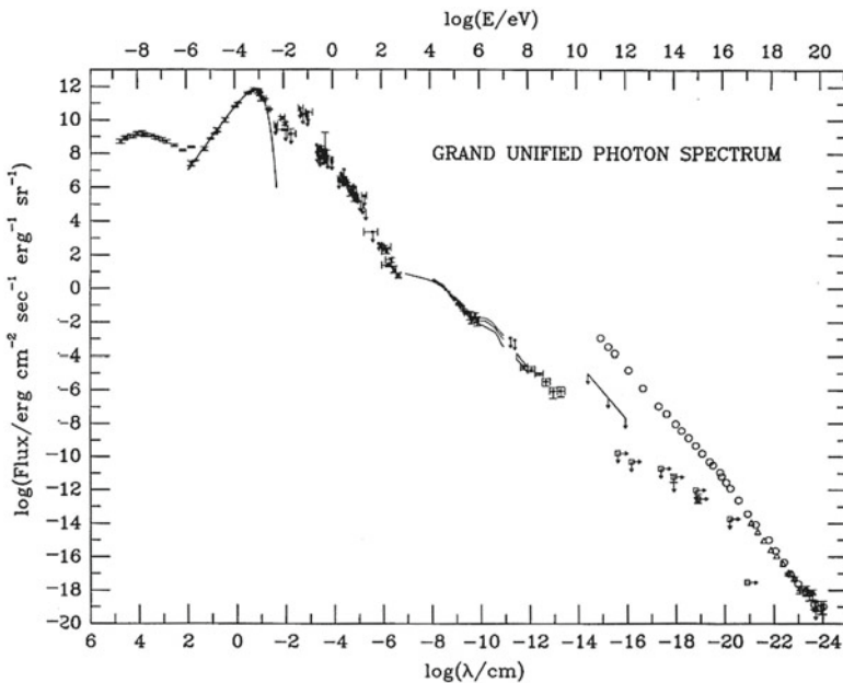
Fig. 10.13 Spectrum of photons was experimentally detected at different energies. From M.T. Ressel and M.S. Turner 1989, "The grand unified photon spectrum: a coherent view of the diffuse extragalactic background radiation," [Batavia, Ill.]: Fermi National Accelerator Laboratory. http://purl.fdlp.gov/GPO/gpo48234
