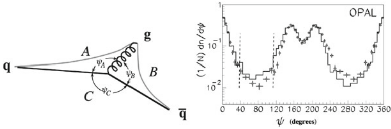
Fig. 7.16 Left Sketch of a 3-jet event in e^+e^- annihilations. In the Lund string model for fragmentation, string segments span the region between the quark q and the gluon g and between the antiquark \bar{q} and the gluon. Right Experimental measurement of the particle flow (1/N)dn/d\psi , for events with \psi_A = 150^\circ \pm 10^\circ and \psi_C = 150^\circ \pm 10^\circ . The points with errors show the flow from the higher energy quark jet to the low-energy quark jet and then to the gluon jet; in the histogram, it is shown the measured particle flow for the same events, starting at the high energy quark jet but proceeding in the opposite sense. The dashed lines show the regions, almost free of the fragmentation uncertainties, where the effect is visible. From OPAL Collaboration, Phys. Lett. B261 (1991) 334
