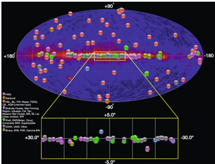
Fig. 10.15 Sources of VHE emission plotted in galactic coordinates. The background represents the high-energy gamma rays detected by Fermi-LAT. The region near the Galactic Center is enlarged. From http://tevcat.uchicago.edu/ , May 2015
