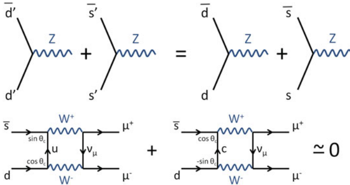
Fig. 6.41 FCNC suppression by diagram cancellation
