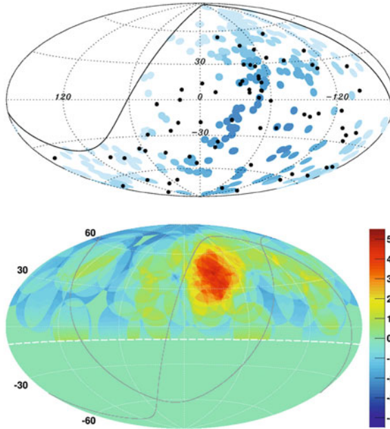
Fig. 10.8 Top Positions of the AGN within 71 Mpc used in the correlation search by Auger ( dots ) and circles centered at the arrival directions of the events with E > 57 EeV observed by Auger in galactic coordinates. Bottom Map in equatorial coordinates (note the difference of coordinates with respect to the plot on top ) for the events above 57 EeV as seen by the Telescope Array collaboration up to May 2014. The color scale represents the estimated significance. For details see arXiv:1404.5890 . Image credit: K Kawata/University of Tokyo Institute for Cosmic Ray Research
