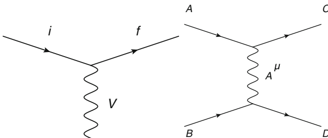
Fig. 6.8 Left Schematic representation of the first-order interaction of a particle in a field. Right Schematic representation (Feynman diagram) of the first-order elastic scattering of two charged non-identical particles
