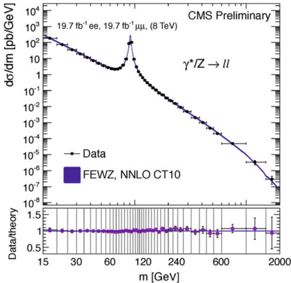
Fig. 6.66 Dilepton cross section measured by CMS. From V. Khachatryan et al. (CMS Collaboration), The European Physical Journal C75 (2015) 147
