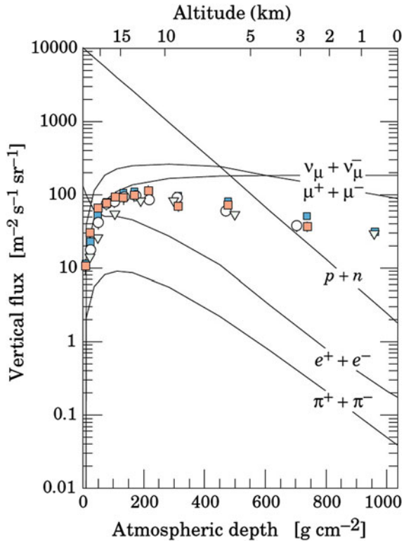
Fig. 10.12 Fluxes of cosmic rays with E > 1 GeV in the atmosphere as a function of height (simulation). The points show experimental measurements of negative muons. From K.A. Olive et al. (Particle Data Group), Chin. Phys. C 38 (2014) 090001
