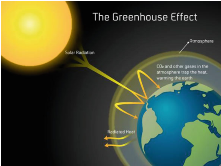
Fig. 11.3 Greenhouse gases trap and keep most of the infrared radiation in the low atmosphere. Source NASA
