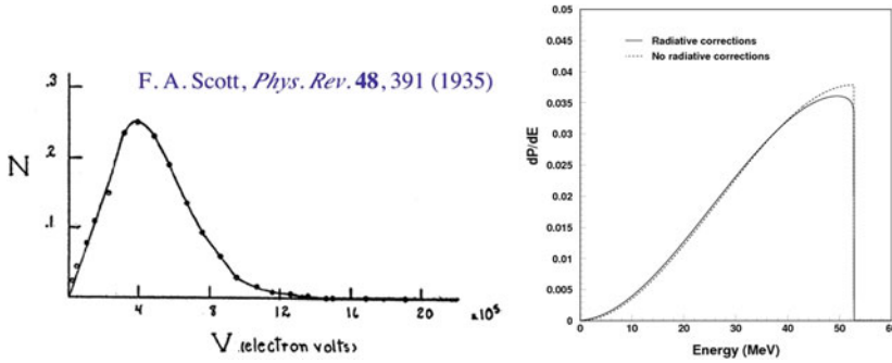
Fig. 6.18 Electron energy spectrum in \beta decay of thallium 206 (left) and in \mu decay (right). Sources F.A. Scott, Phys. Rev. 48 (1935) 391; ICARUS Collaboration (S. Amoruso et al.), Eur. Phys. J. C33 (2004) 233
