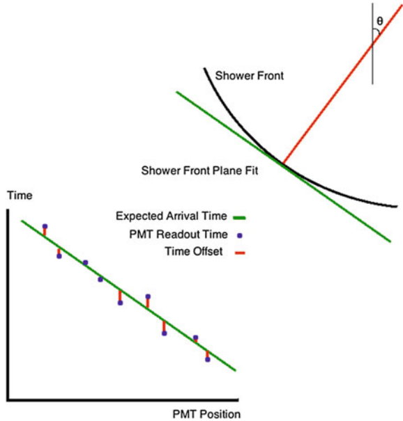
Fig. 4.38 Air shower front arriving at the Earth surface; times of arrival are measured by surface detectors and allow the determination of the direction. From HAWC Collaboration, A.U. Abeyssekara et al. arXiv:1310.0074
