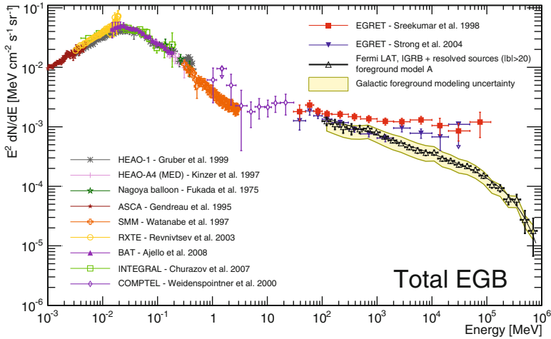
Fig. 10.14 Spectrum of the total extragalactic gamma ray emission measured by the Fermi-LAT. From M. Ackermann et al., The Astrophysical Journal 799 (2015) 86
