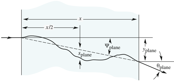
Fig. 4.6 Multiple Coulomb scattering. From K.A. Olive et al. (Particle Data Group), Chin. Phys. C 38 (2014) 090001
