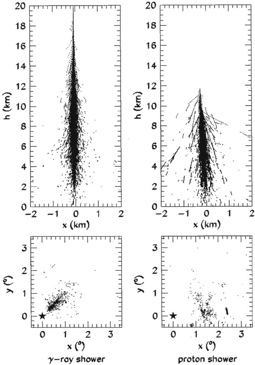
Fig. 4.52 Development of vertical 1 TeV photon ( left ) and proton ( right ) showers in the atmosphere. The upper panels show the positions in the atmosphere of all shower electrons above the Cherenkov threshold; the lower panels show the resulting Cherenkov images in the focal plane of a 10m reflecting mirror when the showers fall 100m from the detector (the center of the focal plane is indicated by a star ). From C.M. Hoffmann et al., “Gamma-ray astronomy at high energies,” Reviews of Modern Physics 71 (1999) 897
