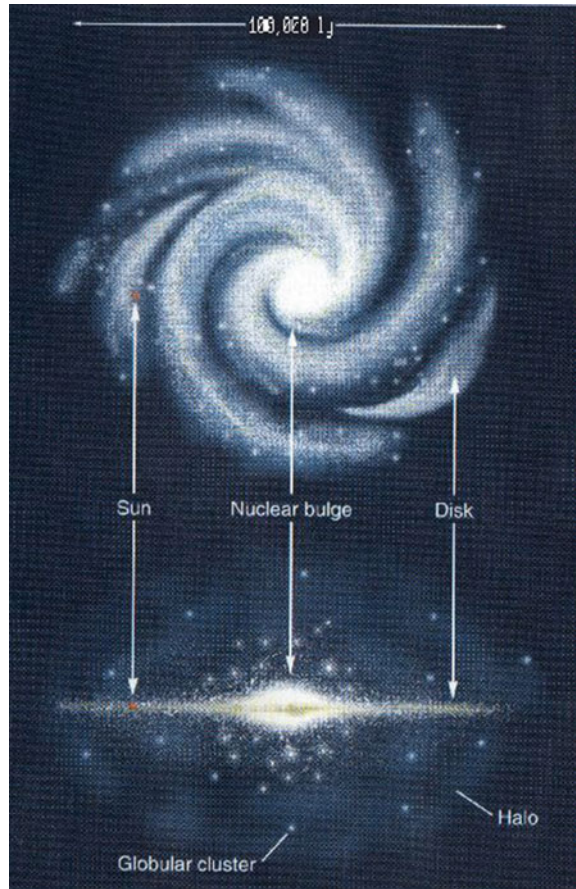
Fig. 1.3 The Milky Way seen from top and from side. Source http://casswww.ucsd.edu/archive/public/tutorial/mw.html
