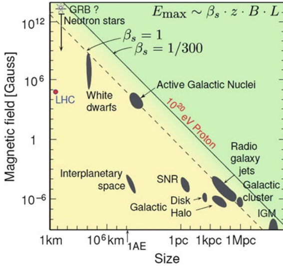
Fig. 10.32 The “Hillas plot” represents astrophysical objects which are potential cosmic ray accelerators on a two-dimensional diagram where on the horizontal direction the size linear extension R of the accelerator, and on the vertical direction the magnetic field strength B are plotted. The maximal acceleration energy E is proportional to ZRBv , where v is the shock velocity in units of the speed of light and Z is the absolute value of the particle charge in units of the electron charge. Particular values for the maximal energy correspond to diagonal lines in this diagram and can be realized either in a large, low field acceleration region or in a compact accelerator with high magnetic fields. Typical shock velocities go from v \sim 1 in extreme environments down to v \sim 1/300 . From http://astro.uni-wuppertal.de/~kampert
