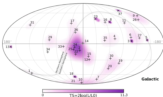
Fig. 10.23 Arrival directions of the IceCube events above 30 TeV in galactic coordinates (numbers correspond to the numbering in IceCube’s catalog). Shower-like events (angular resolution \sim 15^\circ ) are marked with “+” and those containing muon tracks (angular resolution \sim 1^\circ ) with “x.” The gray line denotes the equatorial plane. Colors show the test statistic (TS) for the point source clustering test at each location. No significant clustering was observed. Credit: IceCube collaboration
