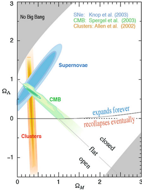
Fig. 8.29 Confidence regions in the plane (\Omega_M, \Omega_\Lambda) . Credit: http://supernova.lbl.gov
