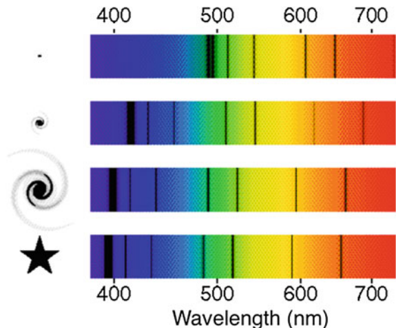
Fig. 1.4 Redshift of emission spectrum of stars and galaxies at different distances. A star in our galaxy is shown at the bottom left with its spectrum on the bottom right. The spectrum shows the dark absorption lines, which can be used to identify the chemical elements involved. The other three spectra and pictures from bottom to top show a nearby galaxy, a medium distance galaxy, and a distant galaxy. Using the redshift we can calculate the relative radial velocity between these objects and the Earth. From http://www.indiana.edu/~geol105
