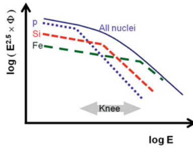
Fig. 10.29 The interpretation of the knee as due to the dependence of the maximum energy on the nuclear charge Z . The flux of each nuclear species sharply decreases after a given cutoff. The behavior of hydrogen, silicon ( Z = 14 ) and iron ( Z = 26 ) nuclei are depicted in figure. From [F10.1]
