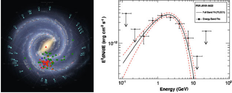
Fig. 10.34 Left Map of the pulsars detected by the Fermi-LAT (the Sun is roughly in the center of the distribution). The open squares with arrows indicate the lines of sight toward pulsars for which no distance estimates exist. Credit: NASA. Right Spectral energy distribution from a typical high-energy pulsar. Credit: NASA
