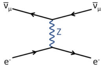
Fig. 6.28 Gargamelle picture ( top ) and sketch ( bottom ) of the first observed neutral current process \bar{\nu}_\mu e^- \rightarrow \bar{\nu}_\mu e^- . A muon anti-neutrino coming from the left knocks an electron forward, creating a small shower of electron-positron pairs. Source CERN
