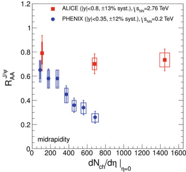
Fig. 6.77 The nuclear modification factor R_{AA} for inclusive J/\psi production at midrapidity as reported by PHENIX (RHIC) and ALICE (LHC) experiments at center-of-mass energy per nucleon of 0.2 and 2.76 TeV, respectively. From http://cerncourier.com/cws/article/cern/48619
