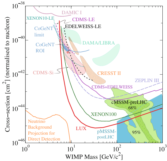
Fig. 8.36 Compilation of experimental results on cross sections of WIMPs versus masses. The areas labeled as DAMA/LIBRA, CREST II, CDMS-Si, and CoGeNT indicate regions of possible signals from those experiments. For context, some supersymmetry implications are also given. From K.A. Olive et al. (Particle Data Group), Chin. Phys. C 38 (2014) 090001, in which experiments are also described in better detail
