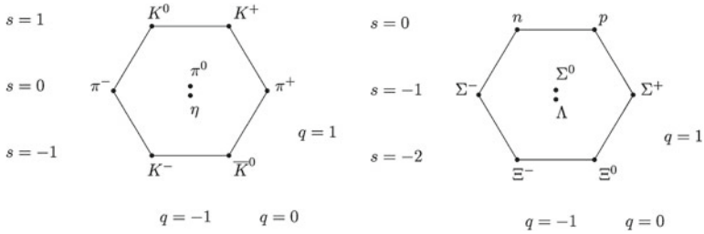
Fig. 5.7 Fundamental meson and baryon octets: on the left spin 0, parity -1 (pseudo-scalar mesons); on the right the spin 1/2 baryons. The I_3 axis is the abscissa, while the Y axis is the ordinate
