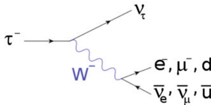
Fig. 5.29 Feynman diagram for the \tau^- decay in \nu_\tau e^- \bar{\nu}_e , \nu_\tau \mu^- \bar{\nu}_\mu , \nu_\tau d \bar{u} . By en:User:JabberWok and Time 3000 [GFDL http://www.gnu.org/copyleft/fdl.html ], via Wikimedia Commons
