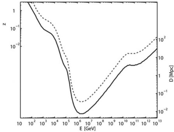
Fig. 10.51 Curves corresponding to the gamma ray horizon \tau(E, z) = 1 (lower) and to a survival probability of e^{-\tau(E, z)} = 1\% (upper). Adapted from A. de Angelis, G. Galanti, M. Roncadelli, MNRAS 432 (2013) 3245
