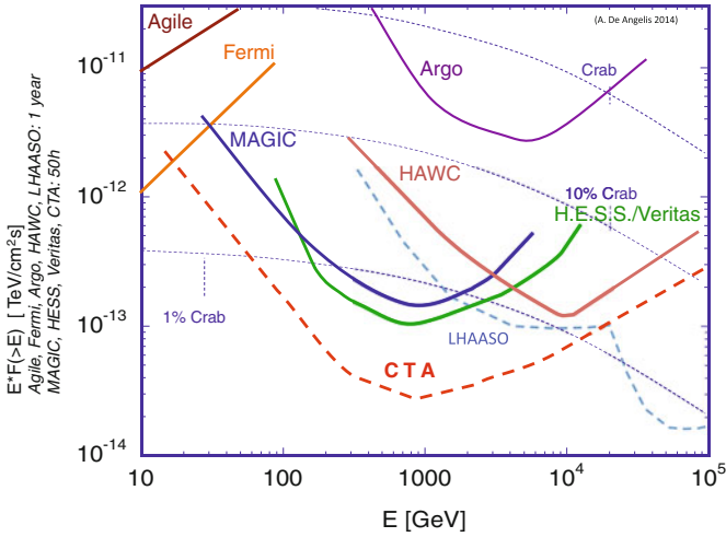
Fig. 4.56 Sensitivities of some present and future HE gamma detectors, measured as the minimum intensity source detectable at 5\sigma . The performance for EAS and satellite detector is based on one year of data taking; for Cherenkov telescopes it is based on 50 h of data
