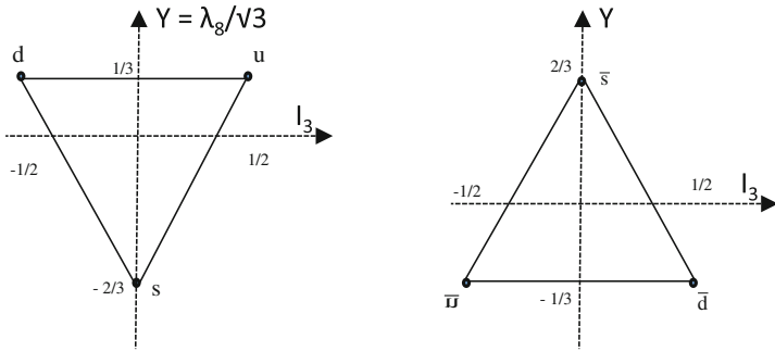
Fig. 5.10 Fundamental representations (3) and \bar{(3)} of SU(3)
