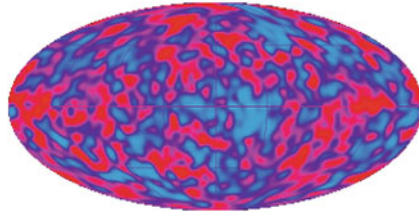
Fig. 8.8 CMB temperature fluctuations sky map as measured by COBE after the subtraction of the dipole component and of the emission from our Galaxy. http://lambda.gsfc.nasa.gov/product/cobe/
