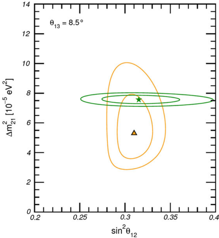
Fig. 9.7 Allowed parameter regions (at 1\sigma and 2\sigma ) in the (\sin^2(\theta_{12}), \Delta m^2_{21}) space for the combined analysis of solar neutrino data and for the analysis of KamLAND data. The result for KamLAND is illustrated by the ellipses with horizontal major axis (with the best fit marked by a green star ). Figure adapted from NuFIT2014: M.C. Gonzalez-Garcia, M. Maltoni and T. Schwetz, “Updated fit to three neutrino mixing: status of leptonic CP violation”, JHEP 11 (2014) 052 (Color in online)
