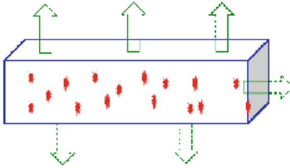
Fig. 10.45 The leaky-box model: a sketch
