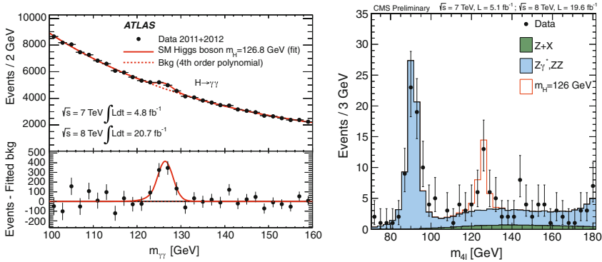
Fig. 7.24 Invariant mass of the \gamma\gamma candidates in the ATLAS experiment (left; in the lower part of the plot the residuals from the fit to the background are shown) and of the 4-lepton events in CMS (right; the expected background is indicated by the dark area, including the peak close to the Z mass and coming from Z\gamma^* events). From K.A. Olive et al. (Particle Data Group), Chin. Phys. C 38 (2014) 090001
