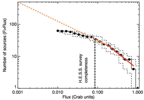
Fig. 10.53 “( \log N - \log S )” diagram of the VHE Galactic sources. From M. Renaud, http://arxiv.org/abs/0905.1287
