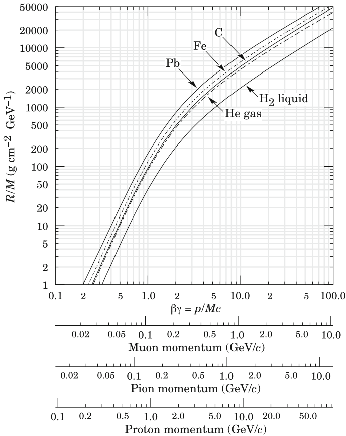
Fig. 4.7 Range per unit of density and of mass for heavy charged particles in liquid (bubble chamber) hydrogen, helium gas, carbon, iron, and lead. Example: a K^+ with momentum 700 MeV/c, \beta\gamma \simeq 1.42 , and we read R/M \simeq 396 , in lead, corresponding to a range of 195 g/cm 2 . From K.A. Olive et al. (Particle Data Group), Chin. Phys. C 38 (2014) 090001
