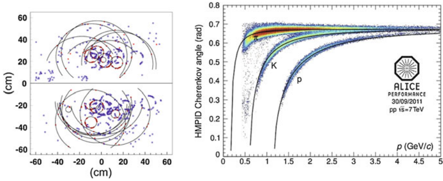
Fig. 4.22 Left Image of the hits on the photon detectors of the RICHs of the LHCb experiment at CERN with superimposed rings. Credit: LHCb collaboration. Right Dependence of the Cherenkov angle measured by the RICH of the ALICE experiment at CERN on the particle momentum; the angle can be used to measure the mass through Eq. 4.6 ( \beta = p/E ). Credit: ALICE Collaboration
