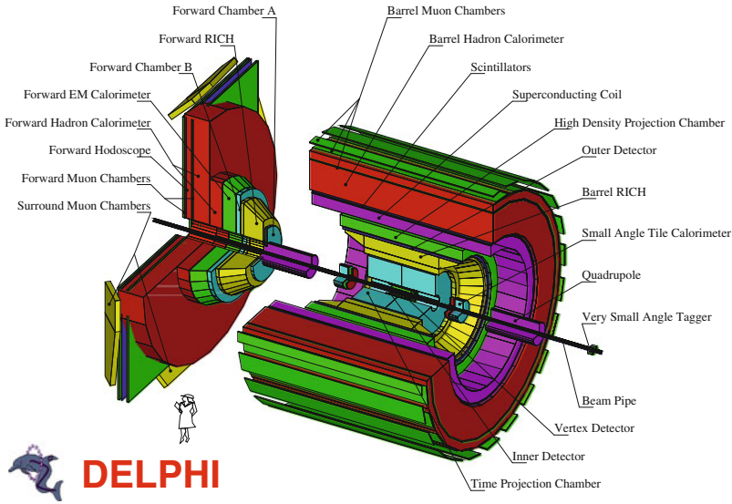
Fig. 4.29 The DELPHI detector at LEP (Source CERN)
