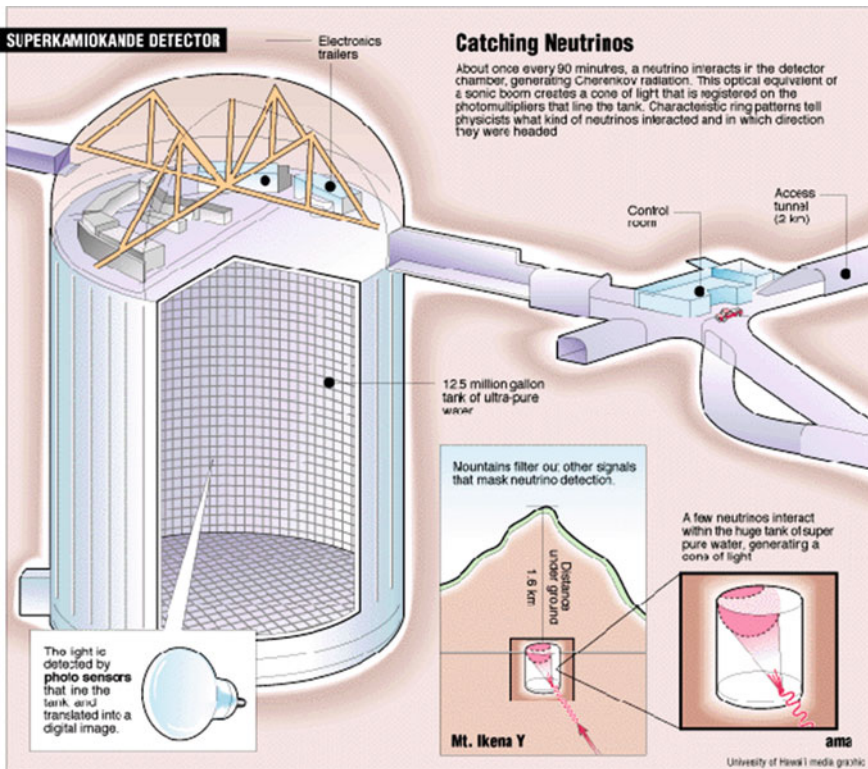
Fig. 4.58 The Super-Kamiokande detector (from the Super-Kamiokande web site)
