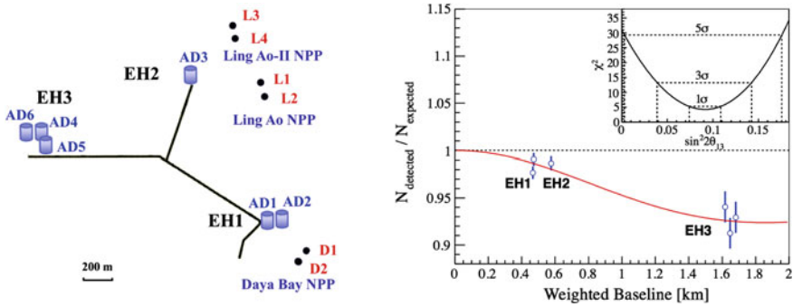
Fig. 9.11 Left Layout of the Daya Bay experiment. The dots represent reactors, labeled as D1, D2, L1, L2, L3, and L4; the locations of the detectors are labeled EH1, EH2 and EH3. Right The \bar{\nu}_e disappearance as measured by the Daya Bay experiment. Right Ratio of the measured signal in each detector versus the signal expected assuming no oscillation. The oscillation survival probability at the best-fit \sin^2 2\theta_{13} value is given by the smooth curve . The \chi^2 versus \sin^2 2\theta_{13} is shown in the inset . Figures from F.P. An et al., Phys. Rev. Lett. 108 (2012) 171803
