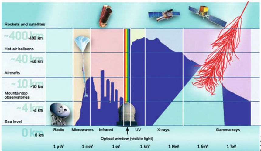
Fig. 4.47 Transparency of the atmosphere for different photon energies and possible detection techniques. Source A. De Angelis and L. Peruzzo, “Le magie del telescopio MAGIC,” Le Scienze , April 2007
