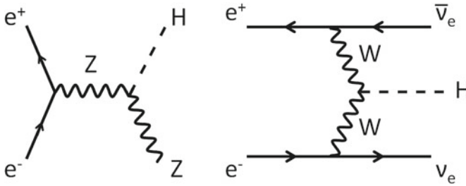
Fig. 7.20 Main Higgs production mechanisms at LEP: Higgs-strahlung ( left ) and vector boson fusion ( right )
