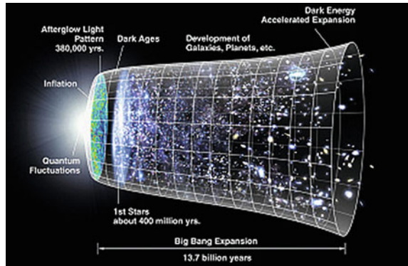
Fig. 8.31 Timeline of our Universe. Credits: NASA ( http://map.gsfc.nasa.gov/ )
