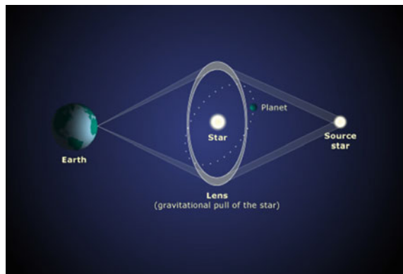
Fig. 11.9 A massive object will bend the light of a bright background object (the source). This can generate distorted, magnified, and brightened images of the background source. The effect can be enhanced if a planet orbiting the lens is aligned. http://www.teara.govt.nz/en/diagram/8008/gravitational-microlensing
