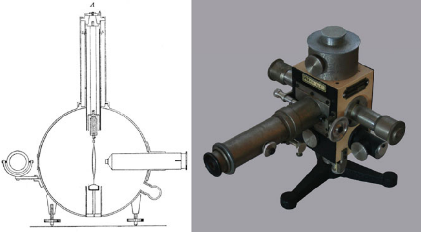
Fig. 3.3 Left Scheme of the Wulf electroscope (drawn by Wulf himself; reprinted from Z. Phys. [public domain]). The main cylinder was made of zinc, 17 cm in diameter and 13 cm deep. The distance between the two silicon glass wires (at the center) was measured using the microscope to the right. The wires were illuminated using the mirror to the left. According to Wulf, the sensitivity of the instrument was 1 V, as measured by the decrease of the inter-wire distance. Right an electroscope used by Wulf (private collection R. Fricke; photo by A. De Angelis)
