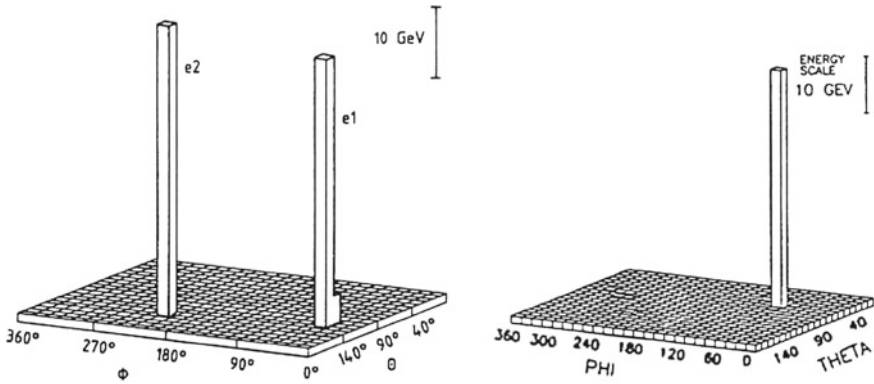
Fig. 6.33 Left Two high-energy deposits from a Z \rightarrow e^-e^+ event seen in the electromagnetic calorimeter of the UA2 experiment. Right One high-energy deposit and the missing transverse momentum from a W^\pm X \rightarrow e^\pm\nu_e event. From http://cern-discoveries.web.cern.ch
