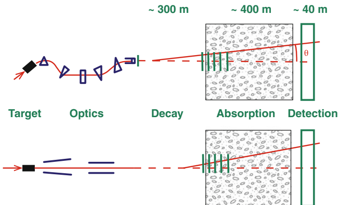
Fig. 6.25 Neutrino narrow-band beam ( top ) and wide-band beam ( bottom ) production
