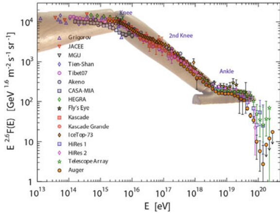
Fig. 10.2 Anthropomorphic representation of the cosmic ray energy spectrum coming from experimental measurements by different experiments; the spectrum has been multiplied by E^{2.6} . From Ref. [10.1] in the “Further reading”
