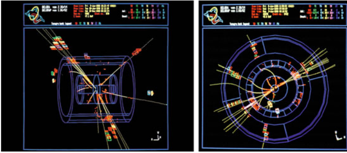
Fig. 4.30 Two events reconstructed by DELPHI, projected on the xz plane ( left ) and on the xy plane ( right ). Credits: CERN
