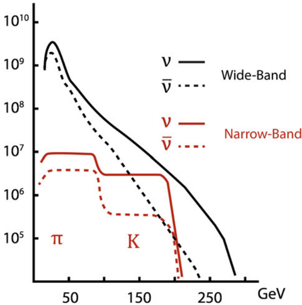
Fig. 6.26 Narrow-band and wide-band neutrino energy spectra. The y axis represents the number of particles per bunch
