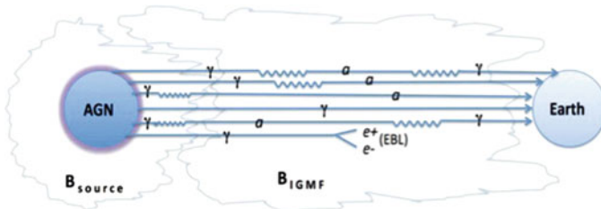
Fig. 10.62 Illustration of gamma ray propagation in the presence of oscillations between gamma rays and axion-like particles. From M.A. Sanchez-Conde et al., Phys. Rev. D79 (2009) 123511
