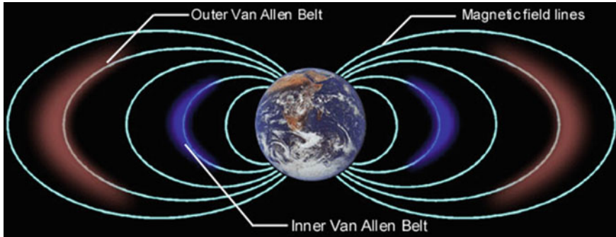
Fig. 11.4 The Earth's magnetic field and the Van Allen belts. From http://www.redorbit.com/
