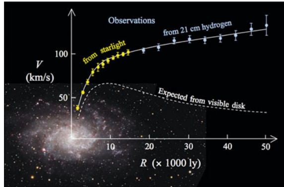
Fig. 8.12 Rotation curve of the Galaxy M33 (from http://en.wikipedia.org/wiki/Galaxy_rotation_curve#/media/File:M33_rotation_curve_HI.gif , public domain)
