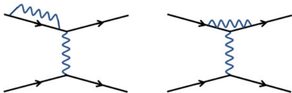
Fig. 6.12 Higher order diagrams with a fermion loop leading to the renormalization of the fermion mass ( left ) and of the magnetic moment ( right )
