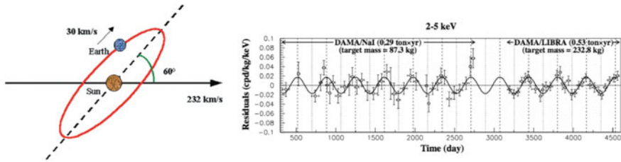
Fig. 8.34 Left the directions of the Sun's and the Earth's motions during a year. Assuming the WIMPs to be on average at rest in the Galaxy, the average speed of the WIMPs relative to the Earth is modulated with a period of 1 year. Right annual modulation of the total counting rate (background plus possible dark matter signal) in 7 years of data with the DAMA detector. A constant counting rate has been subtracted. From R. Bernabei et al., Riv. Nuovo Cim. 26 (2003) 1
