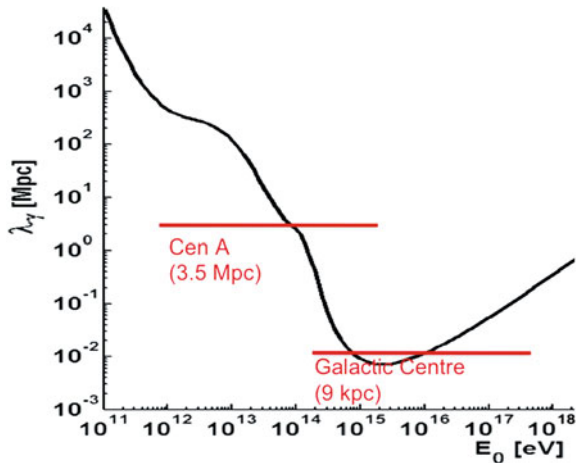
Fig. 10.50 Mean free path as a function of the photon energy, at z = 0 . Adapted from A. de Angelis, G. Galanti, M. Roncadelli, MNRAS 432 (2013) 3245
