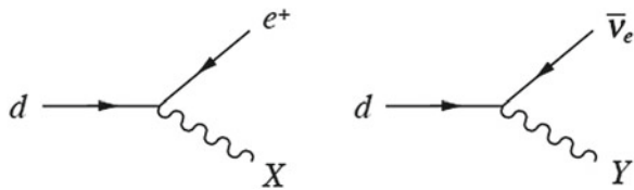
Fig. 7.27 Transitions between quarks and leptons are possible in GUTs
