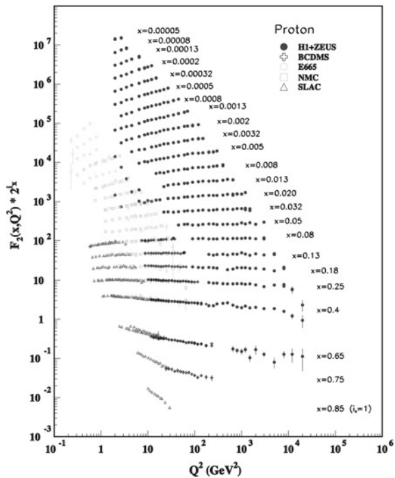
Fig. 5.26 Q^2 dependence of F_2^{ep} . From K.A. Olive et al. (Particle Data Group), Chin. Phys. C 38 (2014) 090001
