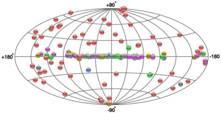
Fig. 1.10 Map of the emitters of photons above 100 GeV in the Universe, in galactic coordinates (from the TeV CAT catalog). The sources are indicated as circles—the colors represent different kinds of emitters which will be explained in Chap. 10. From http://tevcat.uchicago.edu/
