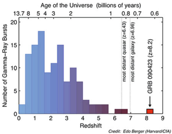
Fig. 10.20 Distribution of redshifts and corresponding age of the Universe for gamma ray bursts detected by NASA’s Swift satellite. Credit: Edo Berger (Harvard), 2009
