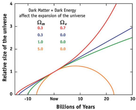
Fig. 8.25 Evolution of the Universe in a two-component model (matter and vacuum) for different (\Omega_m, \Omega_\Lambda) values. (from http://map.gsfc.nasa.gov/universe/uni_fate.html )
