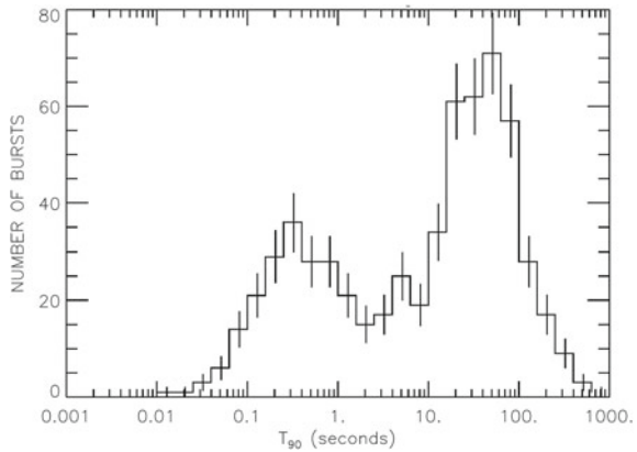
Fig. 10.19 Time distribution of GRBs detected by the BATSE satellite as a function of the time T_{90} during which 90 % of the photons are detected. It is easy to see “short” and “long” GRBs. Credit: NASA
