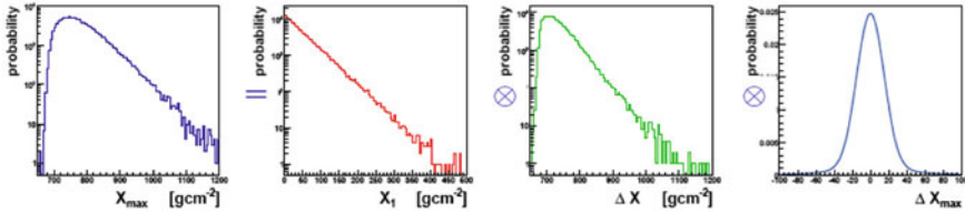
Fig. 10.4 Ingredients of the X_{\max} distribution. Adapted from the Ph.D. thesis of R. Ulrich: “Measurement of the proton–air cross section using hybrid data of the Pierre Auger Observatory,” http://bibliothek.fzk.de/zb/berichte/FZKA7389.pdf
