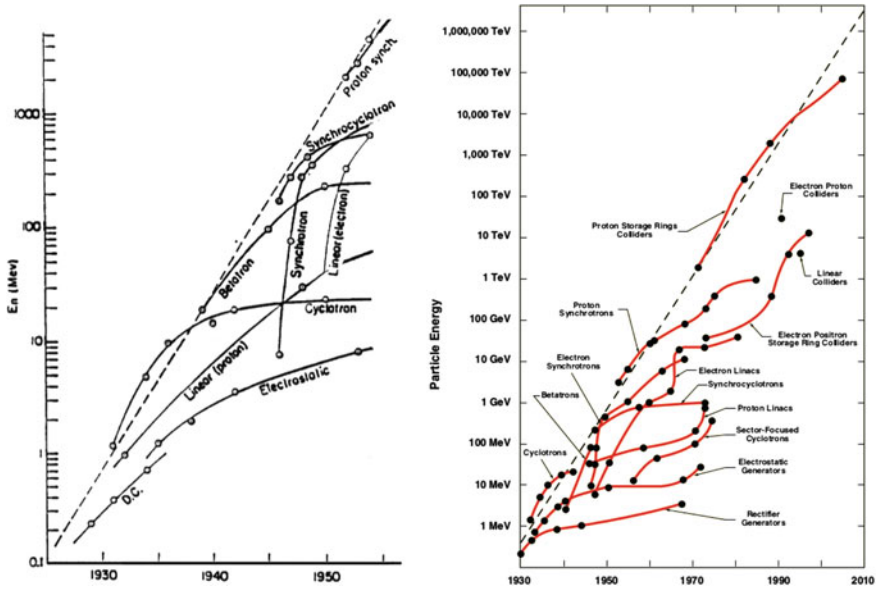
Fig. 5.1 The Livingston plot, representing the maximum energies attained by accelerators as a function of the year: original ( left ) and updated ( right ). For colliders, energies are translated into the laboratory system. Original figures from M.S. Livingston & J.P. Blewett, “Particle Accelerators,” MacGraw Hill 1962; A. Chao et al. “2001 Snowmass Accelerator R&D Report,” eConf C010630 (2001) MT100
