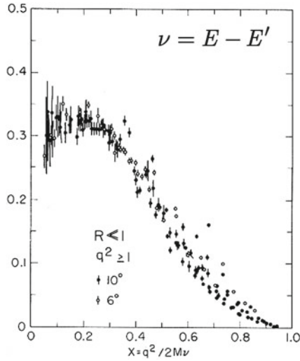
Fig. 5.20 \nu W_2 scaling: measurements at different scattered energies and angles. Source W.B. Atwood, “Lepton Nucleon Scattering,” Proc. 1979 SLAC Summer Institute (SLAC-R-224)
