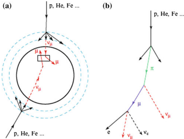
Fig. 9.8 The interaction of cosmic rays in the upper atmosphere give rise to particle showers comprising neutrinos ( right picture ), which originate from a 10–20 km thick atmospheric layer. A large volume detector placed underground, like Super-K, is used to detect them; downward-going neutrinos traveled only few tens of kilometers and had no “space” to oscillate, while upward-going neutrinos have traveled about 10,000km and have likely oscillated. The detector ( left picture ) can distinguish between electron neutrinos and muon neutrinos: secondary muons are likely to escape the detector (non-contained or partially contained events), while secondary electrons formed by neutrino electrons interacting in the detector are likely to be absorbed (fully contained events). In the case of fully contained events the electron ring is “fuzzier” than the muon ring. From Braibant, Giacomelli and Spurio, “Particles and fundamental interactions,” Springer 2014
