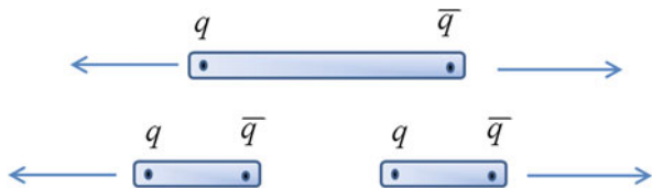
Fig. 5.16 Hadronization: the string mechanism
