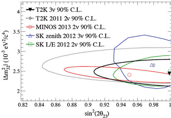
Fig. 9.14 The (|\Delta m^2_{23}|, \sin^2(2\theta_{23})) 90% CL allowed regions. From K. Abe et al. (T2K Collab.), Phys. Rev. Lett. 111 (2013) 211803
