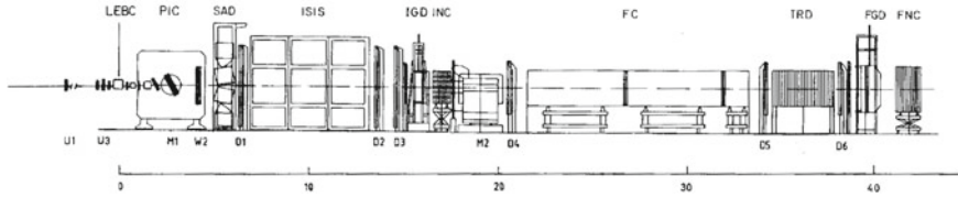
Fig. 4.26 A configuration of the European Hybrid Spectrometer (a fixed target detector at the CERN Super-proton Synchrotron). From M. Aguilar-Benitez et al., “The European hybrid spectrometer,” Nucl. Instr. Methods 258 (1987) 26
