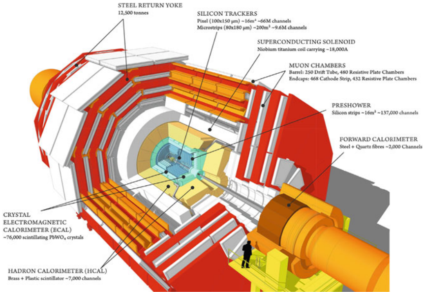
Fig. 4.31 The CMS detector at LHC (Source CERN)
