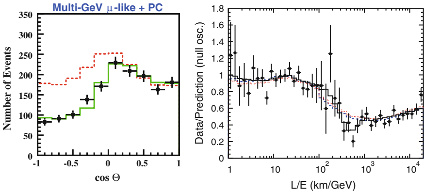
Fig. 9.9 Left Zenith angle distribution of the muon neutrinos in SK. The observed number of upward-going neutrinos was roughly half of the predictions. Right Survival probability of \nu_\mu in function of L/E . Black dots show the observations and the lines shows the prediction based on neutrino oscillation. Data show a dip around L/E \simeq 500 km/GeV. The prediction of two-flavor neutrino oscillations agrees well with the position of the dip. From http://www-sk.icrr.u-tokyo.ac.jp/sk/physics/atmnu-e.html and The Super-Kamiokande Collaboration, Y. Ashie et al., “Evidence for an Oscillatory Signature in Atmospheric Neutrino Oscillations,” Phys. Rev. Lett. 93 (2004) 101801 (color in Online)
