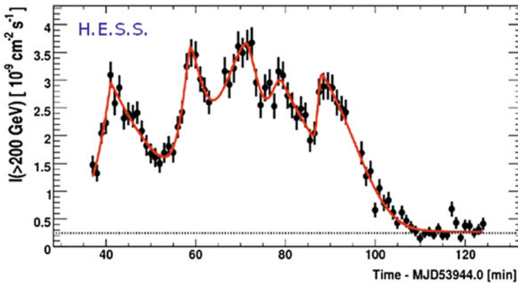
Fig. 10.17 Variability in the very-high-energy emission of the blazar PKS 2155-304. The dotted horizontal line indicates the flux from the Crab Nebula (from the H.E.S.S. experiment, http://www.mpi-hd.mpg.de/hfm/HESS )
