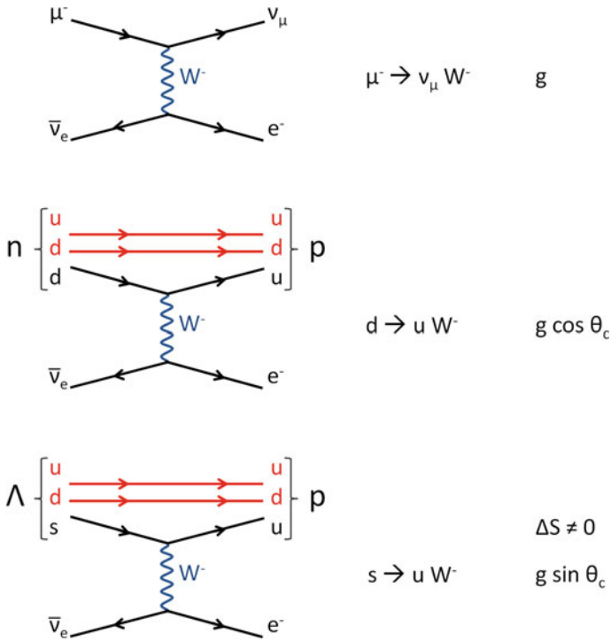
Fig. 6.38 Weak decay coupling: Leptonic ( top ), semileptonic with ( bottom ) and without ( middle ) involving strange quarks
