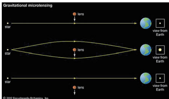
Fig. 8.32 The principle of gravitational microlensing (©Encyclopedia Britannica)
