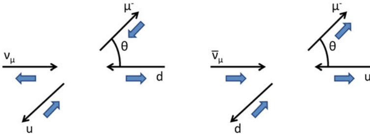
Fig. 6.23 Schematic representation of the spin alignments in \nu_\mu d \rightarrow \mu^- u (left) and in \bar{\nu}_\mu u \rightarrow \mu^- d (right) interactions
