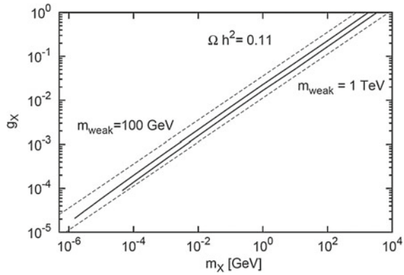
Fig. 8.27 g_\chi as function of m_\chi which satisfy the present relation (from http://physicslearning2.colorado.edu/tasi/tasi_2011/videos/Feng/lecture3/feng-lecture3.pdf )
