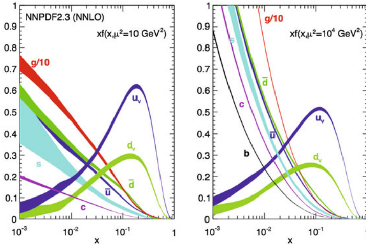
Fig. 5.25 Parton distribution functions at Q^2 = 10\text{GeV}^2 (left) and Q^2 = 10000\text{ GeV}^2 (right). The gluon and sea distributions are scaled down by a factor of 10. The experimental, model, and parameterization uncertainties are shown. From K.A. Olive et al. (Particle Data Group), Chin. Phys. C 38 (2014) 090001
