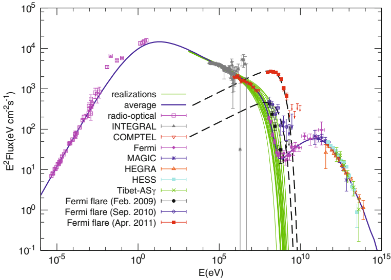
Fig. 10.16 Spectral energy distribution of the Crab Nebula (data from radio-optical up to 100 TeV). From Yuan, Yin et al., arXiv:1109.0075
