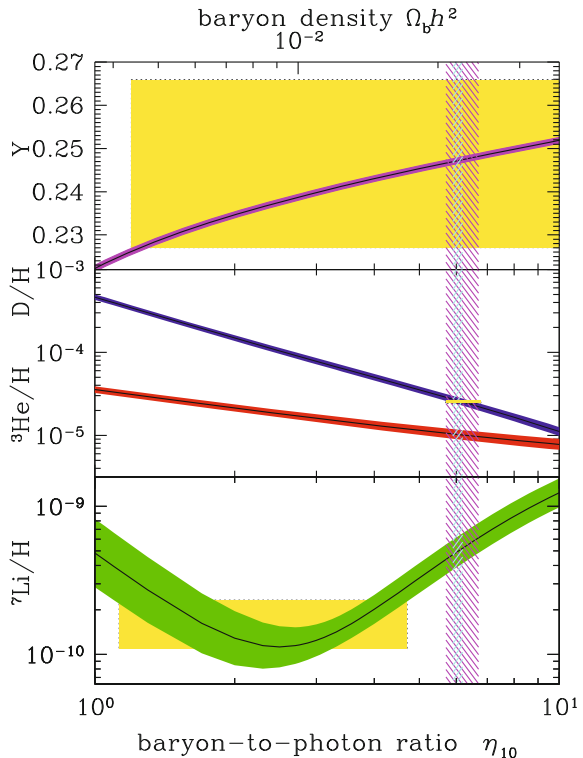
Fig. 8.11 The observed and predicted abundances of ^4\text{He} , D, ^3\text{He} , and ^7\text{Li} . Small (large) boxes represent the measurements within 2 sigma statistical (statistical and systematic) errors. The narrow vertical band represents the constraints on \eta (expressed in units of 10^{10} from the CMB power spectrum analysis while the wider is the best fit to experimental data). From K.A. Olive et al. (Particle Data Group), Chin. Phys. C 38 (2014) 090001
