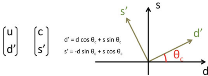
Fig. 6.42 The two orthogonal combinations of the quarks s and d in the d' and s' states
