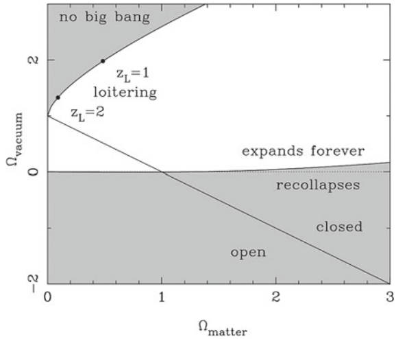
Fig. 8.24 Different scenarios for the expansion of the Universe. The Hubble constant was fixed to H_0 = 70 (km/s)/Mpc. From J.A. Peacock, “Cosmological Physics”, Cambridge University press 1998
