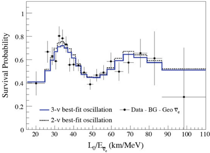
Fig. 9.6 The \bar{\nu}_e survival probability as a function of L/E observed in the KamLAND experiment. Figure from A. Gando et al. (KamLAND Collab.), Phys. Rev. D83 (2011) 052002
