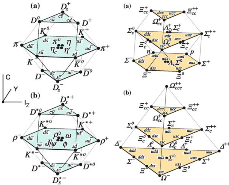
Fig. 5.15 Left The 16-plets for the pseudo-scalar (a) and vector (b) mesons made of the u, d, s , and c quarks as a function of isospin I_3 , charm C , and hypercharge Y = B + S + C . The nonets of light mesons occupy the central planes to which the c\bar{c} states have been added. Right SU(4) multiplets of baryons made of u, d, s , and c quarks: (a) The 20-plets including an SU(3) octet; (b) The 20-plets with an SU(3) decuplet. From K.A. Olive et al. (Particle Data Group), Chin. Phys. C 38 (2014) 090001
