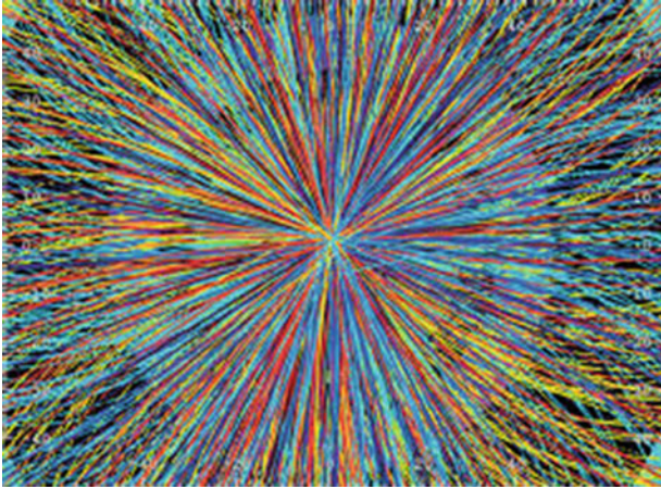
Fig. 6.73 First lead-lead event recorded by ALICE detector at LHC at center-of-mass energy per nucleon of 2.76 TeV. Thousands of charged particles were recorded by the time-projection chamber. Source CERN
