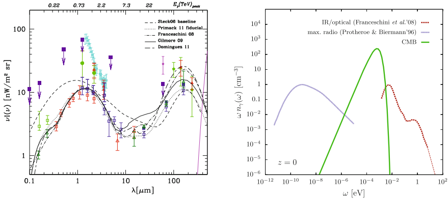
Fig. 10.48 Left Spectral energy distribution of the EBL as a function of the wavelength. Open symbols correspond to lower limits from galaxy counts while filled symbols correspond to direct estimates. The curves show a sample of different recent EBL models, as labeled. On the upper axis the TeV energy corresponding to the peak of the \gamma\gamma cross section is plotted. From L. Costamante, IJMPD 22 (2013) 1330025. Right A summary of our knowledge about the density of background photons in intergalactic space, from the radio region to the CMB, to the infrared/optical/ultraviolet region. Reference: M. Ahlers et al., Astroph. Phys. 34 (2010) 106
