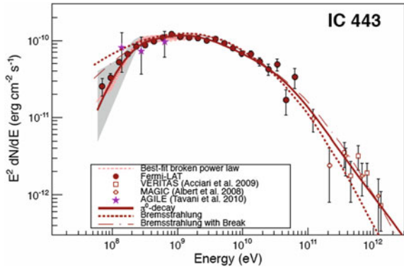
Fig. 10.40 Spectral energy distribution of photons emitted by the SNR IC443. The fit requires on top of photons coming from a leptonic acceleration mechanism also photons from \pi^0 decay. Credit: Fermi-LAT Collaboration (M. Ackermann et al.), Science 339 (2013) 807
