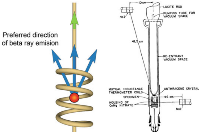
Fig. 6.19 Conceptual ( left ) and schematic diagram ( right ) of the experimental apparatus used by Wu et al. (1957) to detect the violation of the parity symmetry in \beta decay. The left plot comes from Wikimedia commons; the right plot from the original article by Wu et al., Physical Review 105 (1957) 1413
