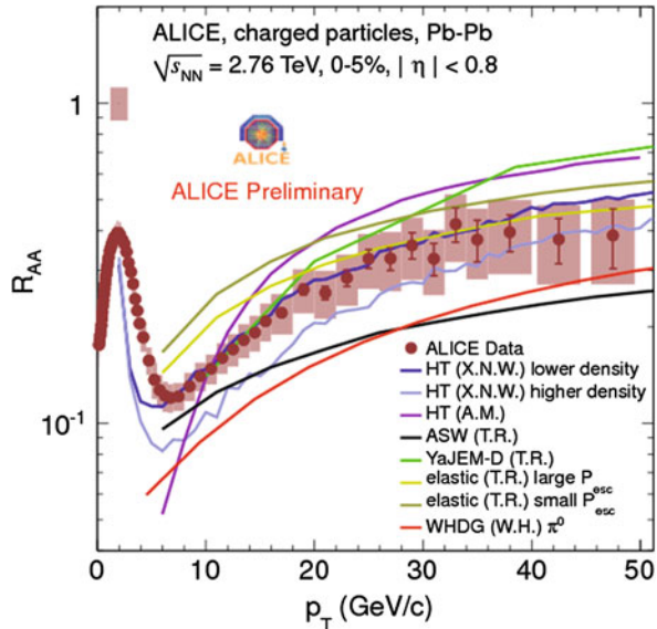
Fig. 6.76 The nuclear modification factor R_{AA} as a function of P_T , measured by ALICE experiment at LHC at center-of-mass energy per nucleon of 2.76 TeV, compared to different models. From J. Otwinowski, “High- p_{\perp} processes measured with ALICE at the LHC”, arXiv:1301.5285
