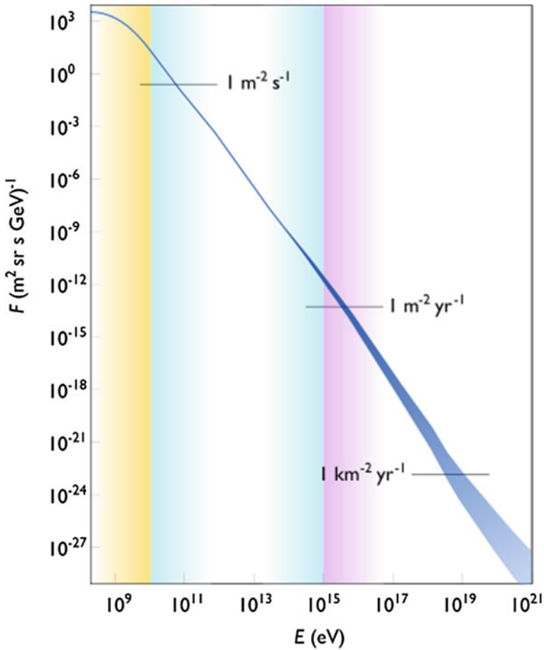
Fig. 1.8 The energy spectrum (number of incident particles per unit of energy, per second, per unit area, and per unit of solid angle) of the primary cosmic rays. The vertical band on the left indicates the energy region in which the emission from the Sun is supposed to be dominant; the central band the region in which most of the emission is presumably of galactic origin; the band on the right the region of extragalactic origin. By Sven Lafebre (own work) [GFDL http://www.gnu.org/copyleft/fdl.html ], via Wikimedia Commons.
