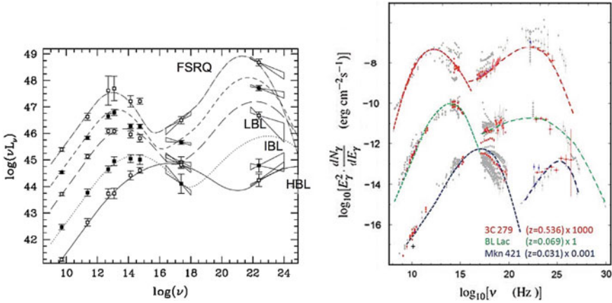
Fig. 10.37 Left The blazar sequence. From G. Fossati et al., Mon. Not. Roy. Astron. Soc. 299 (1998) 433. Right The SED of three different AGN at different distance from the Earth and belonging to different subclasses. To improve the visibility of the spectra, the contents of the farthest (3C 279) have been multiplied by a factor 1000, while that of the nearest (Mrk 421) by a factor 0.001. The dashed lines represent the best fit to the data assuming leptonic production. From D. Donato et al., Astron. Astrophys. 375 (2001) 739
