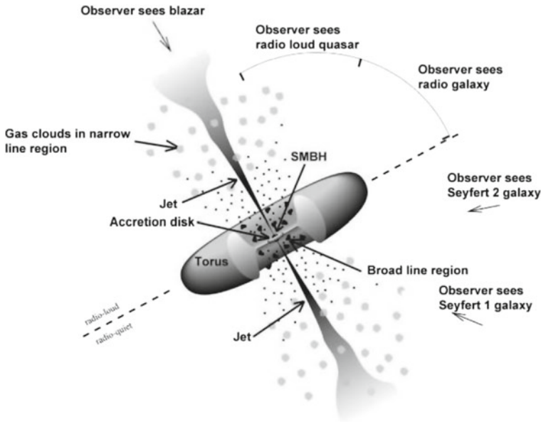
Fig. 10.36 Schematic diagram for the emission by an AGN. In the “unified model” of AGN, all share a common structure and only appear different to observers because of the angle at which they are viewed. From http://www.astro-photography.net , adapted
