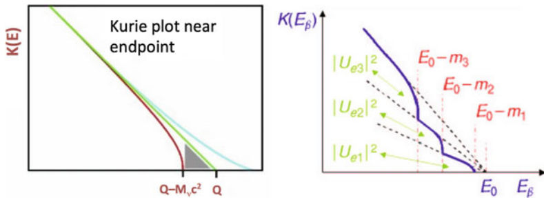
Fig. 9.17 Left Kurie plot. The green line represents the ideal case for m_{\nu_e} = 0 , the red line the ideal case for m_{\nu_e} \neq 0 and the blue line the real case where a finite detector resolution introduces a smearing at the endpoint. Right Detail of the endpoint in case of a mixing scenario with three non-degenerated mass eigenvalues. Credit: Andrea Giuliani, Review of Neutrino Mass Measurements , Quark-Lepton conference Prague, 2005 (Color in online)
