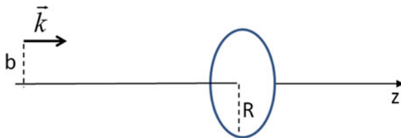
Fig. 6.69 Impact parameter definition in the scattering of particle with momentum \vec{k} over a target region with radius R
