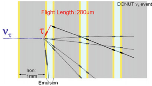
Fig. 5.31 Tau-neutrino event in DONUT. A tau-neutrino produces several charged particles. Among them a tau particle, which decays to another charged particle with missing energy (at least one neutrino). From K. Kodama et al., DONUT Collaboration, “Observation of tau neutrino interactions,” Phys. Lett. B 504 (2001) 218
