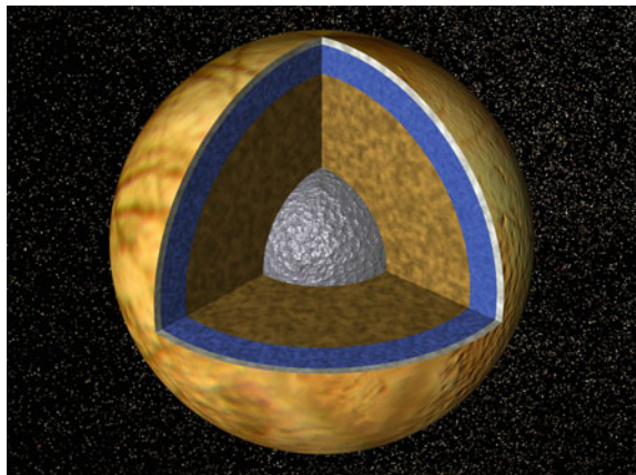
Fig. 11.7 Hypothetical structure of Europa: from outside in, we find the iced crust, the ocean, the rocky mantle, and the nuclear iron core. From NASA/Galileo Project and the University of Arizona
