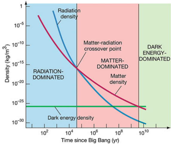
Fig. 8.23 The different ages the Universe passed through since the Big Bang (from http://scienceblogs.com/startswithabang/files/2013/06/AT_7e_Figure_27_01.jpeg , ©2011 Pearson education, Pearson Addison Wesley)
