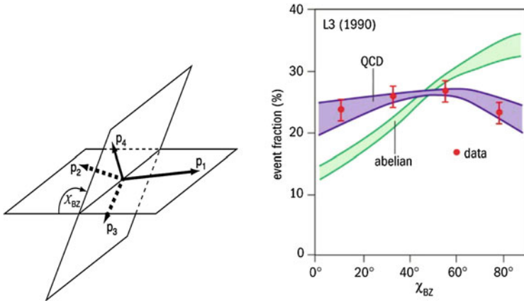
Fig. 7.15 Left Definition of the Bengtsson–Zerwas angle in 4-jet events. From P.N. Burrows, SLAC-PUB-7434, March 1997. Right Distribution for the data, compared with the predictions for QCD and for an Abelian theory. The experimental distribution is compatible with QCD, but it cannot be reproduced by an Abelian field theory of the strong interactions without gauge boson self-coupling. From CERN Courier, May 2004
