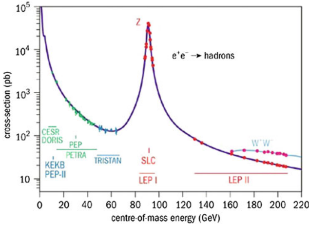
Fig. 7.9 Evolution of the hadronic cross section \sigma(e^+e^- \rightarrow \text{hadrons}) with energy, compared with the predictions of the SM
