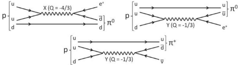
Fig. 7.28 Some mechanisms for proton decay in the SU(5) GUT
