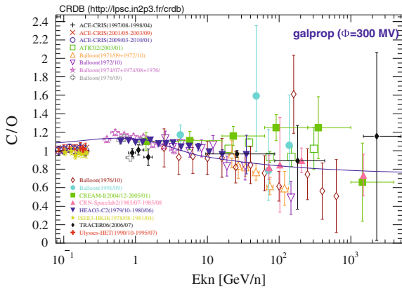
Fig. 10.47 The C/O ratio (primary/primary) as a function of the energy. The data points were made using the Cosmic Ray database reference: Maurin, Melot, Taillet, A&A 569, A32 (2014) [arXiv:1302.5525]. The full lines are fits using Galprop model standard parameters. (reference: http://galprop.stanford.edu )
