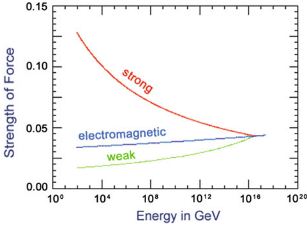
Fig. 7.26 Artistic scheme (qualitative) of the unification of the interaction forces
