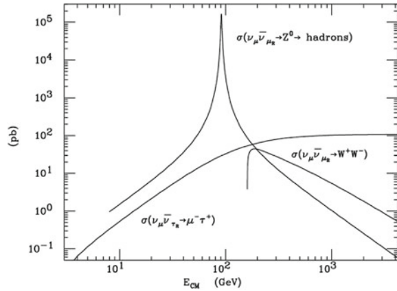
Fig. 10.52 \nu\nu_c inelastic cross section as a function of the interaction center of mass. From D. Fargion and B. Mele, arXiv:astro-ph/9902024
