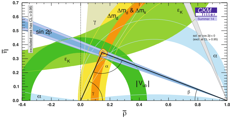
Fig. 6.49 Unitarity triangle and global CKM fit in the plane (\bar{\rho}, \bar{\eta}) . From CKMfitter Group (J. Charles et al.), Eur. Phys. J. C41 (2005) 1, updated results and plots available at http://ckmfitter.in2p3.fr
