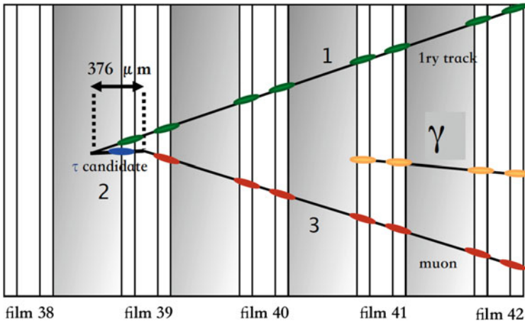
Fig. 9.15 One of the three tau antineutrino candidate events observed by OPERA. From http://operaweb.lngs.infn.it/
