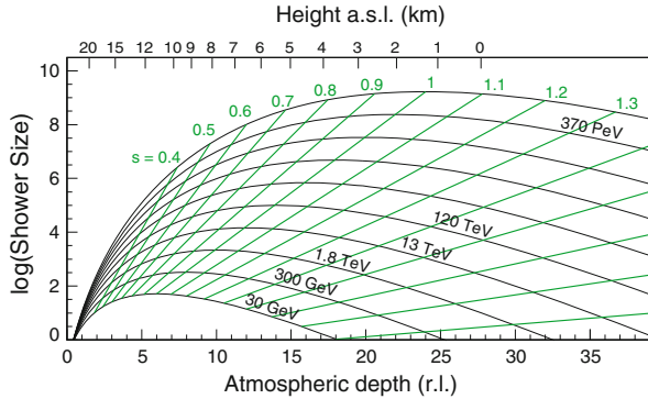
Fig. 4.35 Longitudinal shower development from a photon-initiated cascade. The parameter s describes the shower age. Credit: R.M. Wagner, dissertation, MPI Munich 2007; adapted from reference [F4.1] in the “Further reading”
