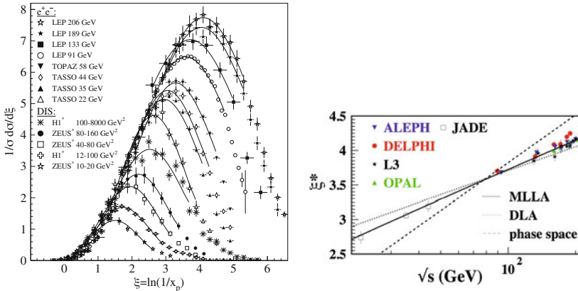
Fig. 7.19 Left Center-of-mass energy dependence of the spectra of charged hadrons as a function of \xi = -\ln x ; x = 2E_h/E_{CM} . From K.A. Olive et al. (Particle Data Group), Chin. Phys. C 38 (2014) 090001. Right Energy dependence of the maximum of the \xi distribution, \xi^*
