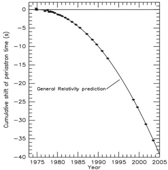
Fig. 10.25 Observed accumulated shifts of the times of periastron in the PSR 1913+16 compared with the general relativity prediction from gravitational radiation (from Joseph H. Taylor Jr.—©The Nobel Foundation 1993)
