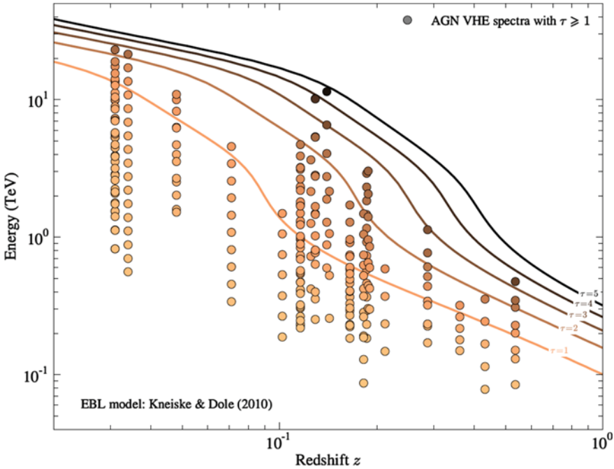
Fig. 10.60 For each individual spectral measurement including points at \tau > 1 , the corresponding value of z and E are marked in this diagram. The iso-contours for \tau = 1, 2, 3, 4 calculated using a minimum EBL model are overlaid. From D. Horns, M. Meyer, JCAP 1202 (2012) 033
