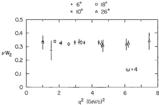
Fig. 5.21 \nu W_2 scaling for the proton: measurements at fixed x and at different Q^2 . Source J.I. Friedman and H.W. Kendall, Annual Rev. Nucl. Science 22 (1972) 203
