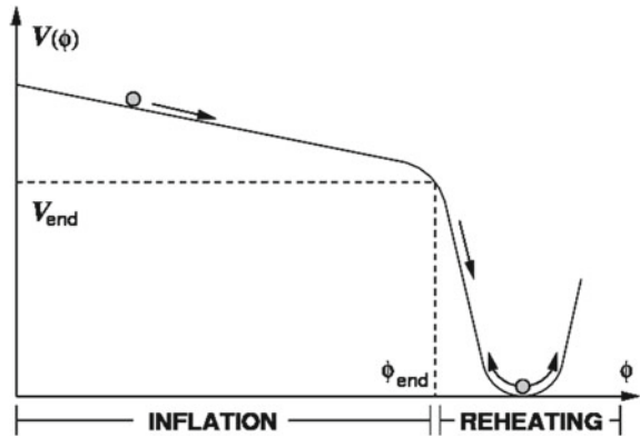
Fig. 8.28 An example of an inflaton potential. (from K. Dimopoulos, J. Phys.: Conf. Ser. 283 012010 (doi:10.1088/1742-6596/283/1/012010))
