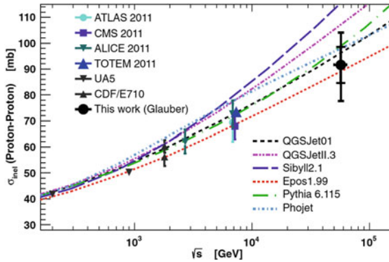
Fig. 10.56 Comparison of the inelastic proton–proton cross section derived by the Pierre Auger Observatory in the energy interval 10^{18} – 10^{18.5} eV to phenomenological model predictions and results from accelerator experiments at lower energies. From P. Abreu et al., Phys. Rev. Lett. 109 (2012) 062002
