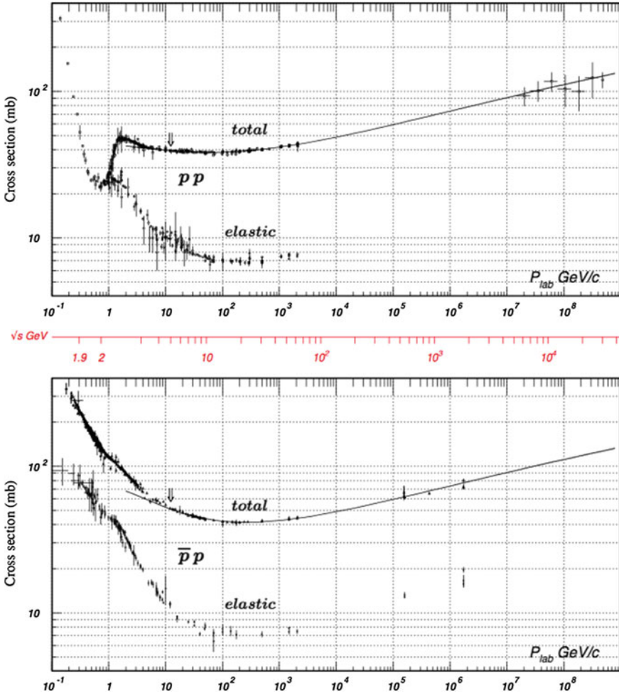
Fig. 2.7 Total and elastic cross sections for pp and \bar{p}p collisions as a function of laboratory beam momentum and total center-of-mass energy. From the Review of Particle Physics, K.A. Olive et al. (Particle Data Group), Chin. Phys. C 38 (2014) 090001
