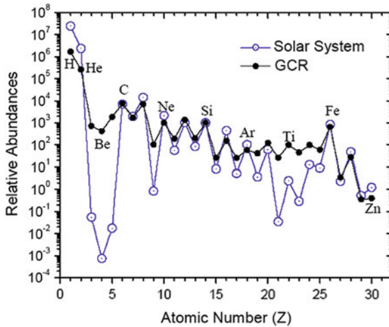
Fig. 10.6 Relative abundance of the main hadronic components present in the cosmic rays arriving at Earth and in the Solar System. Both are normalized to the abundance of Si = 10^3 , and the relevant energy range is a few hundreds MeV/nucleon. Credit: ACE archives, http://www.srl.caltech.edu/ACE
