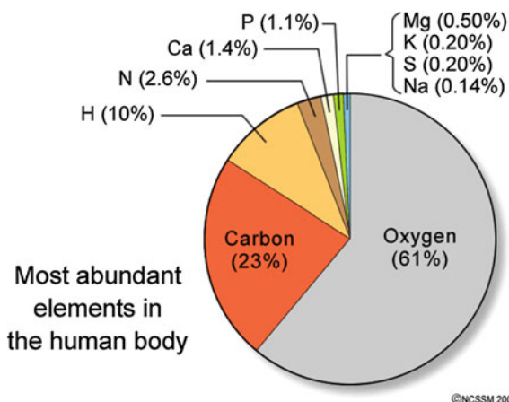
Fig. 11.2 Most abundant elements (in weight) that form the human body. From http://www.dlt.ncssm.edu/tiger/chem1.htm
