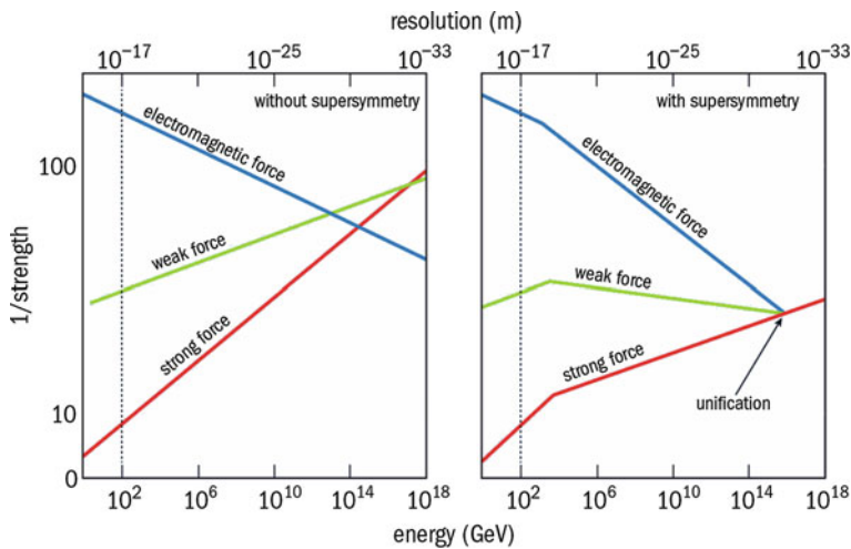
Fig. 7.29 The interaction couplings \alpha_i = g_i^2/4\pi\hbar c fail to meet at a single point when they are extrapolated to high energies in the standard model, as well as in SU(5) GUTs. Minimal SUSY SU(5) model ( right ) does cause the couplings to meet in a point. While there are other ways to accommodate the data, this straightforward, unforced fit is encouraging for the idea of supersymmetric grand unification (Adapted from S. James Gates, Jr., http://live.iop-pp01.agh.sleek.net/2014/09/25/sticking-with-susy/ ; adapted from Ugo Amaldi, CERN)
