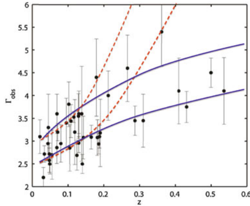
Fig. 10.61 The observed values of the spectral index for all blazars detected in VHE; superimposed is the predicted behavior of the observed spectral index from a source at constant intrinsic spectral index within two different scenarios. In the first one (area between the two dotted lines) \Gamma is computed from EBL absorption; in the second (area between the two solid lines) it is evaluated including also the photon-ALP oscillation. Original from A. de Angelis et al., Mon. Not. R. Astron. Soc. 394 (2009) L21; updated
