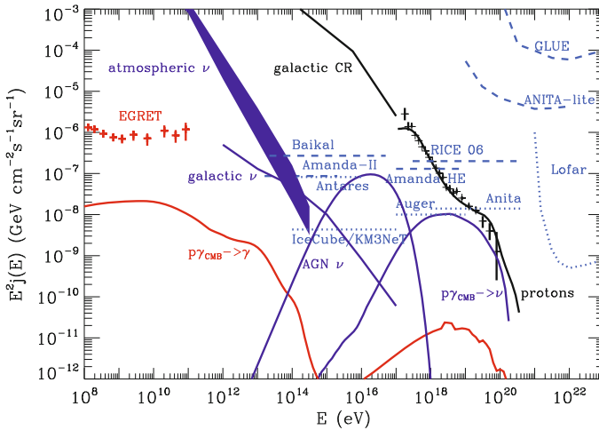
Fig. 10.42 A theoretical model of high-energy neutrino sources. The figure includes experimental data, limits, and projected sensitivities to existing and planned telescopes. Figure from G. Sigl, arXiv:0612240
