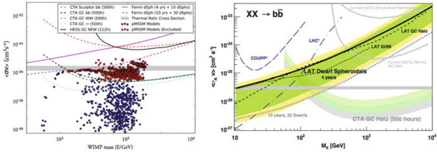
Fig. 10.58 Comparison of current ( solid lines ) and projected ( dashed lines ) limits on the DM annihilation interaction rate from different gamma ray searches as a function of WIMP mass. Left Expected limits for CTA are shown for WIMP annihilation compared to limits from Fermi-LAT and H.E.S.S. The points represent different choices of the parameters in SUSY. Right CTA is compared with the potential from direct detection (COUPP) and accelerator experiments (ATLAS and CMS at LHC). From S. Funk, arXiv:1310.2695
