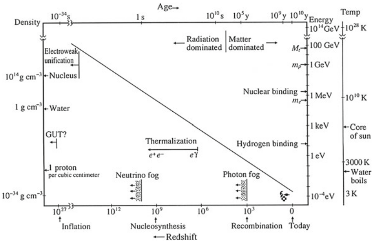
Fig. 8.30 The density, temperature, age, and redshift for the several Universe epochs. From Eric Linder, "First principles of Cosmology", Addison-Wesley 1997
