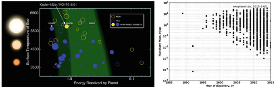
Fig. 11.10 Left discovered extrasolar planets in function of the distance from their sun, and the stellar flux. The Earth, Venus and Mars are included as a reference. Credit: NASA. Right plot of year of discovery of extrasolar planets versus their mass (normalized to Jupiter's mass). Credit: Wikimedia Commons
