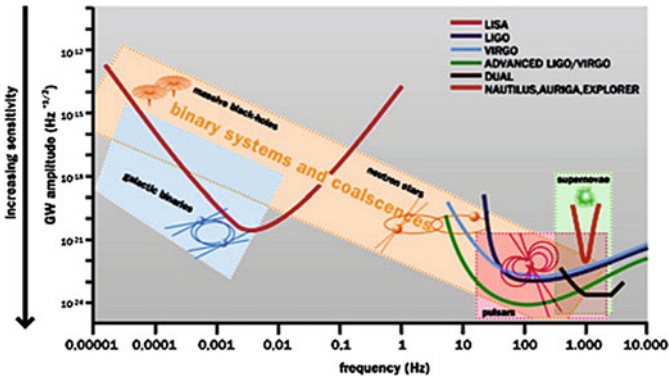
Fig. 4.63 Present and expected sensitivities of gravitational wave detectors ( http://www.aspera-eu.org/ )
