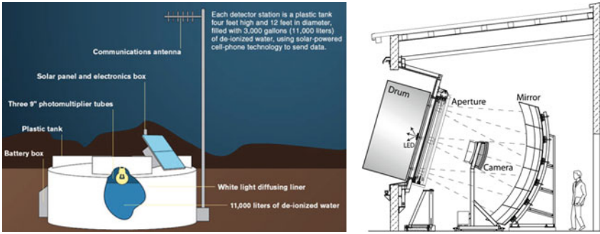
Fig. 4.44 Sketch of one of the Pierre Auger surface detectors ( left ); a fluorescence telescope ( right ). From https://www.auger.org
