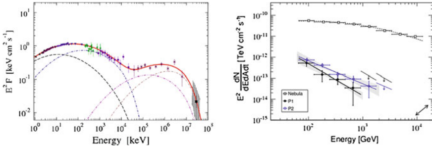
Fig. 10.35 Left Spectral energy distribution of the Crab Pulsar. Right The VHE energy emission, compared with the emission from the pulsar wind nebula powered by the pulsar itself (see later). The two periodical peaks are separated. Credits: MAGIC Collaboration
