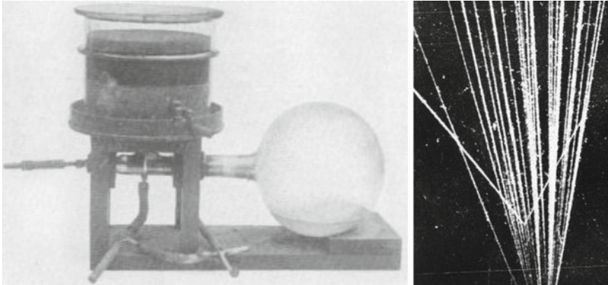
Fig. 3.8 Left A cloud chamber built by Wilson in 1911. By C.T.R. Wilson [public domain], via Wikimedia Commons. Right a picture of a collision in a cloud chamber [CC BY 4.0 http://creativecommons.org/licenses/by/4.0 ] via Wikimedia Commons
