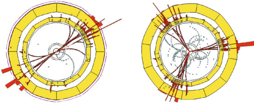
Fig. 6.61 A two-jet event ( left ) and a 3-jet event ( right ) observed by the ALEPH experiment at LEP. Source CERN
