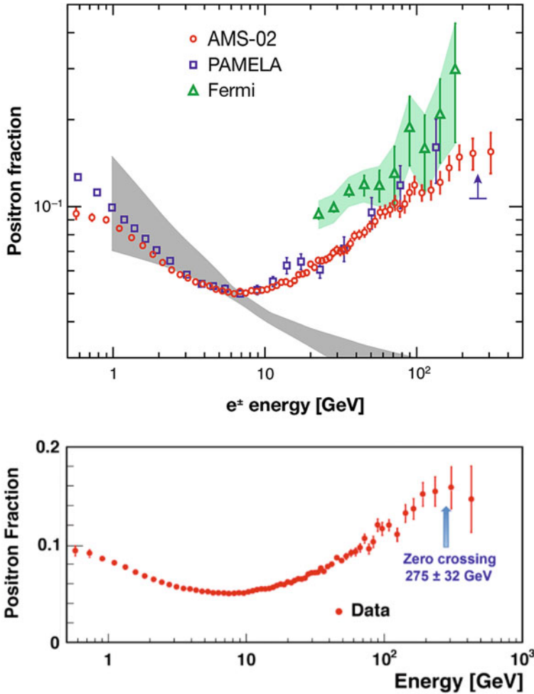
Fig. 10.10 Top The positron fraction in high-energy cosmic rays: measurement from the AMS-02, PAMELA, and Fermi-LAT satellites. The AMS measurement confirms an excess in the high-energy positron fraction, above what is expected from positrons produced in cosmic ray interactions, first observed by PAMELA (the gray band indicates the expected range in the positron fraction, which is based on standard cosmic ray models). Bottom Recently updated results by AMS-02. No sharp structures are observed, besides a hint of a maximum at (275 \pm 32) GeV
