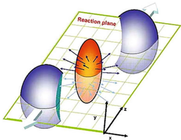
Fig. 6.74 Artistic representation of one heavy-ion collision. The reaction plane is defined by the momentum vectors of the two ions and the shape of the interaction region is due to the sharp pressure gradients. From https://www.bnl.gov/rhic/news/061907/story2.asp
