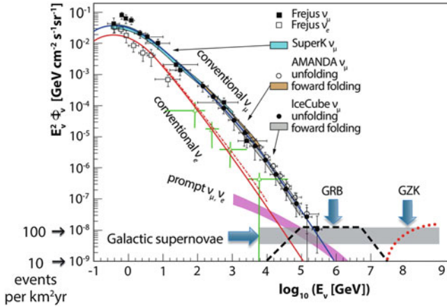
Fig. 10.22 The flux of neutrinos: experimental data. Credit: F. Halzen
