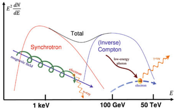
Fig. 10.31 Differential energy spectrum of photons in the SSC model
