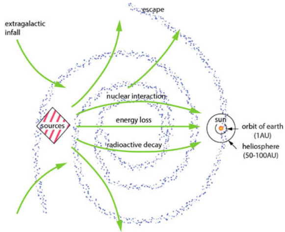
Fig. 10.44 Galactic cosmic ray propagation
