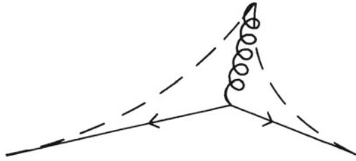
Fig. 6.56 Illustration of a qq\bar{q} system. Color conservation entails the fact that the color string goes from quarks to gluons and vice-versa rather than from quark to antiquark
