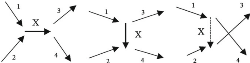
Fig. 2.17 Two-to-two particles interaction channels: left s -channel; center t -channel; right u -channel
