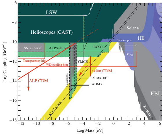
Fig. 8.33 Axion and ALP coupling to photons versus the ALP mass. Colored regions are: generic prediction for the QCD axion, which relate its mass with its coupling to photons ( yellow ), experimentally excluded regions ( dark green ), constraints from astronomical observations ( gray ) or from astrophysical or cosmological arguments ( blue ), and sensitivity of planned experiments ( light green ). Shown in red are boundaries where axions and ALPs can account for all the cold dark matter produced either thermally or nonthermally by the vacuum-realignment mechanism. Adapted from A. Ringwald, J. Phys. Conf. Ser. 485 (2014) 012013
