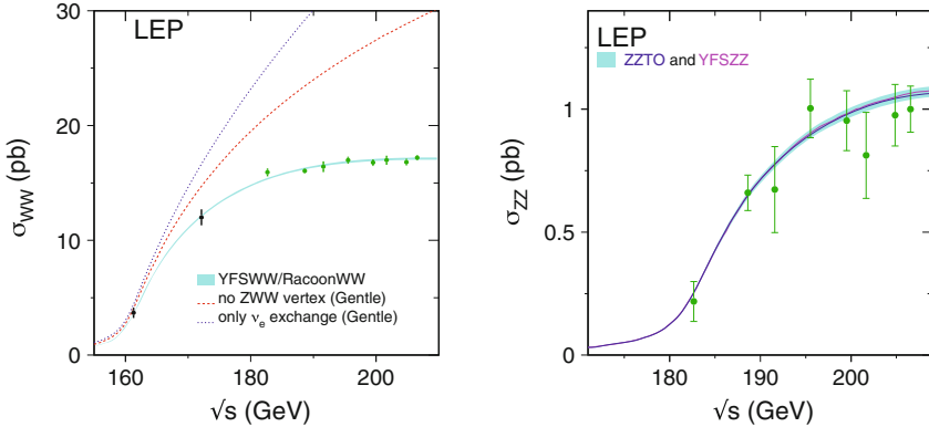
Fig. 7.13 Measured energy dependence of \sigma(e^+e^- \rightarrow W^+W^-) (left) and \sigma(e^+e^- \rightarrow ZZ) (right). The curves shown for the W -pair production cross section correspond to only the \nu_e -exchange contribution (upmost curve), \nu_e exchange plus photon exchange (middle curve), and all contributions including also the ZWW vertex (lowest curve). Only the e -exchange mechanism contributes to Z -pair production. From ALEPH, DELPHI, L3, OPAL Collaborations and the LEP Electroweak Working Group, Phys. Rept. 532 (2013)119
