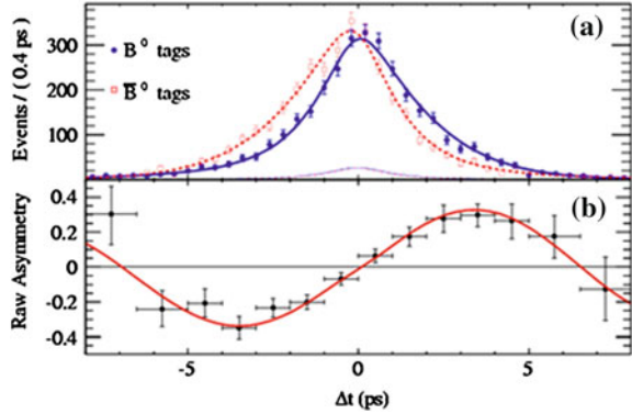
Fig. 6.47 Decay rate to J/\psi K_S as a function of time of each of the B flavor states ( top ) and the derived time asymmetry ( bottom ). From C. Chen (BaBar), Contribution to the 34th International Conference on High-Energy Physics (July 2008)
