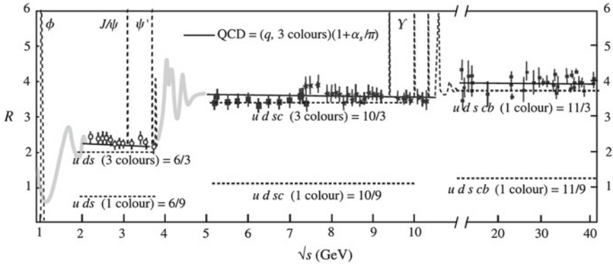
Fig. 5.27 Measurements of R(\sqrt{s}) . From [F5.2] in the “further readings”; the data are taken from K.A. Olive et al. (Particle Data Group), Chin. Phys. C 38 (2014) 090001
