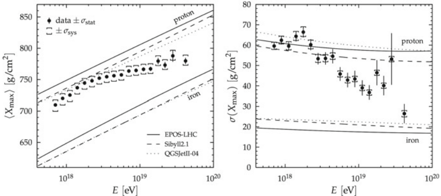
Fig. 10.57 Energy evolution of the mean ( left ) and the RMS ( right ) of the X_{\max} distributions measured by the Pierre Auger Observatory. The lines represent the expectations for pure proton and iron composition for several simulation models which take into account the data obtained at the LHC. From A. Aab et al., Phys. Rev. D90 (2014) 122005
