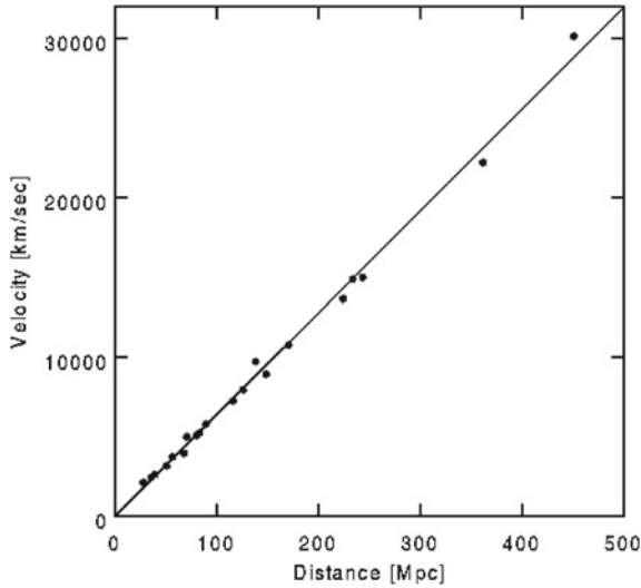
Fig. 1.5 Experimental plot of the relative velocity (in km/s) of known astrophysical objects as a function of distance from Earth (in Mpc). Several methods are used to determine the distances. Distances up to hundreds of parsecs are measured using stellar parallax (i.e., the difference between the angular positions from the Earth with a time delay of 6 months). Distances up to 50 Mpc are measured using cepheids, periodically pulsating stars for which the luminosity is related to the pulsation period (the distance can thus be inferred by comparing the intrinsic luminosity with the apparent luminosity). Finally, distances from 1 to 1000 Mpc can be measured with another type of standard candle, Type Ia supernova, a class of remnants of imploded stars. In between (from 15 to 200 Mpc), the Tully-Fisher relation, an empirical relationship between the intrinsic luminosity of a spiral galaxy and the width of its emission lines (a measure of its rotation velocity), can be used. The methods, having large superposition regions, can be cross-calibrated. The line is a Hubble-law fit to the data. From A. G. Riess, W. H. Press and R. P. Kirshner, Astrophys. J. 473 (1996) 88
