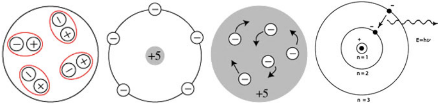
Fig. 1.1 Sketch of the atom according to atomic models by several scientists in the early twentieth century: from left to right , the Lenard model, the Nagaoka model, the Thomson model, and the Bohr model with the constraints from the Rutherford experiment. Source http://skullsinthestars.com/2008/05/27/the-gallery-of-failed-atomic-models-1903-1913/
