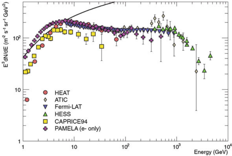
Fig. 10.9 Energy spectrum of e^+ plus e^- (except PAMELA data, for which electrons only are plotted) multiplied by E^3 . The line shows 1% of the proton spectrum. From K.A. Olive et al. (Particle Data Group), Chin. Phys. C 38 (2014) 090001
