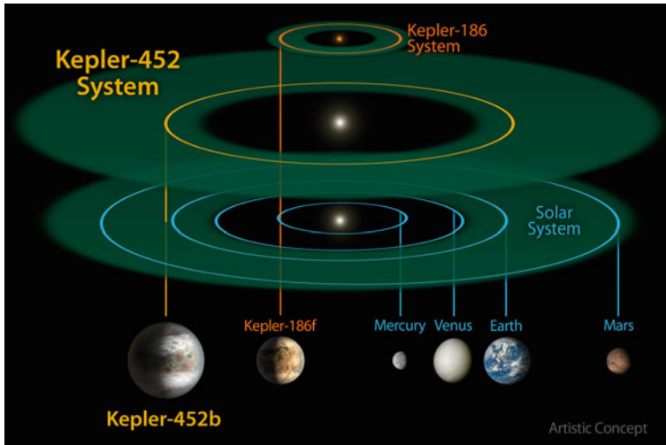
Fig. 11.11 Kepler-186f and Kepler-452b in their solar systems: comparison with the habitable zone of our Solar System. Credit: NASA
