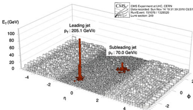
Fig. 6.75 Display of an unbalanced di-jet event recorded by the CMS experiment at the LHC in lead–lead collisions at a center-of-mass energy of 2.76 TeV per nucleon. The plot shows the sum of the electromagnetic and hadronic transverse energies as a function of the pseudorapidity and the azimuthal angle. The two identified jets are highlighted. From S. Chatrchyan et al. (CMS Collaboration), Phys. Rev. C84 (2011) 024906
