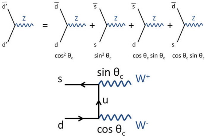
Fig. 6.39 Possible s and d quarks transitions generated by Z ( top ) and W^\pm ( bottom ) couplings (three families)
