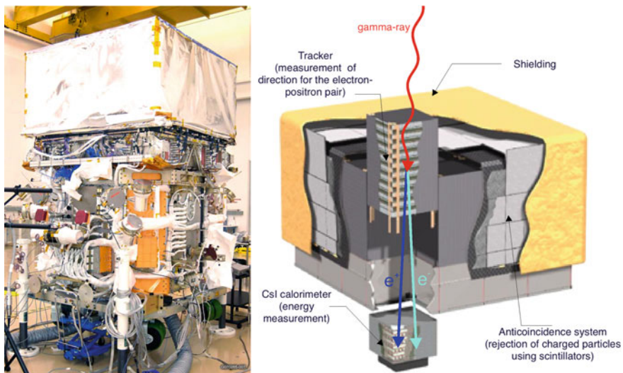
Fig. 4.48 On the left , the Fermi satellite. On the right , the layout of the Large Area Telescope (LAT), and principle of operation. Credits: NASA
