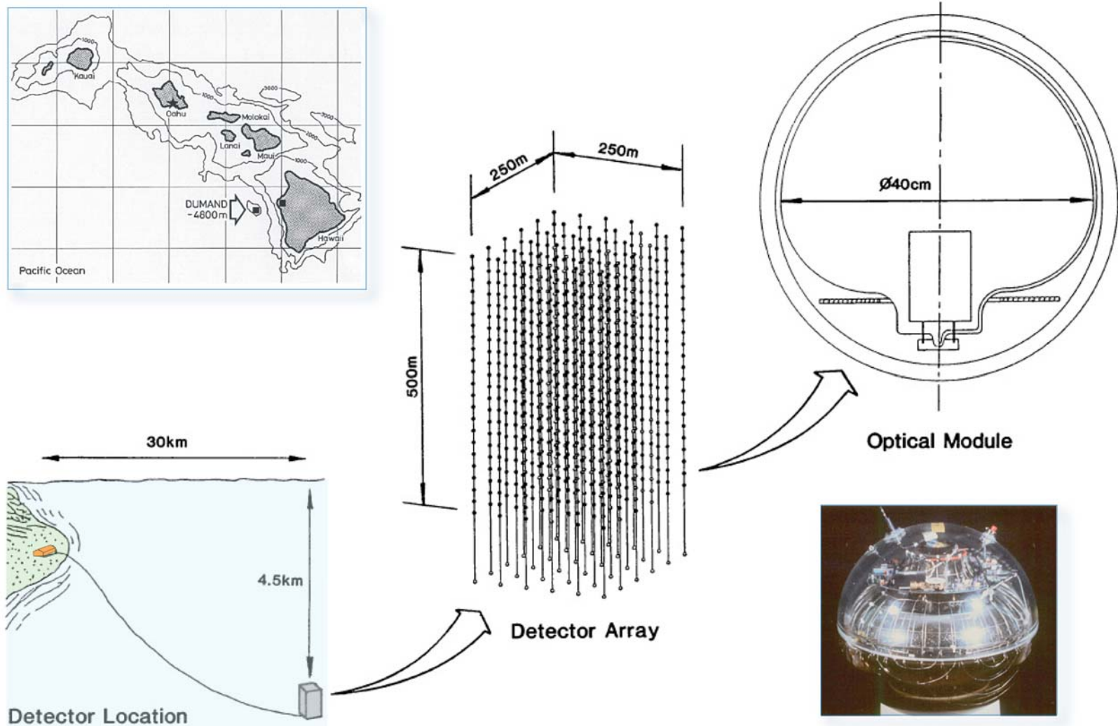
Figure 155: Proposed configuration of the DUMAND detector.
