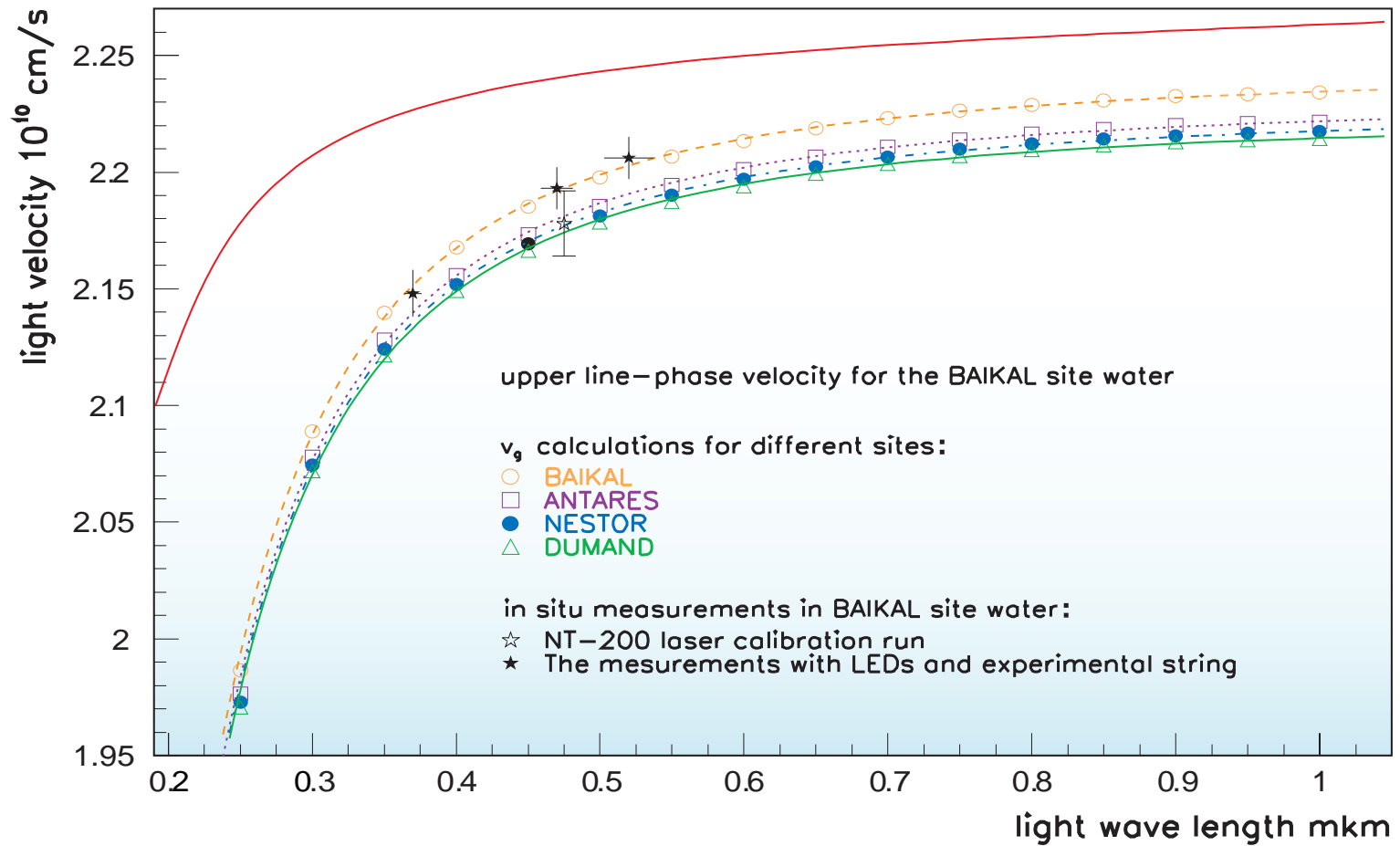
Figure 154: Light velocity vs light wavelength for several underwater neutrino telescope projects. The stars correspond to the experimental results. Other points and lines are calculated data. [From I. A. Danilchenko, "The dispersion formula and the light group velocity in a water," physics/0306020, submitted to Nucl. Instrum. Meth. A.]
