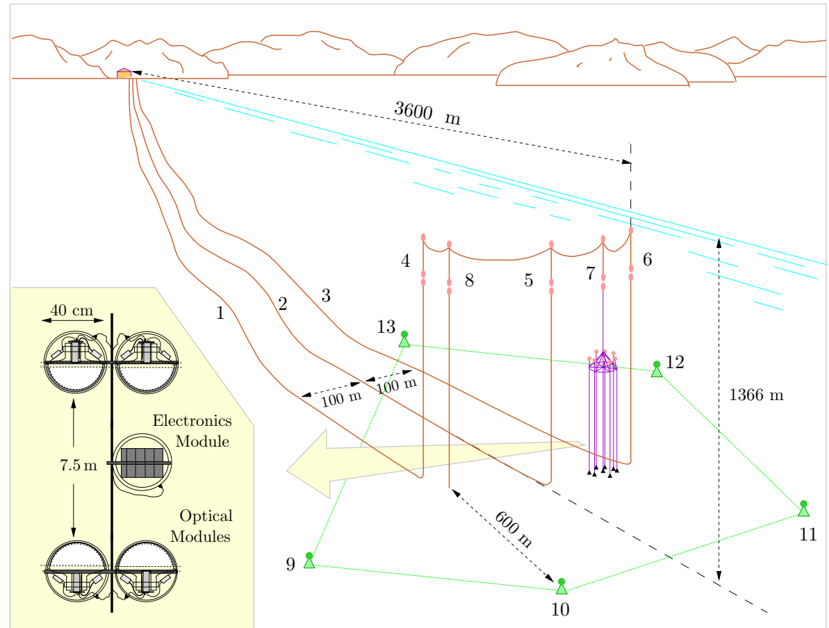
Figure 159: Overall view of the NT-200 complex in Lake Baikal. [From V. A. Balkanov et al. , "In-situ measurements of optical parameters in Lake Baikal with the help of a neutrino telescope," Appl. Opt. 33 (1999) 6818–6825 (astro-ph/9903342).]
