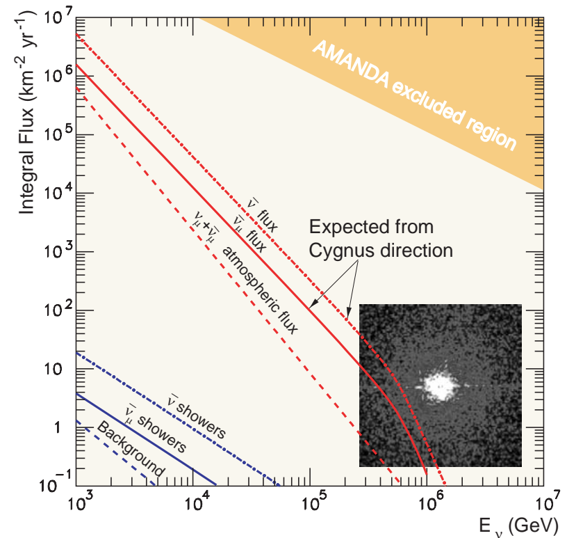
Figure 205: Antineutrino fluxes from Cygnus. The integrated AN flux is shown for an angular bin of 1^{\circ} \times 1^{\circ} . The excluded region is according to J. Ahrens, astro-ph/0309585.
