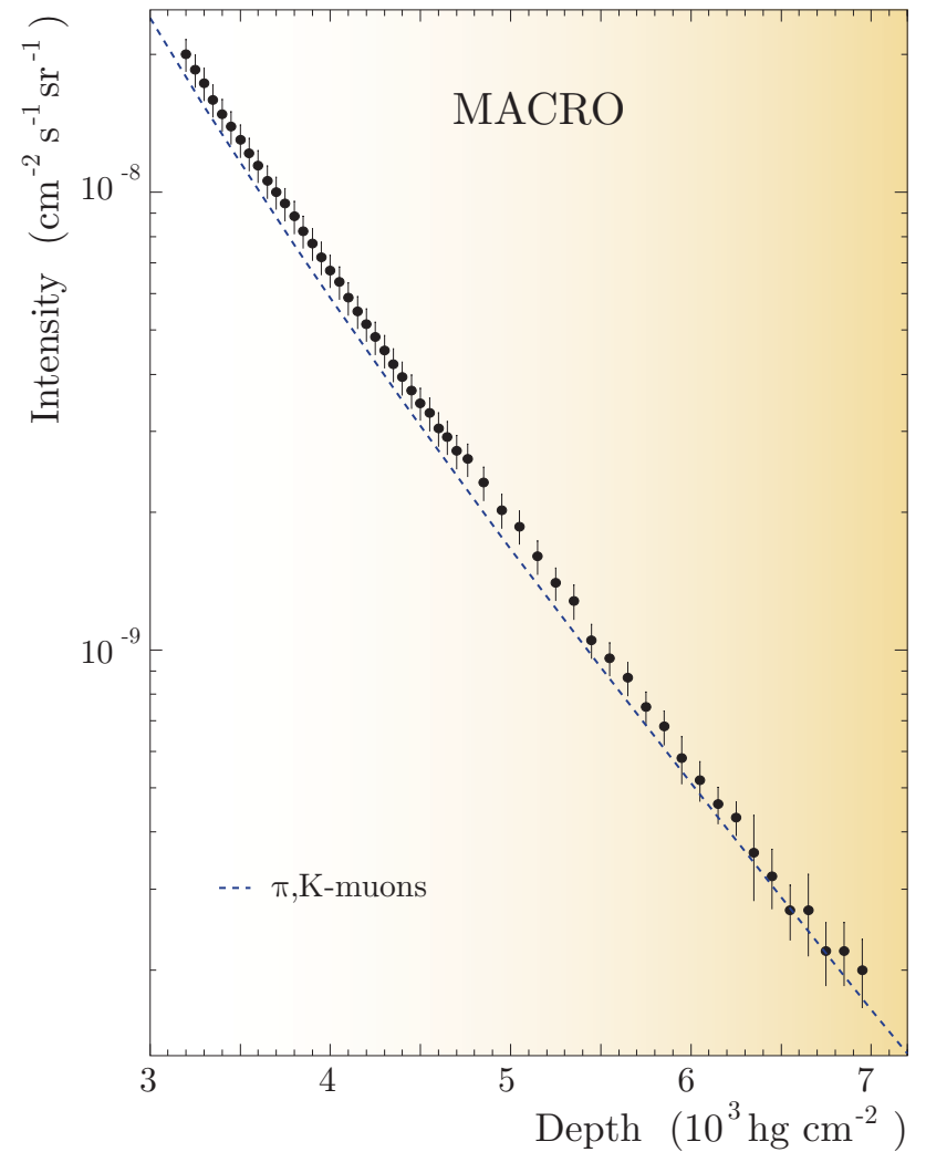
Figure 86: \mu DIR from MACRO.
