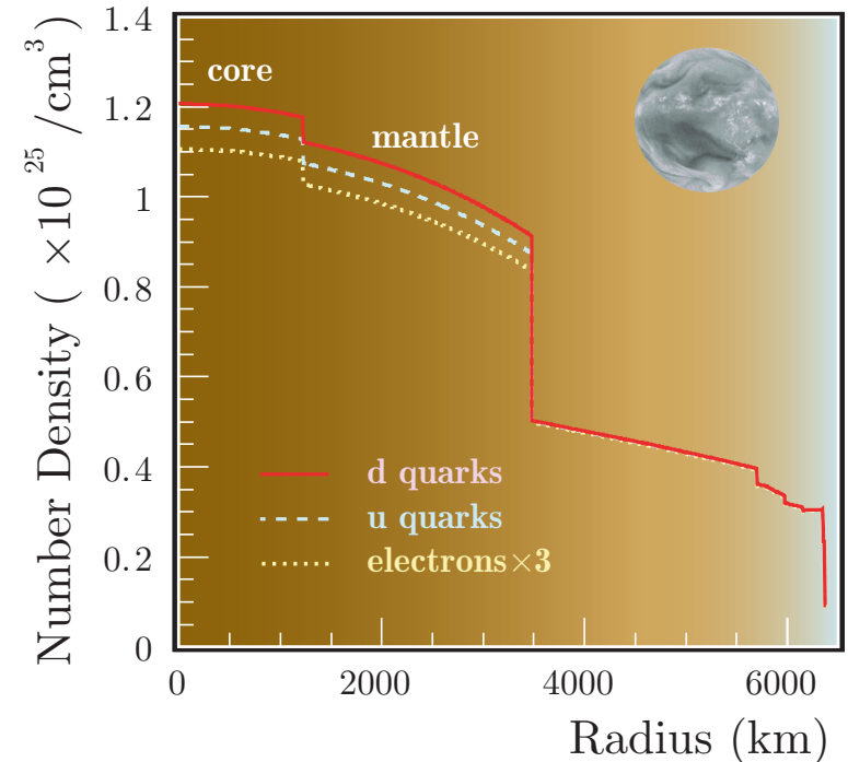
Figure 194: Estimated number densities of quarks and electrons vs distance from the center of the Earth. [From J. Kameda, Ph. D Thesis, University of Tokyo, September, 2002.]
