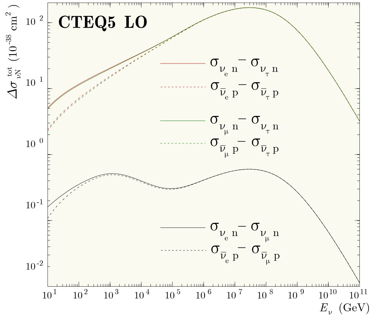
Figure 209: Differences between the total neutrino cross sections for proton and neutron targets evaluated with the CTEQ5-DIS LO PDF model.
