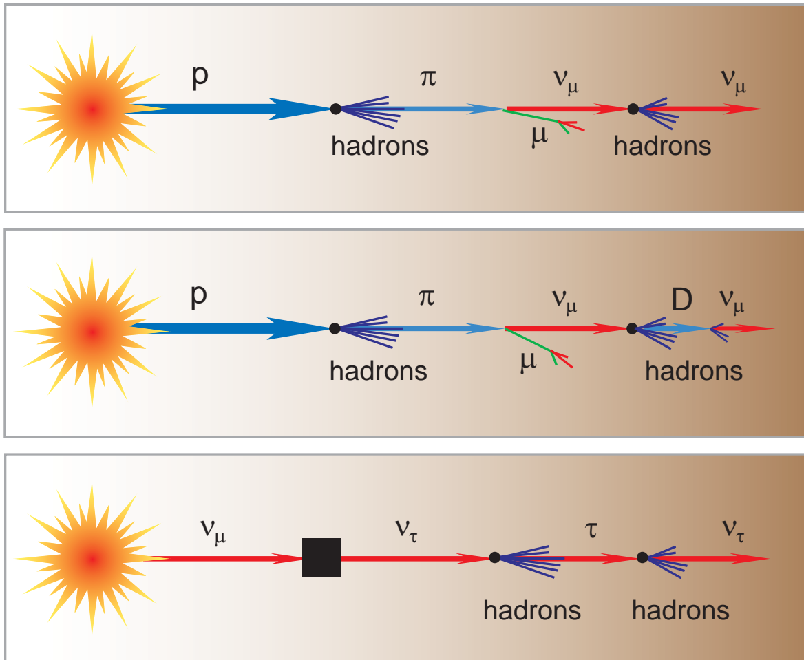
Figure 182: Primitive schemes for neutrino production, absorption and regeneration in matter.
