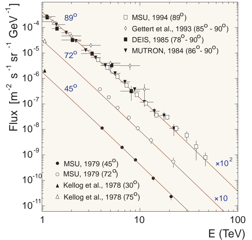
Figure 77: Differential energy spectra of muons at sea level for several zenith angles at E > 1 TeV. The data are scaled with the factors indicated on the rights over the curves. All the curves represent the conventional (\pi, K) muon contribution only.
