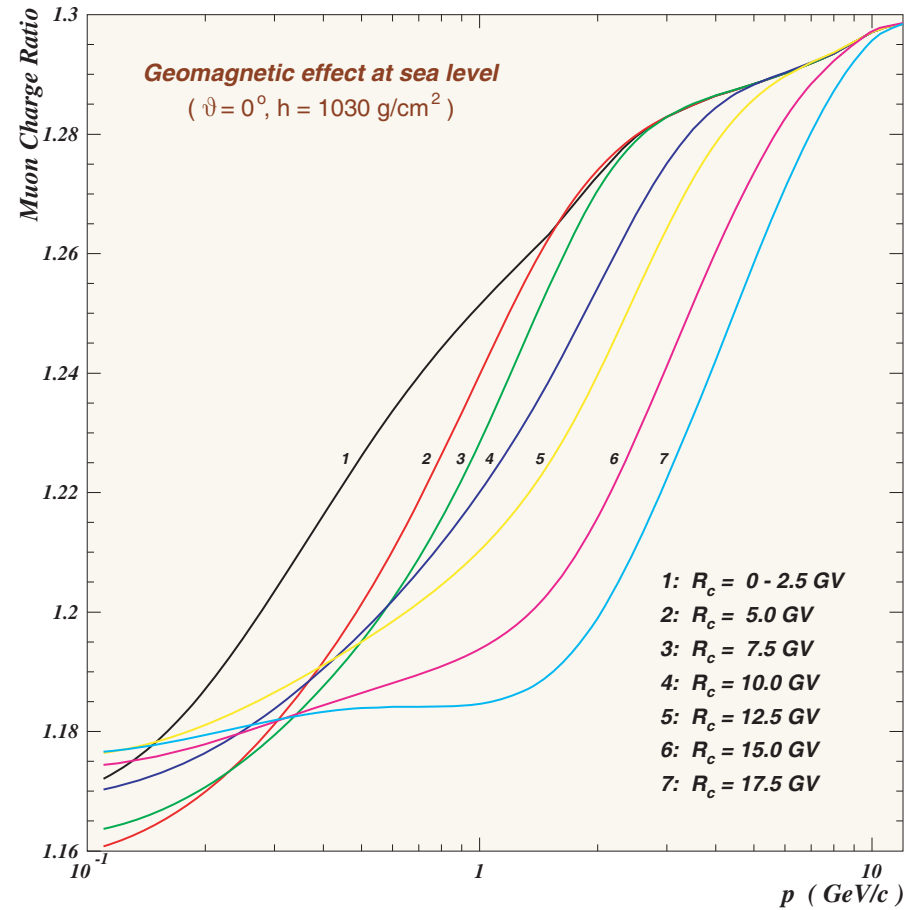
Figure 67: Muon charge ratio, \mu^+/\mu^- , at s.l. as a function of momentum calculated with CORT for several geomagnetic cutoffs R_c .
