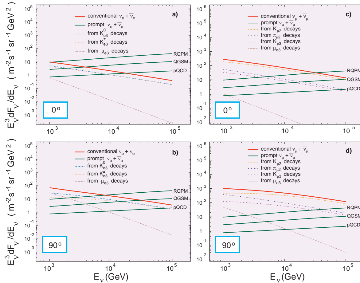
Figure 142: Separate contributions from some mechanisms of neutrino production into the total AN fluxes at \vartheta = 0^\circ and \vartheta = 90^\circ for energies 1 to 100 TeV.
