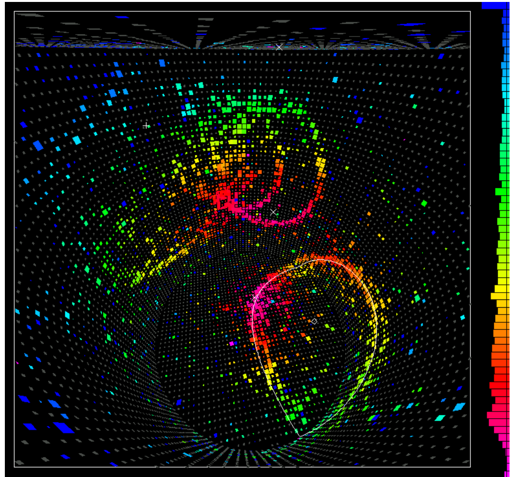
Figure 112: Through-going muon event recorded in the Super-Kamiokande detector on 30/05/1996, 17:12:56.
