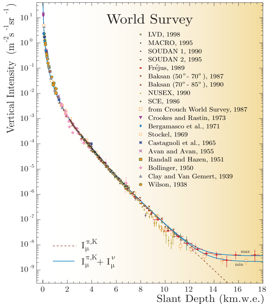
Figure 79: Muon DIR from underground data.
