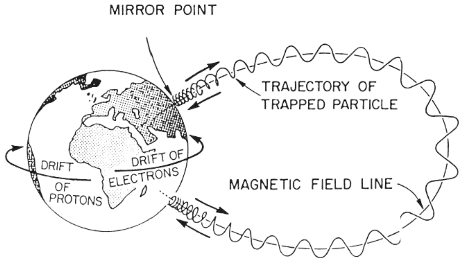
Figure 219: Mirroring of a trapped particle in the Earth's magnetic field. The dipole-like structure of the geomagnetic field provides the mechanism for a trapped population of energetic particles. [From A. P. Stern and N. F. Ness, Planetary Magnetospheres , NASA Technical Memorandum 83841, Goddard Space Flight Center, Greenbelt, MD, 1981.]
