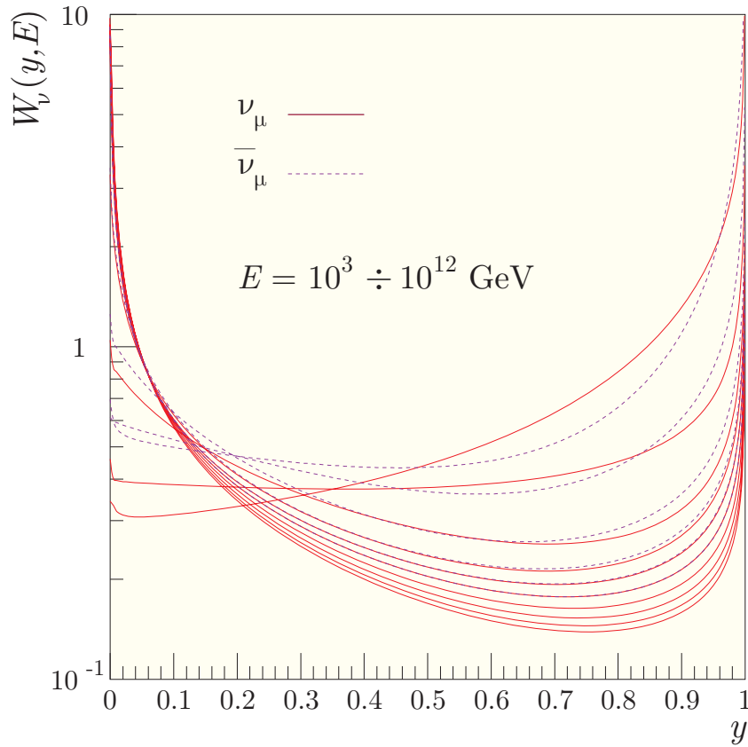
Figure 184: Regeneration functions W_{\nu_\mu}(y, E) and W_{\bar{\nu}_\mu}(y, E) vs Bjorken y for E = 10^k GeV [ k = 3, 4, \dots, 12 from top to bottom].
