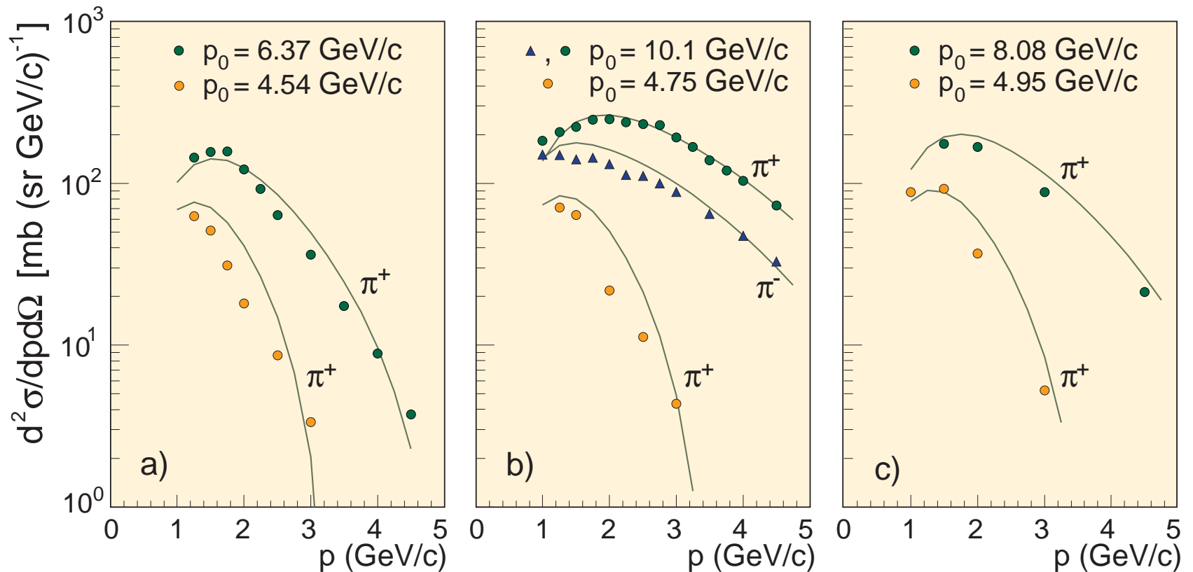
Figure 49: Differential cross sections of \pi^\pm production in interactions of low-momentum protons with Be target vs pion momentum at \theta = 3.5^\circ . Curves are calculated in the KM model. Data points are from A. S. Arefiev et al. , ITEP preprint N. 25, 1985 (unpublished); I. A. Vorontsov et al. , ITEP preprint N. 85, 1983 and N. 144, 1984 (unpublished).
