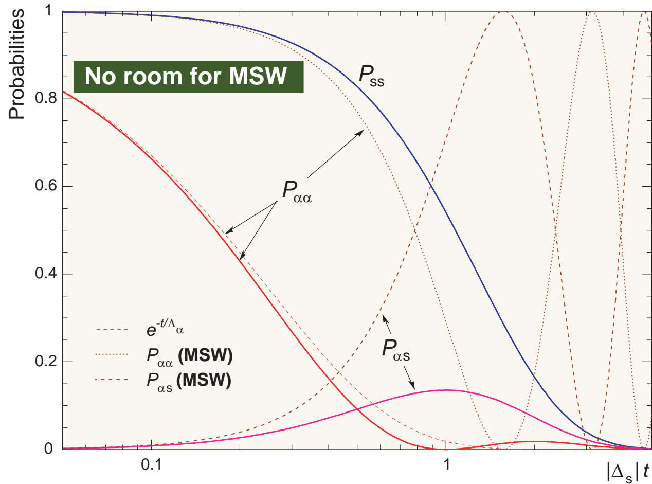
Figure 215: Survival and transition probabilities for \nu_\alpha \leftrightarrow \nu_s oscillations in the case of degeneracy ( q = q_{-\zeta} ). The standard MSW probabilities (dotted and dash-dotted curves) together with the penetration coefficient for unmixed \nu_\alpha (dashed curve) are also shown.
