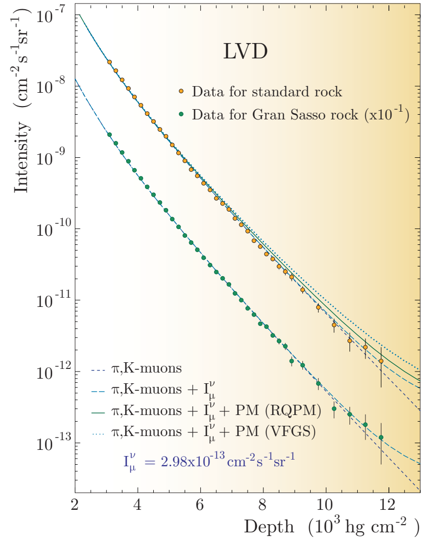
Figure 87: \mu DIR from LVD.
