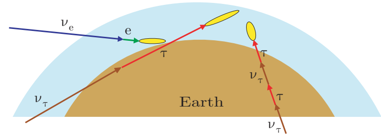
Figure 186: Schematic \nu initiated air showers. [from S. Bottai and S. Giurgola, Astropart. Phys. 18 (2003) 539 (astro-ph/0205325).]
