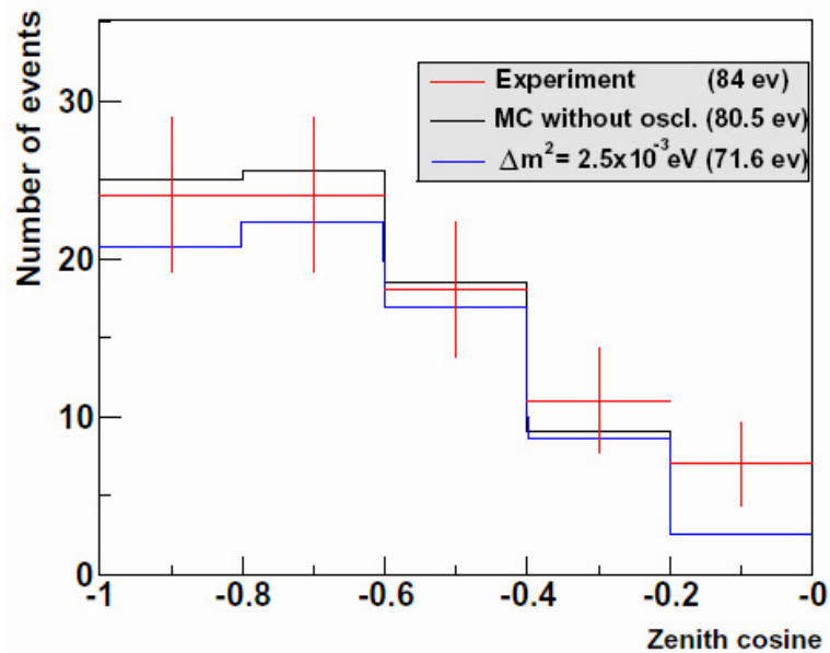
Figure 162: Zenith angle distribution of 84 upward-going reconstructed events in the Baikal NT-200 experiment and MC simulated distribution of upward muon tracks due to atmospheric neutrinos. E_{\text{th}} = 15 - 20 \text{ GeV} in this experiment.
