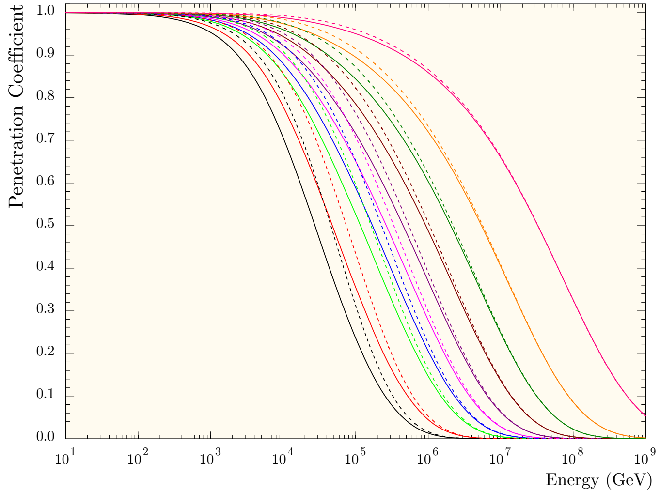
Figure 201: Penetration coefficients for atmospheric \nu_\mu (solid curves) and \bar{\nu}_\mu (dashed curves) vs energy for \cos \vartheta = -0.1, -0.2, \dots, -1.0 . (from top to bottom).
