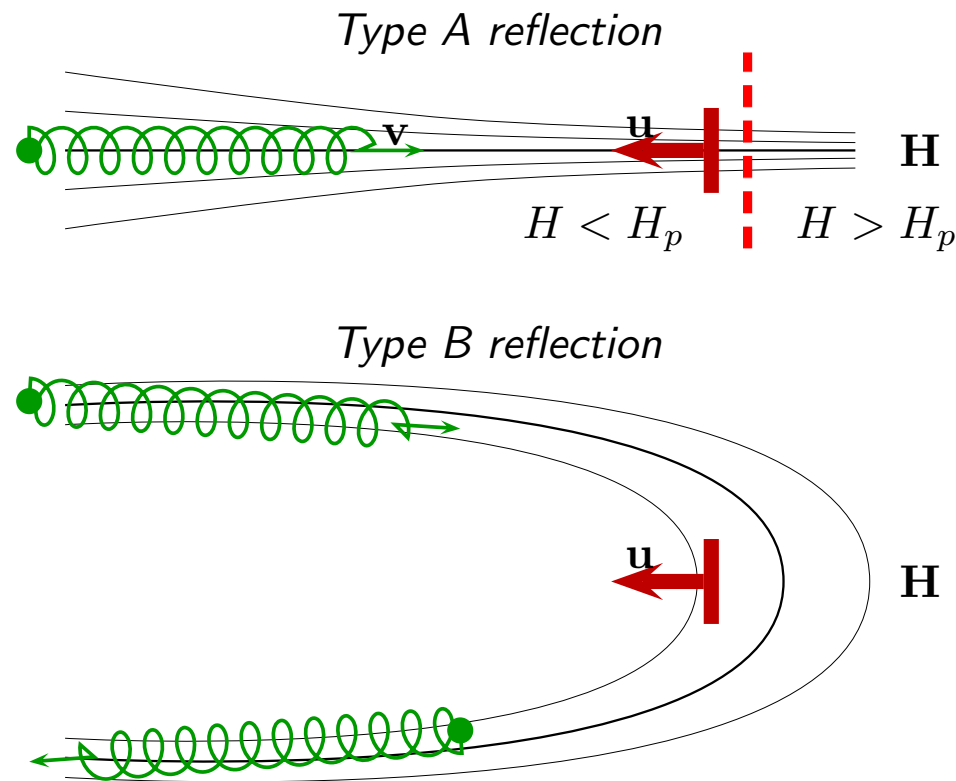
Figure 217: Collisions with moving magnetic irregularities leading to reflection.
