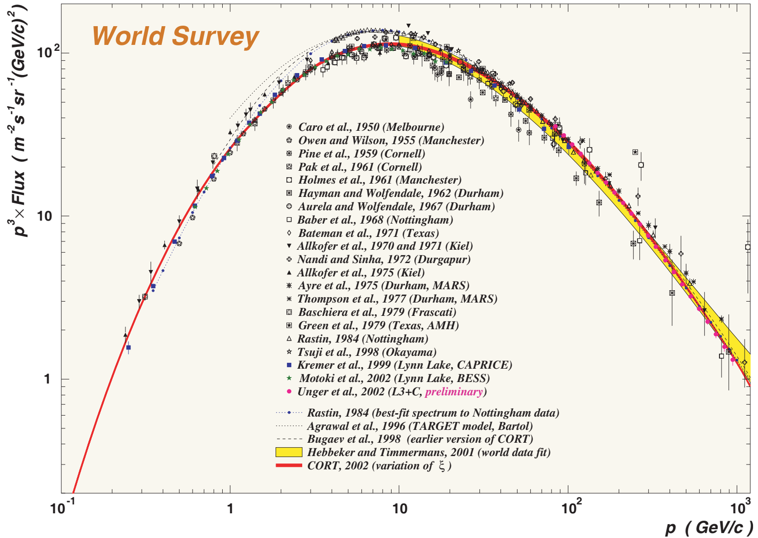
Figure 60: Near-vertical differential momentum spectrum of \mu^+ + \mu^- at ground level.
