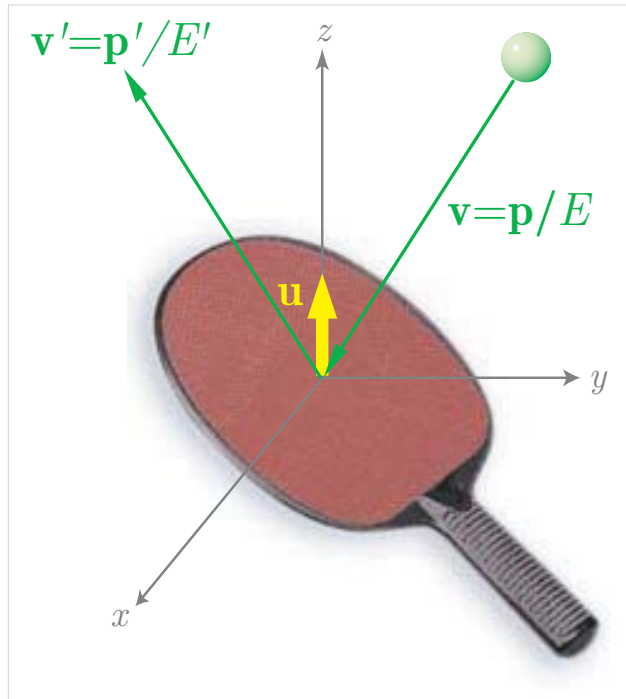
Figure 216: Relativistic pingpong.
