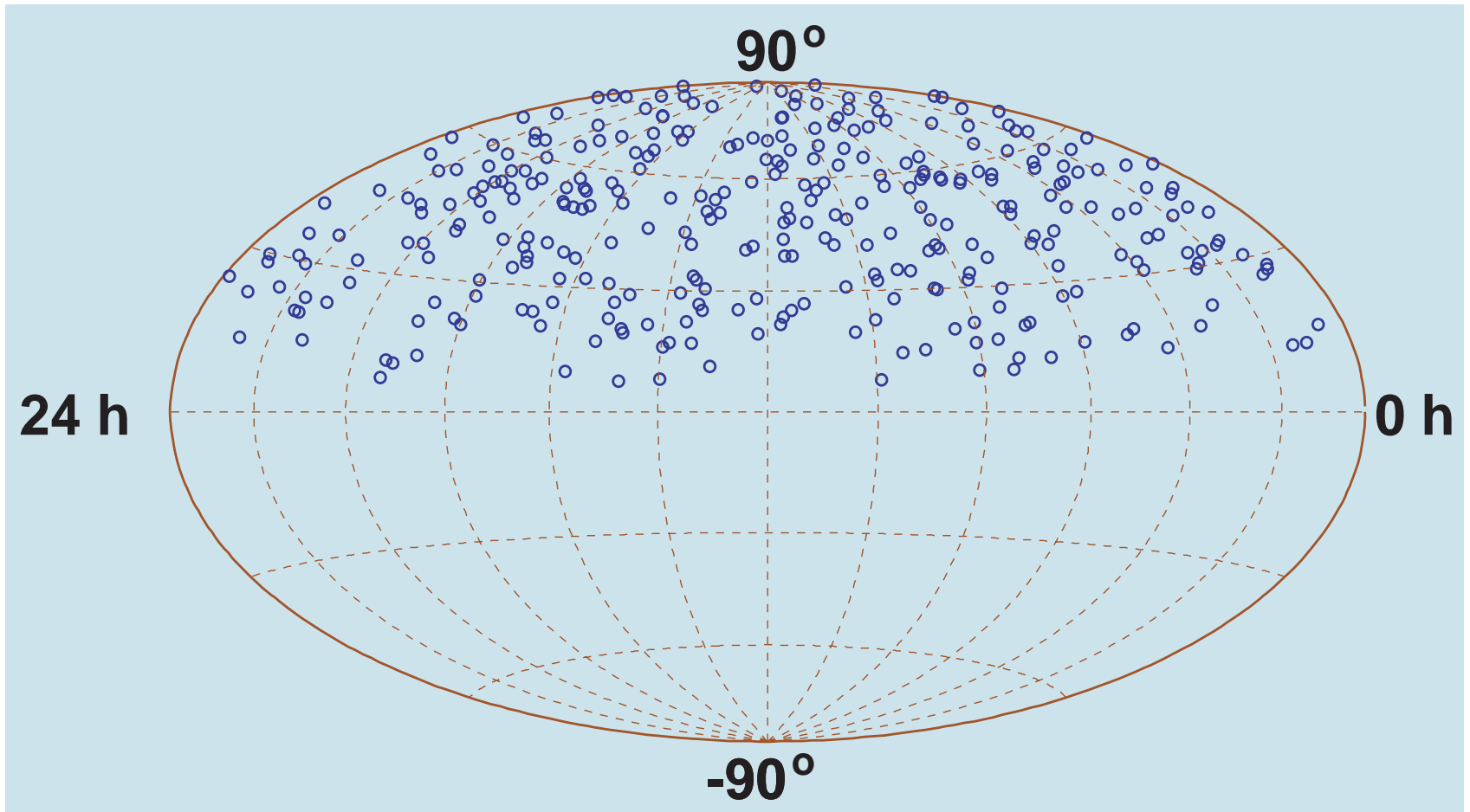
Figure 177: Skyplot of upward-going events as seen with AMANDA-B10 in 1997 in equatorial coordinates. The background of non-neutrino events is estimated to be less than 10%. [From J. Ahrens et al. (2002); see caption to Fig. 173.]
