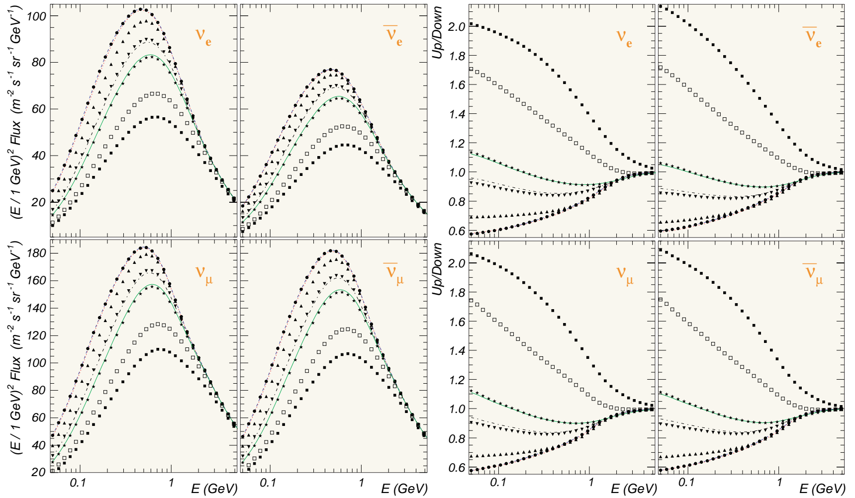
Figure 93: 4\pi averaged fluxes (left panel) and up-to-down ratios (right panel) of the \nu_e , \bar{\nu}_e , \nu_\mu , and \bar{\nu}_\mu fluxes for ten underground laboratories (see Table 15 for the notation).
