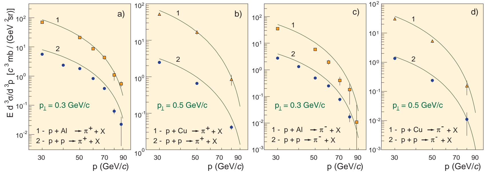
Figure 52: Invariant inclusive cross sections of \pi^\pm production in interactions of 100 GeV/c protons with p , Al and Cu targets vs pion momentum at two values of the pion transverse momentum. Curves are calculated in the KM model. Data points are from D. S. Barton et al. , Phys. Rev. D 27 (1983) 2580.
