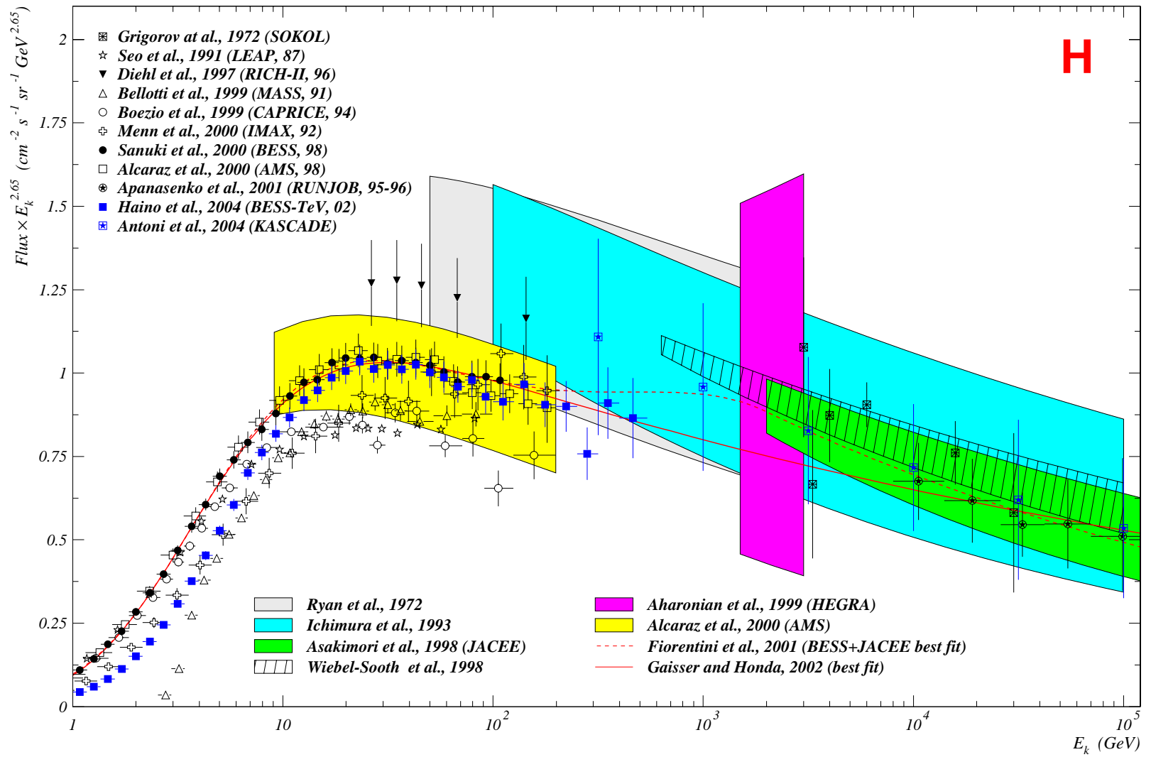
Figure 63: Gaisser-Honda model for primary hydrogen.
