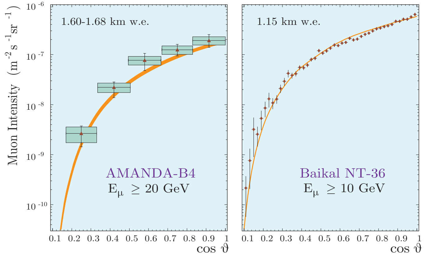
Figure 90: Zenith angle distributions of muons underice and underwater measured with AMANDA-B4 [Andres et al. (2000)] and Baikal NT-36 [Belolaptikov et al. (1997)], respectively. The filled area ( left panel ) and curve ( right panel ) are calculated with no account for the PM contribution. The thickness of the filled area reveals the uncertainty in the average “trigger depth” due to the size of the AMANDA-B4 telescope.
