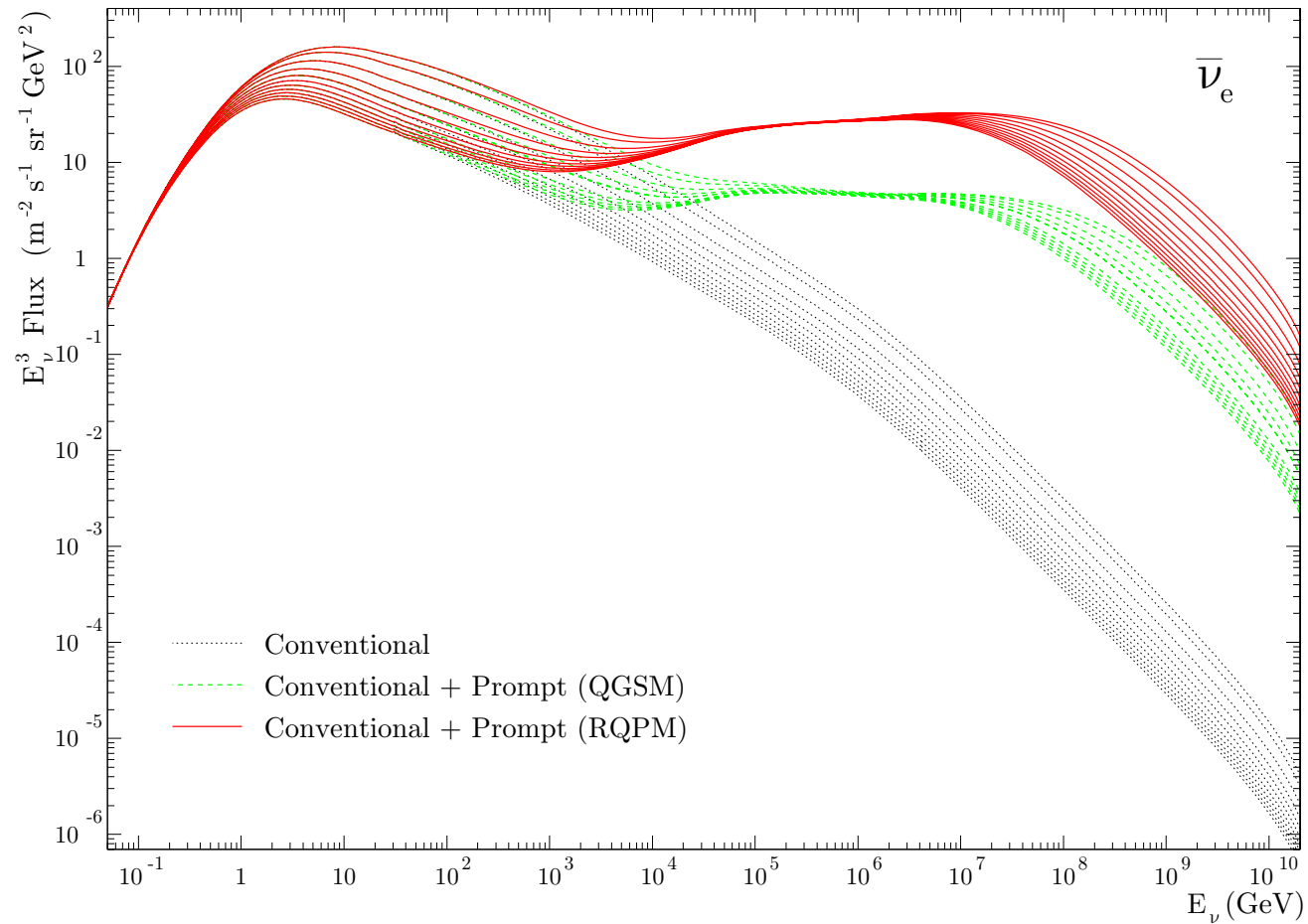
Figure 147: Energy spectra of downward going atmospheric \bar{\nu}_e for 11 zenith angles. Low-energy range is for Kamioka site. At high energies, from smallest to largest fluxes, \cos \theta varies from 0 to 1 with an increment of 0.1 for each group of curves.
