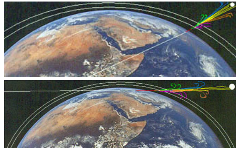
Figure 187: Upward and horizontal \tau showers. [from D. Fargion, astro-ph/0307485].
