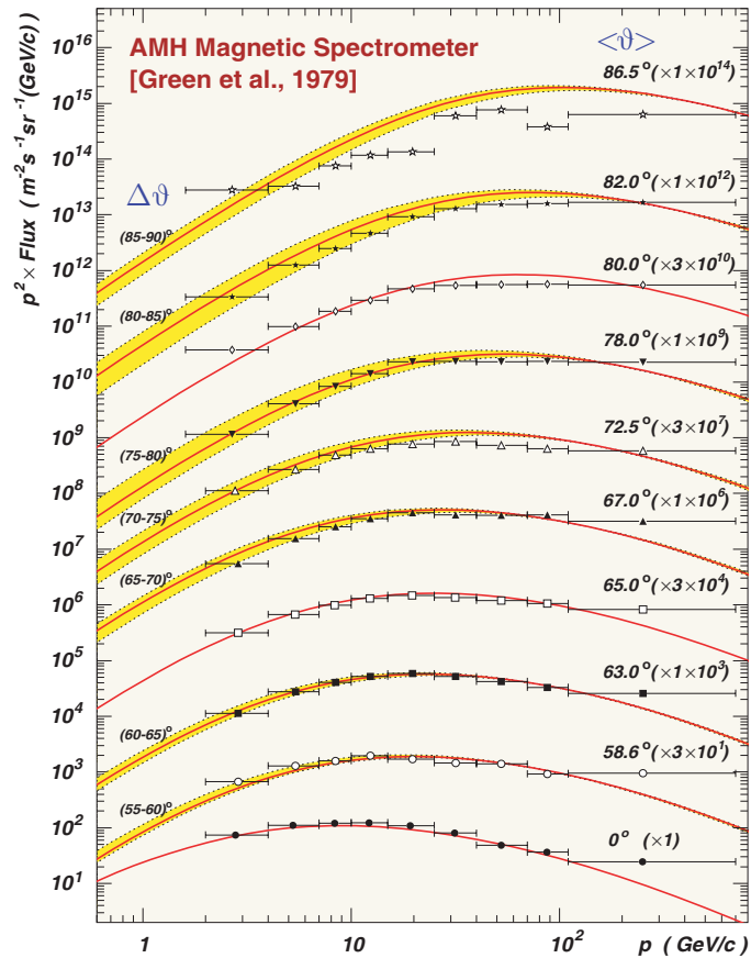
Figure 62: Differential momentum spectra of muons at sea level measured with the AMH magnetic spectrometer.
