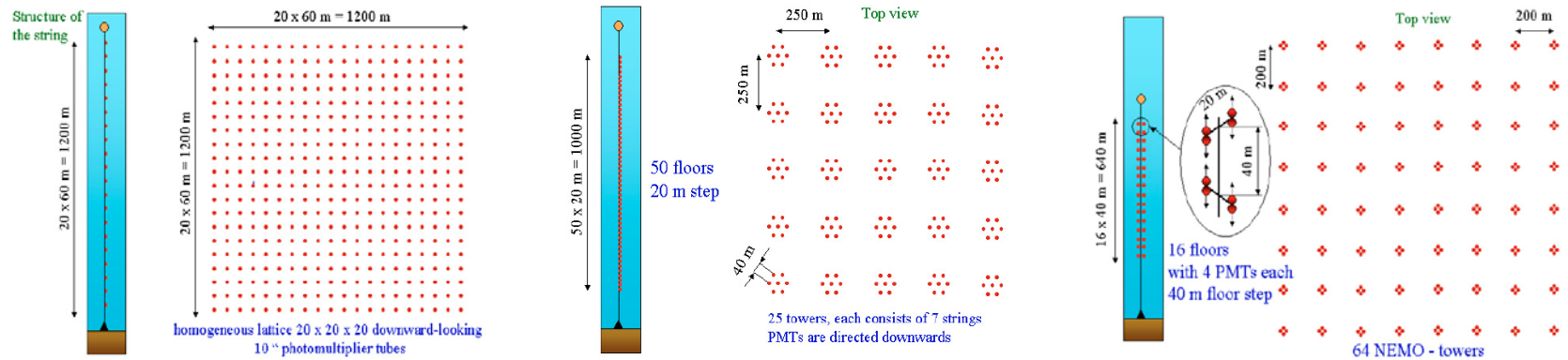
Figure 181: Future KM3 neutrino telescope geometries. Left panel: schematic view of a homogeneous detector with 8000 PMTs (not quite optimal to be built); middle panel: the layout of a NESTOR-like detector with 8750 PMTs; right panel: the layout of a NEMO-like detector with 4096 PMTs. These three designs have very different degrees of homogeneity. One more difference may be due to various numbers of downward-looking and upward-looking PMTs (down-down, up-down, etc.).
