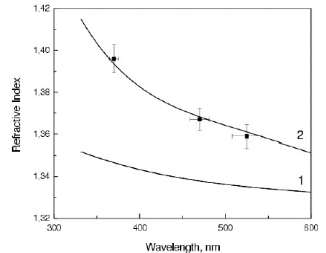
Figure 153: Wavelength dependencies of n (curve 1) and n_g = n - \lambda \partial n / \partial \lambda (data points and curve 2) for distilled Baikal water.
