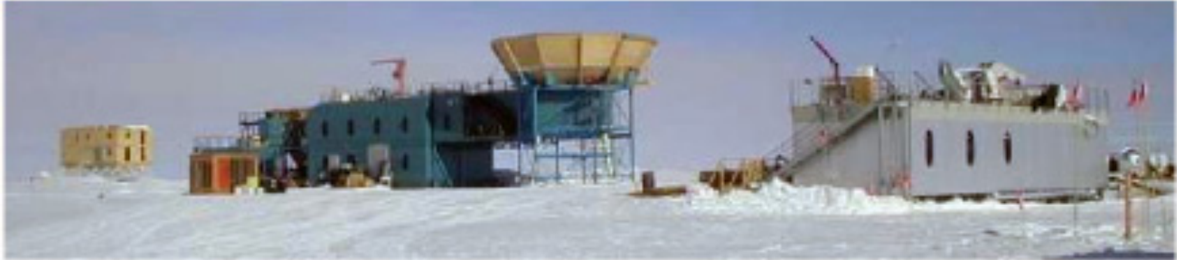
Figure 170: The South Pole Station. The AMANDA-II telescope electronics are located on the 2nd floor of MAPO, the blue building shown in this picture. [From http://www.amanda.uci.edu/ .]
