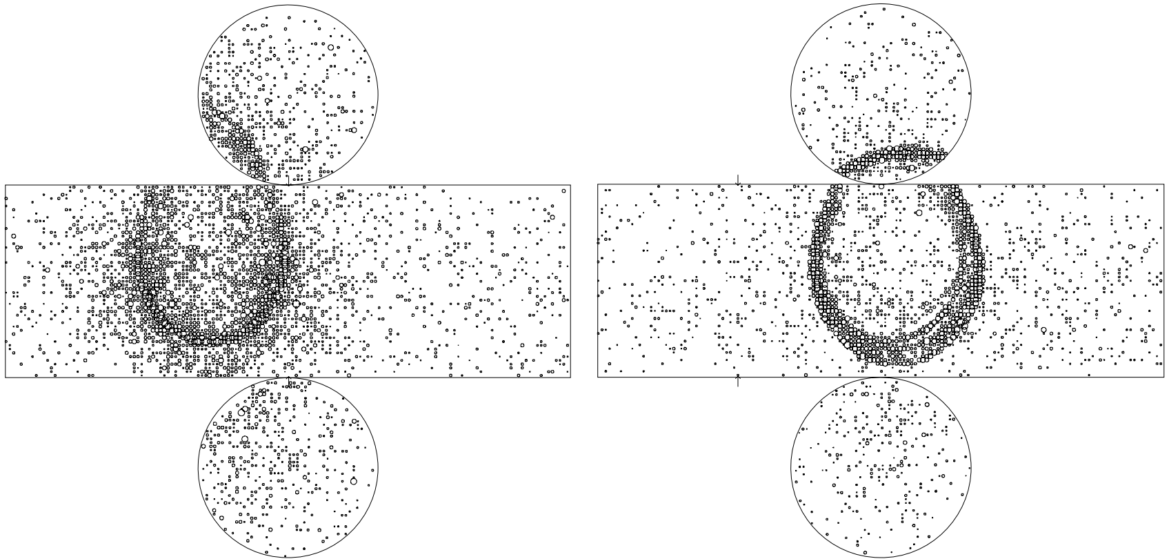
Figure 107: Example event display of a single-ring e -like event (left) and \mu -like event (right) in Super-Kamiokande I. Cherenkov rings from electromagnetic cascades exhibit a more diffuse light distribution than those from muons.
