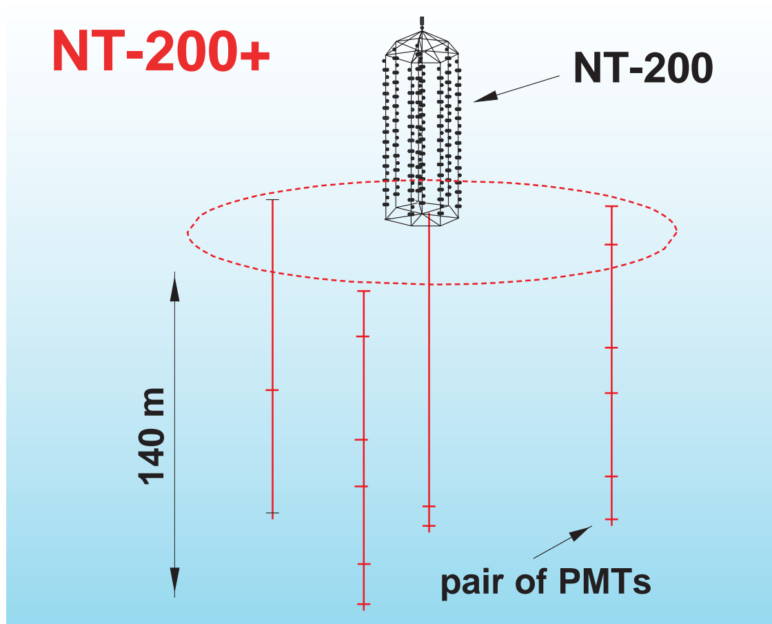
Figure 166: Future NT-200+ configuration. Three additional outer plus one possible central strings will allow a much better vertex identification and hence a significantly more precise measurement of cascade energy in a volume around the NT-200.
