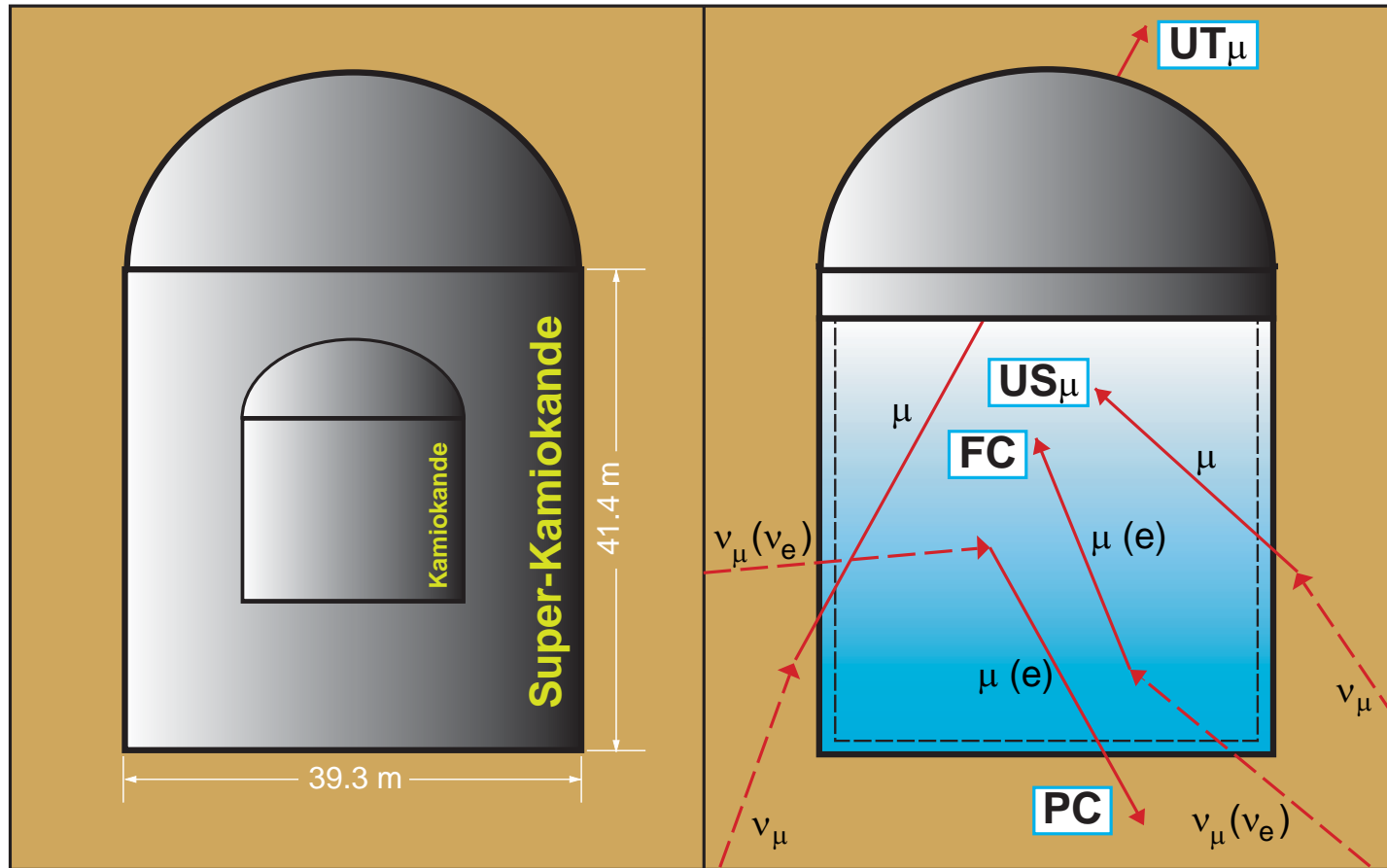
Figure 105: Comparative dimensions of the Kamiokande and Super-Kamiokande (left panel) and neutrino induced event classification (right panel) in these detectors. Abbreviation expansion: FC = Fully Contained, PC = Partially Contained, US_\mu = Upward-going Stopping Muons, UT_\mu = Upward Through-going Muons (see also Table 16).
