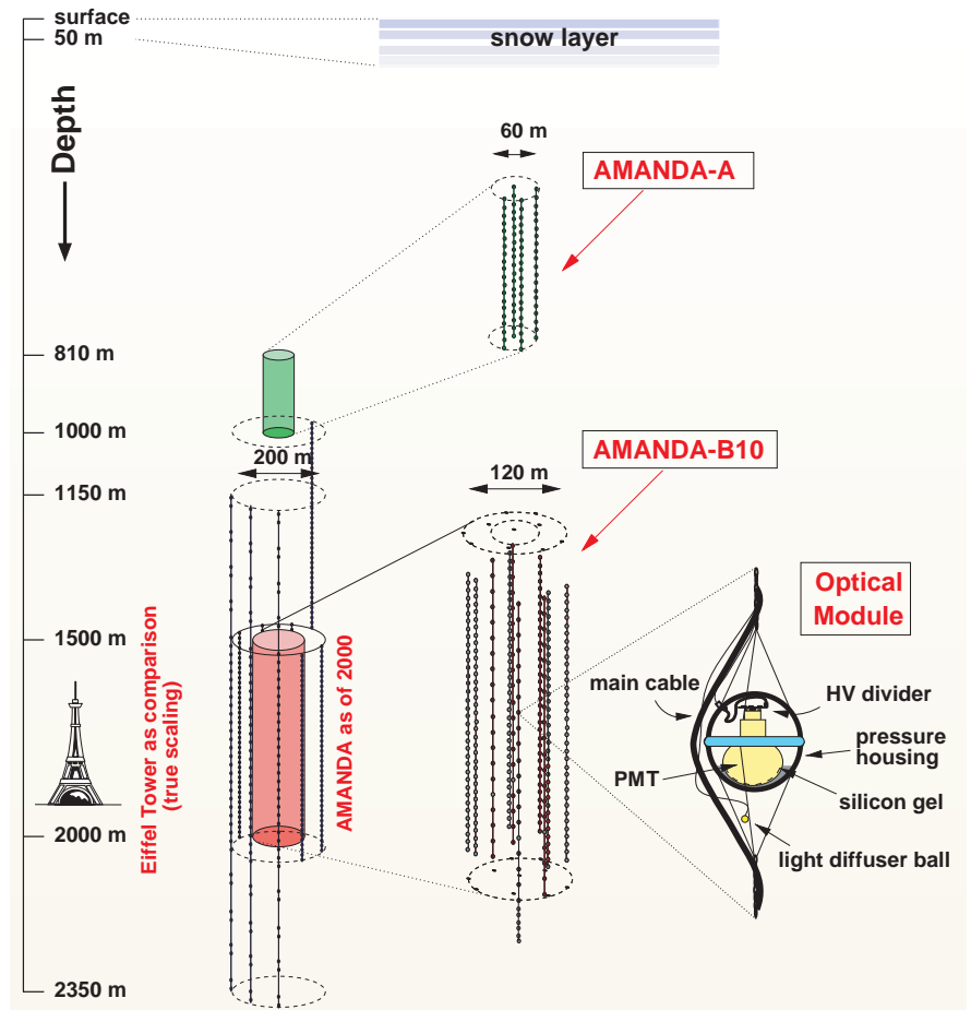
Figure 173: Schematic view of the AMANDA-II array at the South Pole. [From J. Ahrens et al. , Phys. Rev. D 66 (2002) 012005 [astro-ph/0205109].]
