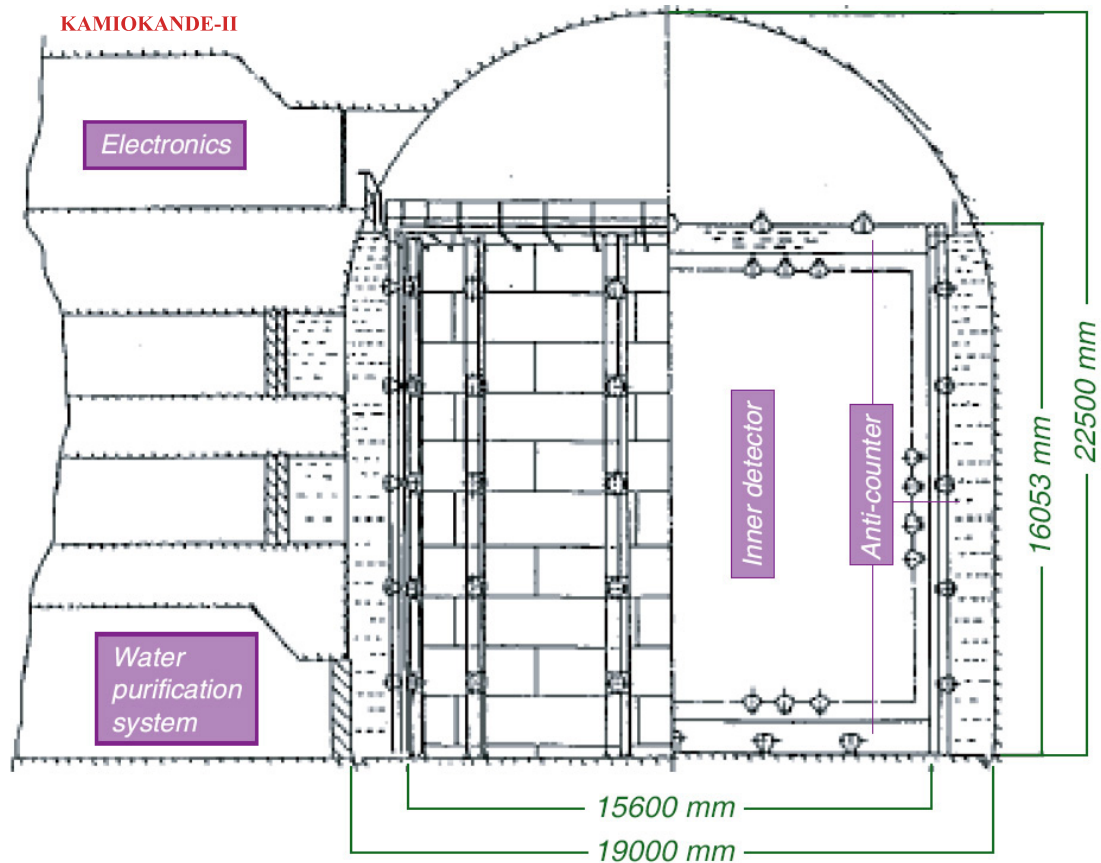
Figure 103: Schematic view of the Kamiokande-II detector. The slantwise hatches mark the surrounding rock. The inner detector contains 3000 tons of water of which 2140 tons are fiducial volume (the area enclosed with dotted-dashed line). It is viewed by 948 20-inch-diameter PMT's mounted on a 1-m grid on the inner surface. The outer (veto) counter surrounds the inner detector and is viewed by 123 PMT's.
