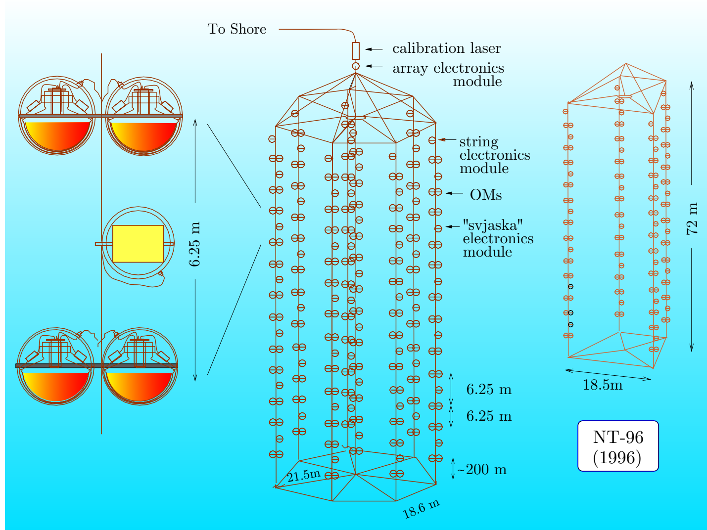
Figure 158: NT-200 and NT-96 schematic view (see text for description and references).
