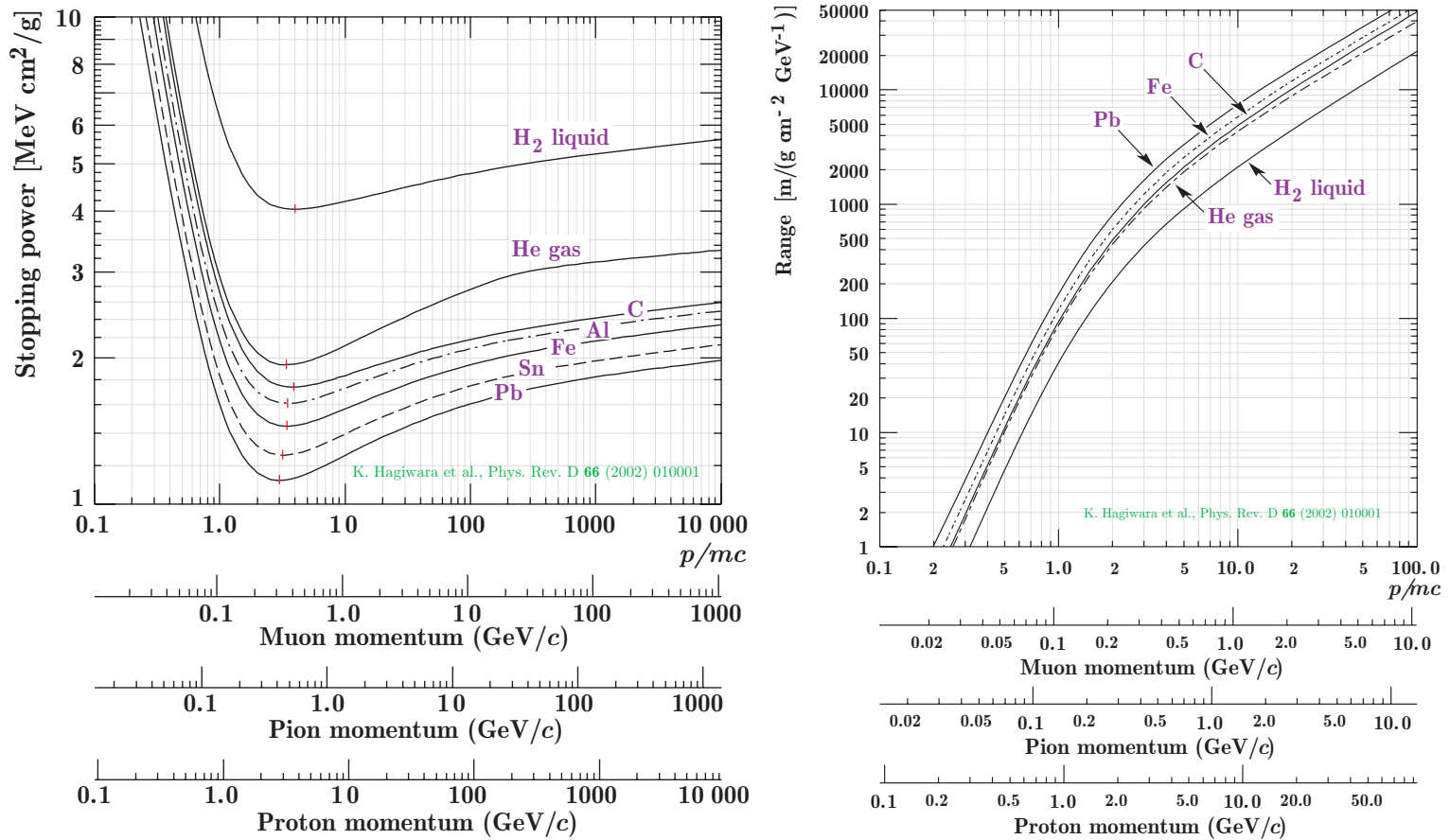
Figure 16: Stopping power and range of heavy particles vs p/mc in liquid hydrogen, gaseous helium, carbon, aluminum, iron, tin, and lead. Radiative effects, relevant for muons and pions, are not included. These become significant for muons in iron for p/mc > 1000 , and at lower momenta, for muons in higher- Z absorbers. [From the Review of Particle Physics by K. Hagiwara et al. , Phys. Rev. D 66 (2002) 010001.]
