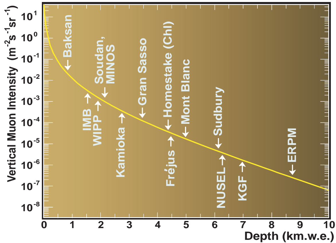
Figure 101: Depths of several underground laboratories. Solid line is the calculated vertical cosmic-ray muon intensity in the standard rock.
