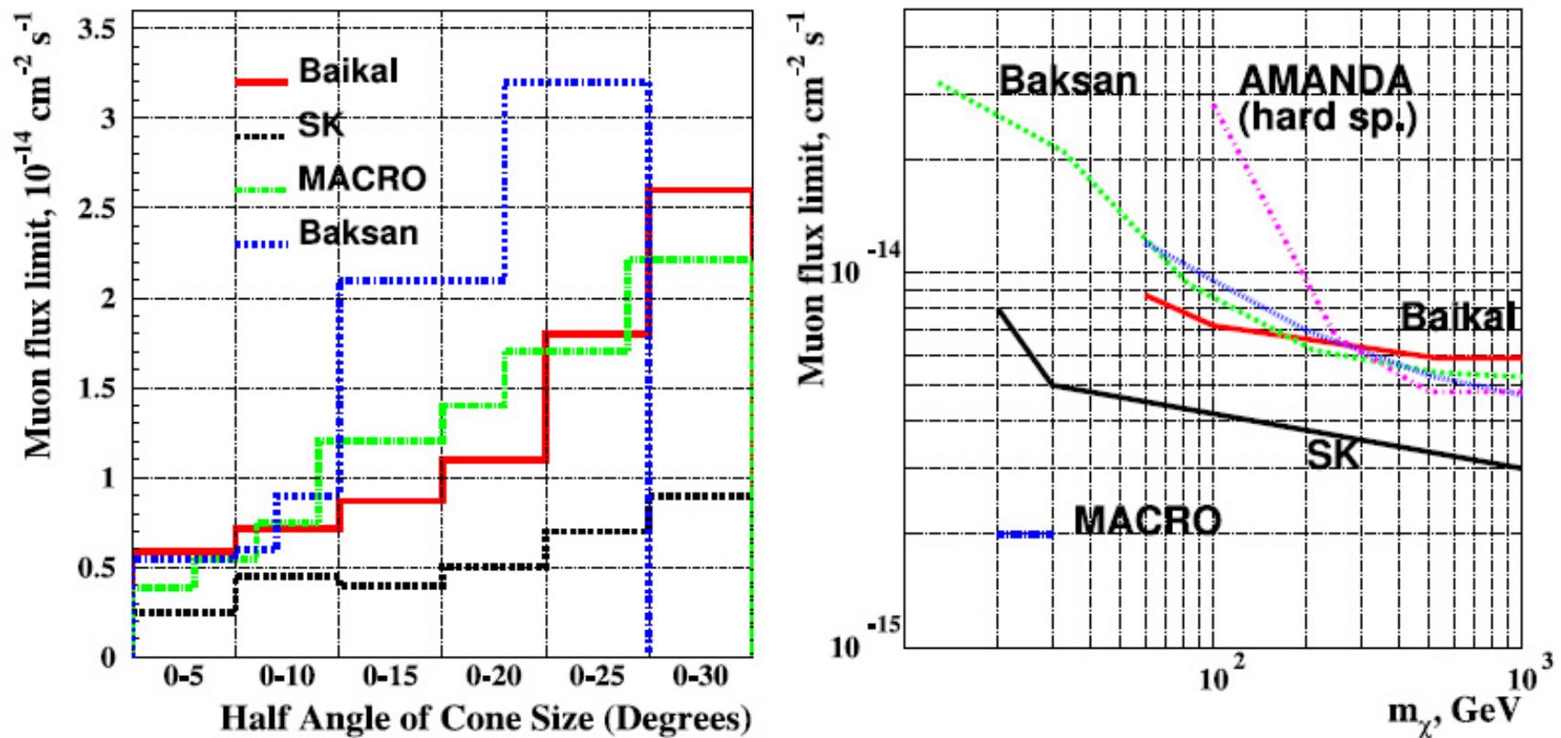
Figure 164: Limits on the excess muon flux from the center of the Earth vs half-cone of the search angle (left panel) and as a function of WIMP mass (right panel).
