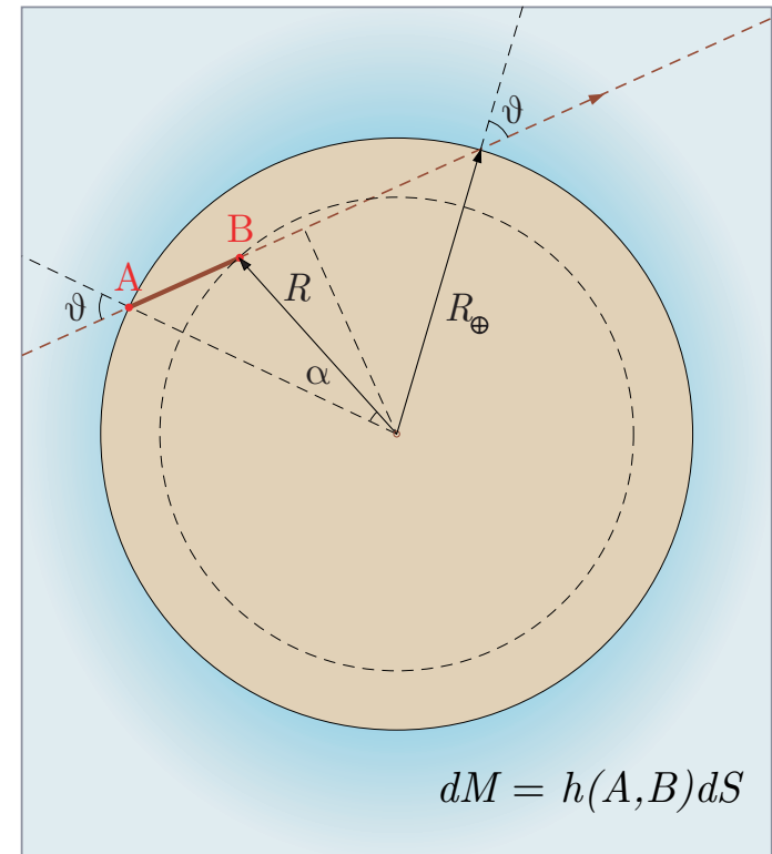
Figure 188: Definition of variables to derive the depth h(\alpha, \vartheta) for the Earth.
