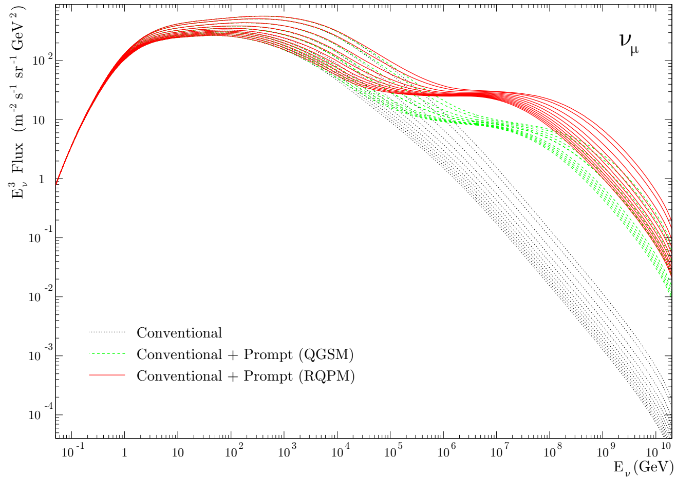
Figure 148: Energy spectra of downward going atmospheric \nu_\mu for 11 zenith angles. Low-energy range is for Kamioka site. At high energies, from smallest to largest fluxes, \cos \theta varies from 0 to 1 with an increment of 0.1 for each group of curves.
