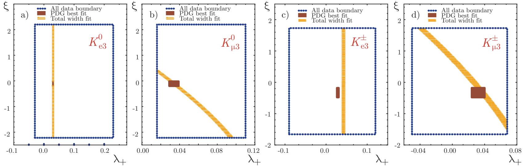
Figure 46: Spread in measured values of the K_{\ell 3} form factor parameters \lambda_+ and \xi and ranges of values which provide the best agreement with the PDG data fit (see Table 9).
