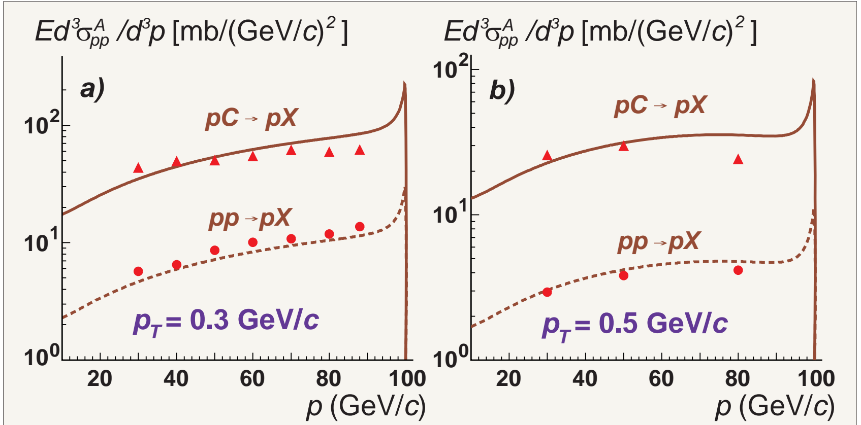
Figure 26: Invariant inclusive cross sections calculated for the reactions p + C \rightarrow p + X (solid curves) and p + p \rightarrow p + X (dashed curves) using the KM model at p_0 = 100 GeV/c and the p_{\perp} values of 0.3 GeV/c (a) and 0.5 GeV/c (b). The experimental data points are from D.S. Barton et al., Phys. Rev. D 27 , (1983) 2580.
