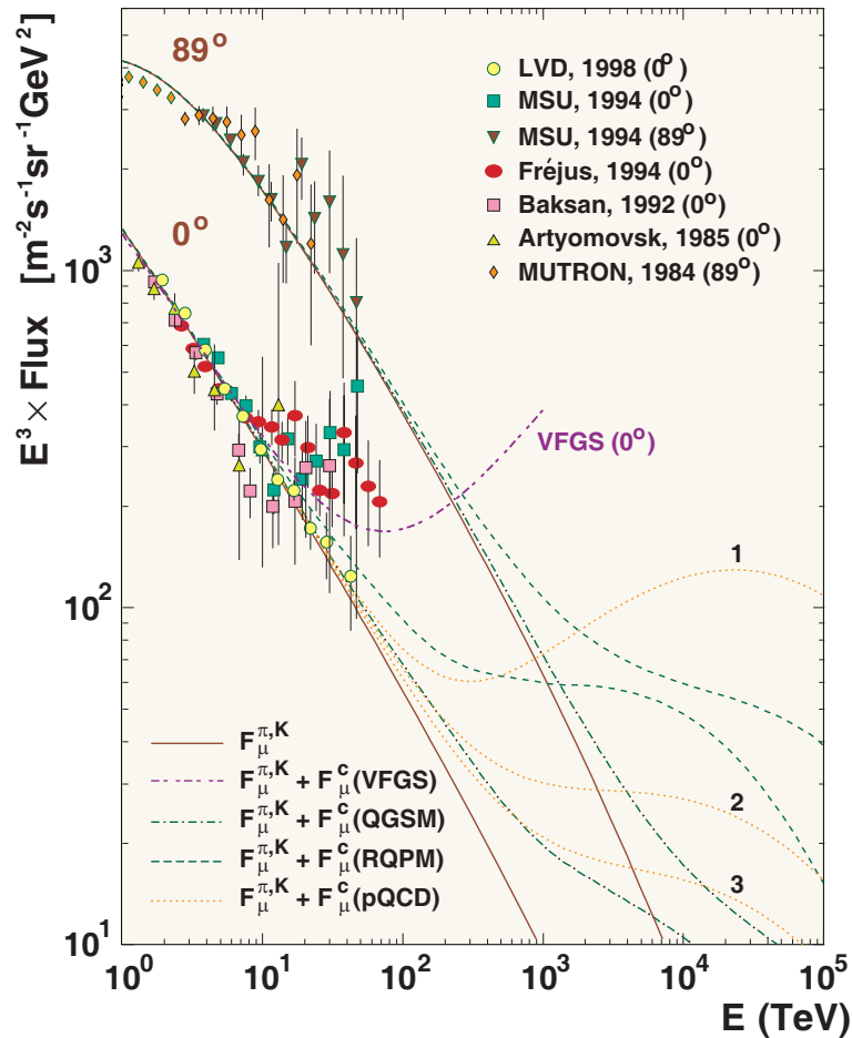
Figure 76: Differential energy spectra of muons at s.l. for vertical and horizontal directions above 1 TeV.
