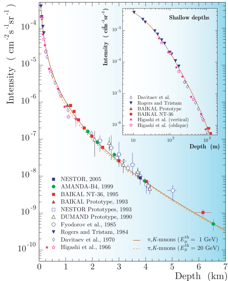
Figure 89: Muon DIR from the underwater/ice experiments.
