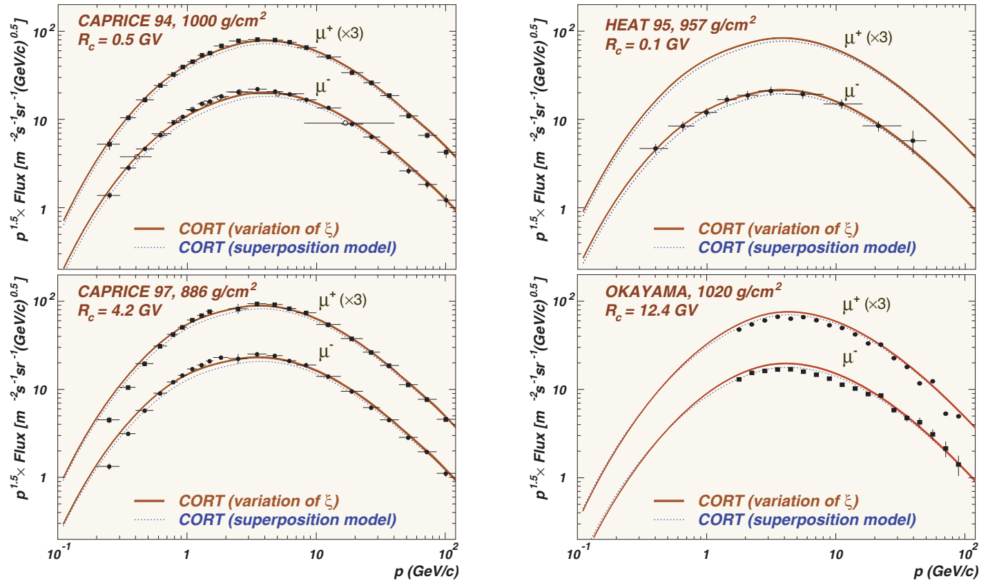
Figure 59: Vertical differential momentum spectra of \mu^+ and \mu^- at ground level for different depths and geomagnetic cutoffs. The data points are from the CAPRICE 94 [Kremer et al. (1999), Boezio et al. (2000)], CAPRICE 97 [Kremer et al. (1999)], HEAT 95 [Coutu et al. (2000)] and from the Okayama altazimuthal counter cosmic-ray telescope [Tsuji et al. (2001)]. Solid narrow bands and dotted curves are calculated with CORT.
