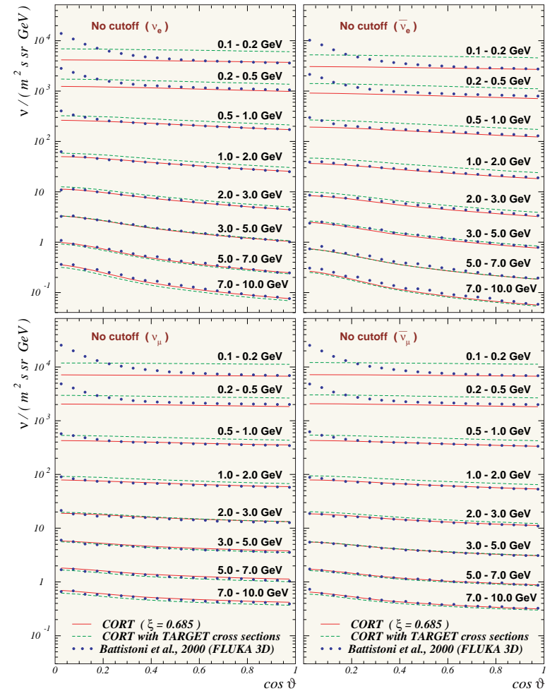
Figure 94: Zenithal distributions of down-going ANs on geomagnetic poles.
