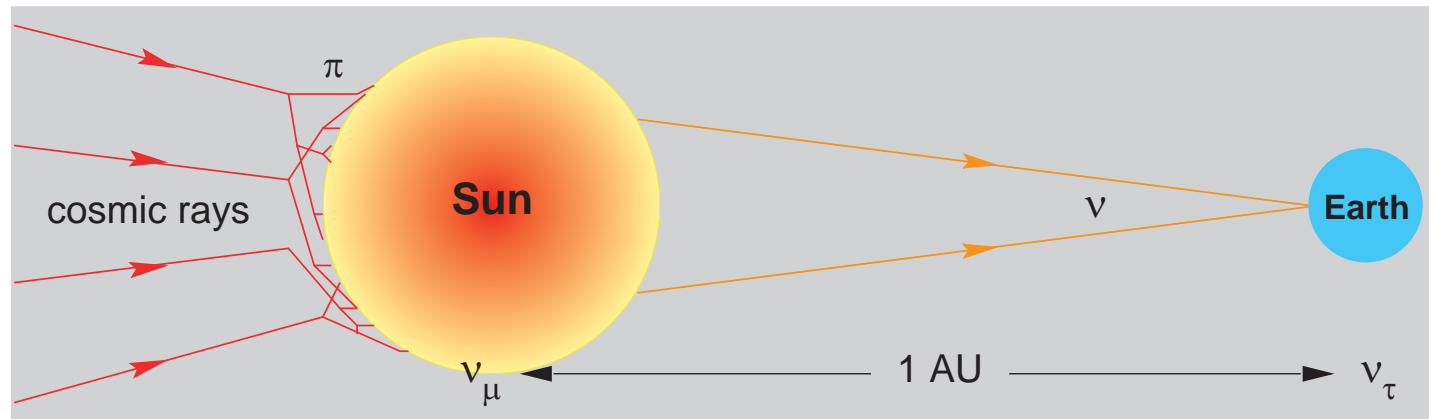
Figure 206: Cosmic rays hitting the Sun produce \nu_{\mu} 's which propagate further to Earth. At an energy of 10 \text{ TeV} the length for \nu_{\mu} \leftrightarrow \nu_{\tau} oscillations is (according to the SK AN result) about 1 \text{ AU} . [From J. G. Learned and K. Mannheim, Ann. Rev. Nucl. Part. Sci. 50 (2000) 679, Fig. 7.]
