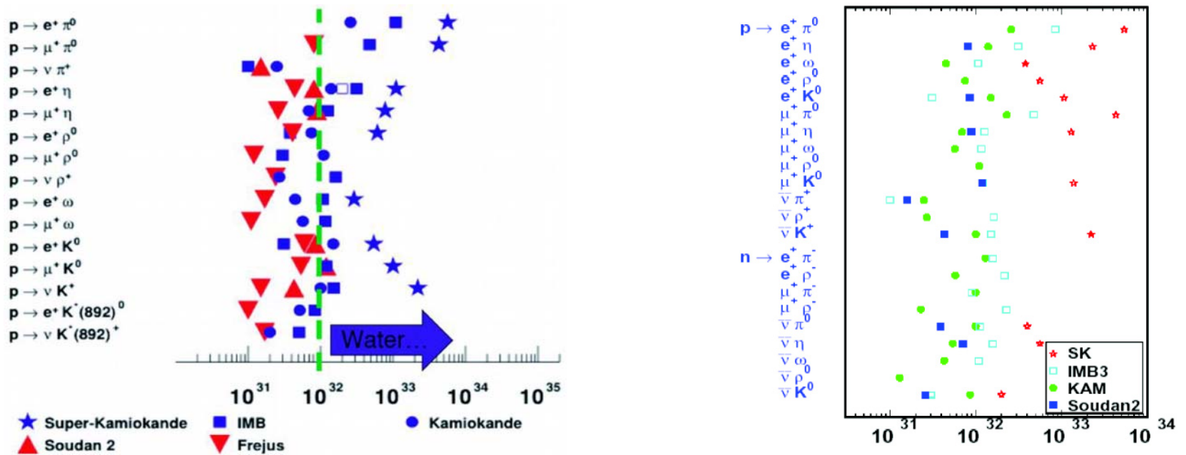
Figure 40: Proton decay limits.
