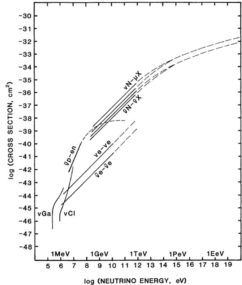
Figure 41: A tentative representation of atmospheric and extraterrestrial neutrino fluxes on the Earth (left) and cross sections for neutrino interactions with nuclei, nucleons and electrons (right). [From A. M. Bakich, "Aspects of neutrino astronomy," Space Sci. Rev. 49 (1989) 259–310.]
