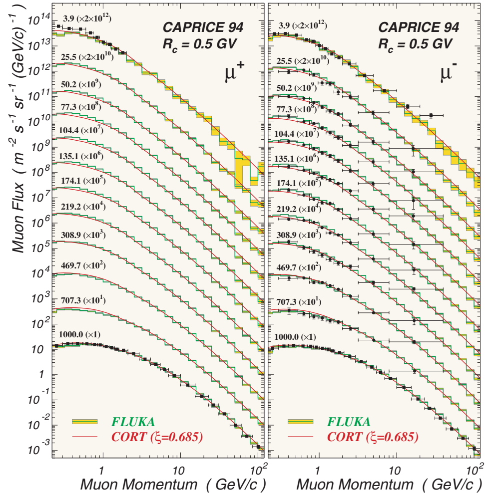
Figure 56: Differential momentum spectra of \mu^+ and \mu^- for 12 FADs. The data points are from the CAPRICE94 experiment [Boezio et al. (2000)]. The curves and histograms are calculated with CORT and FLUKA 3D, respectively.
