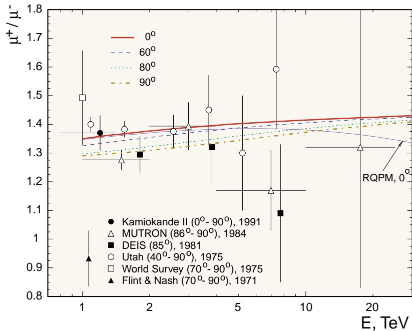
Figure 78: Muon charge ratio at s.l. for E > 1 TeV and for several zenith angles. The data of Kamiokande and Utah are deduced from underground measurements. The curve marked 'RQPM' accounts for the PM contribution according to the RQPM (for \vartheta = 0^\circ ).
