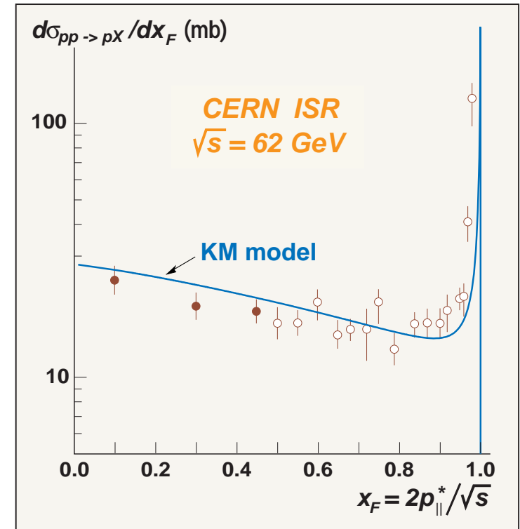
Figure 25: Differential cross section d\sigma_{pp \rightarrow pX}/dx_F vs x_F calculated with the KM model at \sqrt{s} = 62 GeV. The data of two CERN ISR experiments are from M. Basile et al. (ISR Collaboration), Nuovo Cim. 41A (1984) 298.
