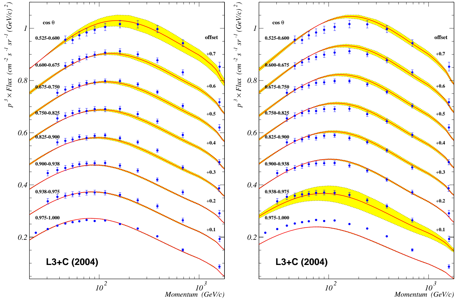
Figure 65: Comparison with the most recent result by L3+C. Calculations are done with the Gaisser-Honda primary spectra: “High Helium” (left) and “Low Helium” (right).
