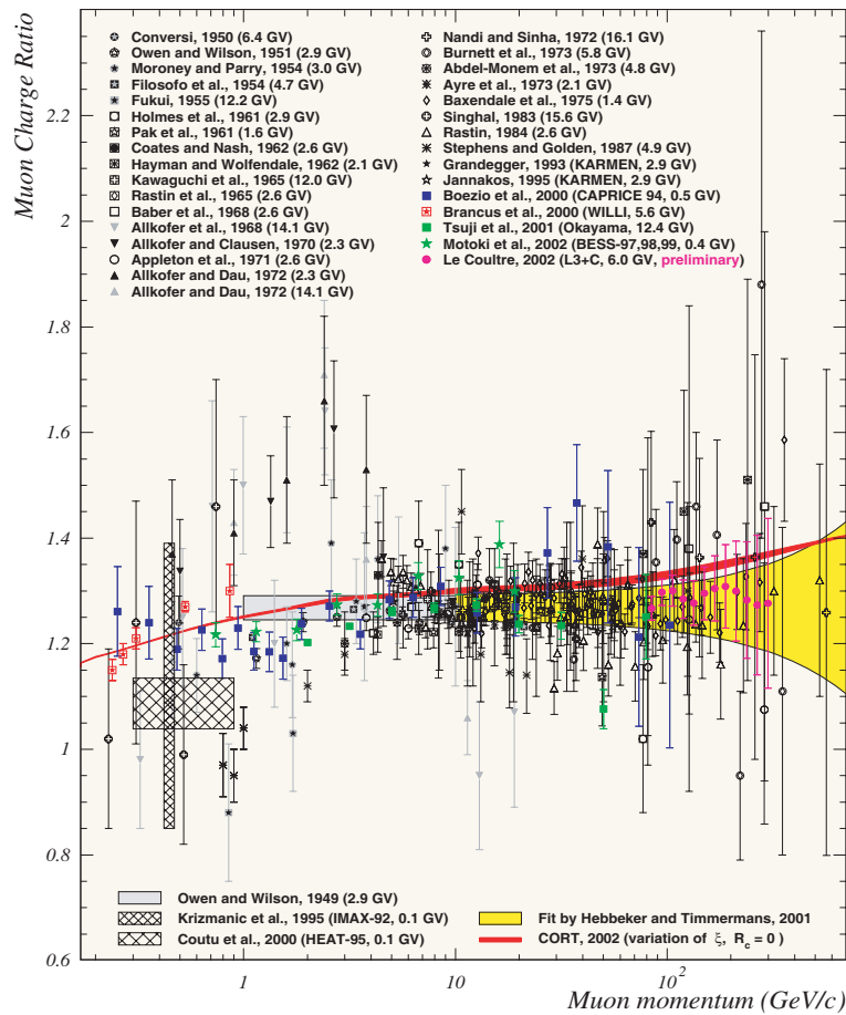
Figure 71: Near-vertical muon charge ratio at ground level. World survey.
