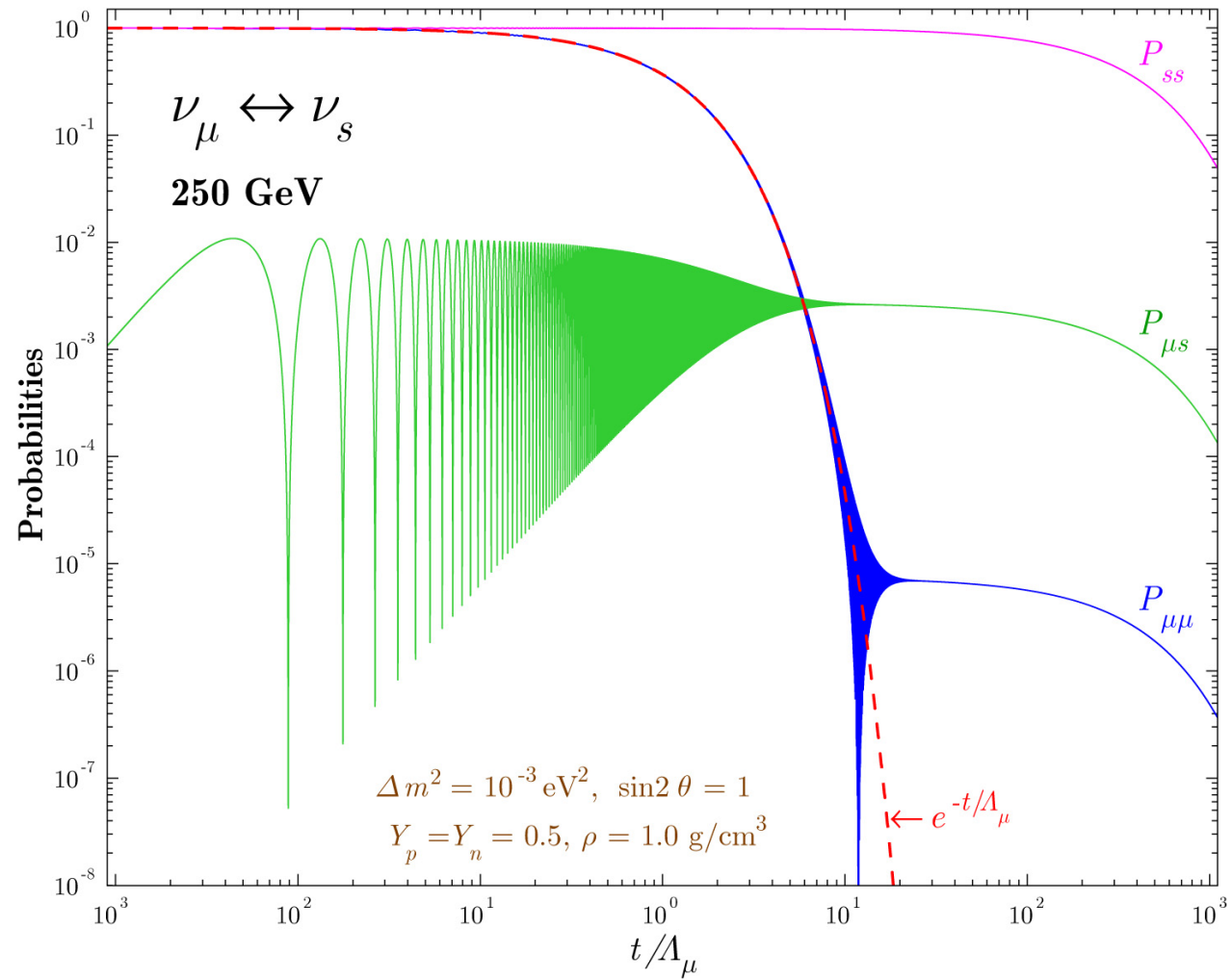
Figure 211: Survival and transition probabilities for \nu_{\mu} \leftrightarrow \nu_s oscillations ( E_{\nu} = 250 \text{ GeV} , \rho = 1 \text{ g/cm}^3 ).
