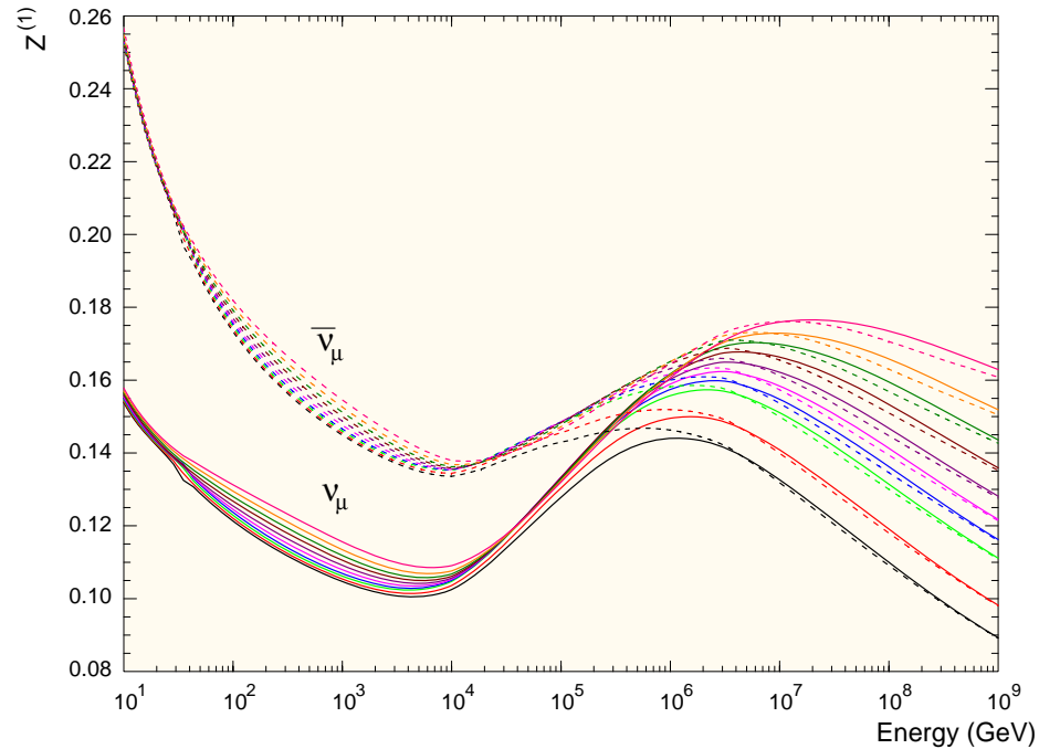
Figure 198: Z factors for atmospheric \nu_\mu (solid curves) and \bar{\nu}_\mu (dashed curves) vs energy, calculated in the 1st approximation in for \cos\vartheta = -0.1, -0.2, \dots, -1.0 (the sequence corresponds to the curves from top to bottom).
