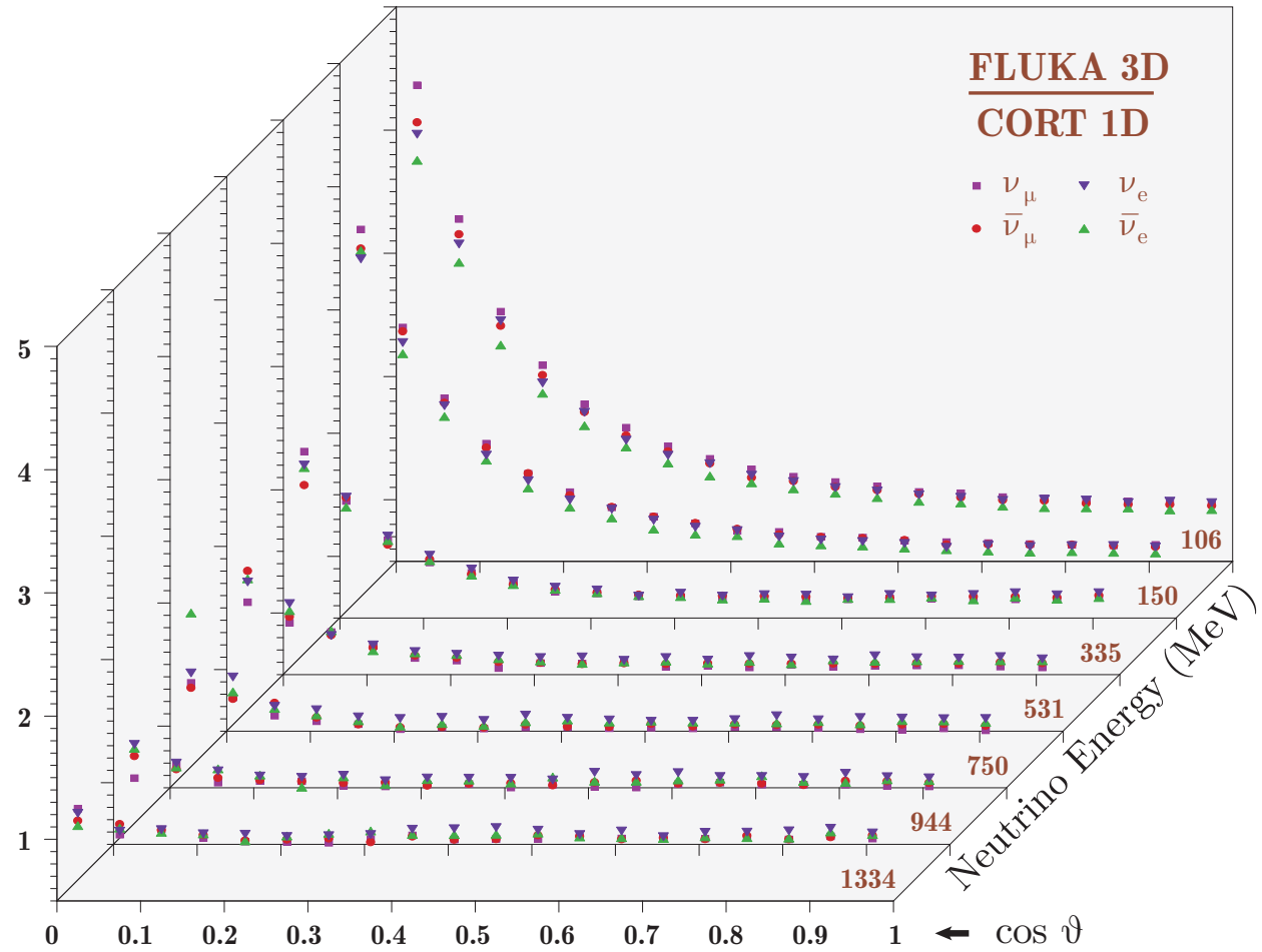
Figure 96: Zenithal distributions of ANs calculated with FLUKA 3D for seven values of neutrino energy and normalized to the same distributions calculated with CORT. The geomagnetic effects are neglected.
