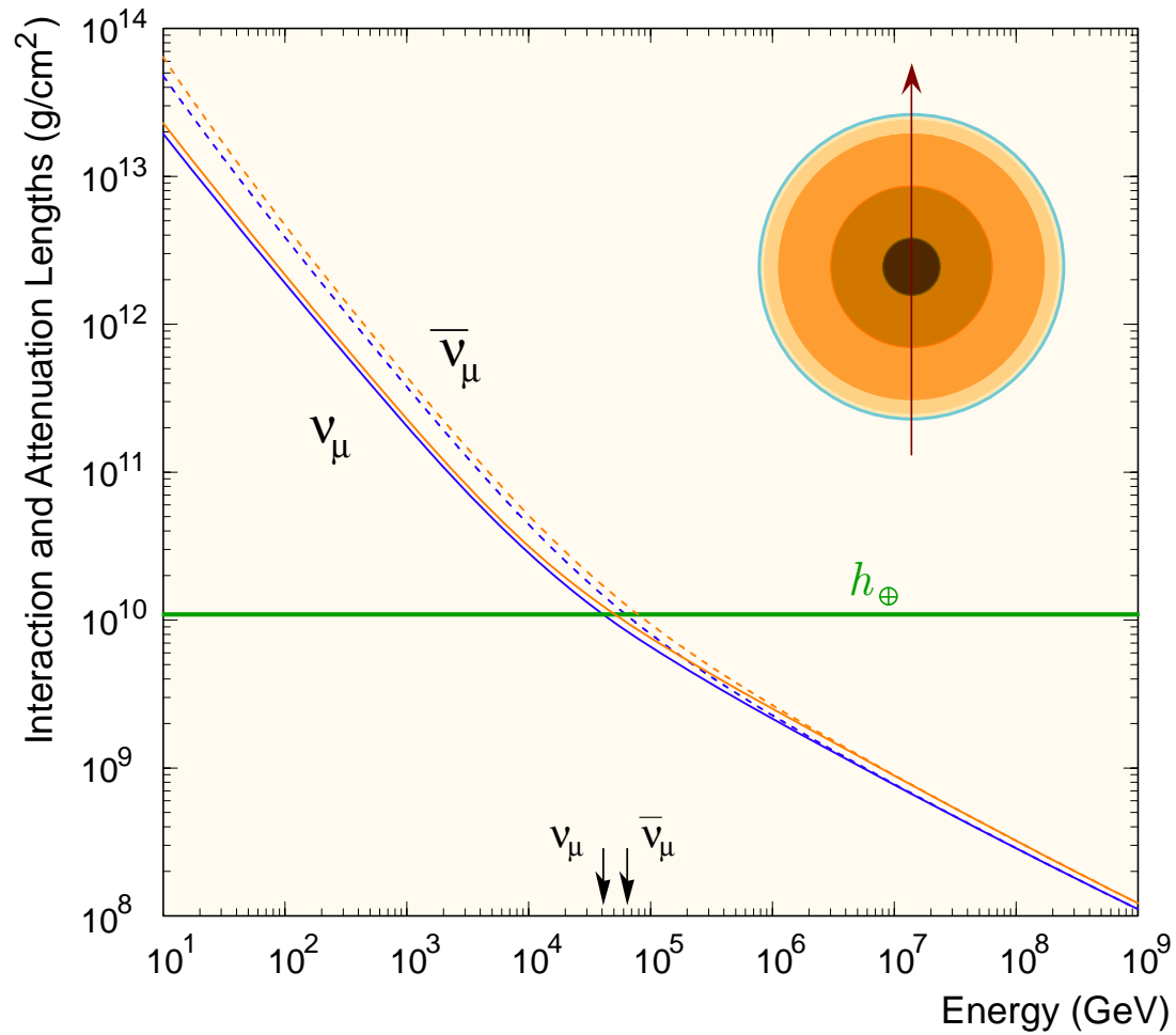
Figure 199: Interaction and attenuation lengths for atmospheric upward going \nu_{\mu} and \bar{\nu}_{\mu} in the Earth. The total depth of the Earth along its diameter is also shown for comparison.
