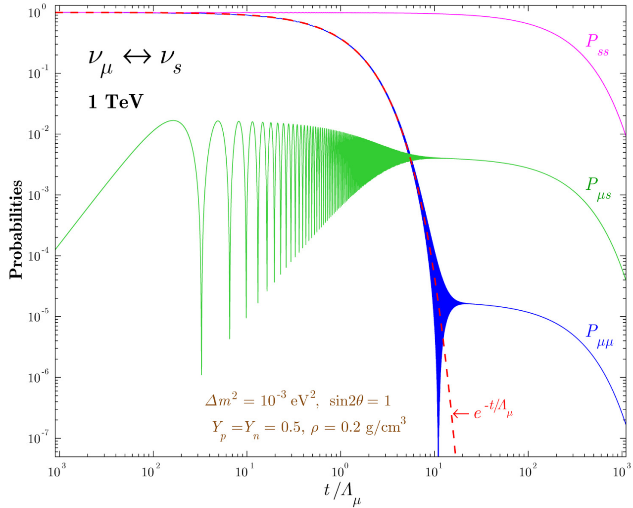
Figure 212: Survival and transition probabilities for \nu_\mu \leftrightarrow \nu_s oscillations ( E_\nu = 1000 \text{ GeV} , \rho = 0.2 \text{ g/cm}^3 ).
