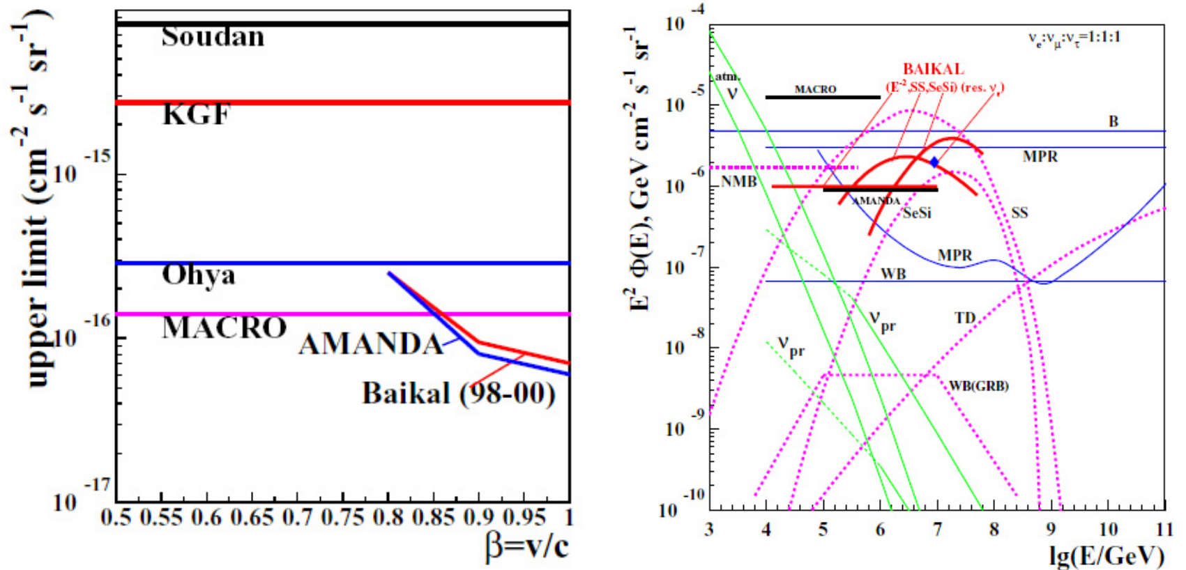
Figure 165: Upper limits on the flux of fast monopoles (left panel) and neutrino fluxes (right panel) obtained in different experiments. The neutrino fluxes expected from some astrophysical sources are also shown in the right panel.
