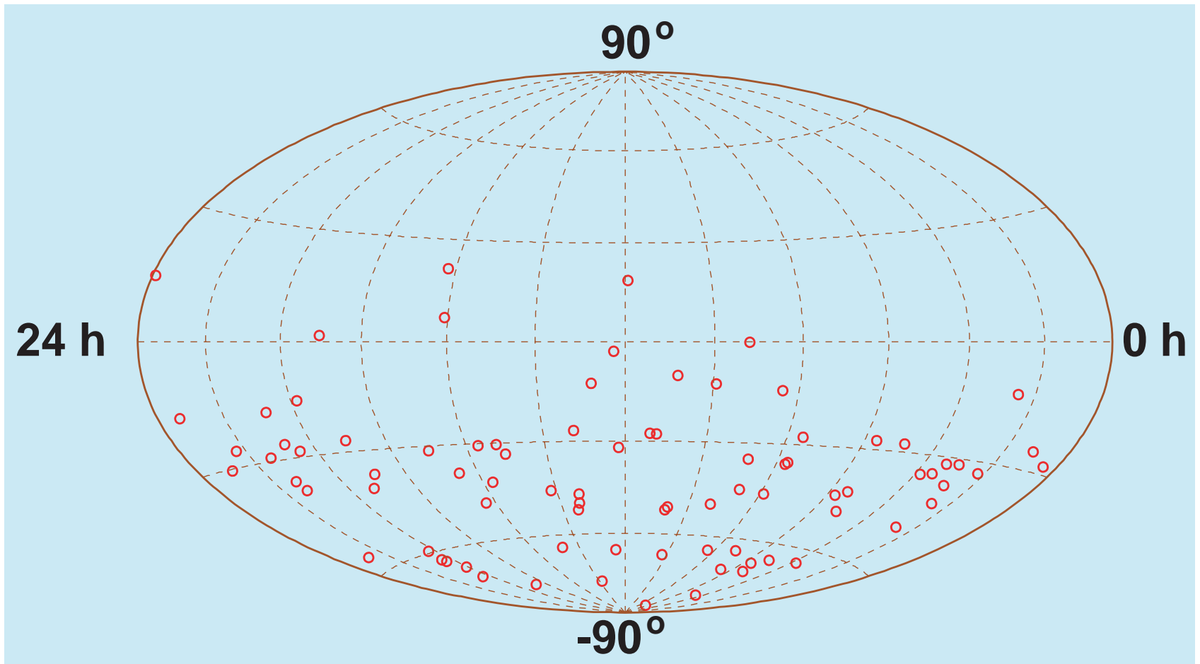
Figure 161: Skyplot (in equatorial coordinates) of 84 upward-going muon events recorded in the Baikal NT-200 experiment. [From R. Wischnewski (for the Baikal Collaboration), contribution to the 28th ICRC, Tsukuda, Japan, July 31 – August 7, 2003 (astro-ph/0305302).]
