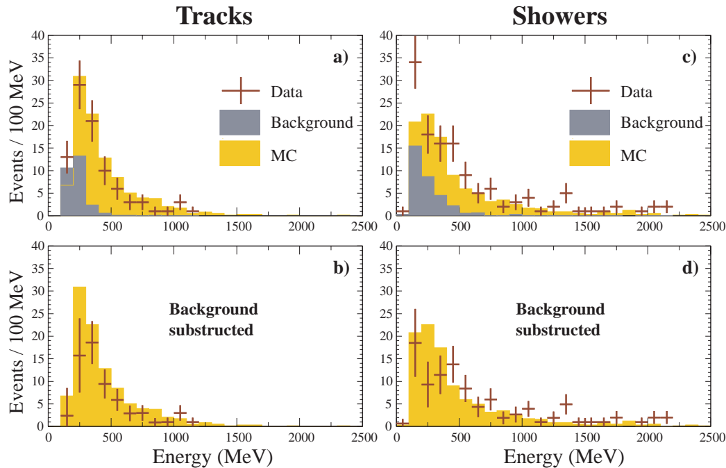
Figure 130: Energy distributions of SOUDAN 2 events.
