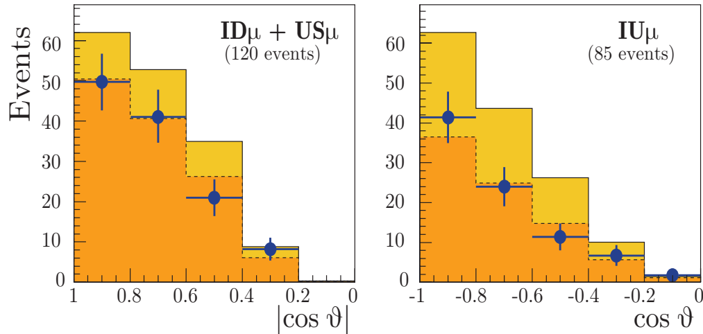
Figure 124: Angular distributions of ID_{\mu}+US_{\mu} and IU_{\mu} events in MACRO. MC histograms are for nonoscillating (higher) and oscillating ANs.
