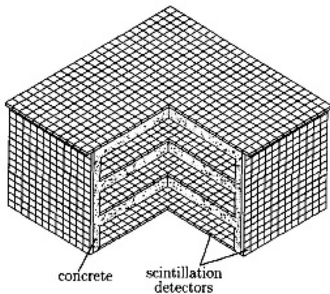
Figure 138: Schematic sectional view of the BUST ( left panel ) and of one of its horizontal scintillator planes ( right panel ).
