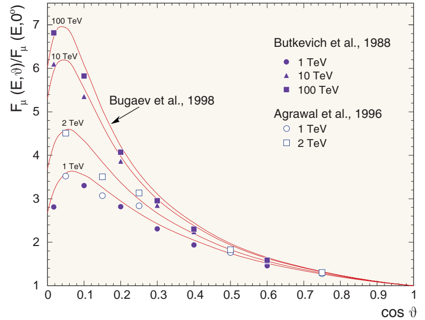
Figure 74: Comparison of the muon angular distributions at sea level predicted by different workers.
