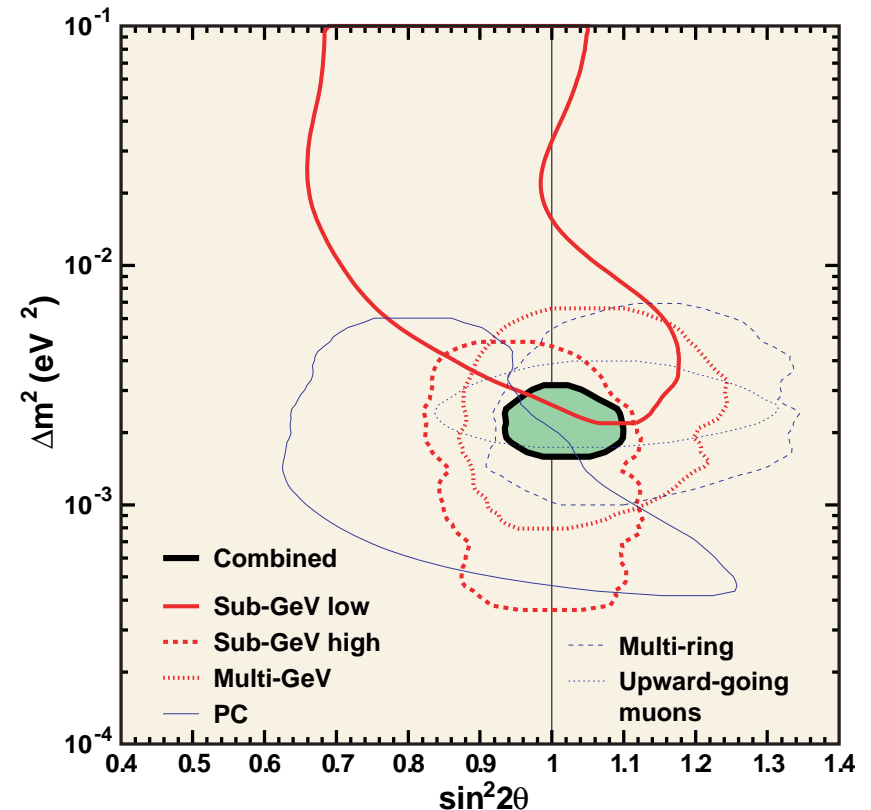
Figure 117: 90% confidence level allowed oscillation parameter regions for \nu_{\mu} \leftrightarrow \nu_{\tau} oscillations from six sub-samples of the SK I. [From Y. Ashie et al. (Super-Kamiokande Collaboration), Phys. Rev. D 71 (2005) 112005 (hep-ex/0501064).]
