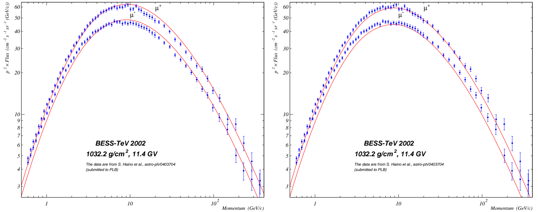
Figure 66: Comparison with the most recent result by BESS-TEV. Calculations are done with the Gaisser-Honda primary spectra: “High Helium” (left) and “Low Helium” (right).
