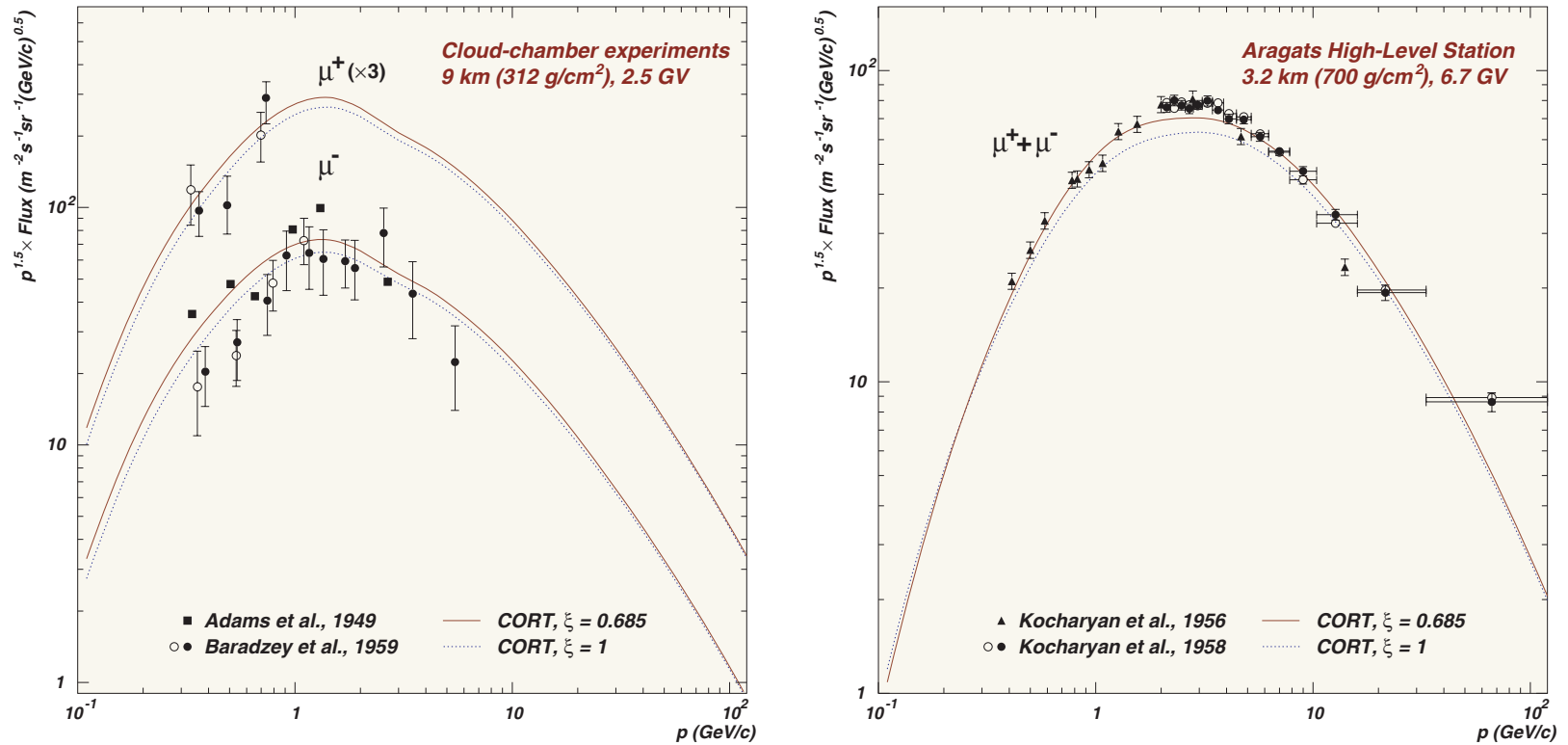
Figure 58: Left panel : differential momentum spectra of \mu^+ and \mu^- measured with cloud chambers on board of airplanes at an altitude of about 9 km above s.l. [Adams et al. (1949), Baradzey et al. (1959)]. Right panel : differential momentum spectrum of \mu^+ + \mu^- at an altitude of 3.2 km above s.l. measured at the Aragats high altitude laboratory (35° N) during the period 1953 to 1956 [Kocharyan et al. (1956, 1958)]. The solid and dashed curves are calculated with the standard CORT interaction model and with the superposition model for interactions of nuclei, respectively.
