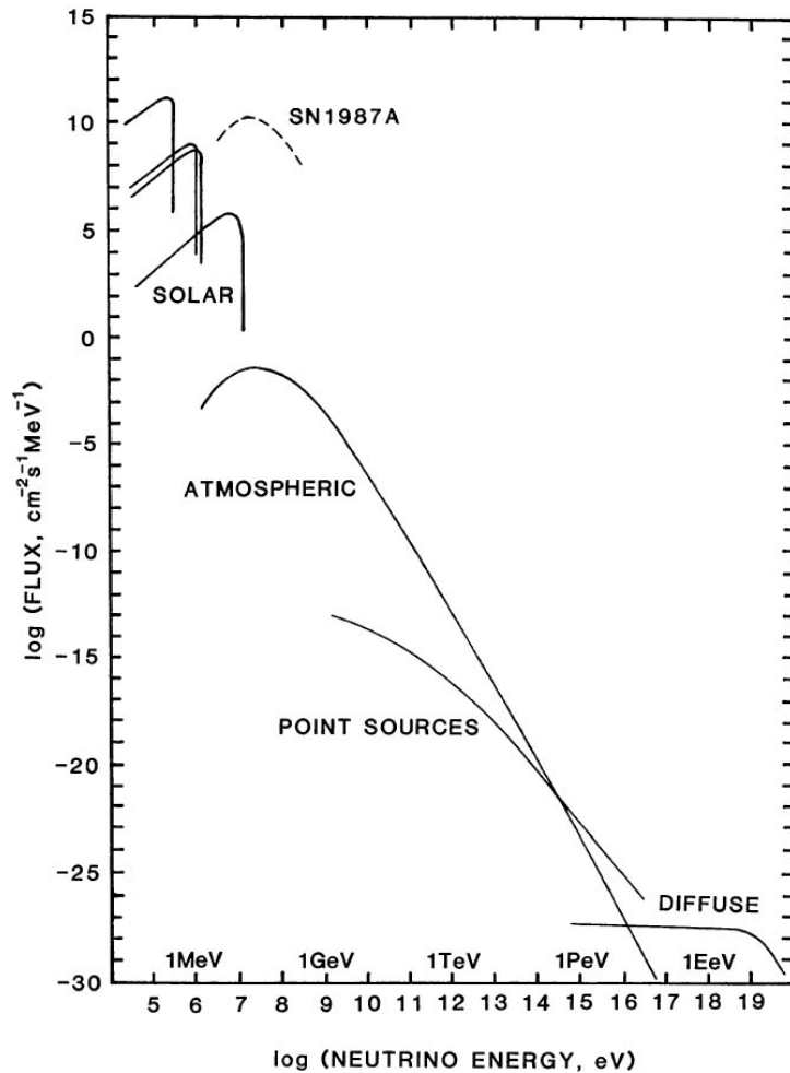
Figure 41: A tentative representation of atmospheric and extraterrestrial neutrino fluxes on the Earth (left) and cross sections for neutrino interactions with nuclei, nucleons and electrons (right). [From A. M. Bakich, "Aspects of neutrino astronomy," Space Sci. Rev. 49 (1989) 259–310.]
