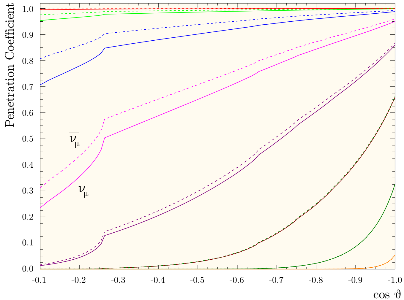
Figure 200: Penetration coefficients for atmospheric \nu_\mu (solid curves) and \bar{\nu}_\mu (dashed curves) vs \cos \vartheta for energies E_\nu = 10^k GeV with k = 3, 4, \dots, 10 from top to bottom.
