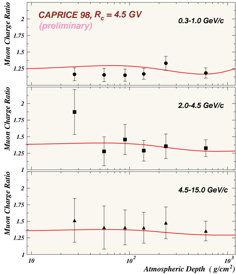
Figure 70: Muon charge ratio as a function of atmospheric depth for three momentum ranges and \langle \vartheta \rangle = 8^\circ . The data points are from the CAPRICE 98 experiment [Hansen et al. (2001) preliminary ]. The curves are calculated with CORT ( \xi = 0.685 ).
