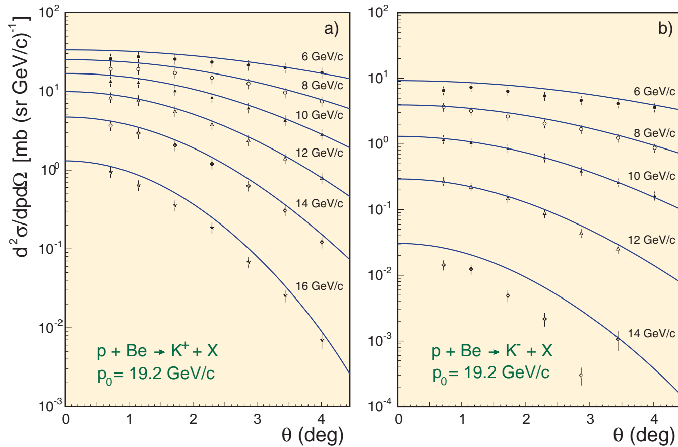
Figure 51: Differential cross sections of K^\pm production in interactions of 19.2 \text{ GeV/c} momentum protons with Be target vs scattering angle. Curves are calculated in the KM model. Kaon momenta are shown near the curves. Data points are from J. V. Allaby et al. , CERN Yellow Report 70–12, 1970 (unpublished).
