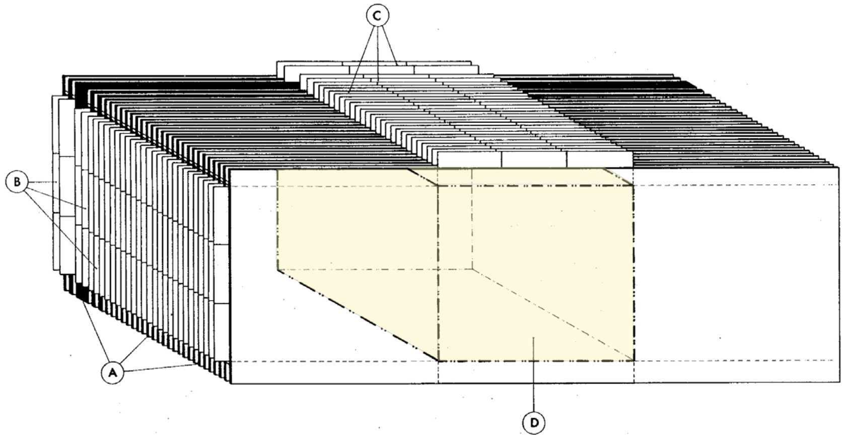
Figure 136: A sketch of the detector used in the NUSEX experiment: (A) the vertical iron plates; (B) the detector tubes plus the x -strips; (C) the y -strips; (D) the fiducial volume. [From G. Battistoni et al. , Nucl. Instrum. Meth. 219 (1984) 300–310.]
