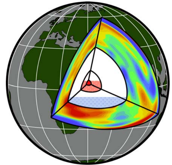
Figure 189: A schematic view of the Earth’s interior.
