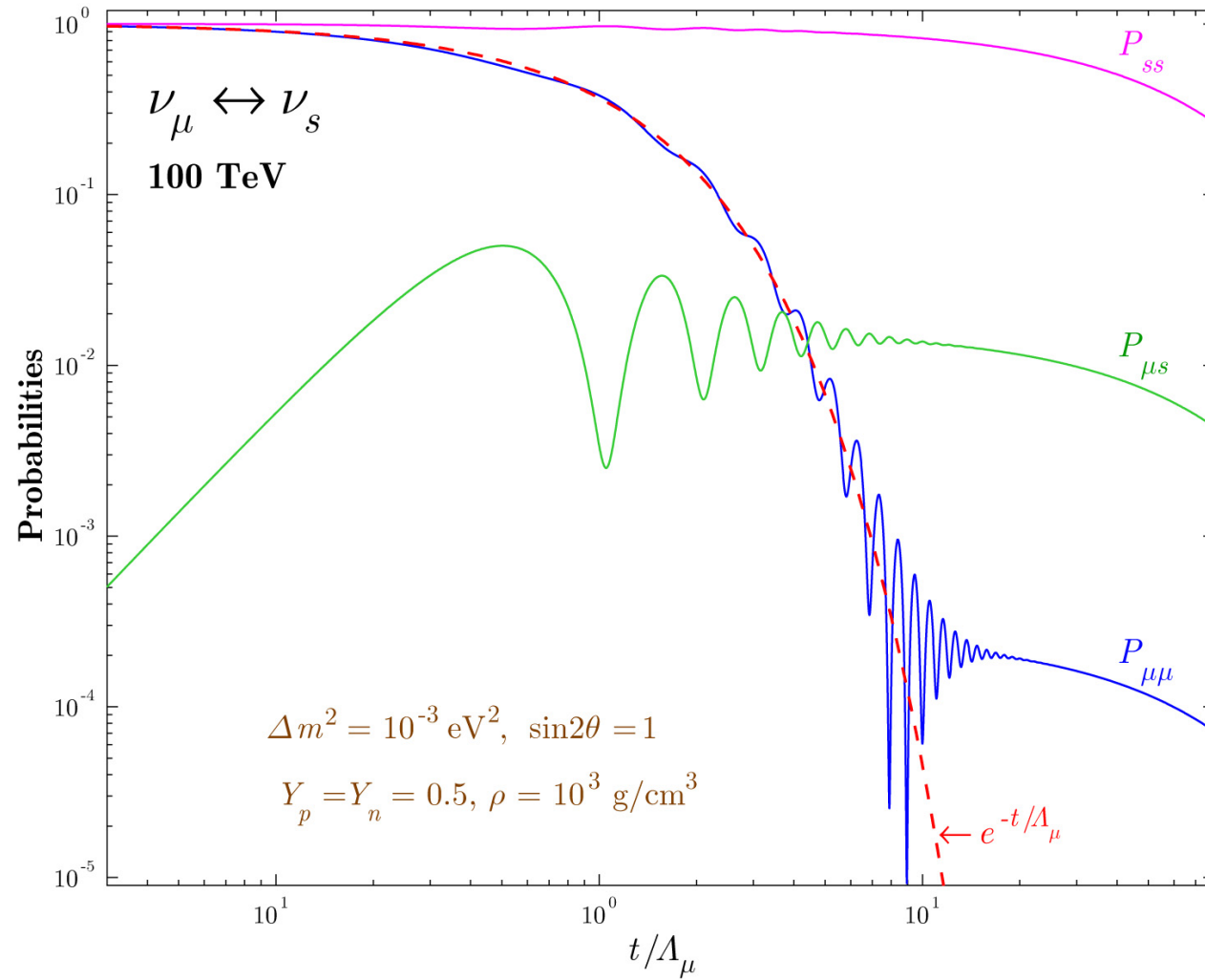
Figure 213: Survival and transition probabilities for \nu_\mu \leftrightarrow \nu_s oscillations ( E_\nu = 100 \text{ TeV} , \rho = 10^{-3} \text{ g/cm}^3 ).
