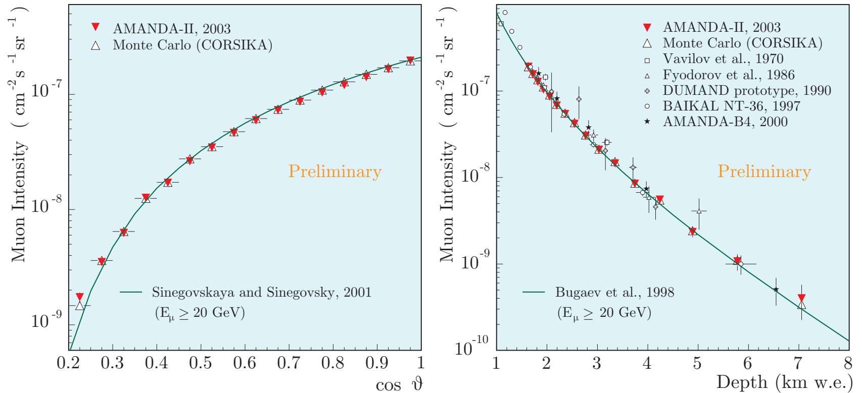
Figure 91: Preliminary zenith angle distribution of muons ( left panel ) and vertical muon DIR ( right panel ) measured with AMANDA-II. The data of some earlier experiments (c. f. Fig. 89) and MC calculations with CORSIKA are also shown. The AMANDA-II unfolded data are normalized to the vertical MC point. The curves are from Bugaev et al. (1998) and Sinegovskaya & Sinegovsky (2001).
