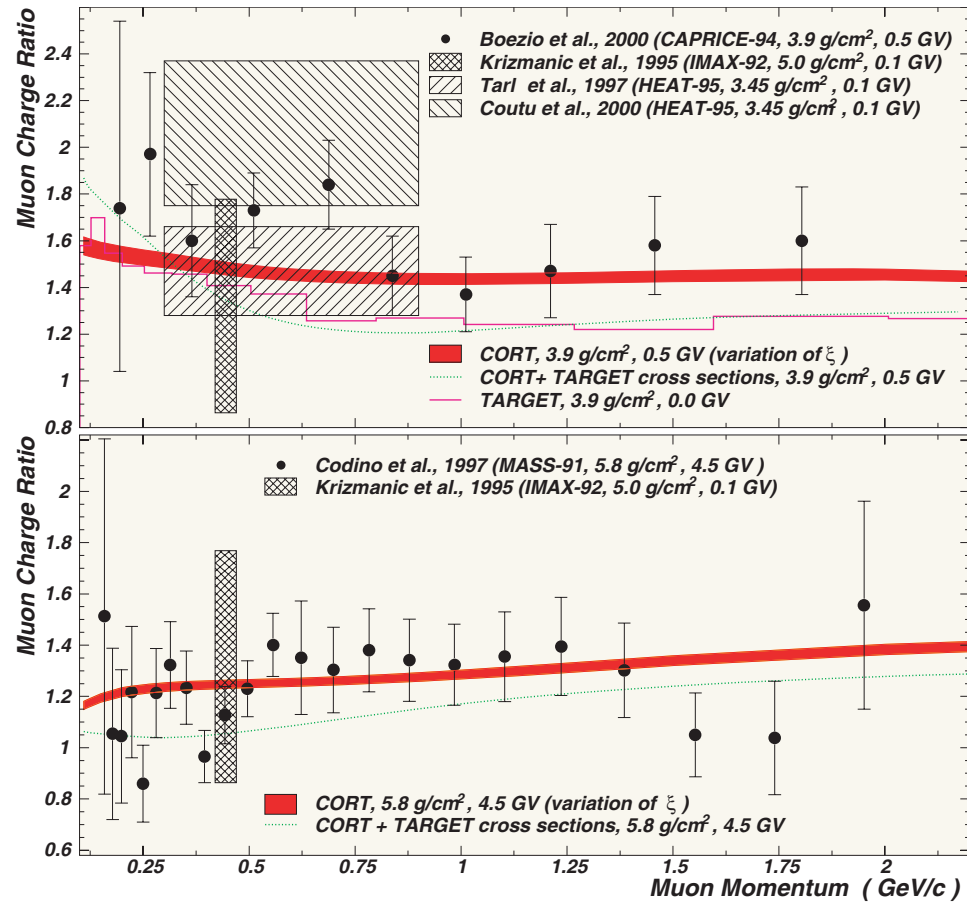
Figure 68: Muon charge ratio near the top of the atmosphere for \langle \vartheta \rangle = 9^\circ . The points and shaded rectangles represent the data from many experiments. The curves and filled areas are the results of calculations with CORT, TARGET-1 and “CORT+TARGET”.
