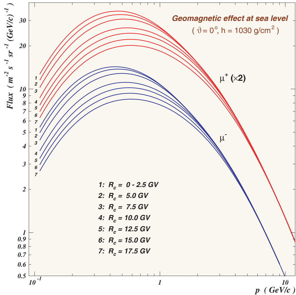
Figure 53: Expected geomagnetic effect for vertical atmospheric muons at sea level.
