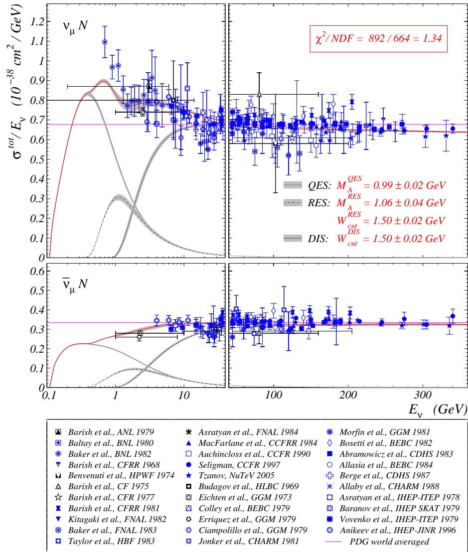
Figure 42: Comparison of theoretical estimation of the CC total cross sections for \nu_\mu N and \bar{\nu}_\mu N interactions with world survey experimental data. The main contributions, – quasi-elastic scattering (QES), single-pion production through baryon resonances (RES) and deep-inelastic scattering (DIS) are calculated with the best-fitted values of the parameters depicted in the legend in top panel. Uncertainties of the main contributions and their sum are shown by the bands. The averaged values (0.677 \pm 0.014) \times 10^{-38} (for \nu_\mu N ) and (0.334 \pm 0.008) \times 10^{-38} \text{ cm}^2/\text{GeV} (for \bar{\nu}_\mu N ) suggested by the Particle Data Group are shown by straight lines.
