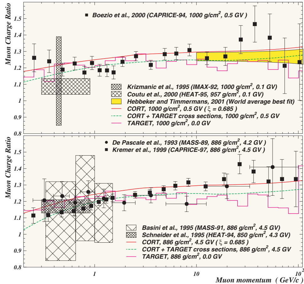
Figure 69: Muon charge ratio at ground level for \langle \vartheta \rangle = 9^\circ . The points and shaded rectangles represent the data from many experiments. The curves and filled areas are the results of calculations with CORT, TARGET-1 and “CORT+TARGET”, and the best fit obtained by Hebbeker and Timmermans (2001) from many data at p \geq 10 GeV/c.
