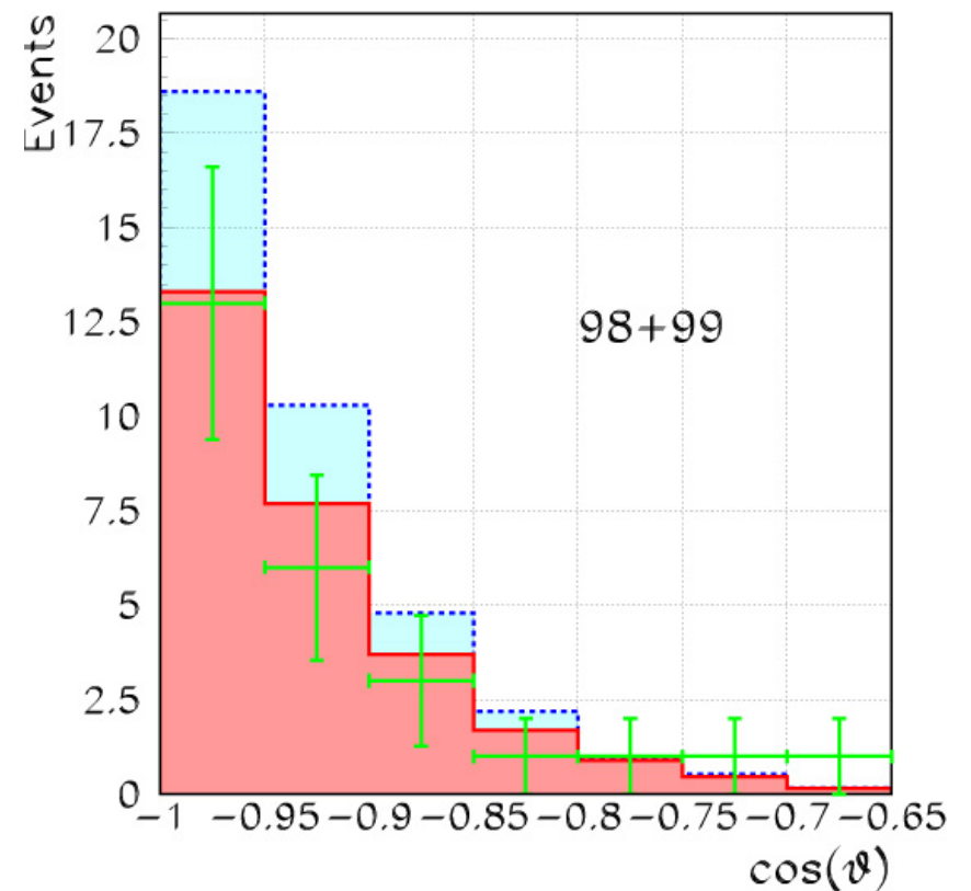
Figure 163: The same as in Fig. 162 but for selected neutrino candidates. E_{\text{th}} = 10 \text{ GeV} .
