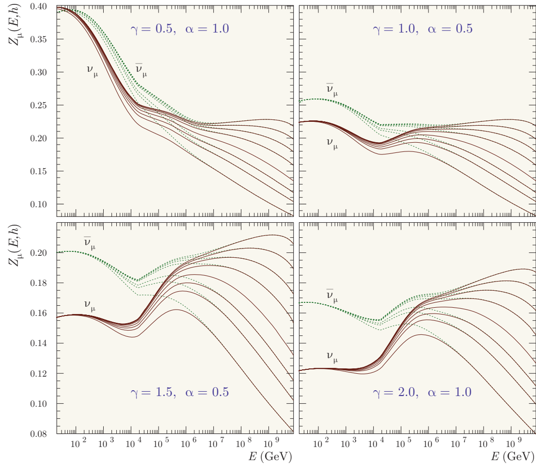
Figure 196: Z factors, Z_{\bar{\nu}_\mu}(E, h) and Z_{\nu_\mu}(E, h) vs energy for the initial spectra (133), calculated with four different sets of \gamma and \alpha with E_0 = 1 PeV for depths h = h_\oplus/k [ k = 1, 2, 3, 5, 10, 20, 50 from bottom to top] and h = 0 (the largest Z factors).
