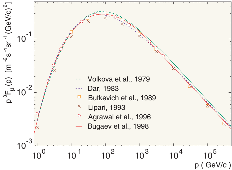
Figure 73: Comparison of the vertical momentum spectra of conventional muons at s.l. predicted by different workers.
