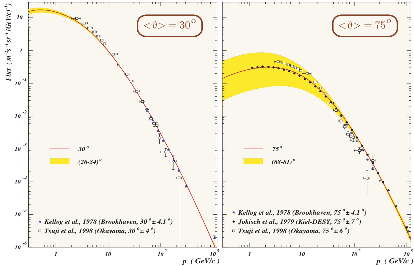
Figure 61: Differential momentum spectra of muons at s.l. for \vartheta = 30^\circ and 75^\circ . The data points are from the Brookhaven magnetic spectrometer [Kellogg et al. (1978)], Kiel-DESY muon spectrometer at Hamburg [Jokisch et al. (1979)] and Okayama cosmic-ray telescope [Tsuji et al. (1998)]. The filled areas display the expected flux variations inside the angular bins while the solid curves correspond to the average zenith angles.
