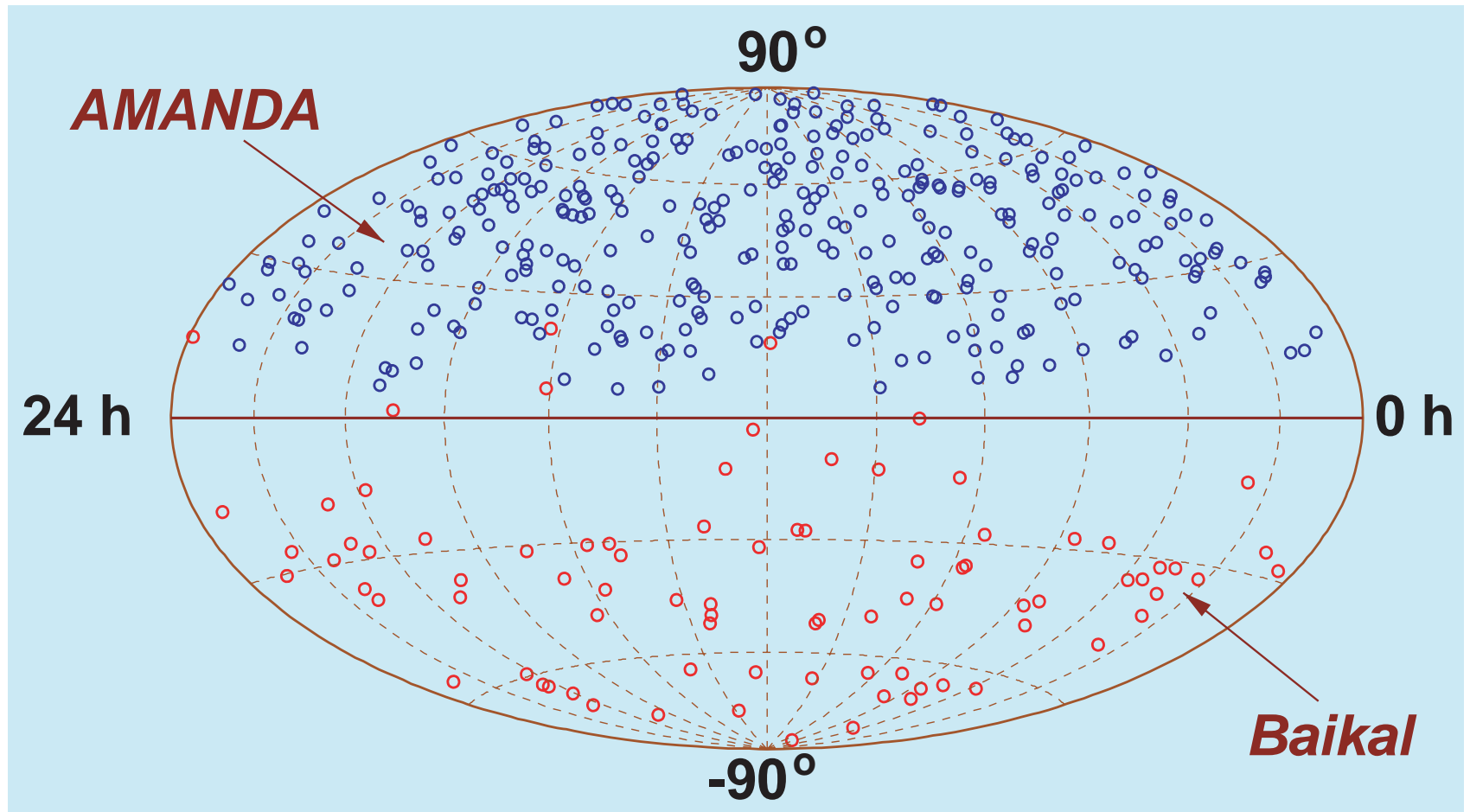
Figure 178: Merged skyplot of upward-going events recorded in both Baikal NT-200 and AMANDA-B10 experiments. The data are the same as in Figs. 161 and 177.
