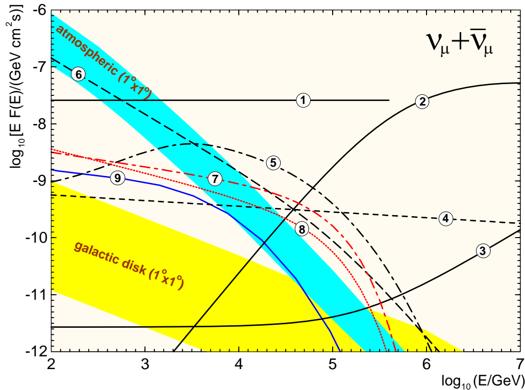
Figure 203: Summary of expected \nu_{\mu} + \bar{\nu}_{\mu} from candidate cosmic-ray accelerators (“point sources”).
