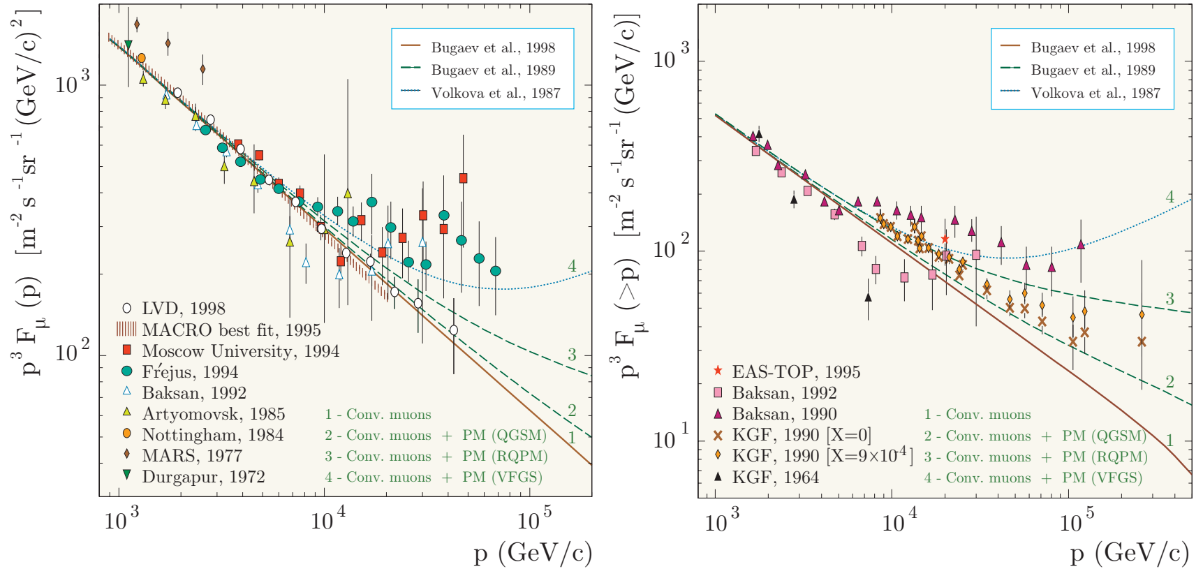
Figure 75: Differential ( left panel ) and integral ( right panel ) momentum spectra of muons at sea level for \vartheta = 0^\circ and p > 1 TeV. The prompt muon contributions are evaluated with the three models for charm hadroproduction: recombination quark-parton model (RQPM), quark-gluon string model (QGSM) and a semiempirical, QGSM inspired model by Volkova et al. (VFGS).
