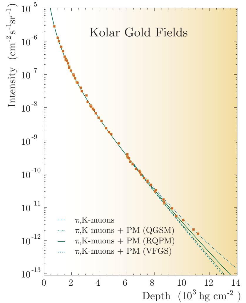
Figure 82: \mu DIR from KGF.
