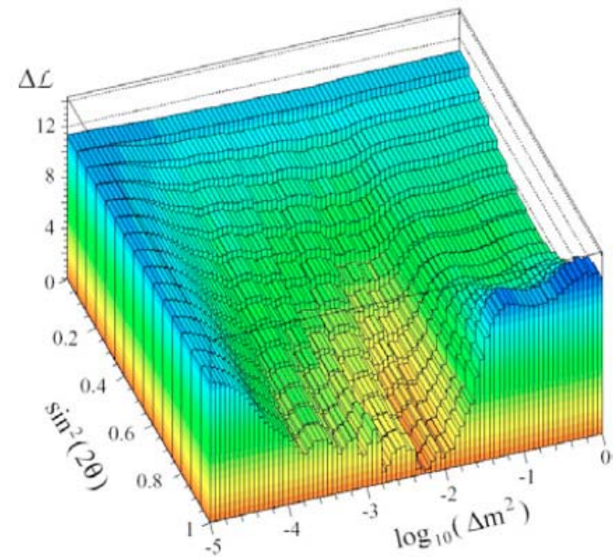
Figure 135: The data likelihood difference.
