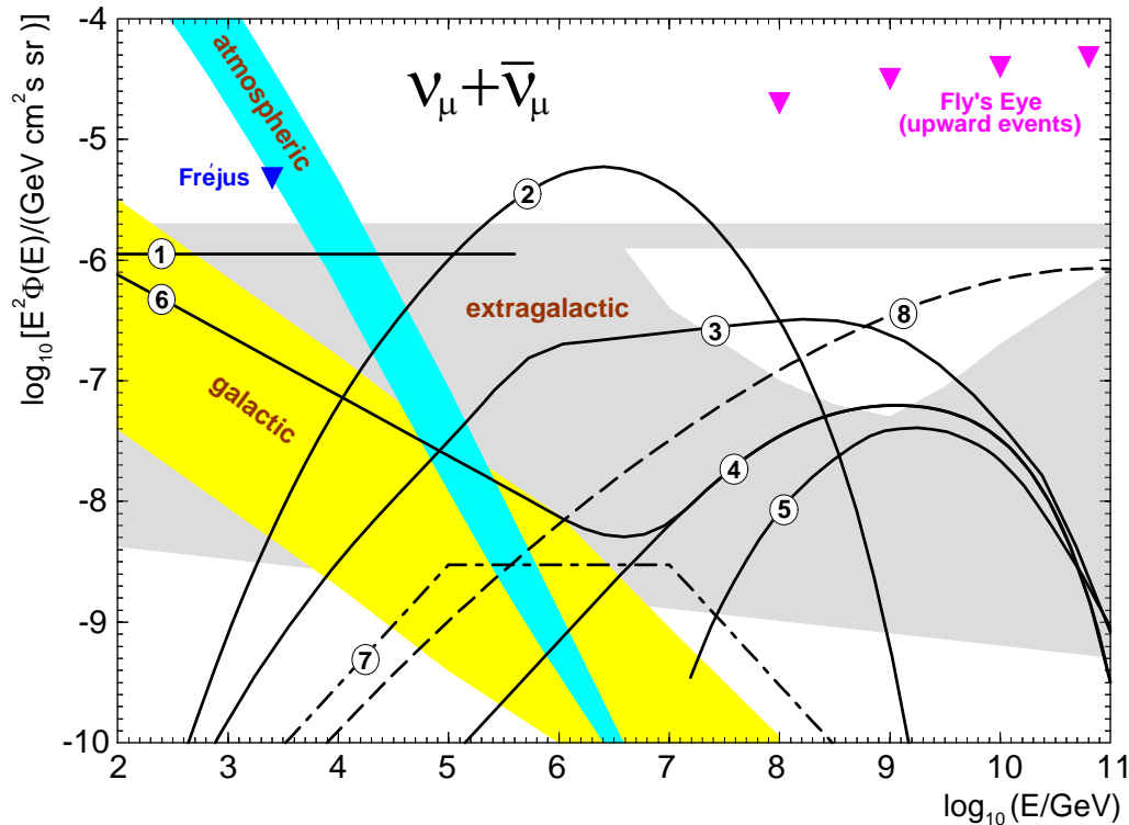
Figure 202: Summary of expected \nu_\mu + \bar{\nu}_\mu intensities for diffuse emission from various sources. The experimental data (triangles) are from Frejús proton decay detector (limit on any excess above the atmospheric background) and Fly's Eye fluorescence air shower detector (limits on upward events).
