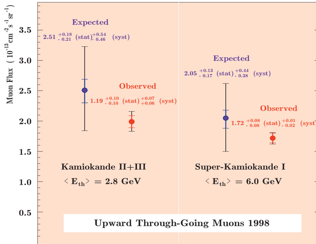
Figure 141: Expected and observed total fluxes of upward through-going muons for Kamiokande II+III and Super-Kamiokande I. [From S. Hatakeyama, “Search for muon neutrino oscillations in Kamiokande and Super-Kamiokande,” Ph.D. thesis (1998).]
