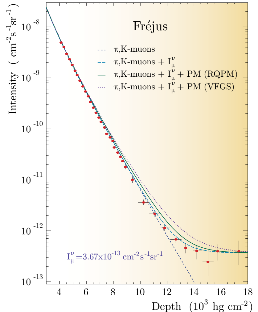
Figure 88: \mu\text{DIR} from Frèjus.
