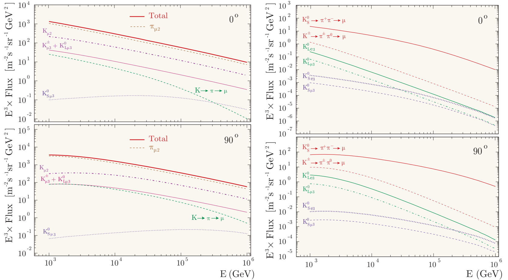
Figure 72: Separate contributions from different meson decay modes and chains into the total muon flux at \vartheta = 0^\circ and \vartheta = 90^\circ for energies above 1 TeV.
