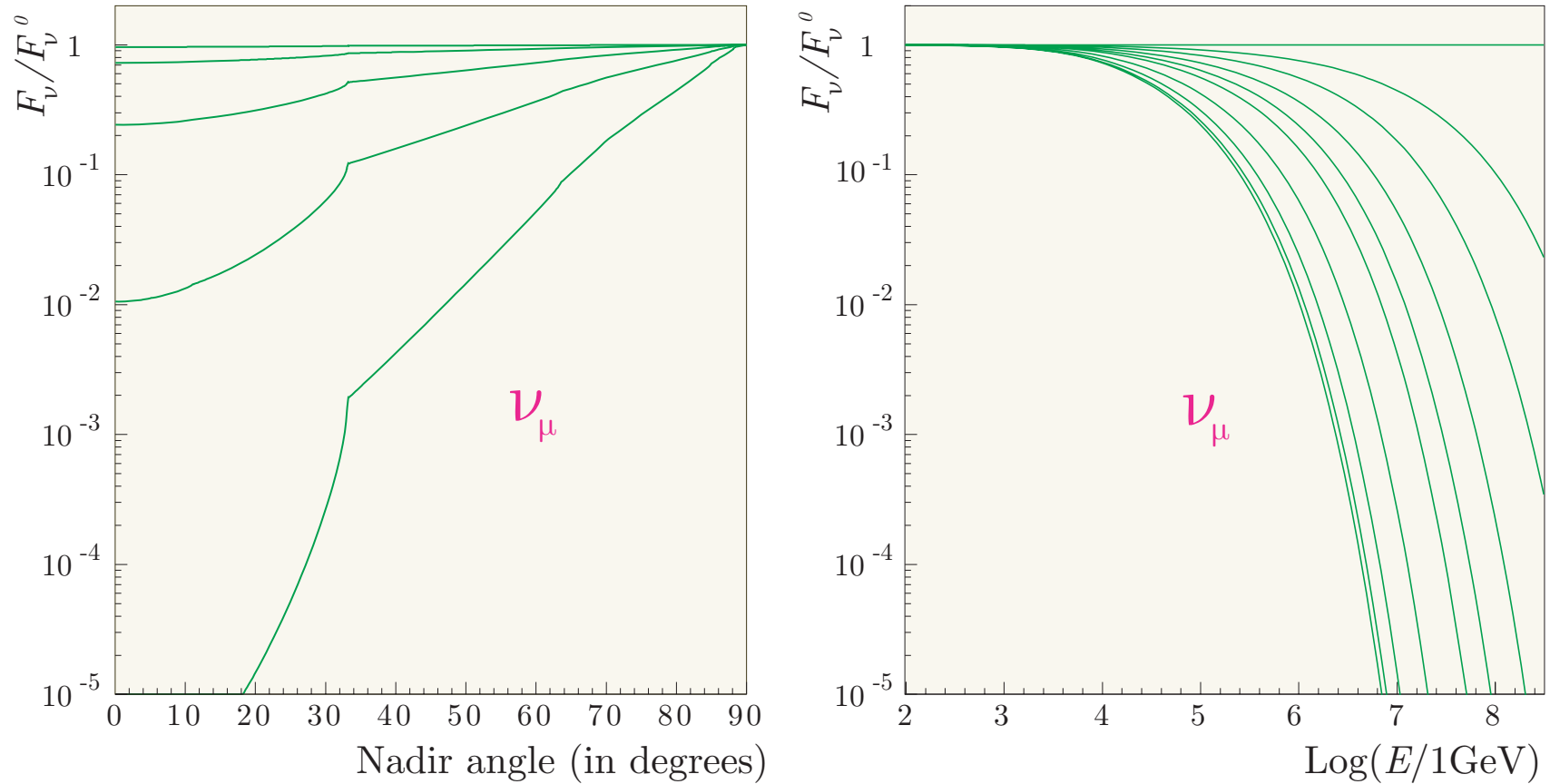
Figure 197: Muon neutrino penetration coefficients in the Earth for the quasi-power-law initial spectrum with \gamma = 0.7 . Left panel: as a function of \vartheta for E = 10^k GeV [ k = 3, 4, \dots, 7 from top to bottom]. Right panel: as a function of E at fixed nadir angles [ 0^\circ to 90^\circ from bottom to top with steps of 10^\circ ].
