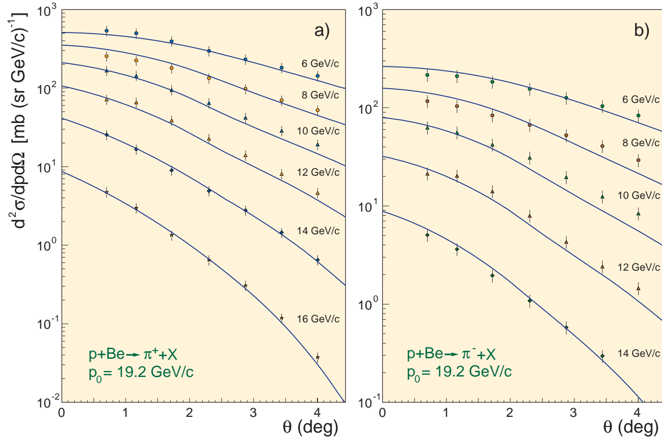
Figure 50: Differential cross sections of \pi^\pm production in interactions of 19.2 GeV/c momentum protons with Be target vs scattering angle. Curves are calculated in the KM model. Pion momenta are shown near the curves. Data points are from J. V. Allaby et al. , CERN Yellow Report 70–12, 1970 (unpublished).
