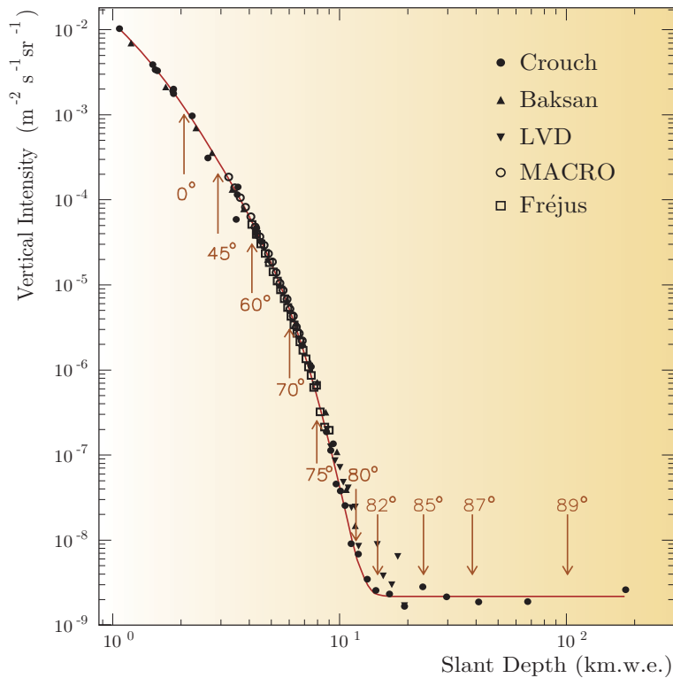
Figure 81: Yet another view of the muon DIR. Arrows indicate the average depth at different zenith angles at the SOUDAN2 detector. The curve represents the fitting formula by Crouch (127). [From D. Demuth et al. , hep-ex/0304016.]
