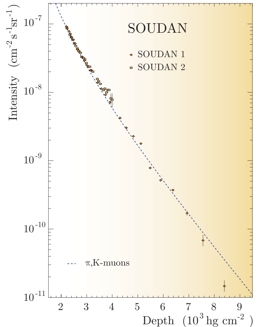
Figure 85: \mu DIR from SOUDAN 1 and 2.
