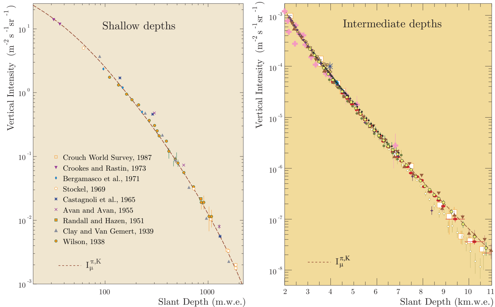
Figure 80: Fragments of Fig. 79 for shallow (left) and intermediate (right) depths.
