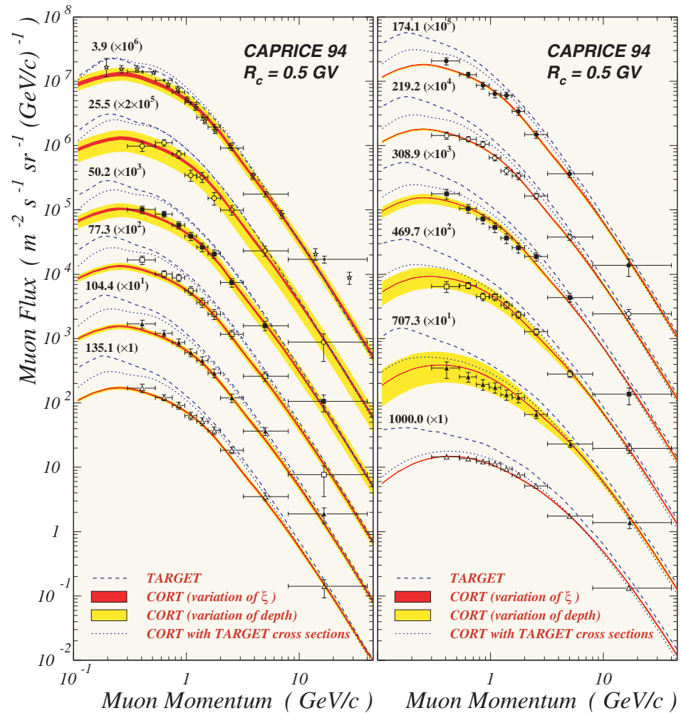
Figure 57: Differential momentum spectra of \mu^- for 12 depth ranges. The data points are from the CAPRICE 94 experiment [Boezio et al. (2000)]. The curves and filled areas are the results of calculations with CORT, TARGET-1 and “CORT+TARGET”.
