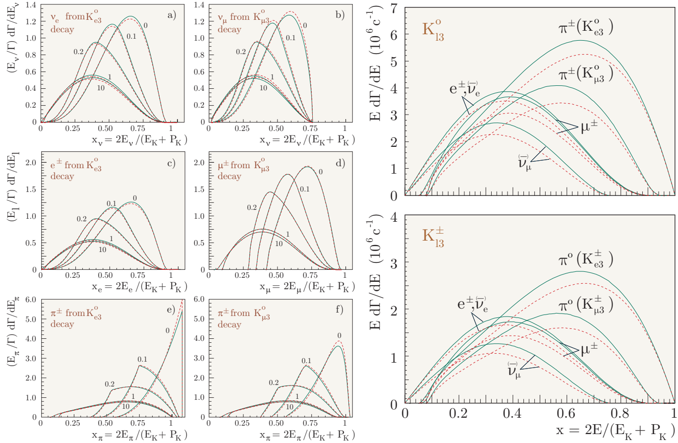
Figure 47: Normalized and absolute distributions of secondary particles from K_{l3} decays evaluated with (solid lines) and without (dashed lines) form factors. The numbers near the curves denote the kaon momenta (in \text{GeV}/c ). The absolute differential widths (two right panels) are evaluated for ultrarelativistic K_L^0 and K^\pm mesons.
