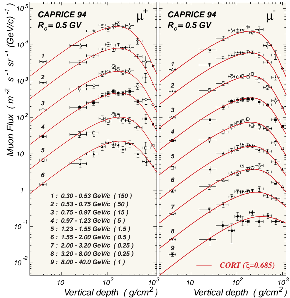
Figure 55: Atmospheric growth curves for \mu^+ and \mu^- . The data points are from the CAPRICE 94 experiment [Boezio et al. (2000)].
