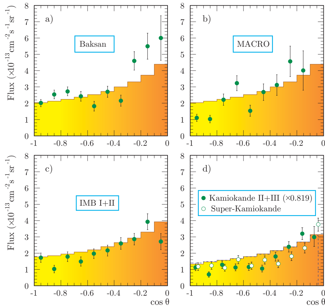
Figure 140: Zenith-angle distributions of upward through-going muons observed in 5 experiments.
