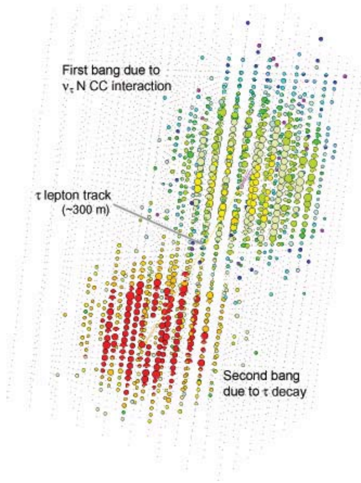
Figure 185: A “double-bang” \nu_\tau induced even simulation in IceCube.
