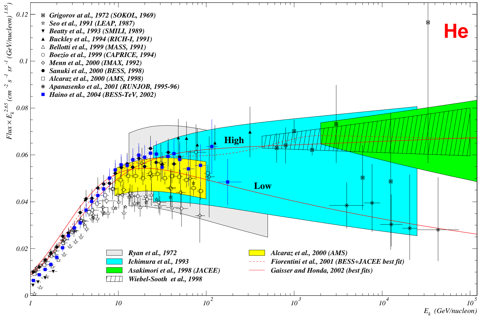
Figure 64: Gaisser-Honda models for primary helium.
