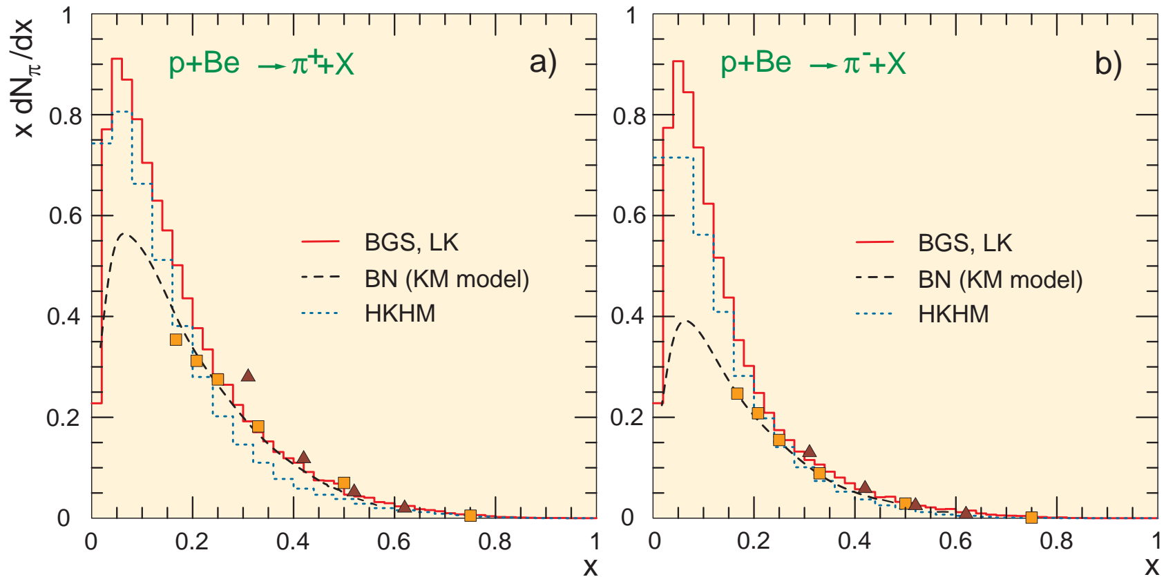
Figure 48: Inclusive spectrum of charged pions produced in interactions of \approx 20 GeV/c momentum protons with Be target. Models are shown for air target (abbreviations are the same as in Figs. 98 and 99). Data points are from J. V. Allaby et al. , CERN Yellow Report 70–12, 1970 (unpublished) and T. Eichten et al. , Nucl. Phys. B 44 (1972) 333 for Be target.
