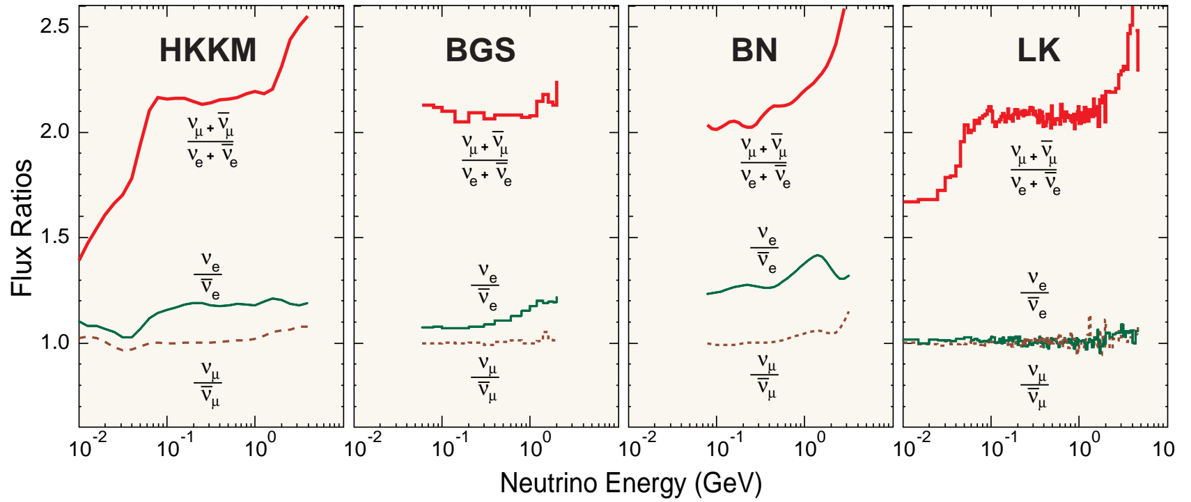
Figure 99: Early calculations of the low-energy 4\pi averaged AN flux ratios for Kamioka site. Notation is the same as in Fig. 98.
