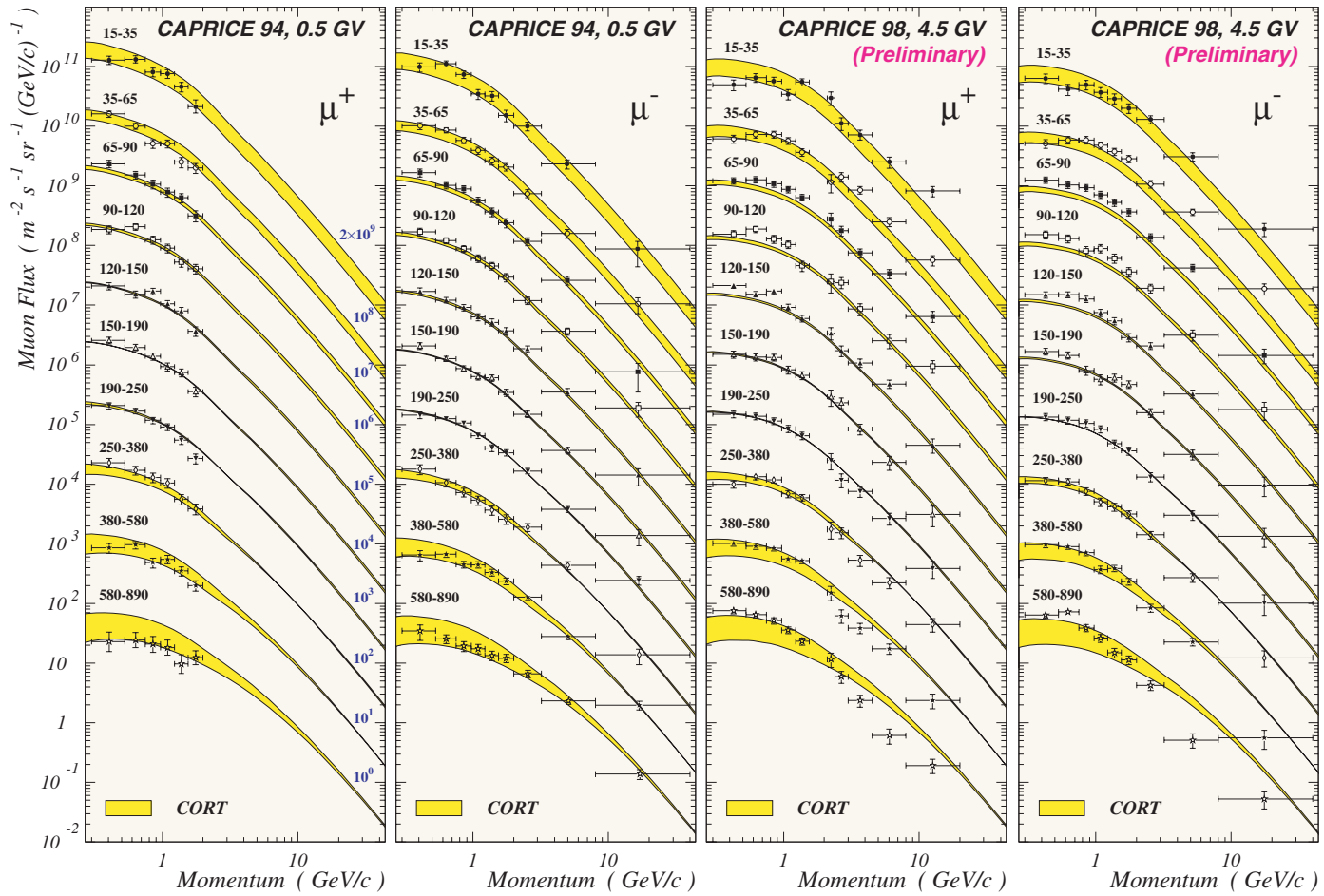
Figure 54: Differential momentum spectra of \mu^+ and \mu^- for 10 depth ranges \Delta h_i . The data points are from the CAPRICE 94 [Boezio et al. (2000)] and CAPRICE 98 [Hansen et al. (2001)] ( preliminary ). The filled areas display the expected flux variations within the ranges \Delta h_i . The data are scaled with the factors indicated on the left panel.
