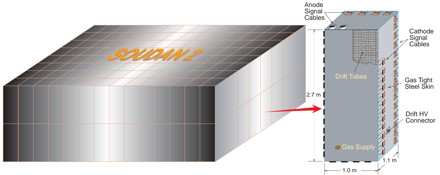
Figure 129: Schematic view of the SOUDAN 2 detector and its module (zoomed).
